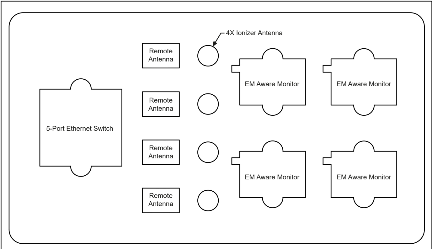
Figure 3. Item compartments
