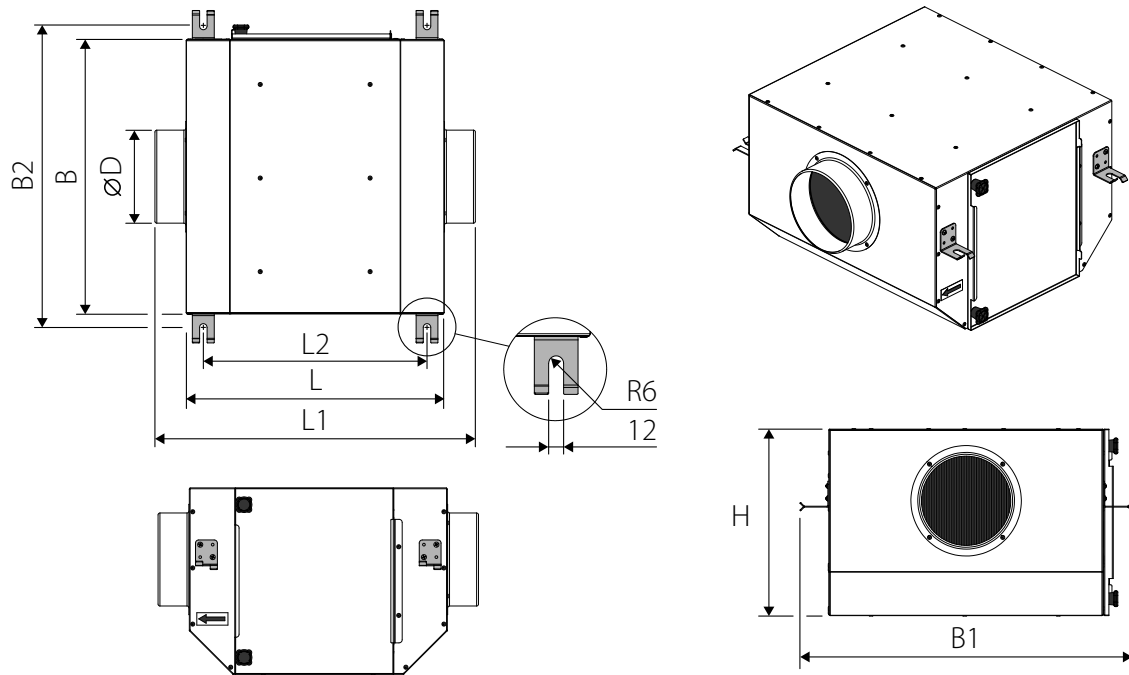
Overall dimensions of the unit [mm]
