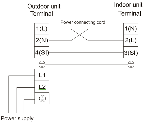
Outdoor unit connected to a wall-mounted indoor unit
