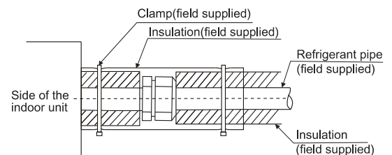
Piping insulation procedure
