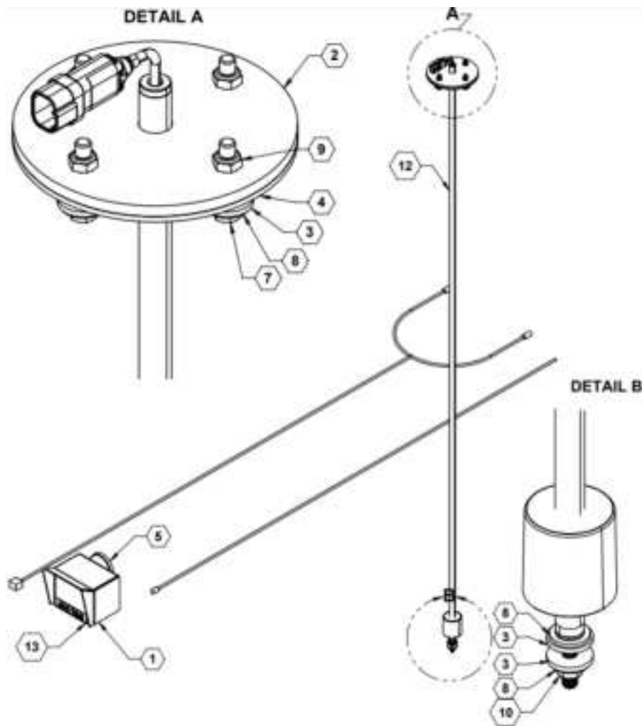
Parts List 37976: Sight Gauge, Electric, Rota
