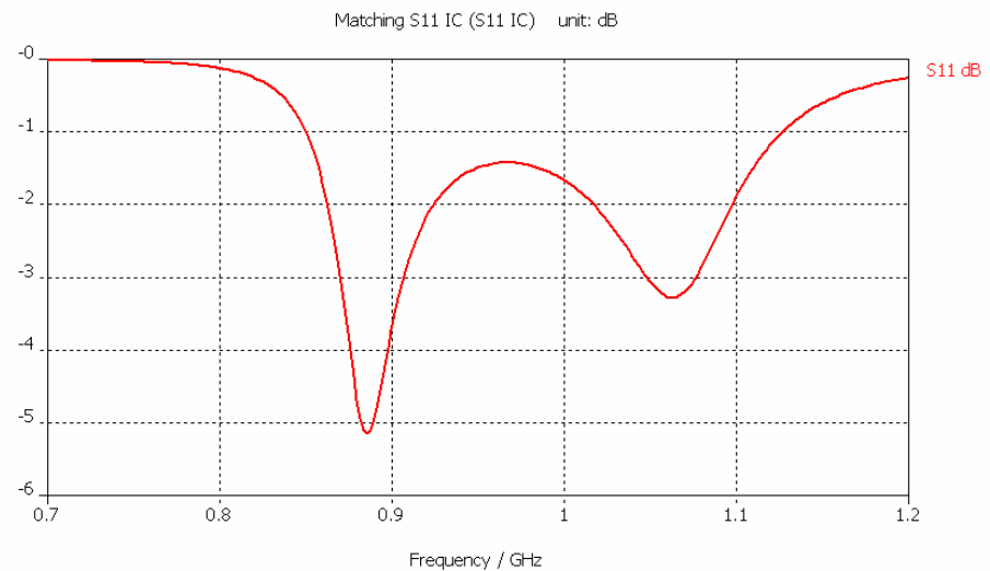
Fig 29. Reflection Coefficient S11
