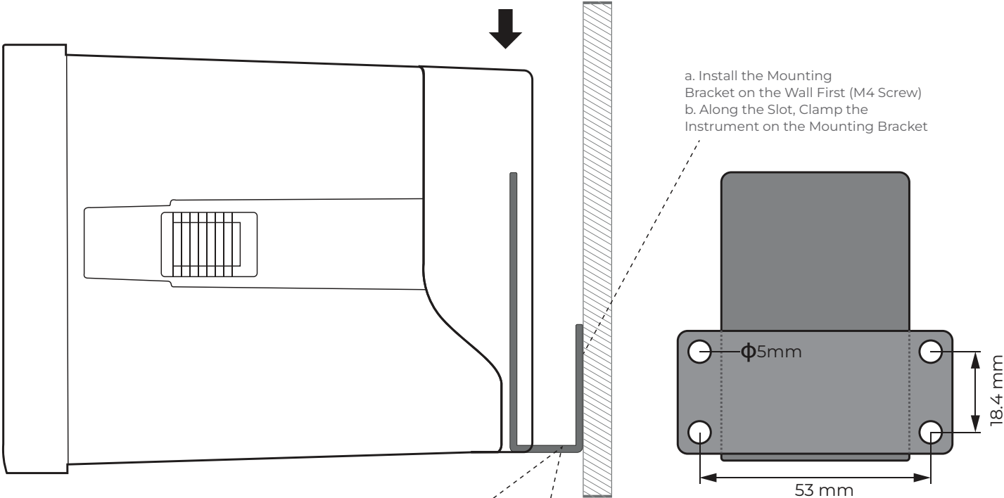
Wall Mount Installation Diagram
