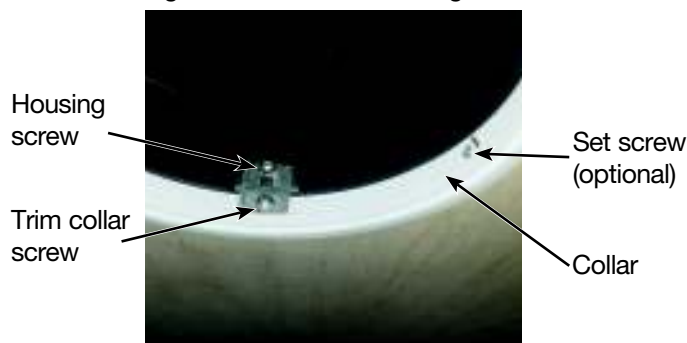
Figure 2: Collar and Locking Screws
