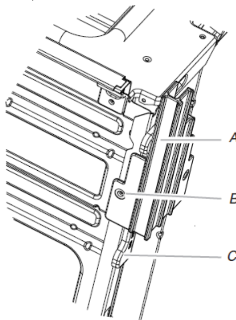
A. Spacers B. Foot C. #8-18 x \frac{3}{8} " screw.
