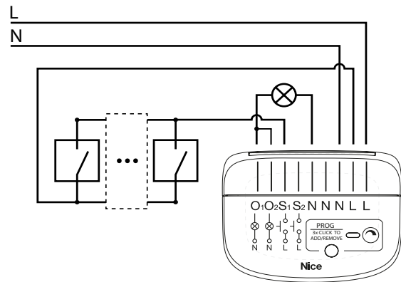
Diagram 5: Momentary switches ×1 - connected outputs
