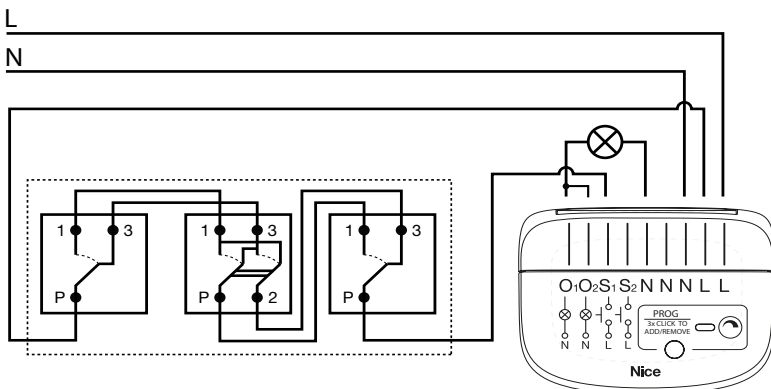
Diagram 7: Stair-cross switches ×1 - connected outputs
