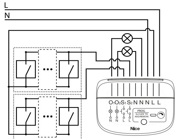
Diagram 6: Momentary switches ×2 - independent outputs
