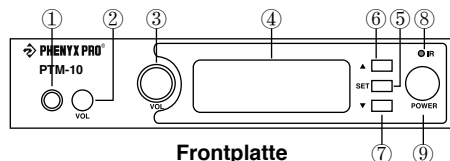
Frontplatte
