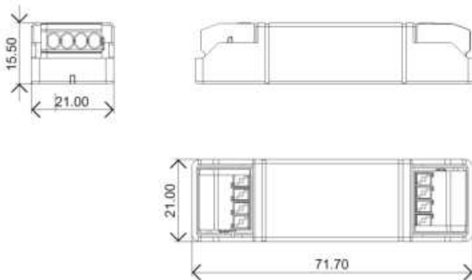
Figure 12: Mechanical dimensions
