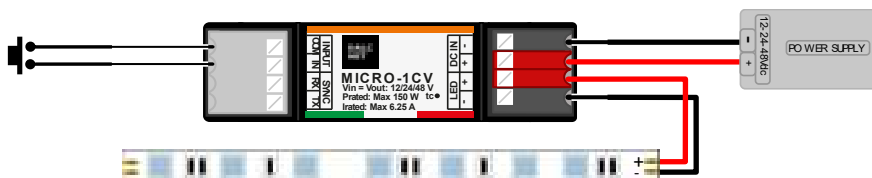
Figure 2: White or Single-Color LED loads wiring diagram
