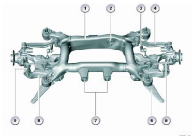
Rear Axle
