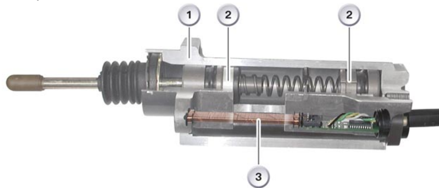
Clutch Slave Cylinder
