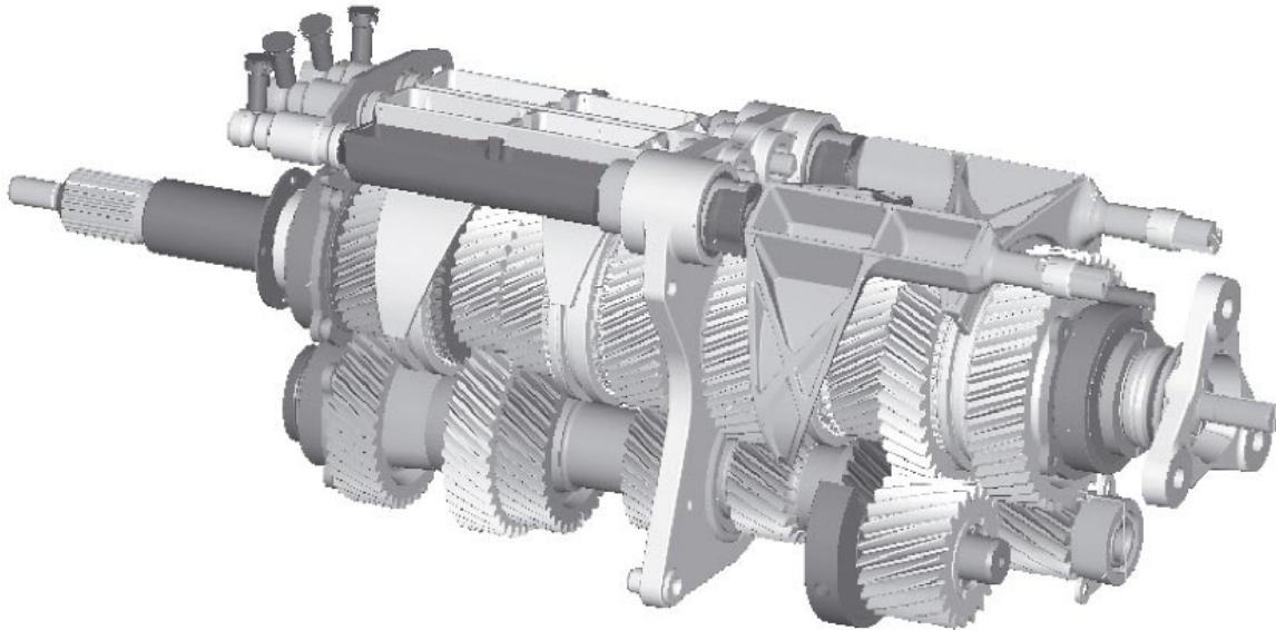
Pinion Arrangement of the SMG Getrag 247
