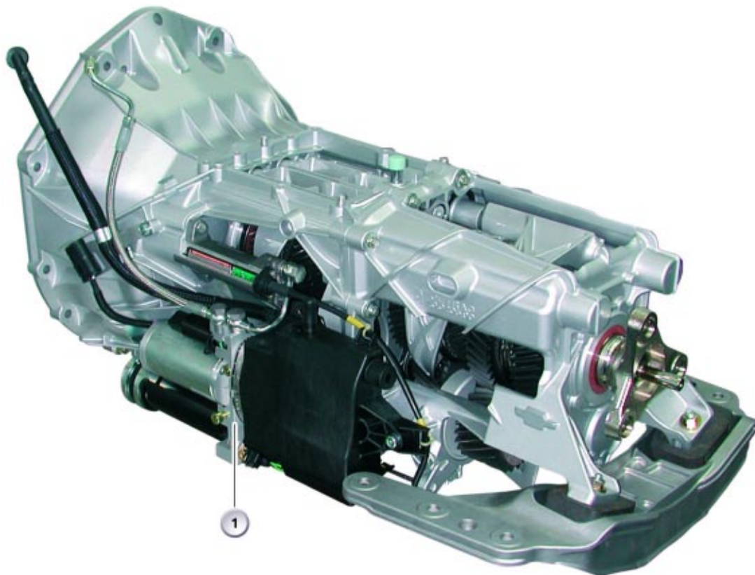
SMG with Hydraulic Unit
