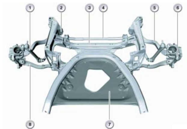
Front Axle
