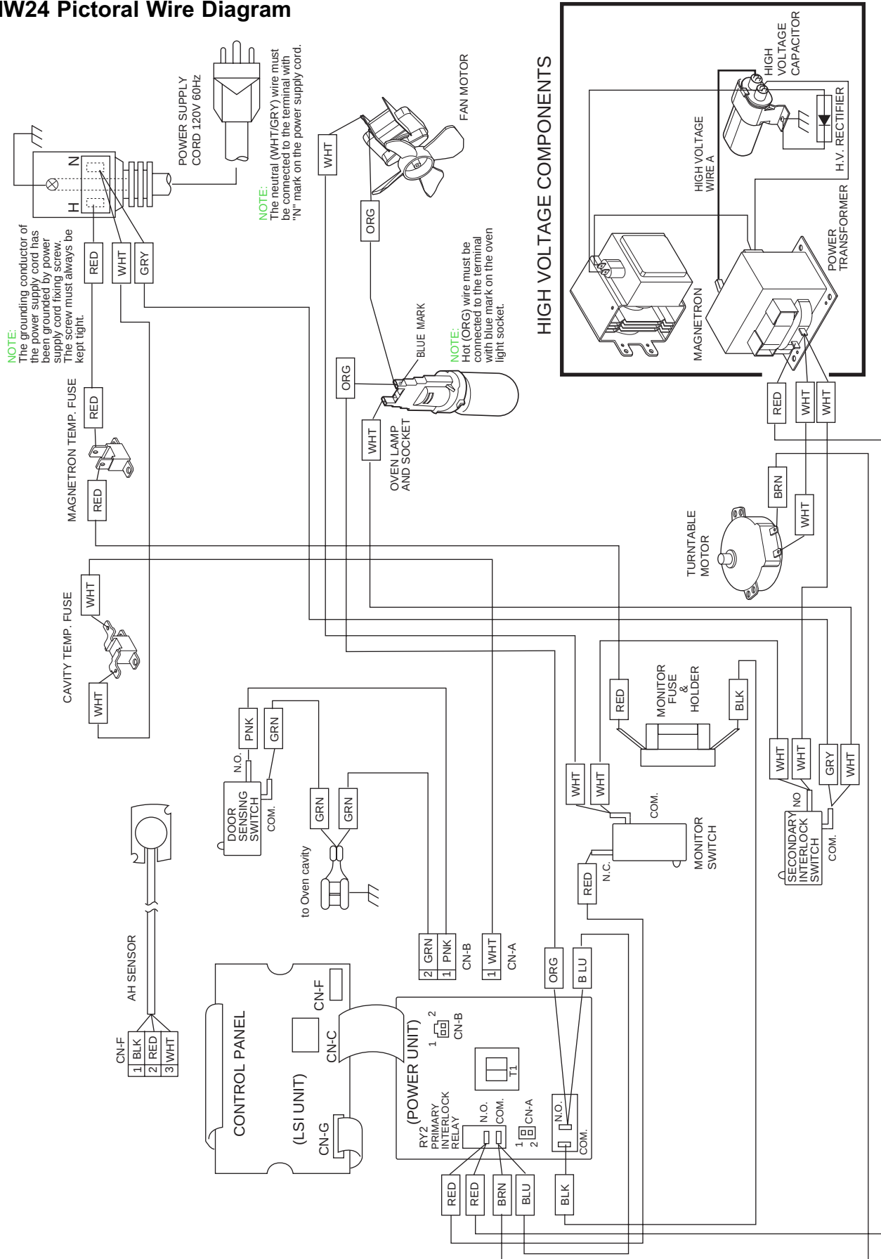
Pictorial Diagram
