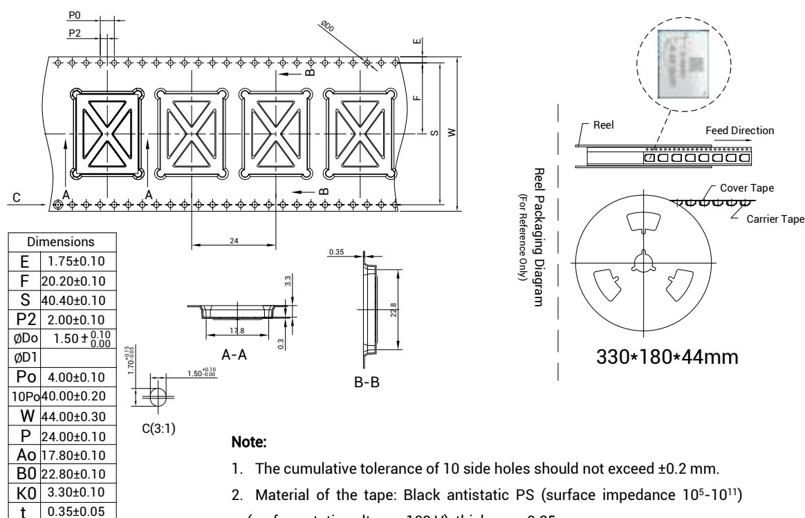
Figure 5-2 UM981S Package
