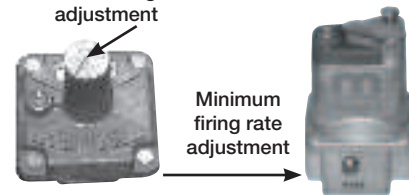
Fig. 4 Separate Regulator & Modulating Valves
