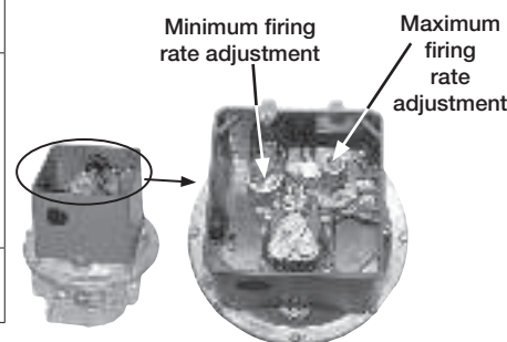
Fig. 5 Combined Modulating Regulator
