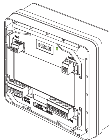
Fig. 2 Connector Side
