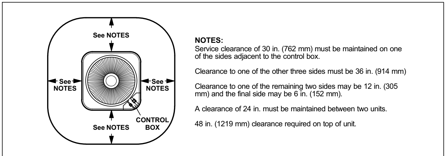
Figure 2. Installation Clearances
