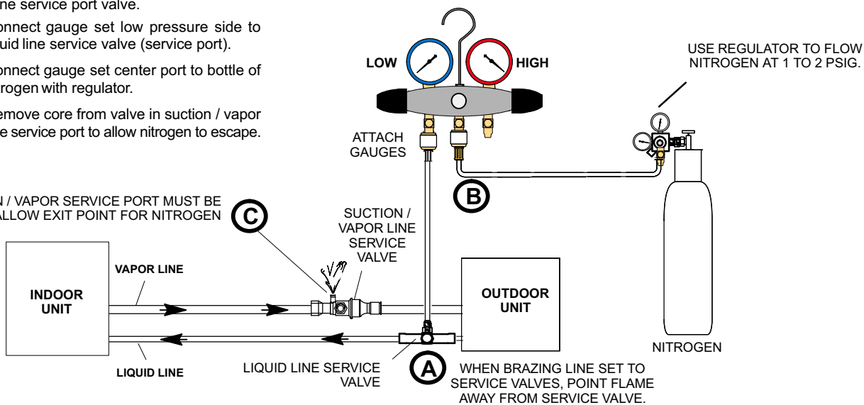
Figure 7. Brazing Procedures
