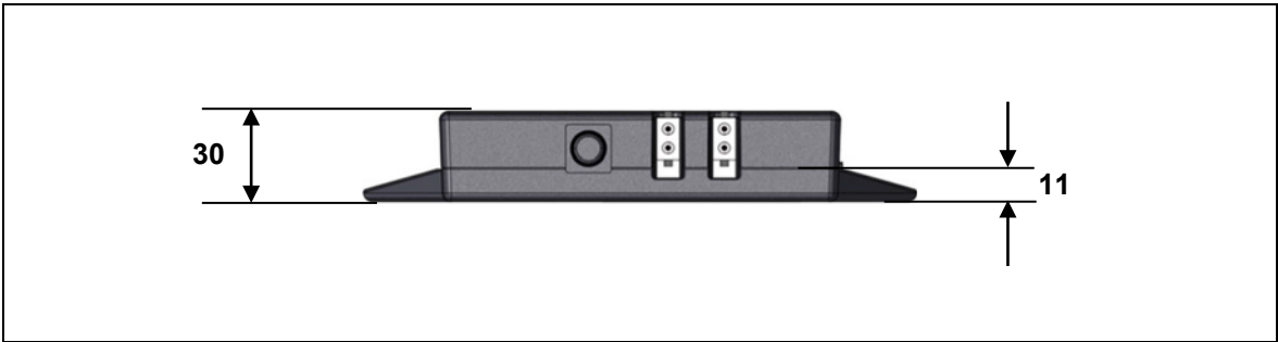
Figure 4 Dimensions of the CONTROL UNIT, side view (in mm)
