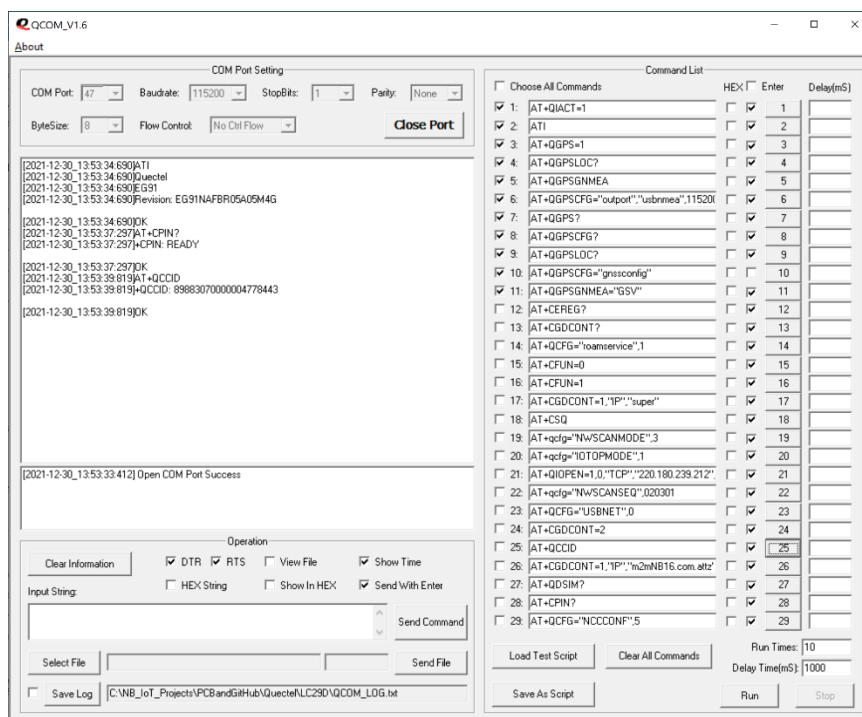
Figure 14: More AT commands examples using QCOM tool.
