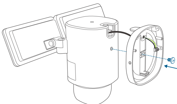
Wall Mounting
