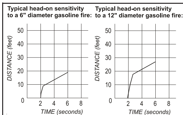
Figure 2 Model 30-2021E-24 Detector Sensitivity
