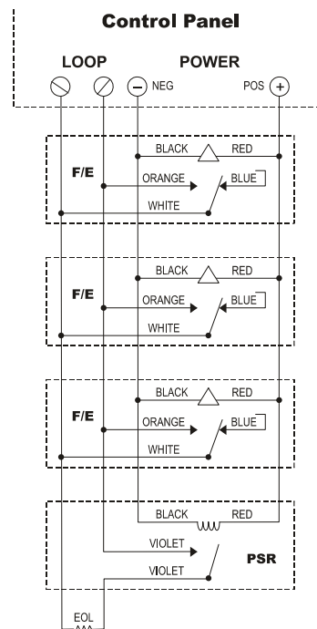
Figure 8 Single Loop Panel Wiring
