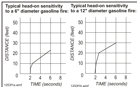
Figure 1 Model 30-2021-24 Detector Sensitivity
