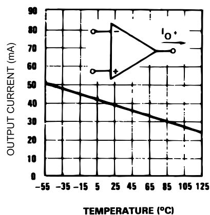
Figure 5: Output current limitation
