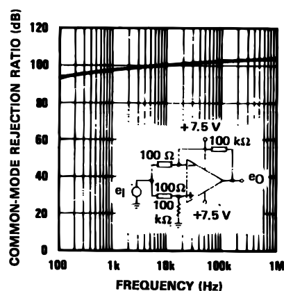
Figure 9: Common-mode rejection ratio
