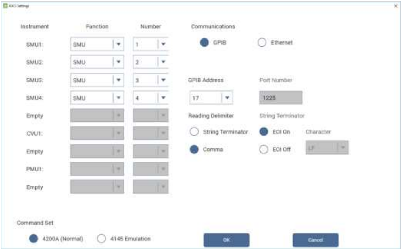
Figure 9. KXCI settings screen for GPIB control.
