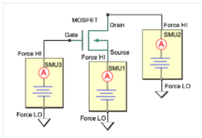
Figure 13. MOSFET circuit diagram using three SMUs.
