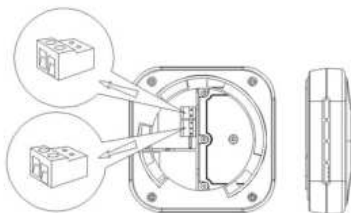
Figure 7. Unplug the terminal block
