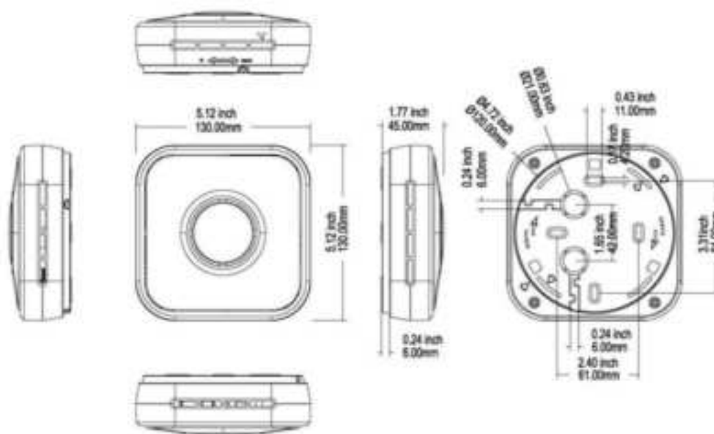
Figure 3. Device Dimensions
