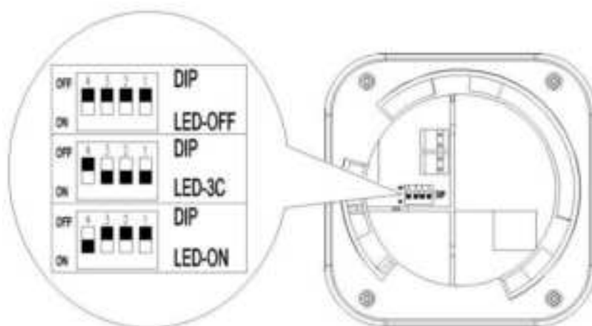
Figure 2. DIP switches
