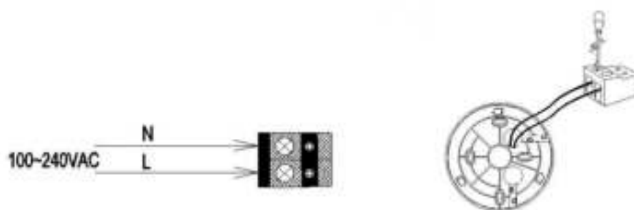
Figure 8. Connect to the terminal block
