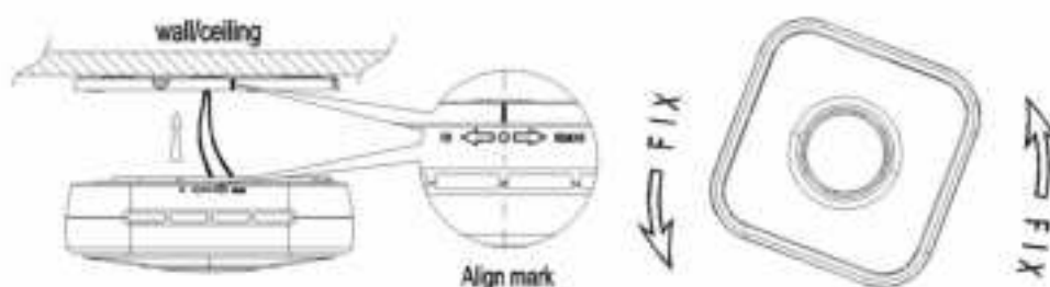
Figure 10. Attach the sensor to the backplane
