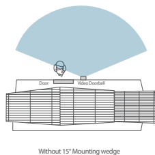
Without 15° Mounting wedge
