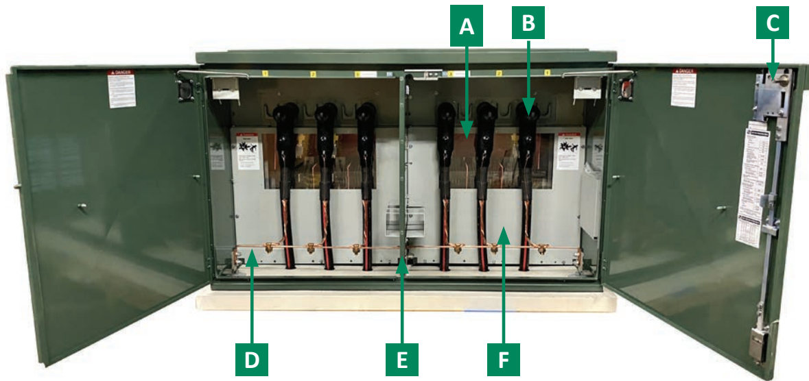
FIGURE 3. Switch compartment features.
