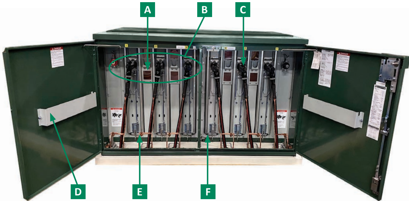
FIGURE 5. Fuse compartment features.
