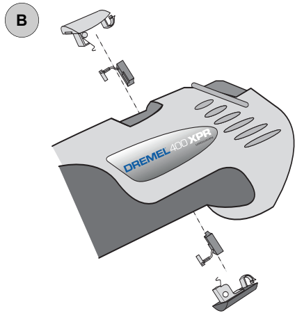
Removing/Inspecting Brushes
