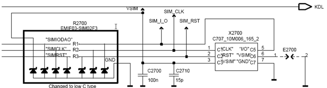
Figure 108 SIM filtering
