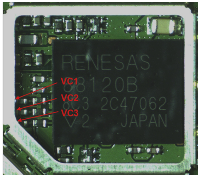
Figure 62 RX measurements point of the control voltages to FEM N7700
