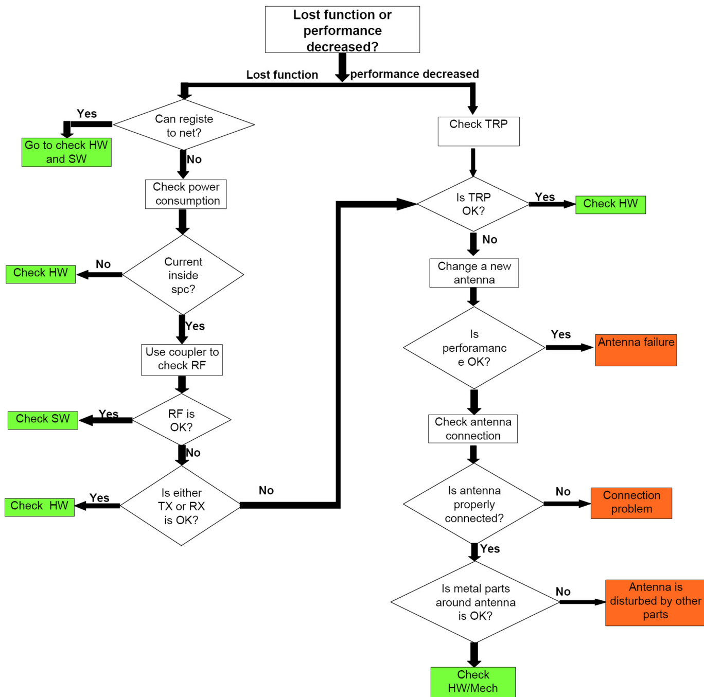
Figure 89 Antenna troubleshooting
