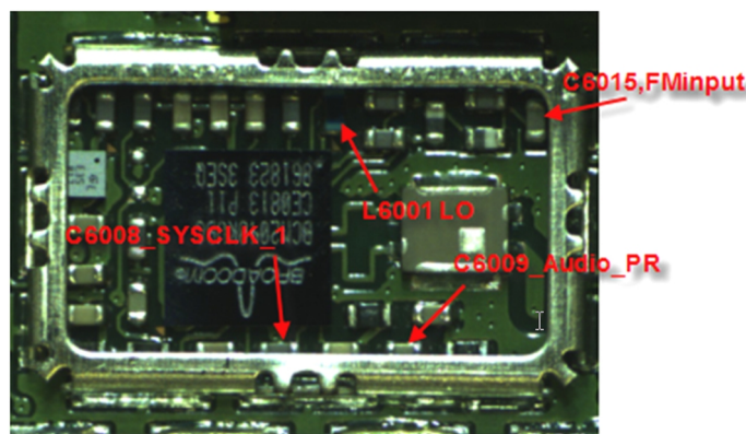
Figure 84 Bluetooth and FM radio test points
