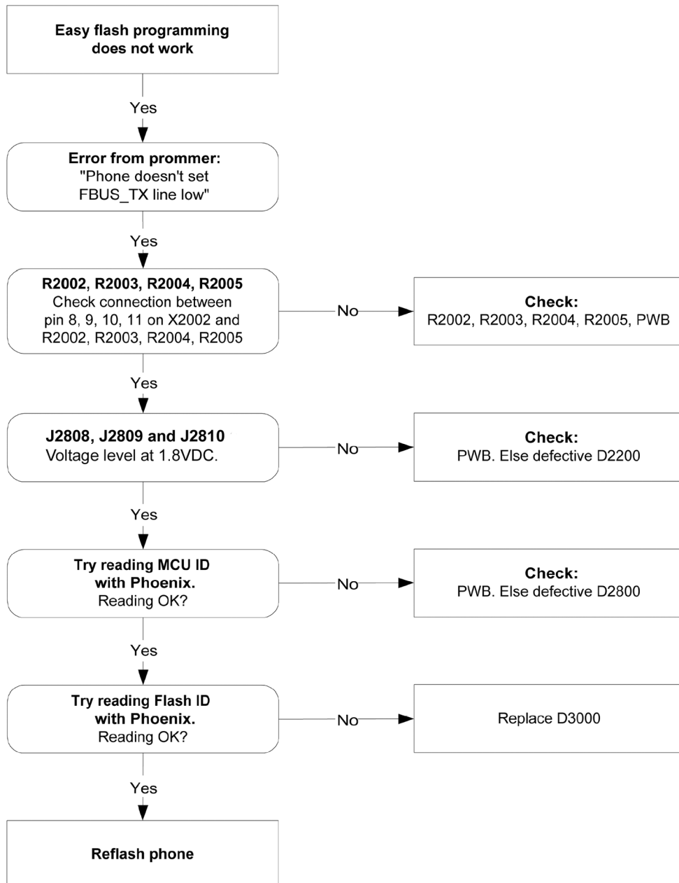
Figure 12 Easy flash programming fault
