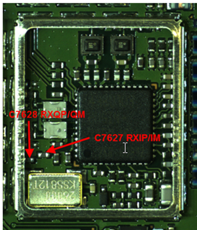
Figure 64 RX I/Q signals
