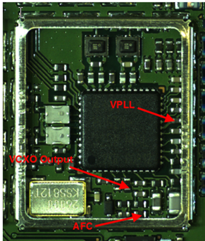
Figure 81 Measurement point for VCXO
