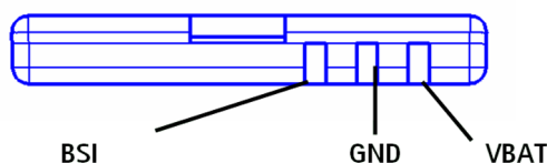
Figure 114 BL-4B battery pack contacts
