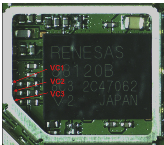
Figure 39 RX measurements point of the control voltages to FEM N7700
