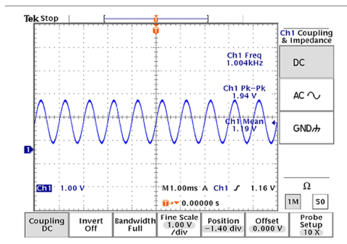
Figure 85 XAUDIO output signal
