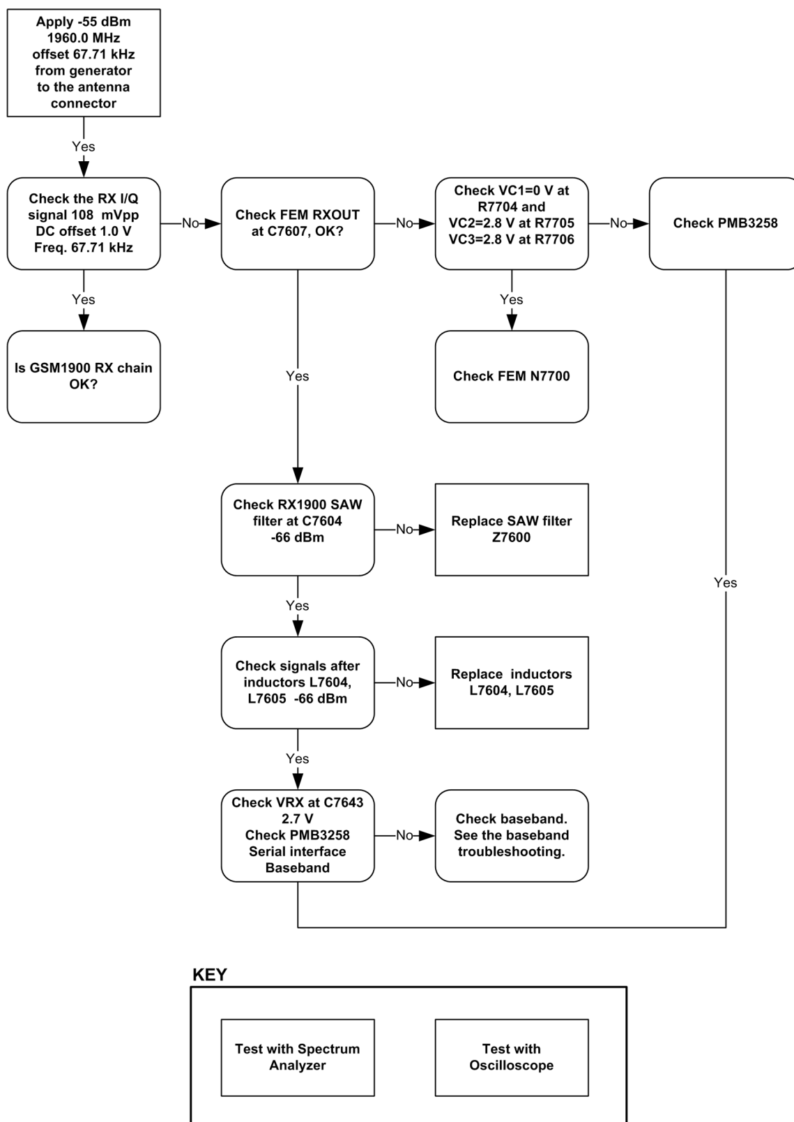
Figure 60 GSM1900 receiver troubleshooting
