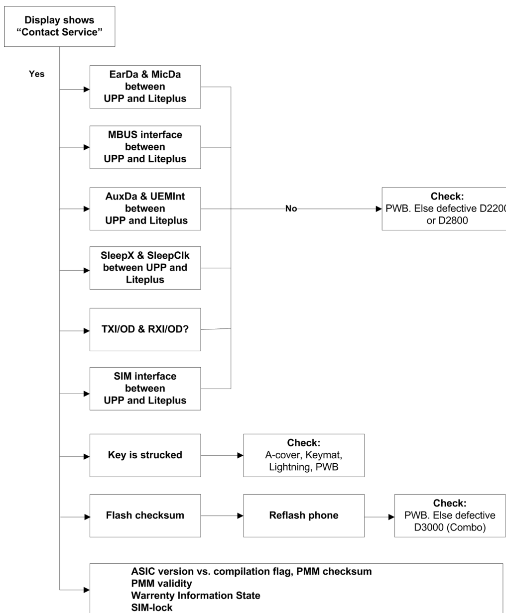
Figure 13 Troubleshooting when the "Contact Service" message is seen
