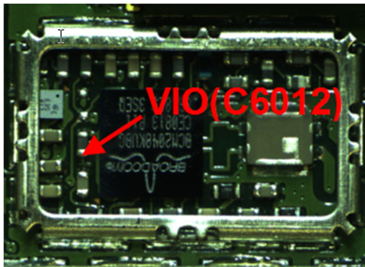
Figure 32 Supply point at BT & FM IC (N6000)
