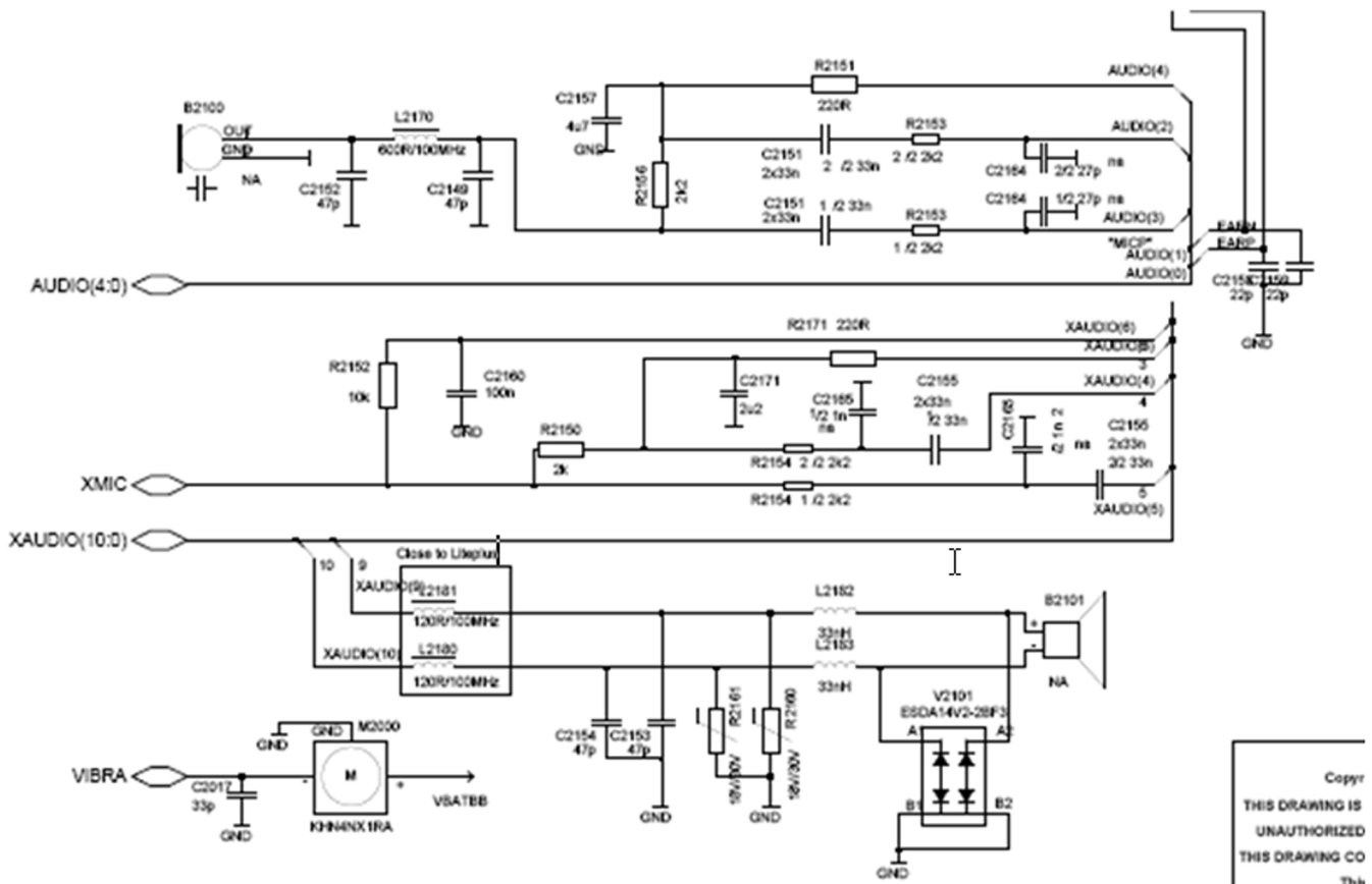
Figure 109 Audio block diagram
