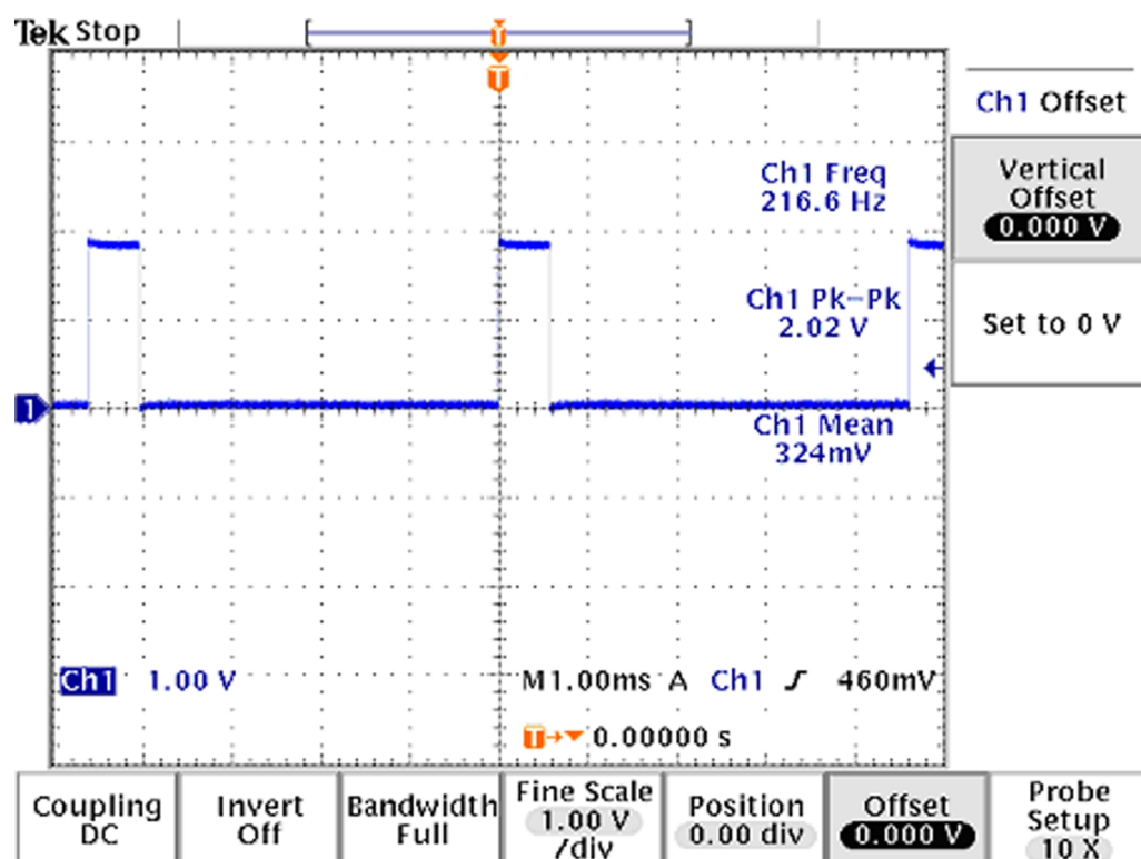
Figure 46 TXP signal
