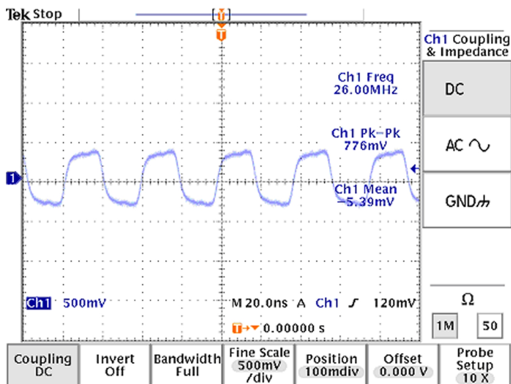
Figure 79 VCXO 26 MHz waveform
