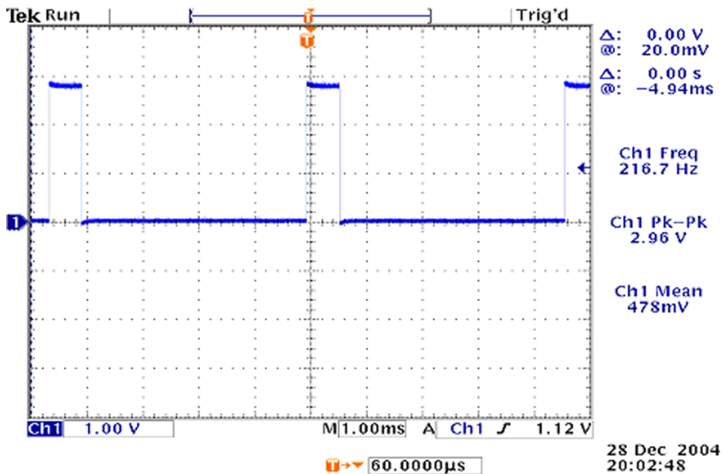
Figure 68 VC1, VC3 signal
