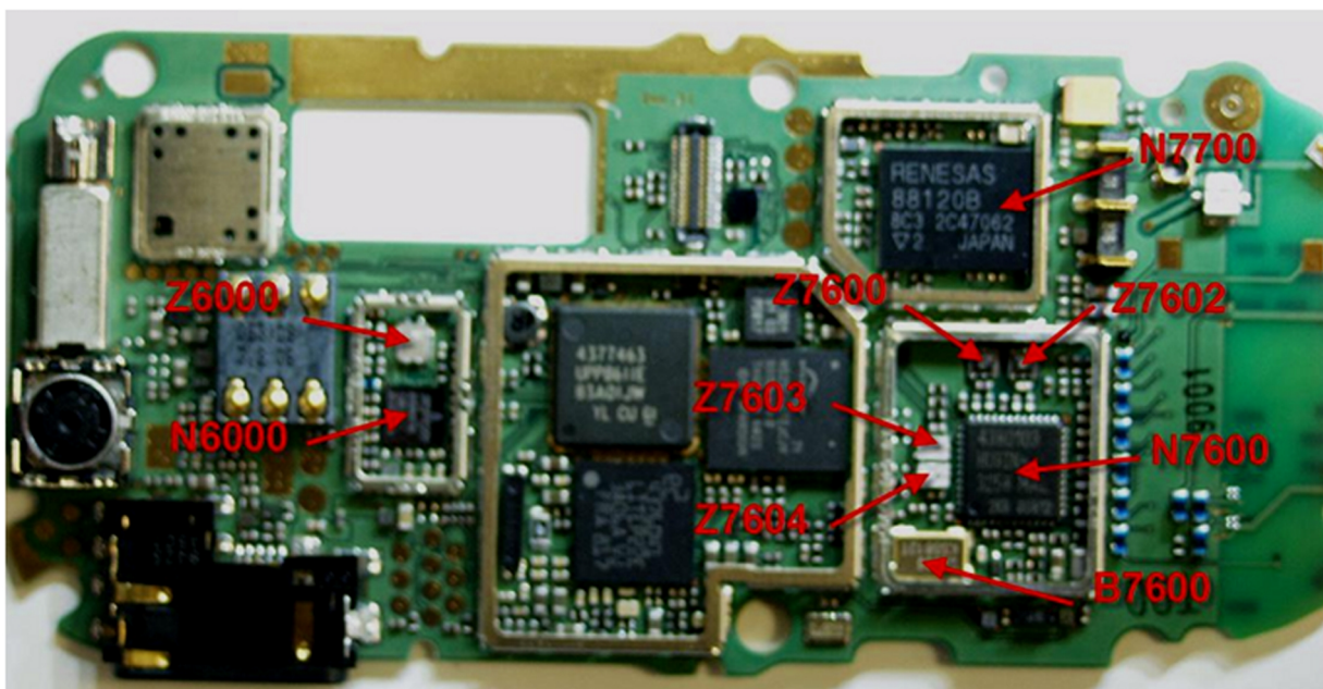
Figure 29 RF key components on PWB
