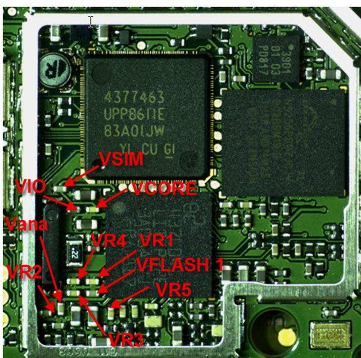
Figure 30 Supply points at UEM (D2200)
