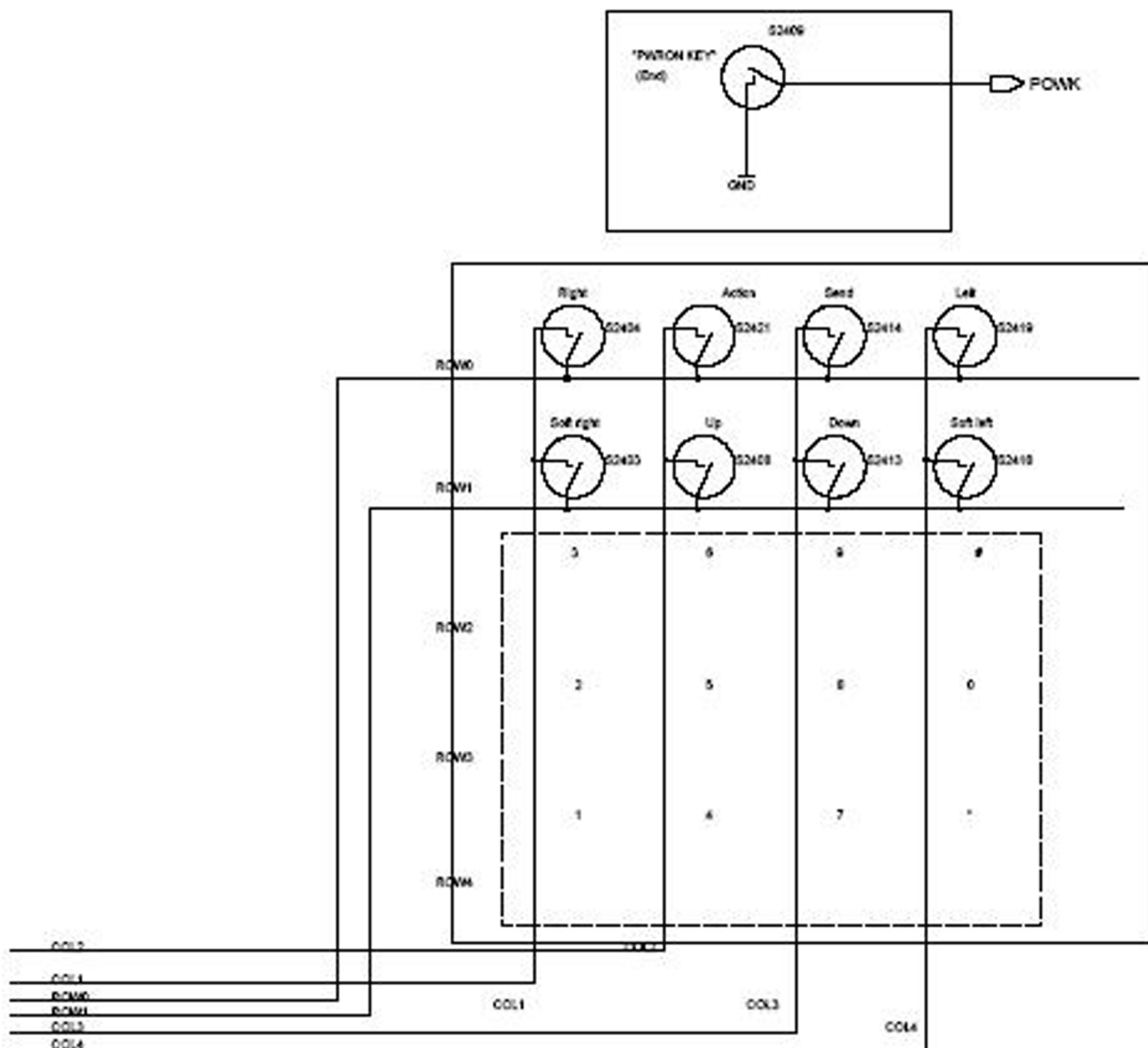
Figure 112 Keypad schematics
