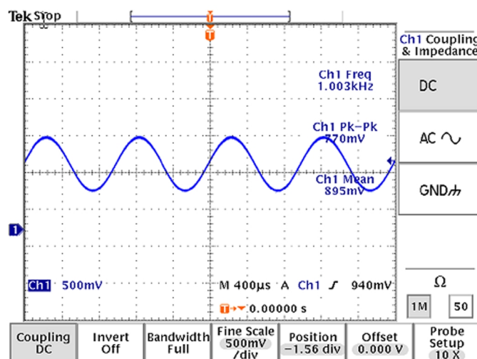
Figure 86 FM module output signal
