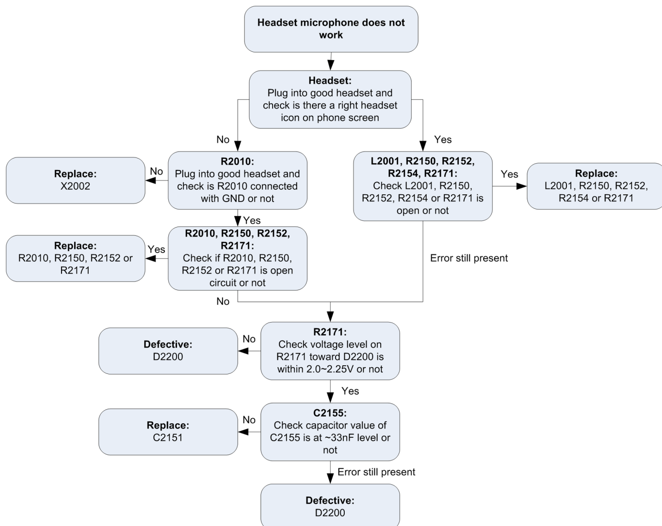
Figure 28 Headset microphone fault flow chart
