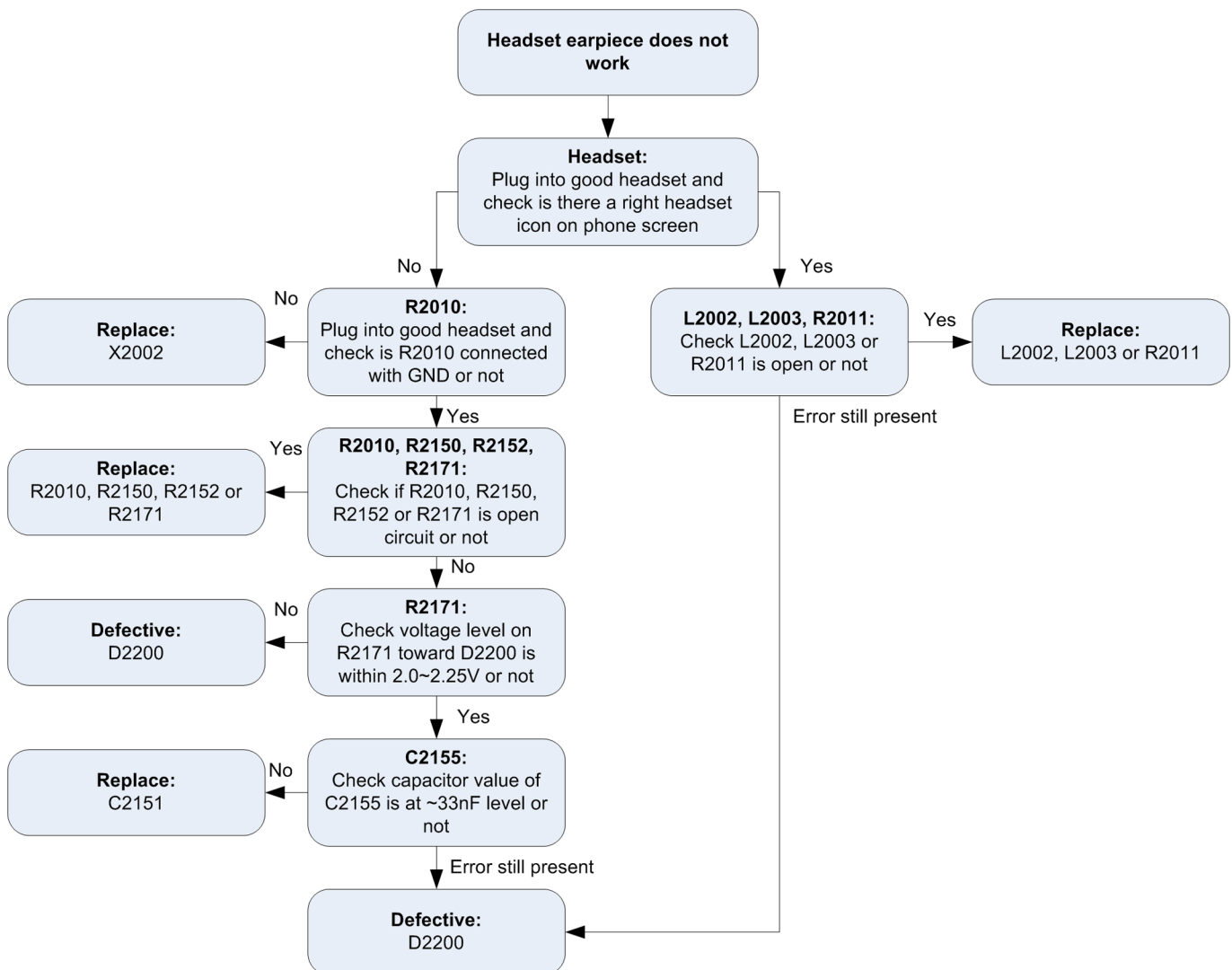
Figure 27 Headset earpiece fault flow chart
