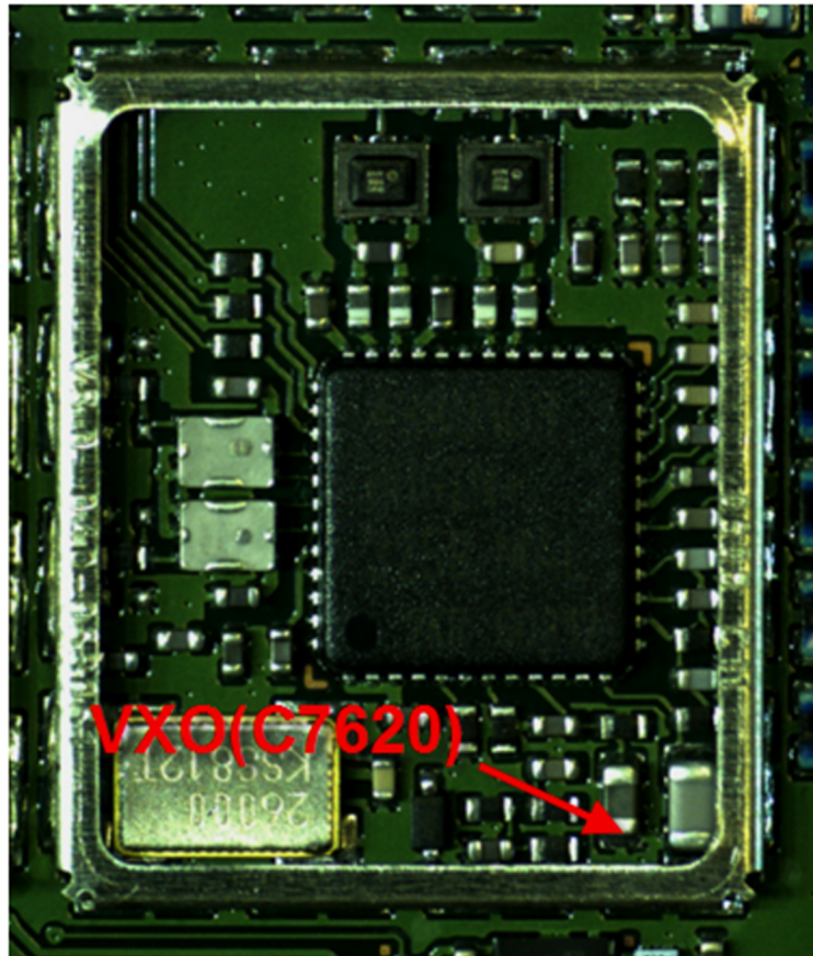
Figure 31 Supply point at RF IC (N7600)
