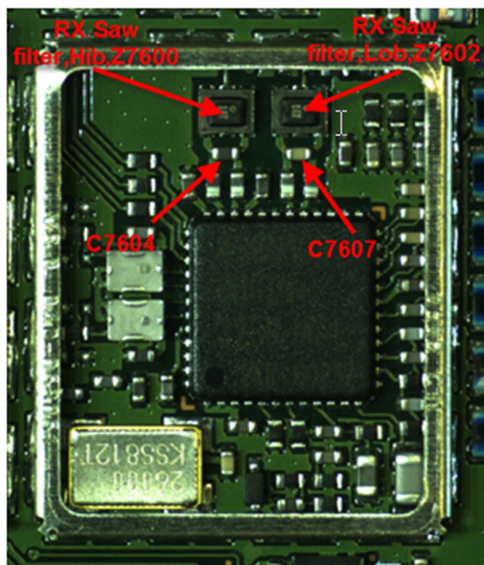
Figure 63 Measurement points at the RX SAW Filters – Z7600/Z7602
