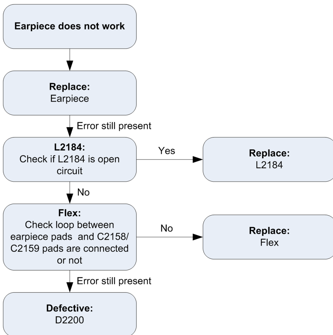
Figure 24 Earpiece fault flow chart
