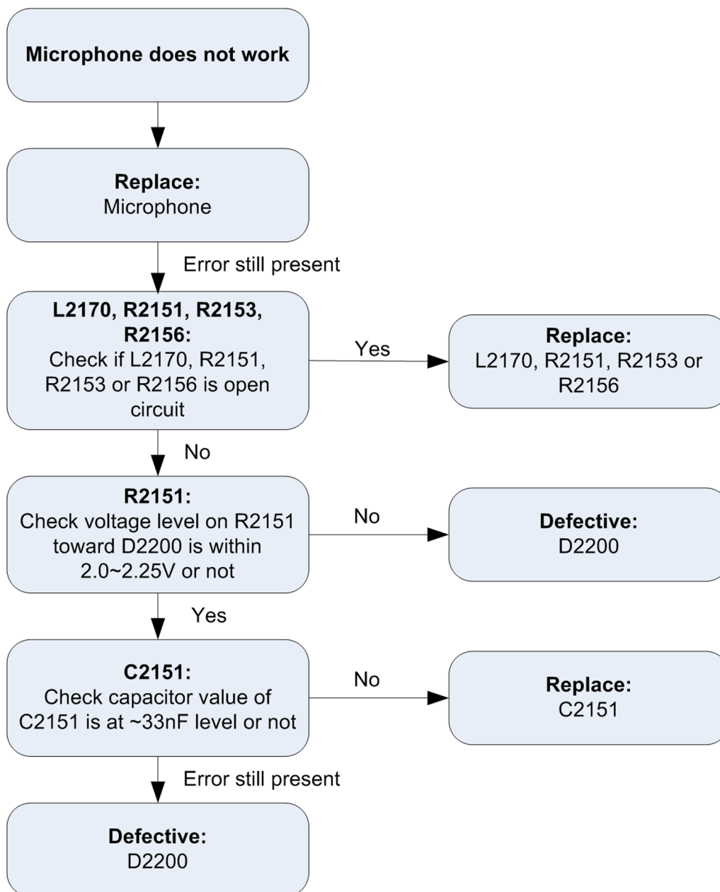
Figure 26 Microphone fault flow chart
