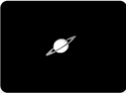
Fig. 44: Saturn with its ring system.
