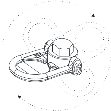
Single Point Swivel Anchor for Concrete Structure (DXFP843101)
