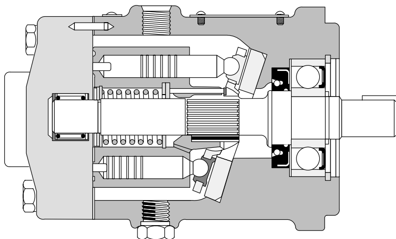
Assembly View
