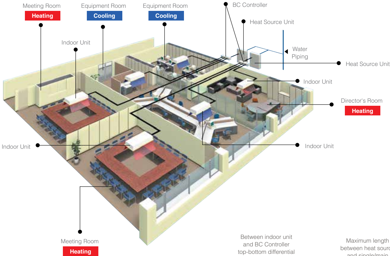
Installation image WR2 Series
