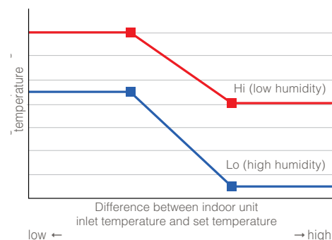
Image of evaporating temperature control during high sensible heat operation in full cooling mode
