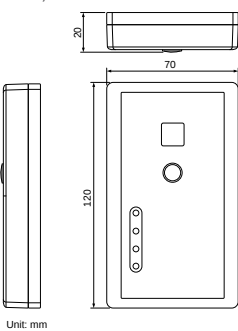
SEPARATE RECEIVER FOR WIRELESS REMOTE CONTROLLER (CZ-RWRC3)
