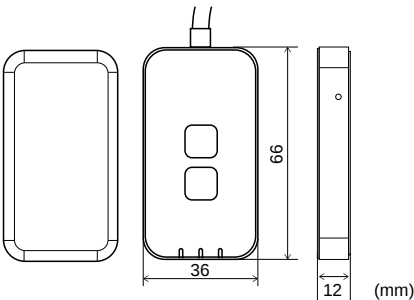
WLAN ADAPTOR (CZ-TACG1)
