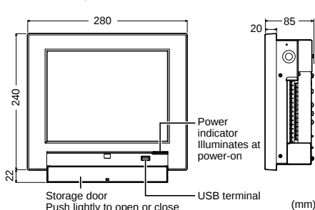
INTELLIGENT CONTROLLER (CZ-256ESMC3)
