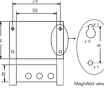
SERI-PARA I/O UNIT FOR OUTDOOR UNIT (CZ-CAPDC2)
