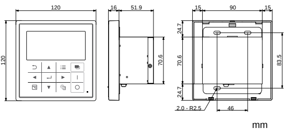
System Controller
