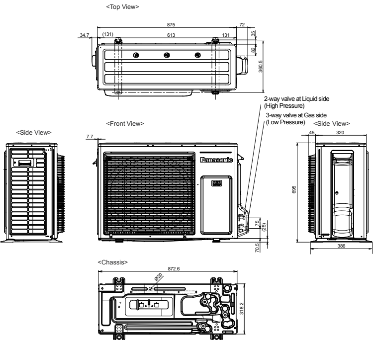
Dimensions (4.8kW – 5.7kW) CU-Z50UBRA / CU-Z60UBRA
