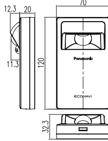
ECONAVI SENSOR (CZ-CENSC1)
