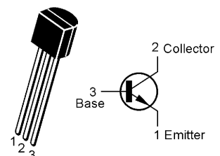
2SC1815 Q101,102,111,112,113,115,118, 201,206,207,301,302
