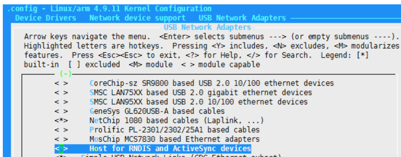
Figure 3: Configure ECM and RNDIS in Kernel
