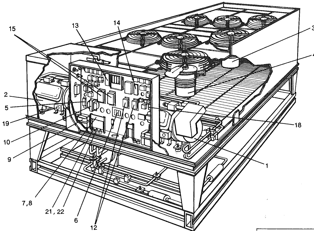
FIG. 1 - AIR COOLED WATER CHILLER
