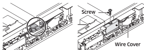
Fridge Door
