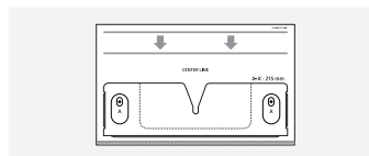
Ⓐ Wall-mounting Guide
