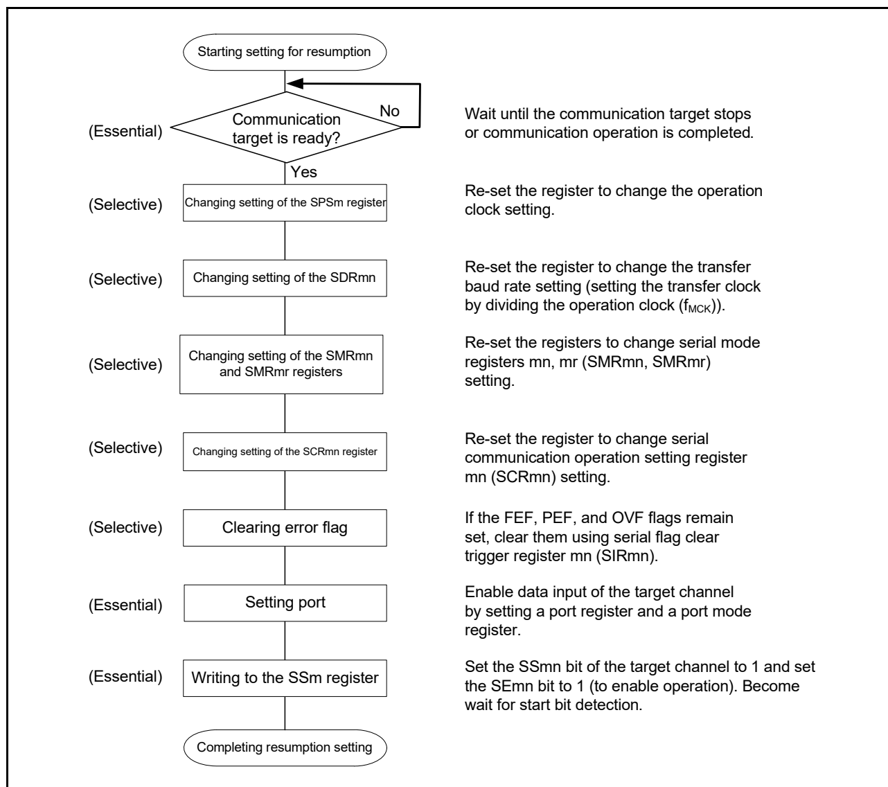
Figure 15 - 89 Procedure for Resuming UART Reception
