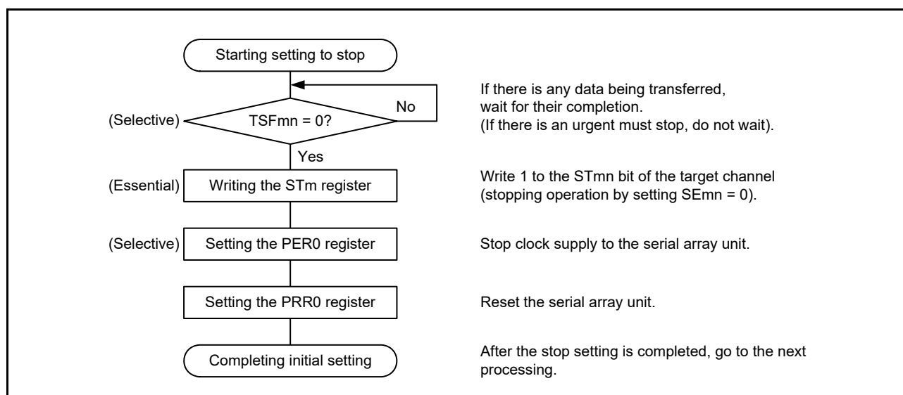
Figure 15 - 88 Procedure for Stopping UART Reception
