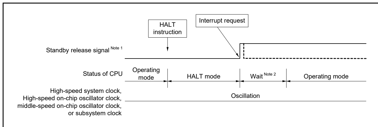
Figure 23 - 5 HALT Mode Release by Interrupt Request Generation
