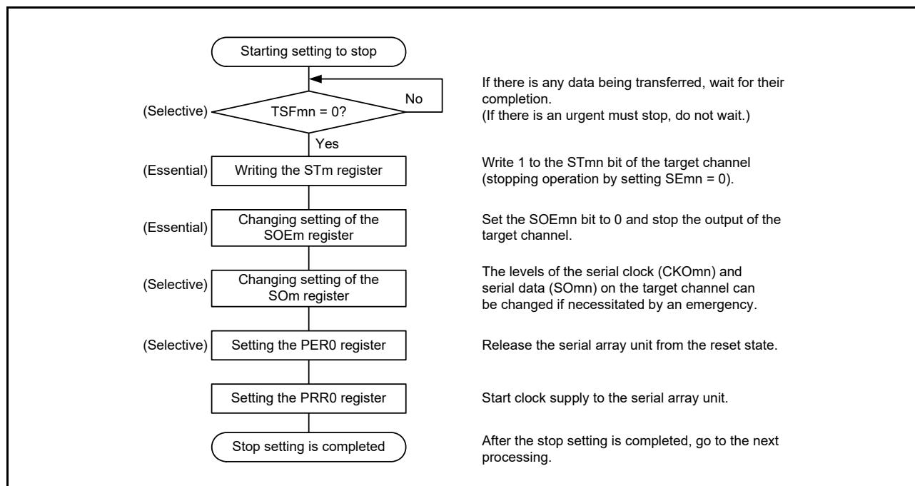
Figure 15 - 45 Procedure for Stopping Master Transmission/Reception
