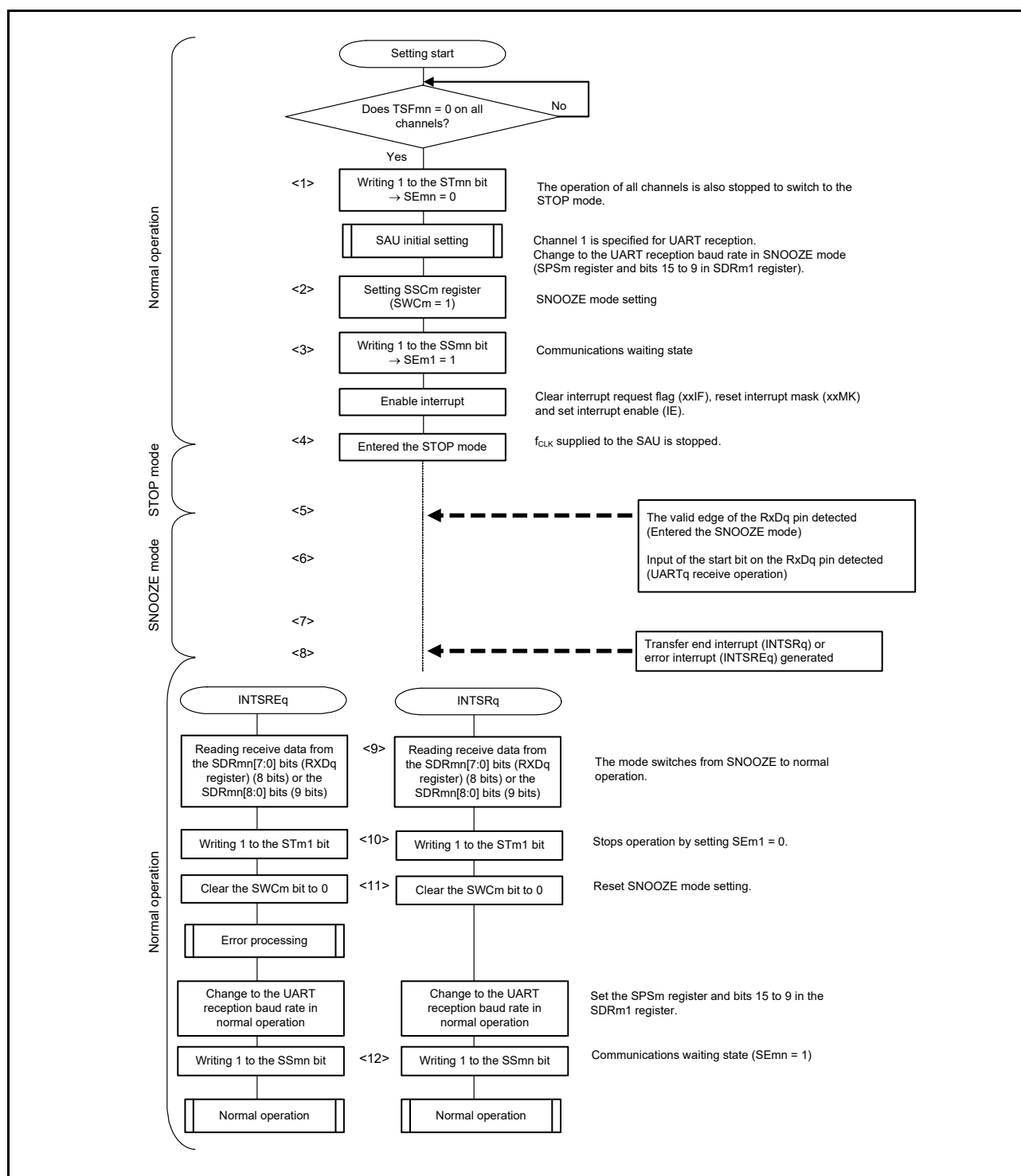
Figure 15 - 94 Flowchart of SNOOZE Mode Operation (EOCm1 = 0, SSECm = 0/1 or EOCm1 = 1, SSECm = 0)
