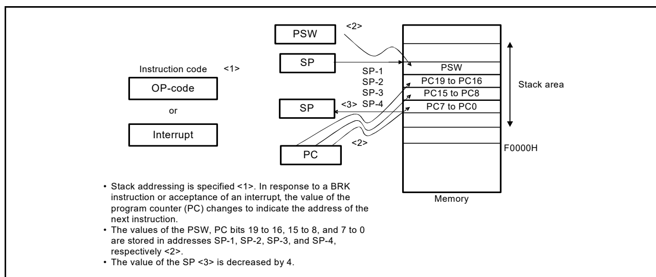
Figure 3 - 42 Example of Interrupt, BRK
