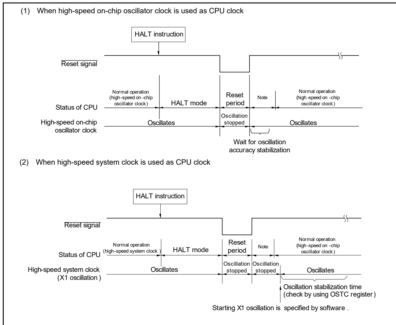
Figure 23 - 6 HALT Mode Release by Reset (1/2)
