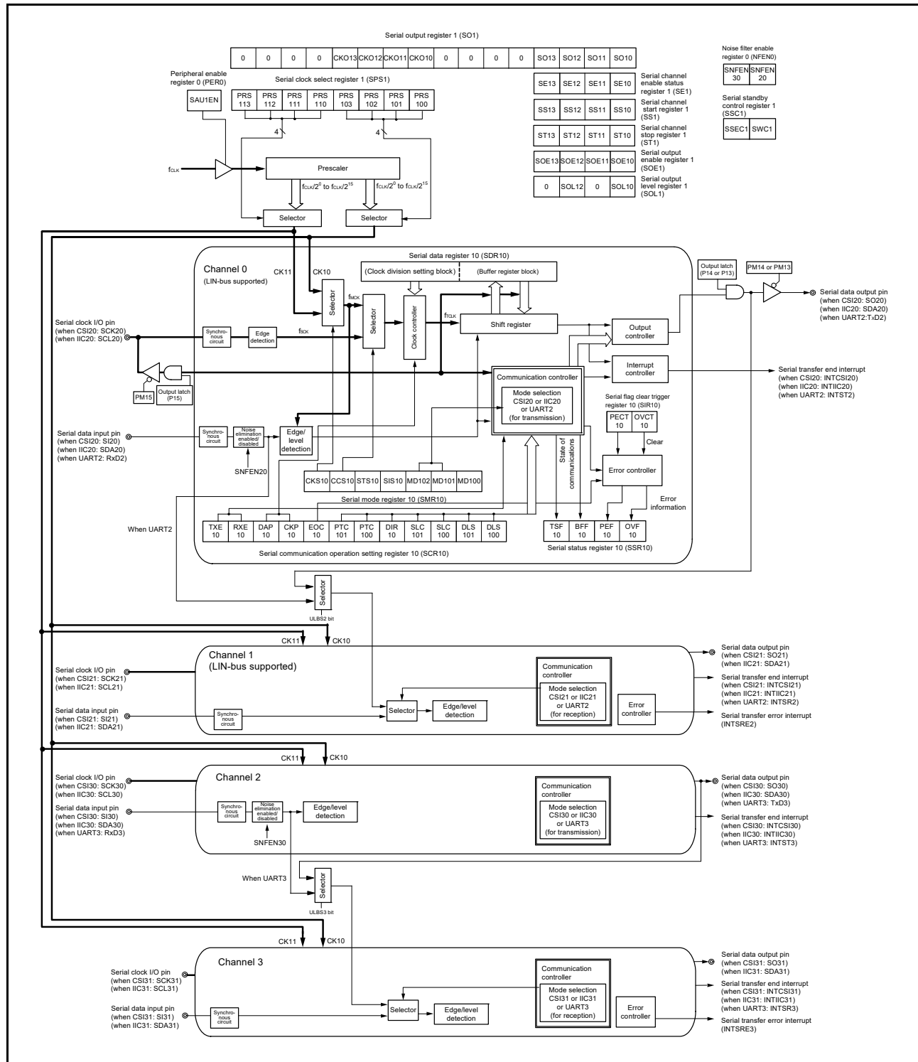
Figure 15 - 2 Block Diagram of Serial Array Unit 1
