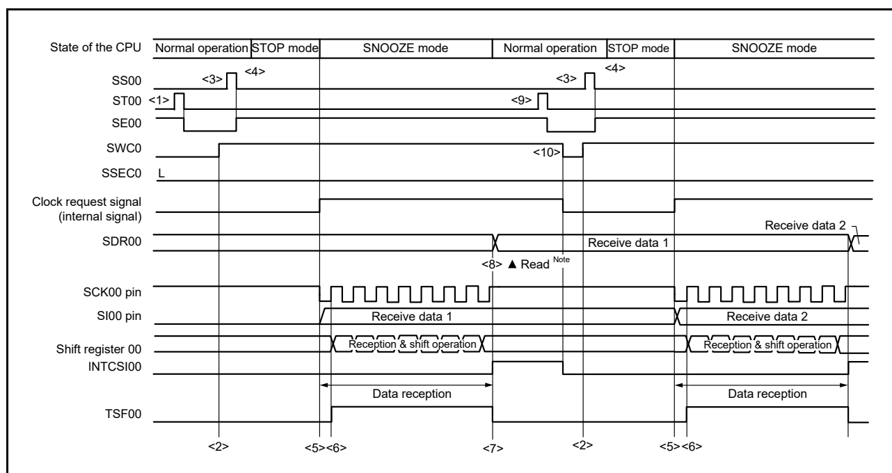
Figure 15 - 75 Timing Chart of SNOOZE Mode Operation (continuous startup) (Type 1: DAPmn = 0, CKPmn = 0)
