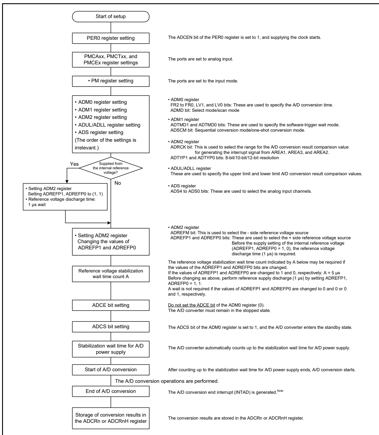
Figure 12 - 35 Setting up Software Trigger Wait Mode
