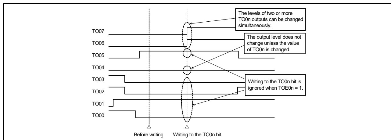
Figure 7 - 41 TO0n Pin States by Collective Manipulation of TO0n Bits
