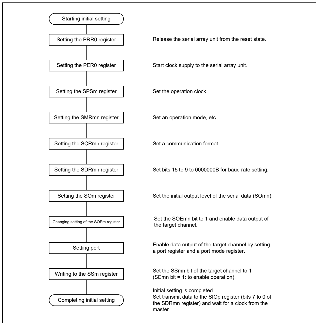
Figure 15 - 66 Initial Setting Procedure for Slave Transmission/Reception
