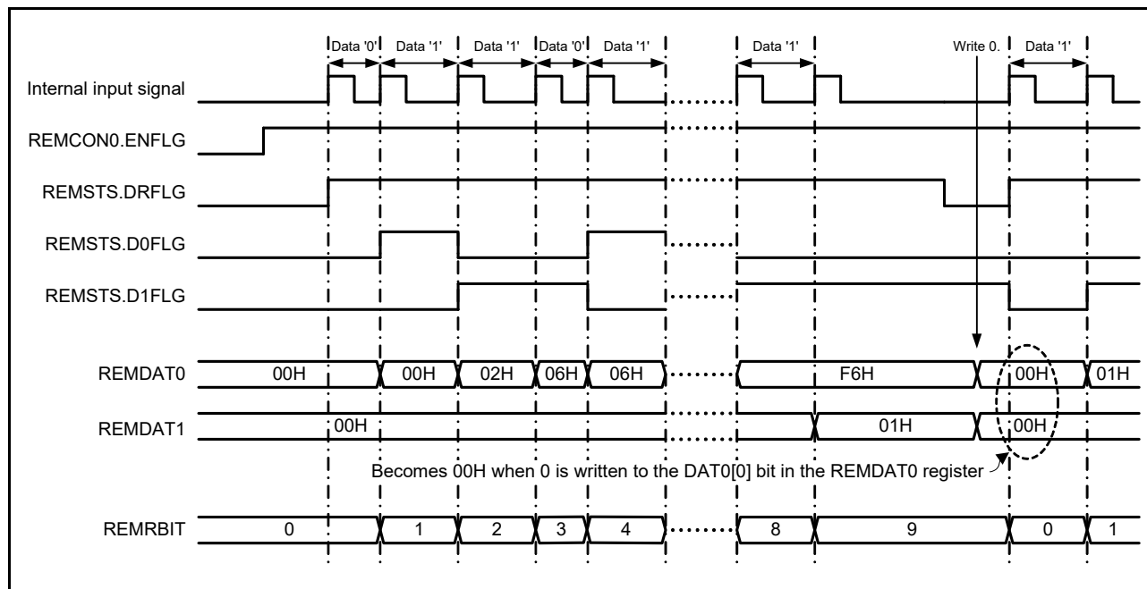
Figure 18 - 35 REMDATj/REMRBIT Register Operation (00H is Written to REMDAT0 Register)
