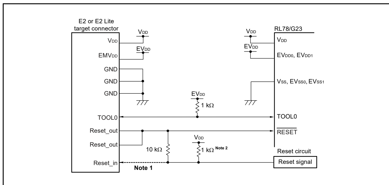
Figure 34 - 1 Example of Connection between the E2 or E2 Lite On-Chip Debugging Emulator and RL78/G23
