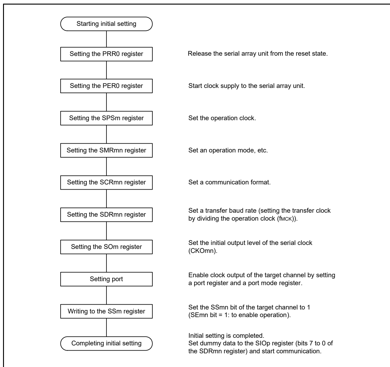
Figure 15 - 36 Initial Setting Procedure for Master Reception
