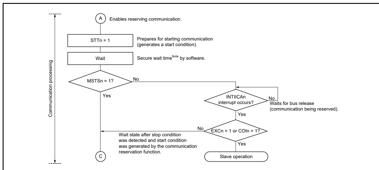
Figure 16 - 29 Master Operation in Multi-Master System (2/3)
