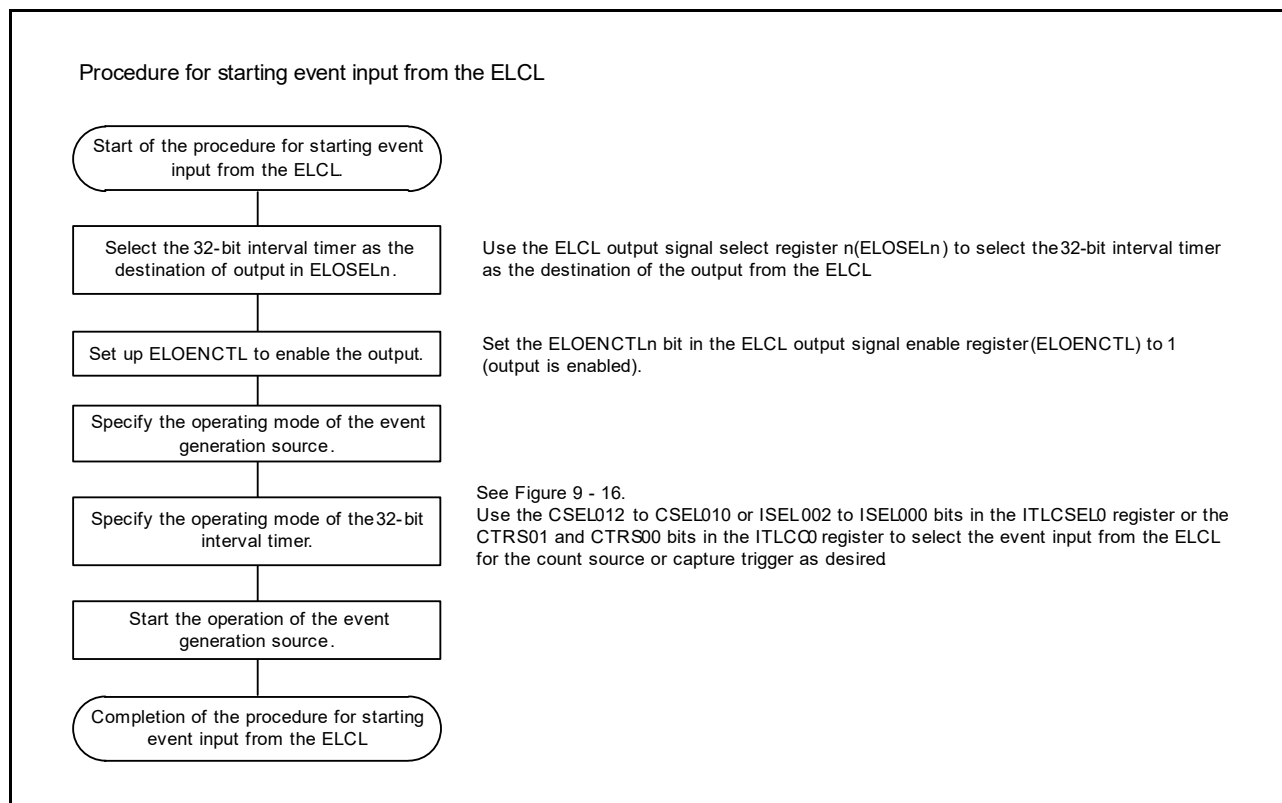
Figure 9 - 20 Procedure for Starting Event Input from the ELCL
