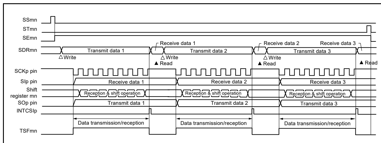
Figure 15 - 69 Timing Chart of Slave Transmission/Reception (in Single-Transmission/Reception Mode) (Type 1: DAPmn = 0, CKPmn = 0)
