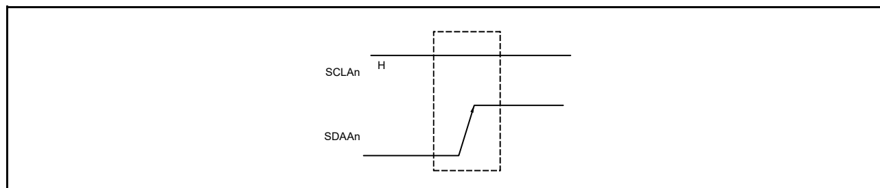
Figure 16 - 19 Stop Condition
