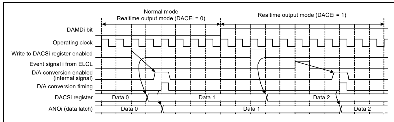
Figure 13 - 6 Timing for Outputting D/A Conversion Value
