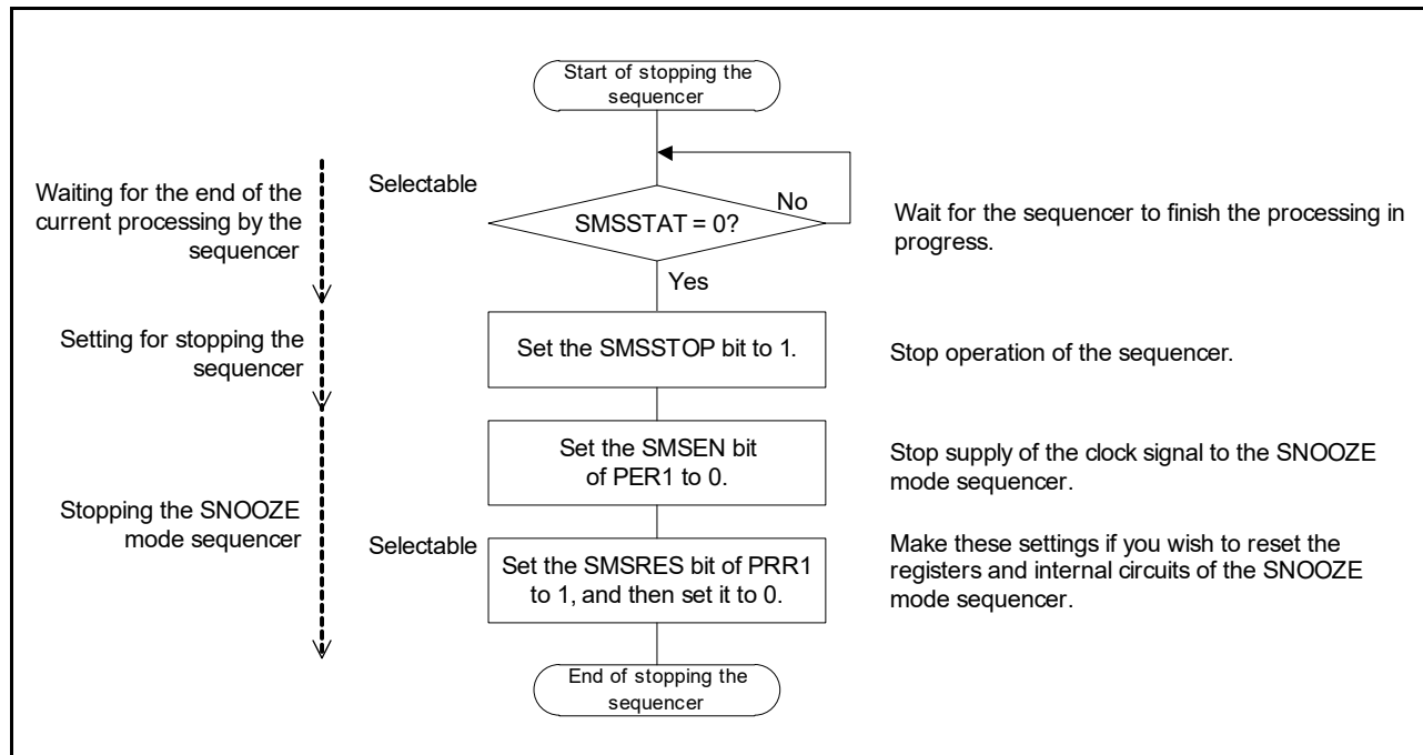
Figure 29 - 12 Flow of Stopping the SNOOZE Mode Sequencer
