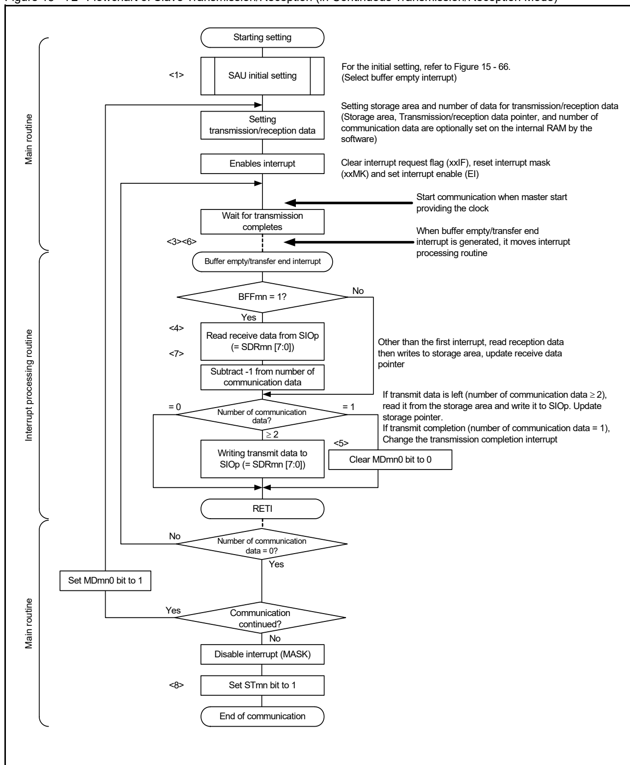
Figure 15 - 72 Flowchart of Slave Transmission/Reception (in Continuous Transmission/Reception Mode)
