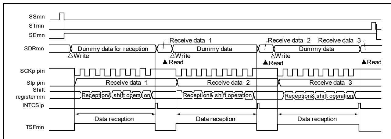
Figure 15 - 39 Timing Chart of Master Reception (in Single-Reception Mode) (Type 1: DAPmn = 0, CKPmn = 0)
