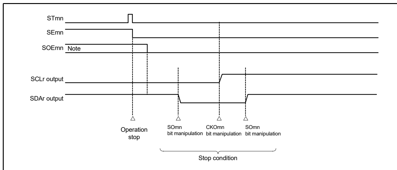
Figure 15 - 116 Timing Chart of Stop Condition Generation
