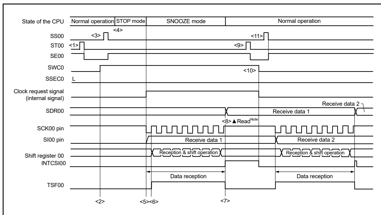
Figure 15 - 73 Timing Chart of SNOOZE Mode Operation (once startup) (Type 1: DAPmn = 0, CKPmn = 0)
