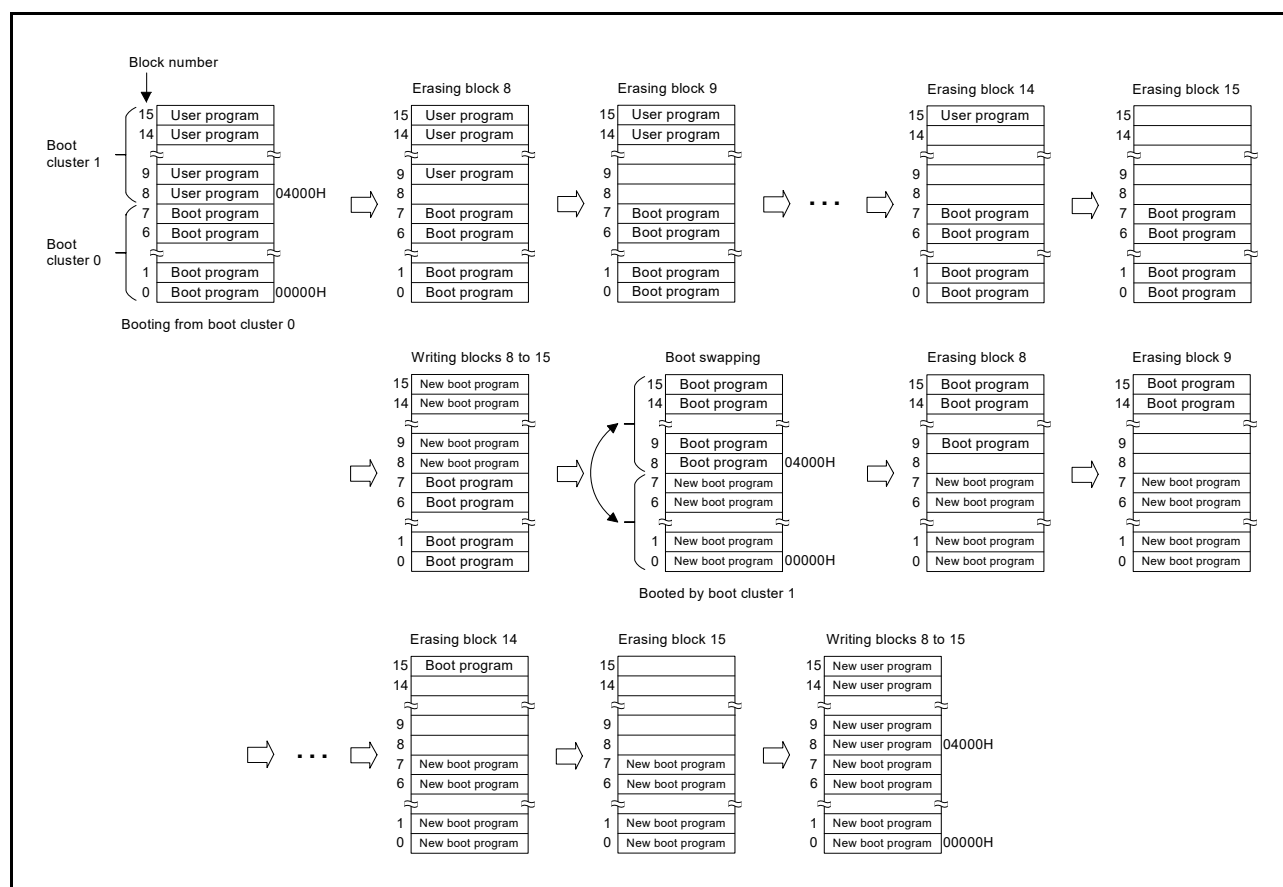
Figure 33 - 28 Example of Executing Boot Swapping
