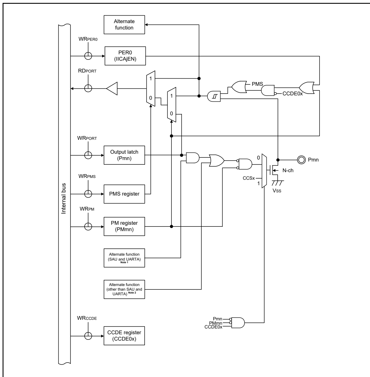
Figure 2 - 32 Pin Block Diagram for Pin Type 12-38-2
