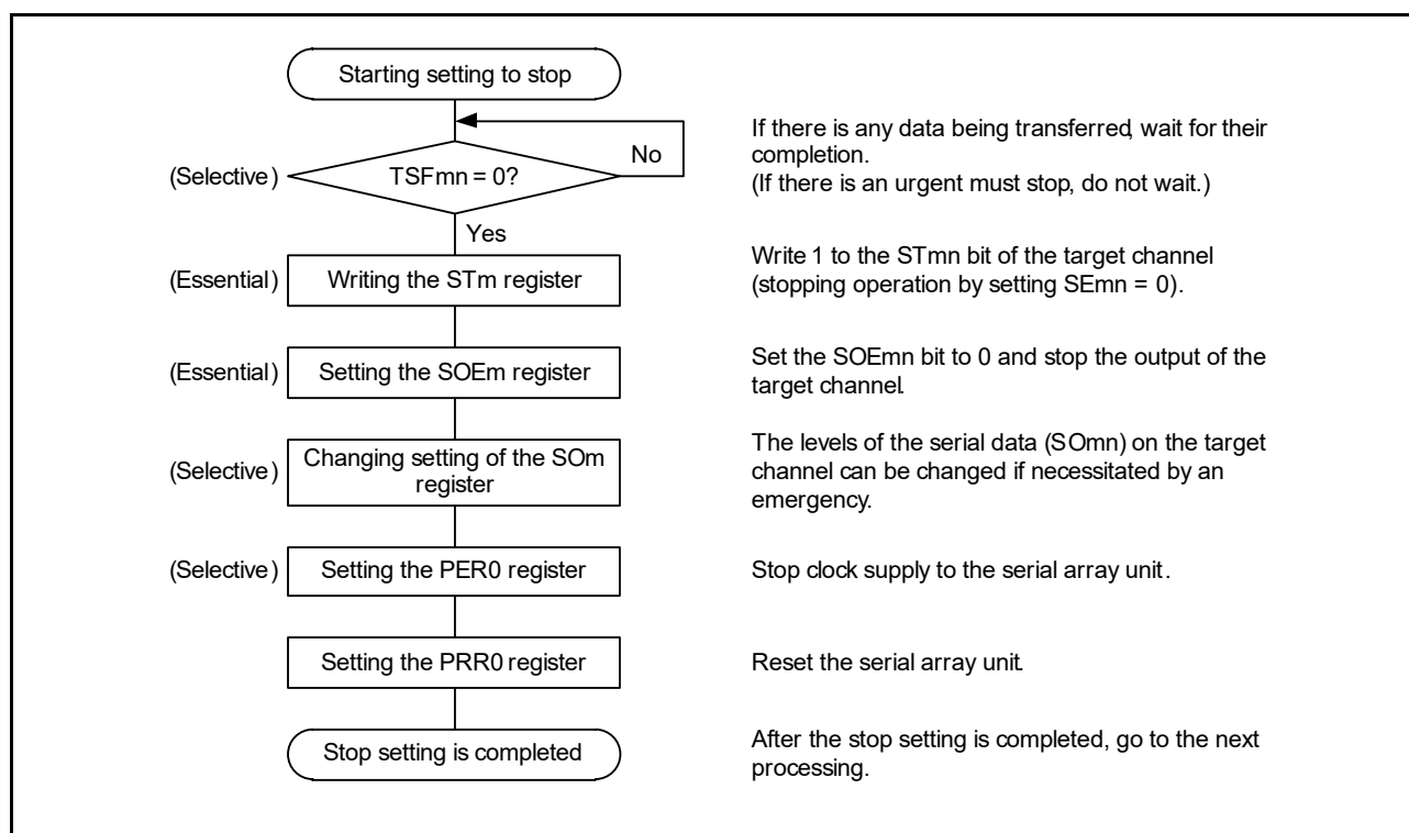
Figure 15 - 80 Procedure for Stopping UART Transmission
