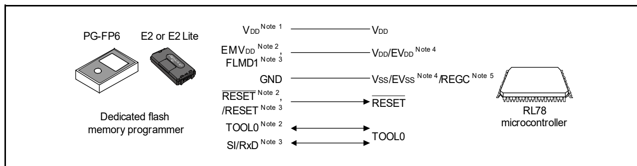
Figure 33 - 2 Communication with Dedicated Flash Memory Programmer
