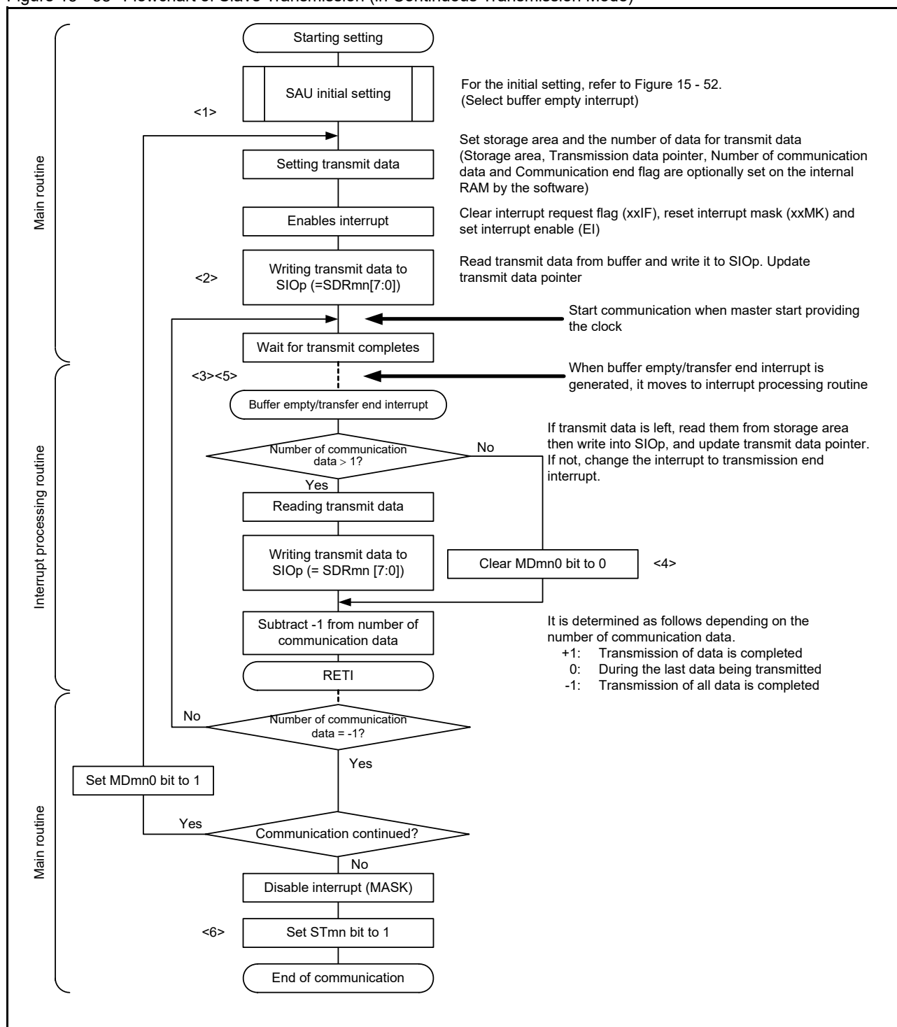
Figure 15 - 58 Flowchart of Slave Transmission (in Continuous Transmission Mode)
