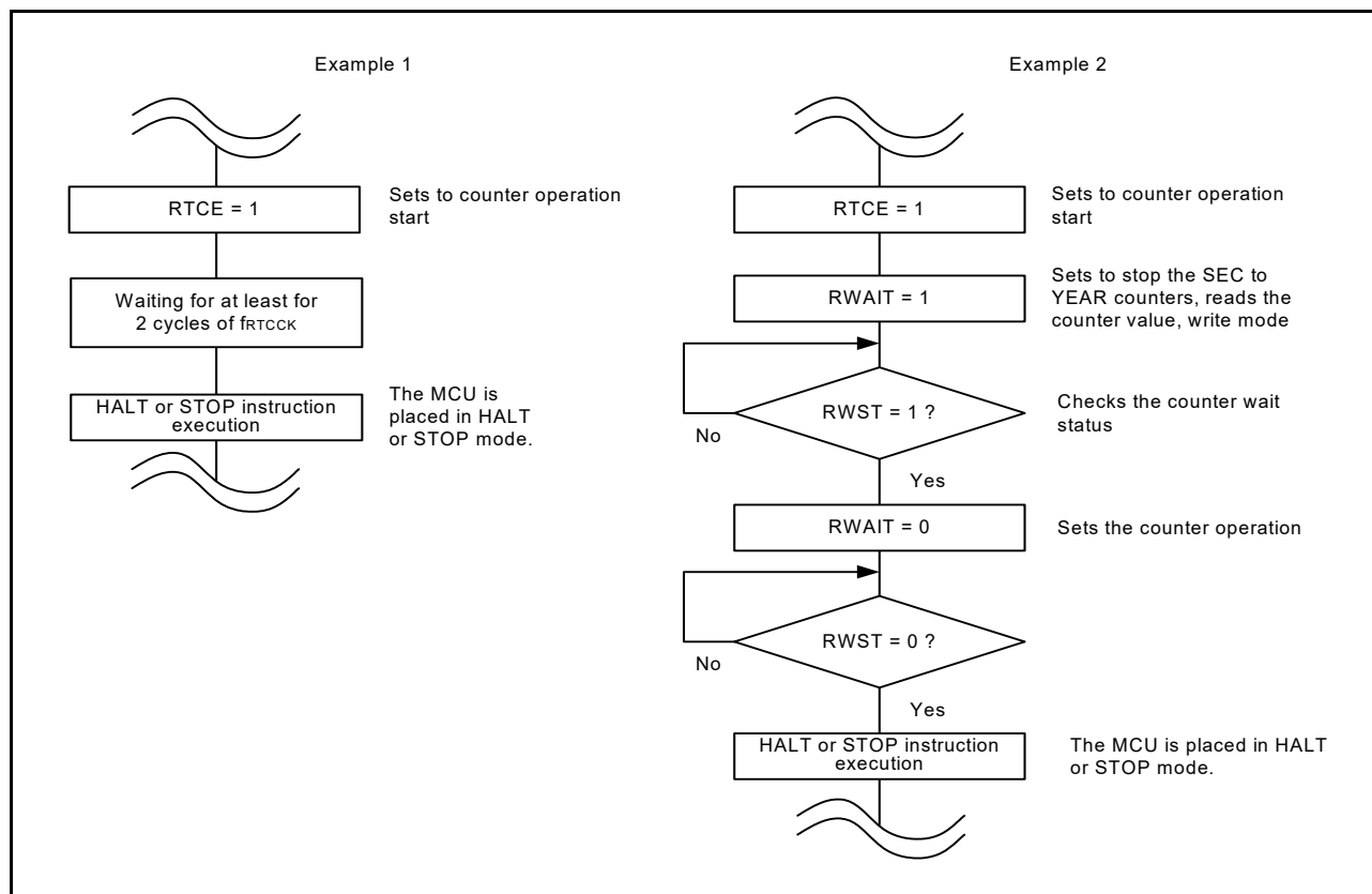
Figure 8 - 20 Procedure for Shifting to HALT or STOP Mode after Setting RTCE Bit to 1
