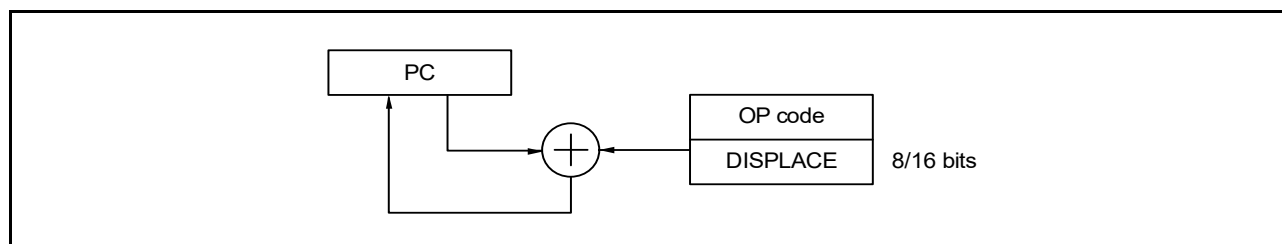
Figure 3 - 16 Outline of Relative Addressing
