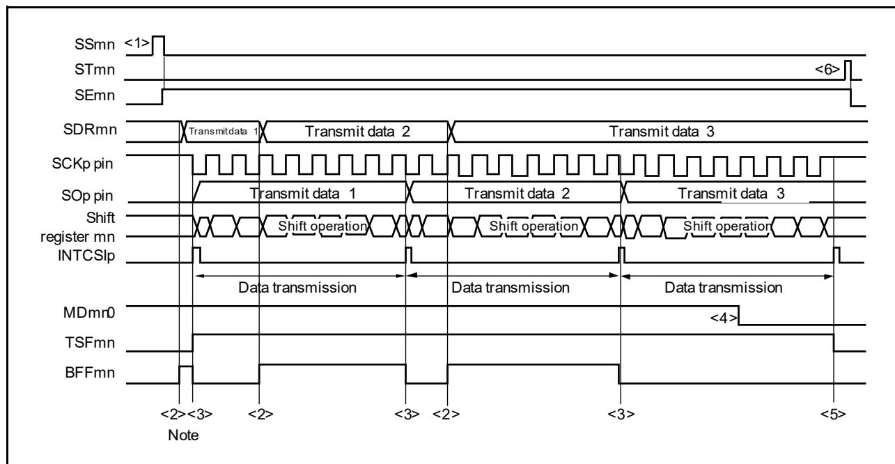
Figure 15 - 33 Timing Chart of Master Transmission (in Continuous Transmission Mode) (Type 1: DAPmn = 0, CKPmn = 0)
