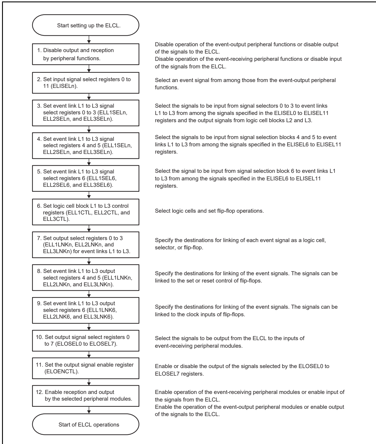
Figure 20 - 31 Procedure of Setting the ELCL
