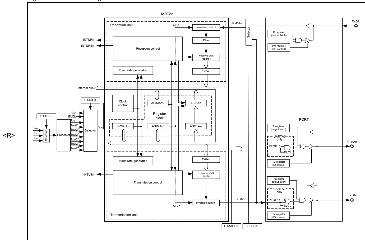
Figure 17 - 1 Block Diagram of UARTAn
