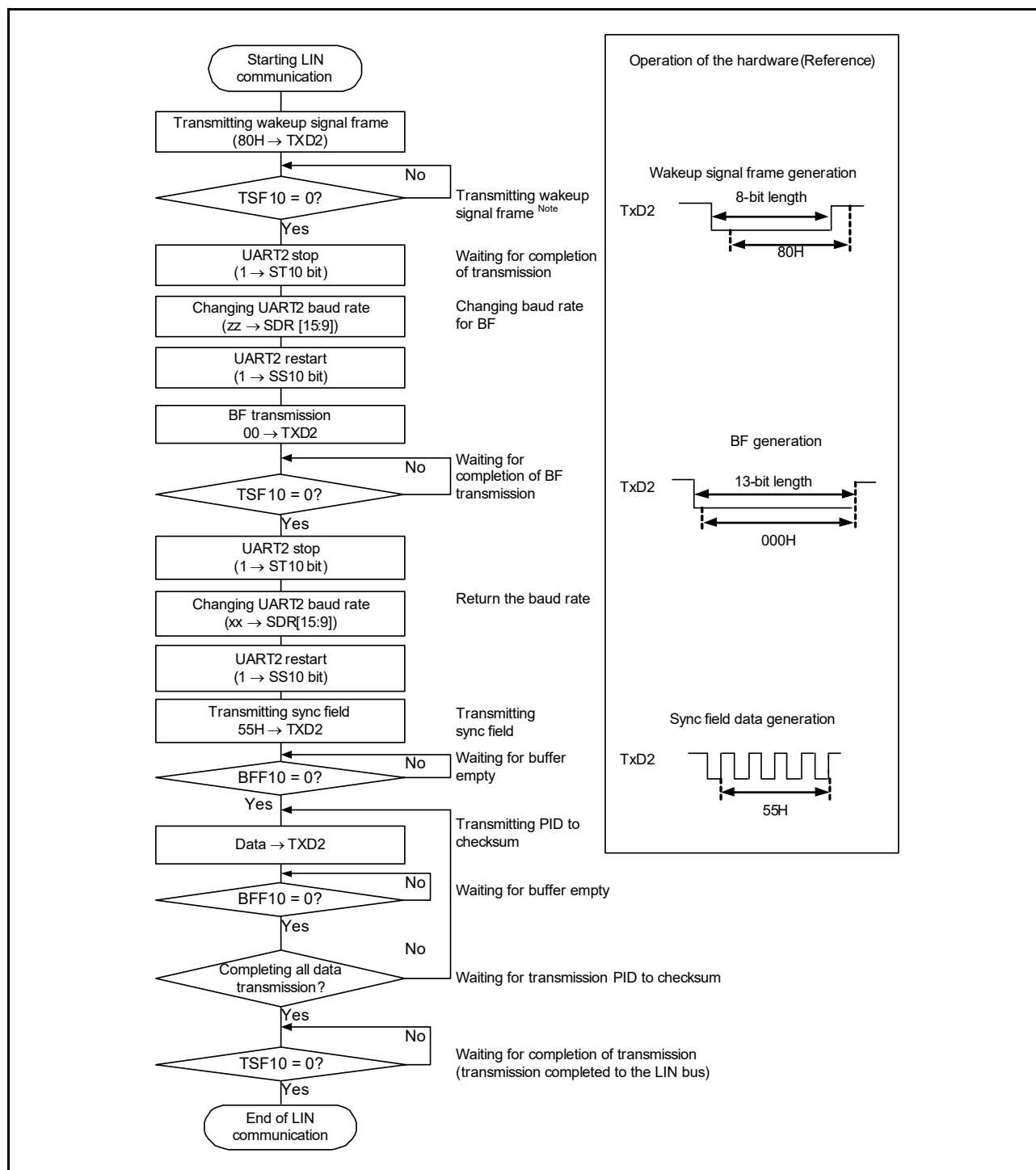
Figure 15 - 101 Flowchart for LIN Transmission
