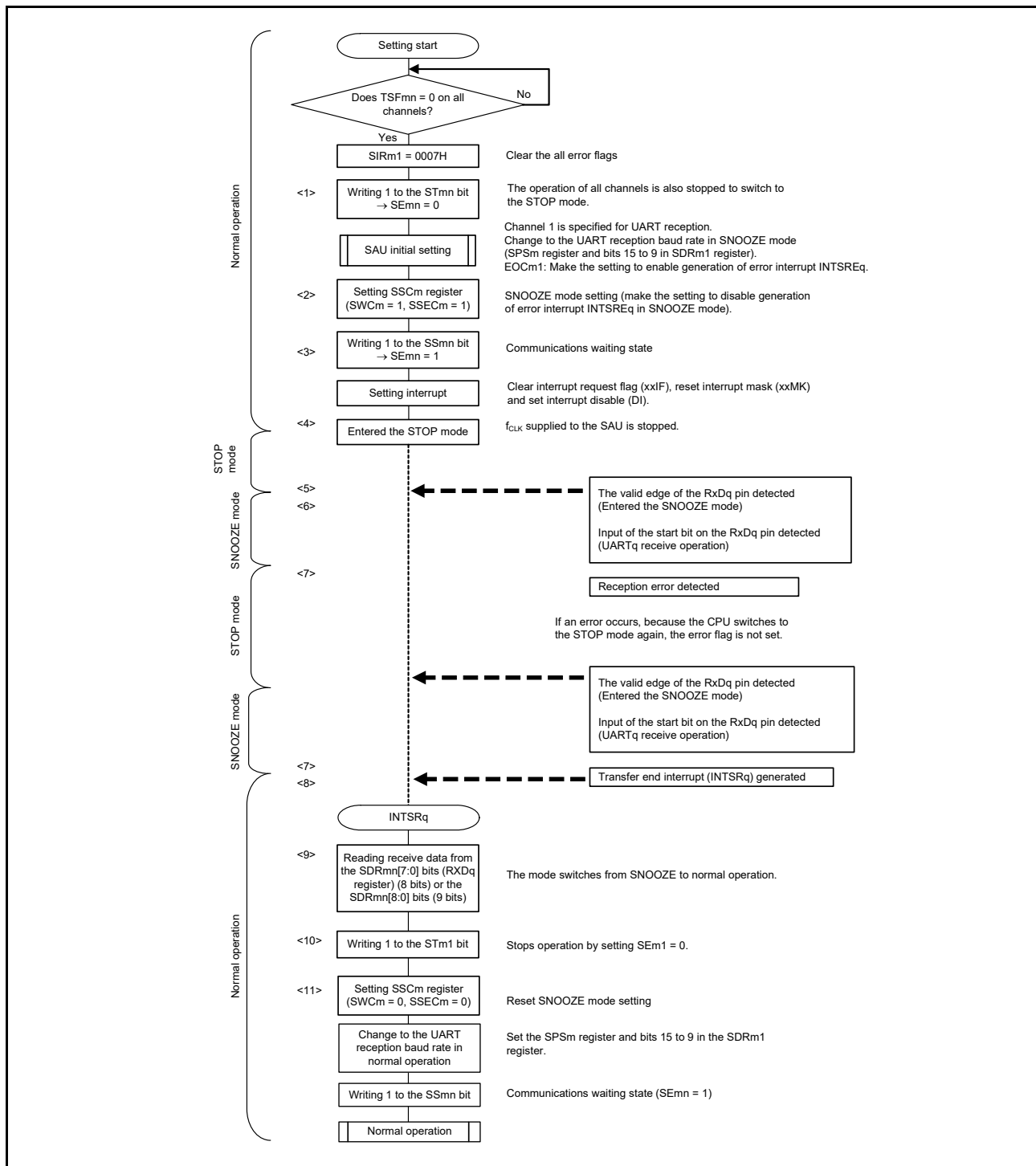
Figure 15 - 96 Flowchart of SNOOZE Mode Operation (EOCm1 = 1, SSECm = 1)
