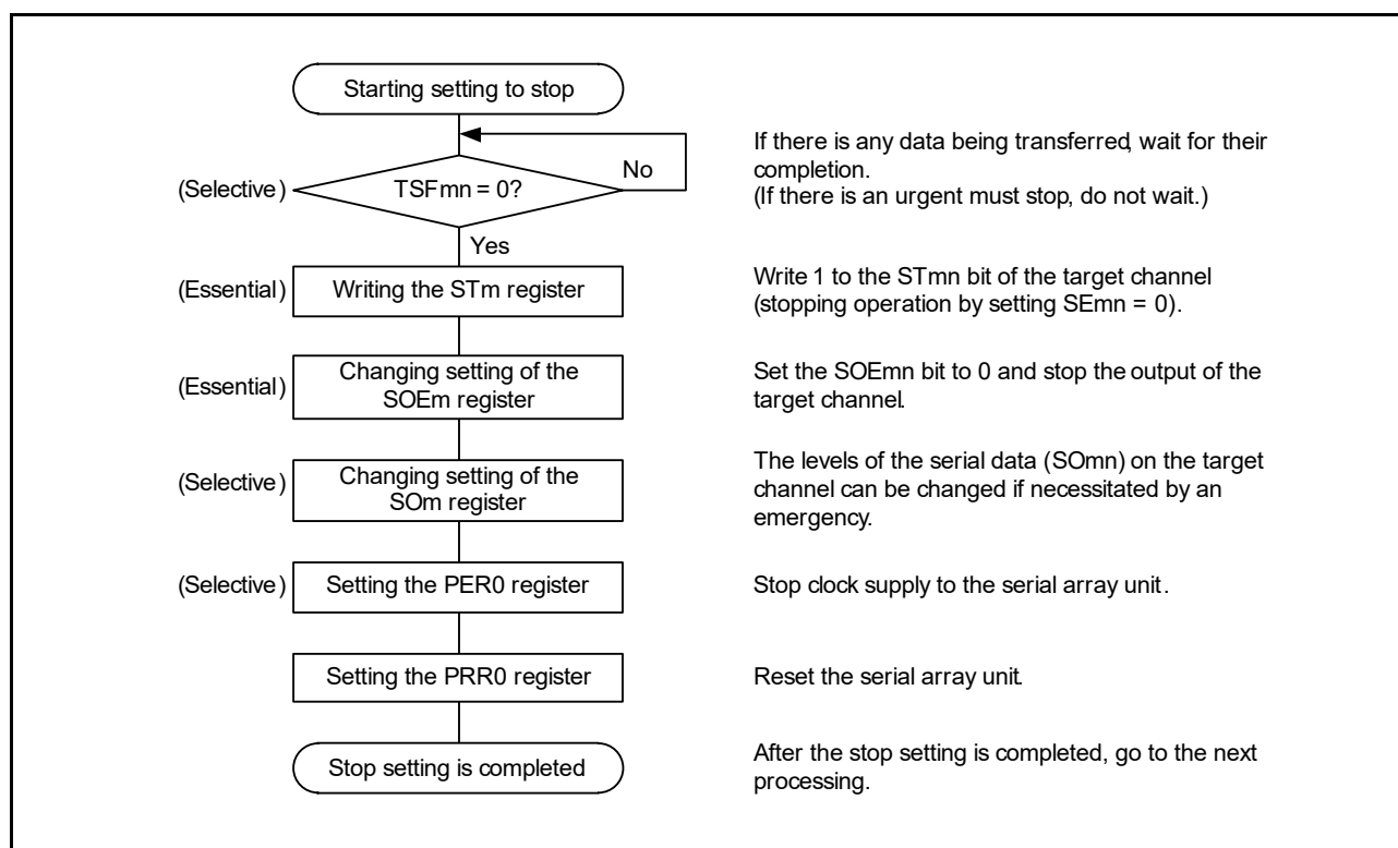
Figure 15 - 67 Procedure for Stopping Slave Transmission/Reception
