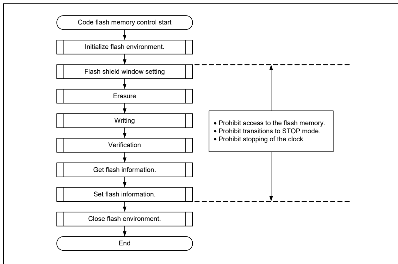
Figure 33 - 8 Flow of Self-Programming (Rewriting Flash Memory)
