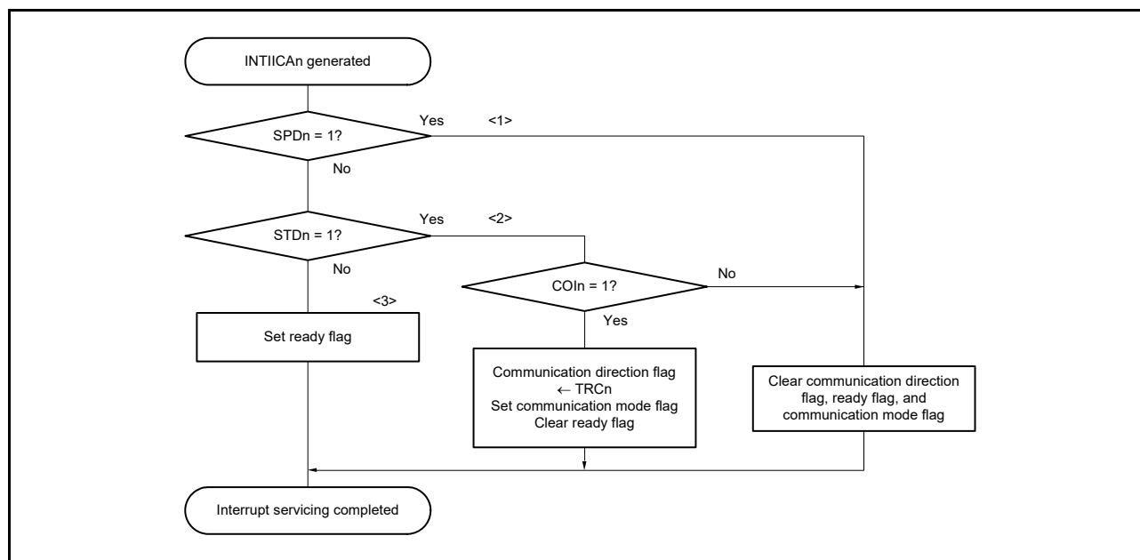
Figure 16 - 31 Slave Operation Flowchart (2)
