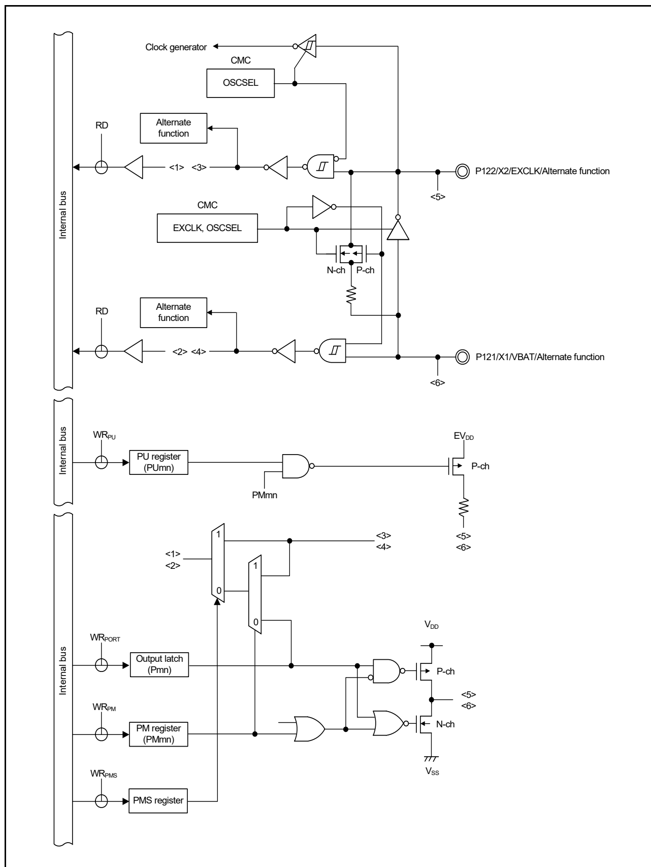
Figure 2 - 12 Pin Block Diagram for Pin Type 7-2-1
