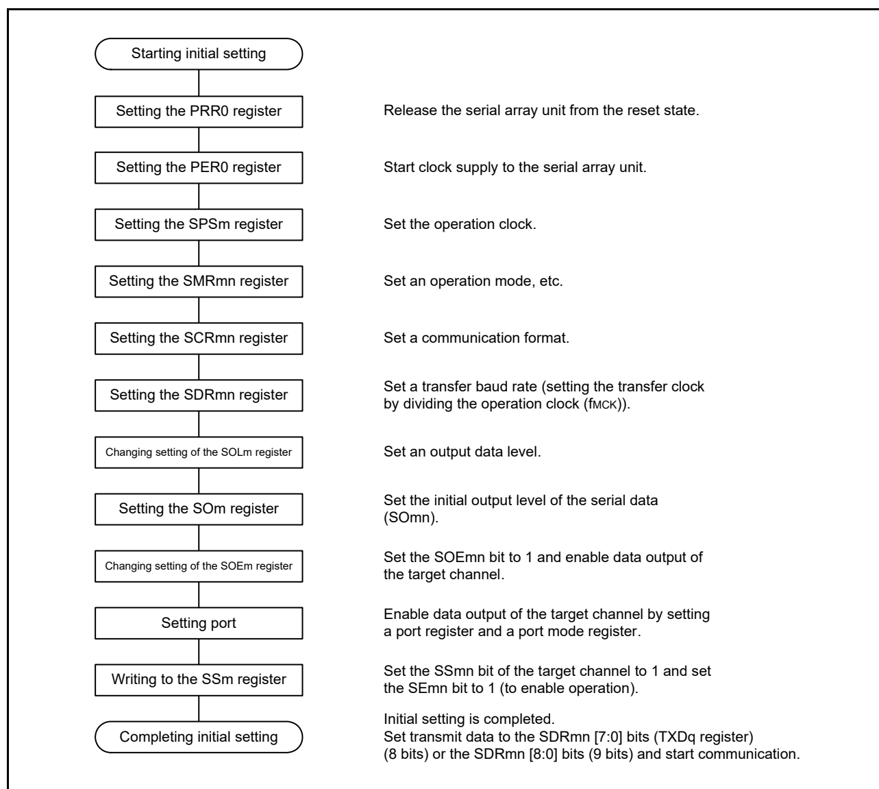
Figure 15 - 79 Initial Setting Procedure for UART Transmission
