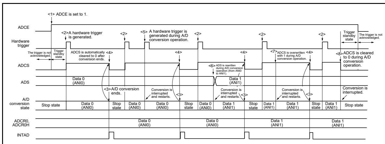
Figure 12 - 31 Example of Hardware Trigger Wait Mode (Select Mode, One-Shot Conversion Mode) Operation Timing
