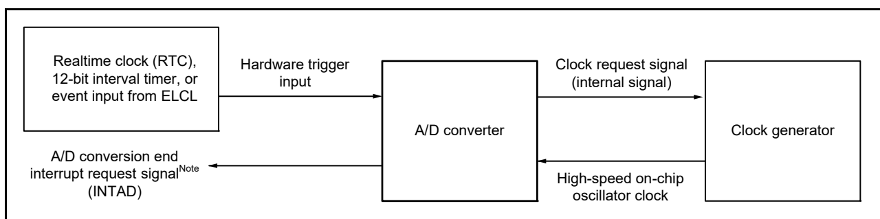
Figure 12 - 42 Block Diagram When Using SNOOZE Mode Function (in Hardware Trigger Wait Mode)
