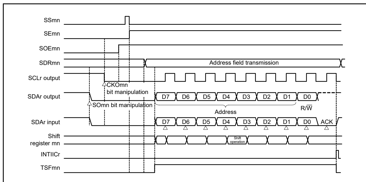
Figure 15 - 108 Timing Chart of Address Field Transmission
