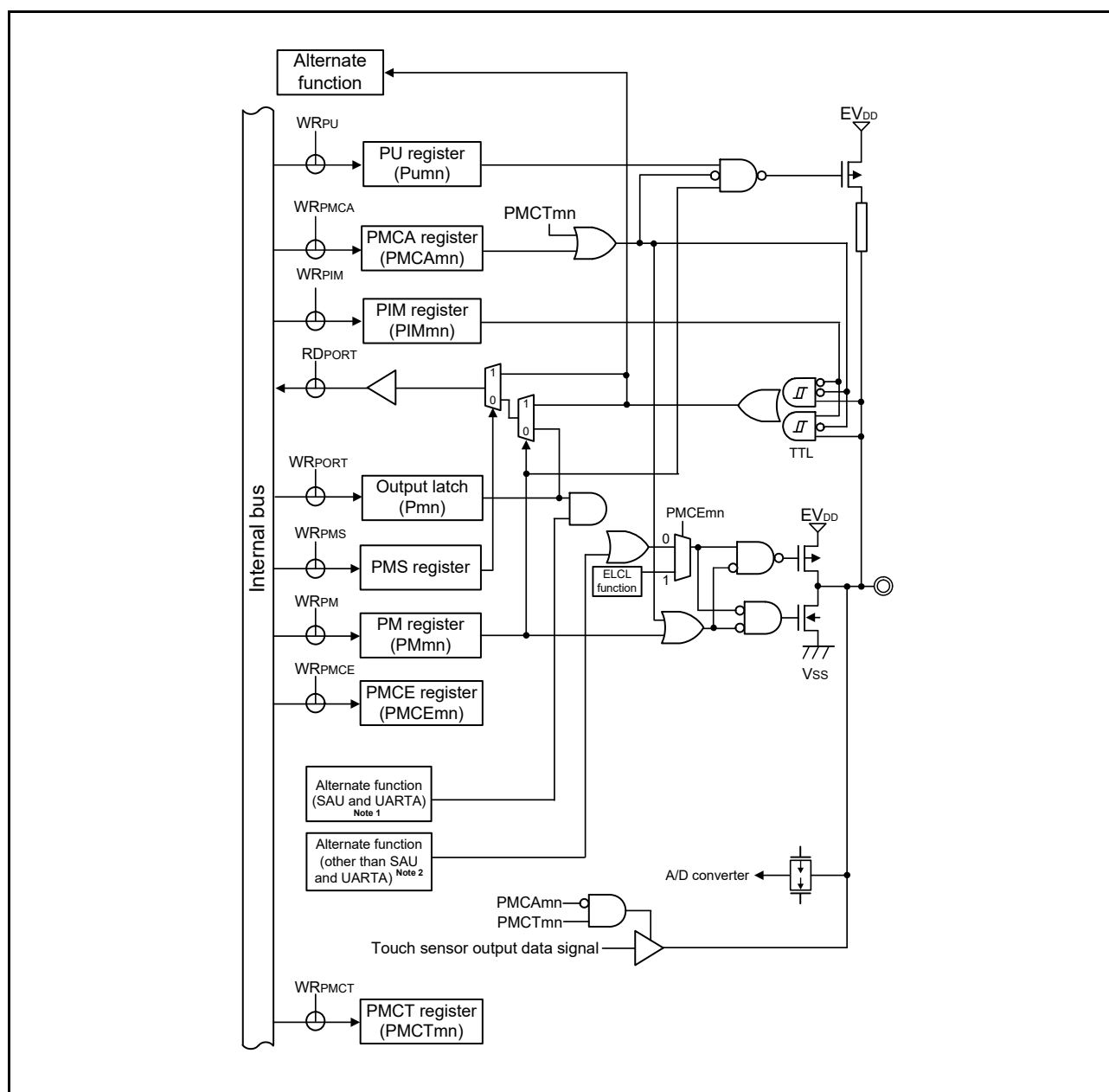
Figure 2 - 27 Pin Block Diagram for Pin Type 8-33-2
