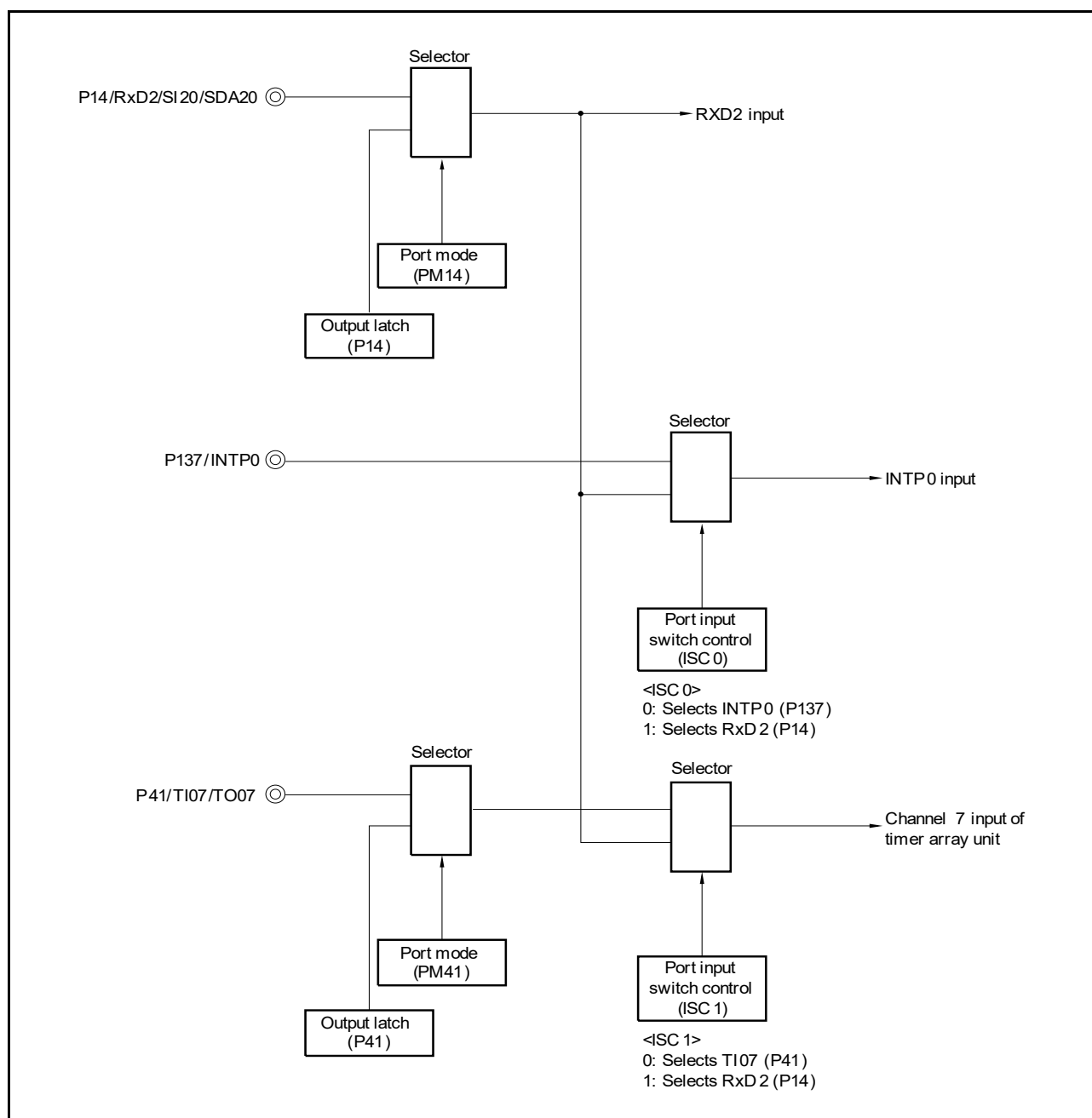
Figure 15 - 105 Port Configuration for Reception of LIN (44-, 48-, 52-, and 64-pin)
