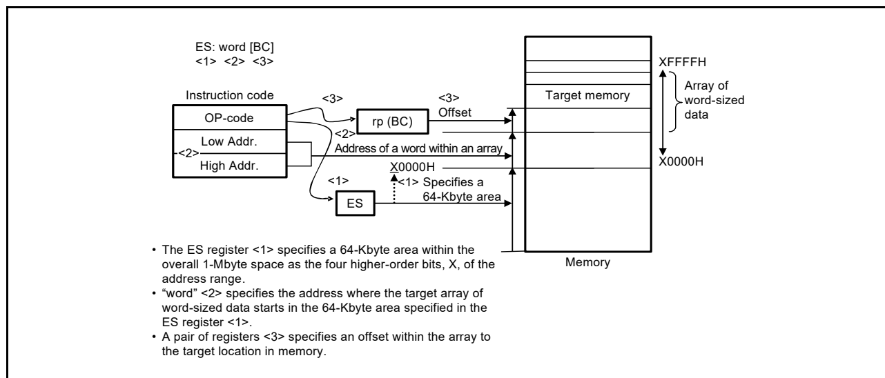
Figure 3 - 35 Example of ES:word [BC]
