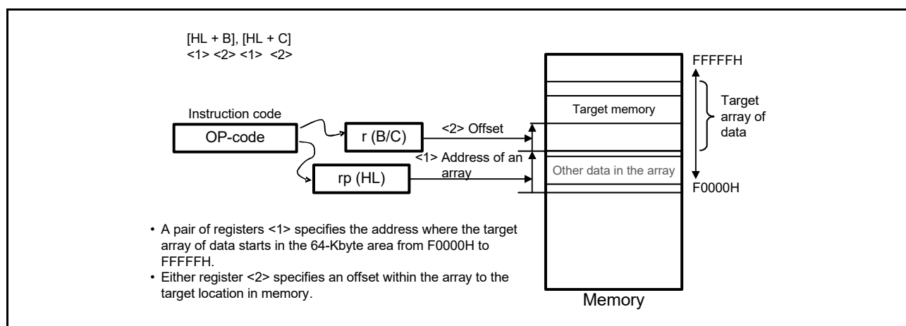
Figure 3 - 37 Example of ES:[HL + B], ES:[HL + C]
