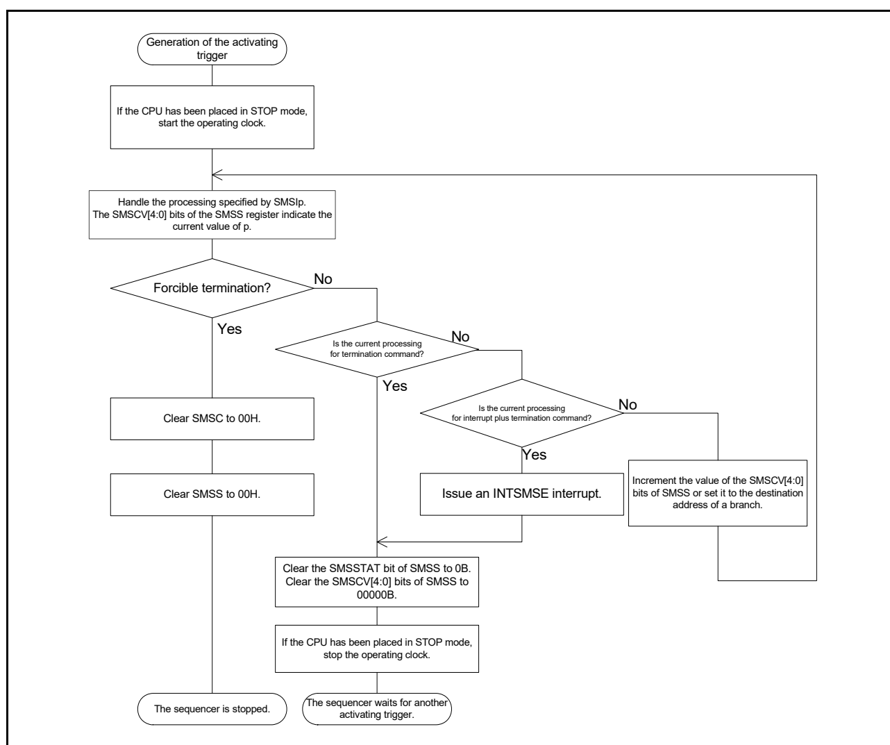
Figure 29 - 8 Flow of Internal Operations of the SNOOZE Mode Sequencer
