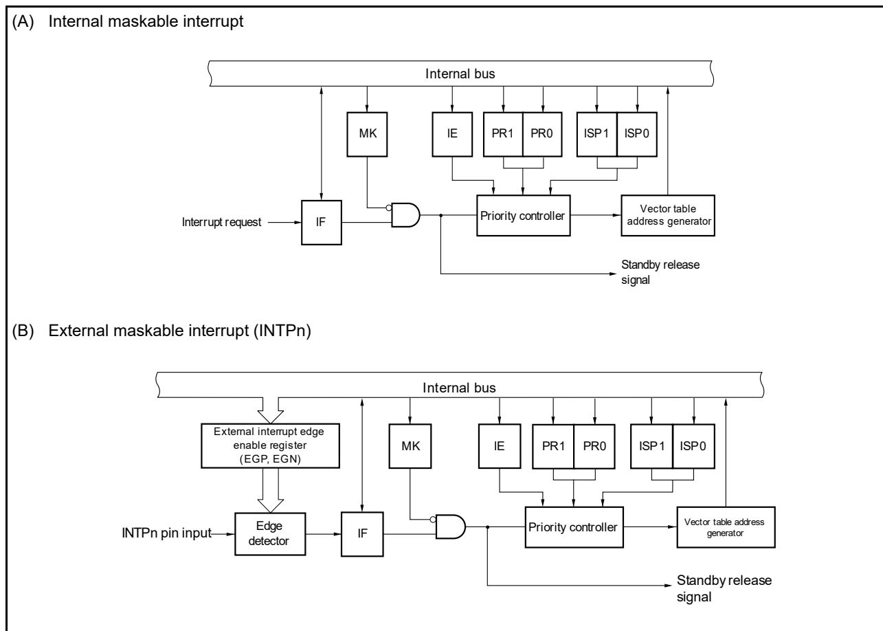
Figure 21 - 1 Basic Configuration of Interrupt Function (1/2)
