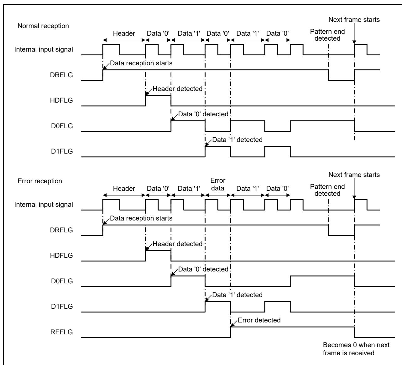
Figure 18 - 32 Example of Flag Operation
