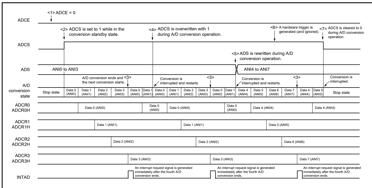
Figure 12 - 24 Example of Software Trigger Wait Mode (Scan Mode, Sequential Conversion Mode) Operation Timing
