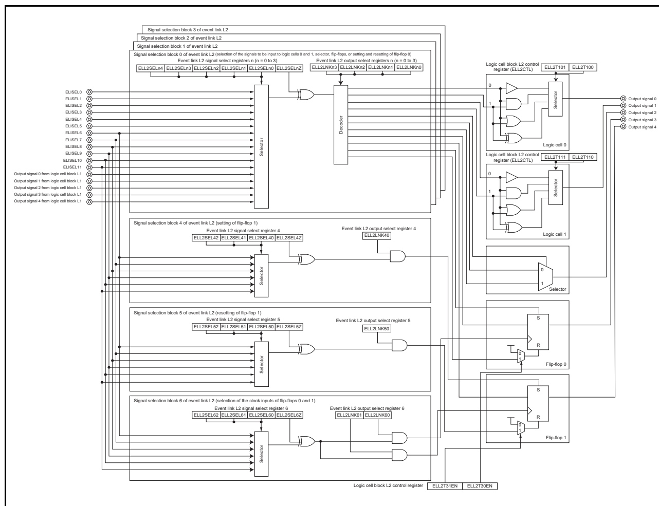
Figure 20 - 3 Block Diagram of Logic Cell Block L2
