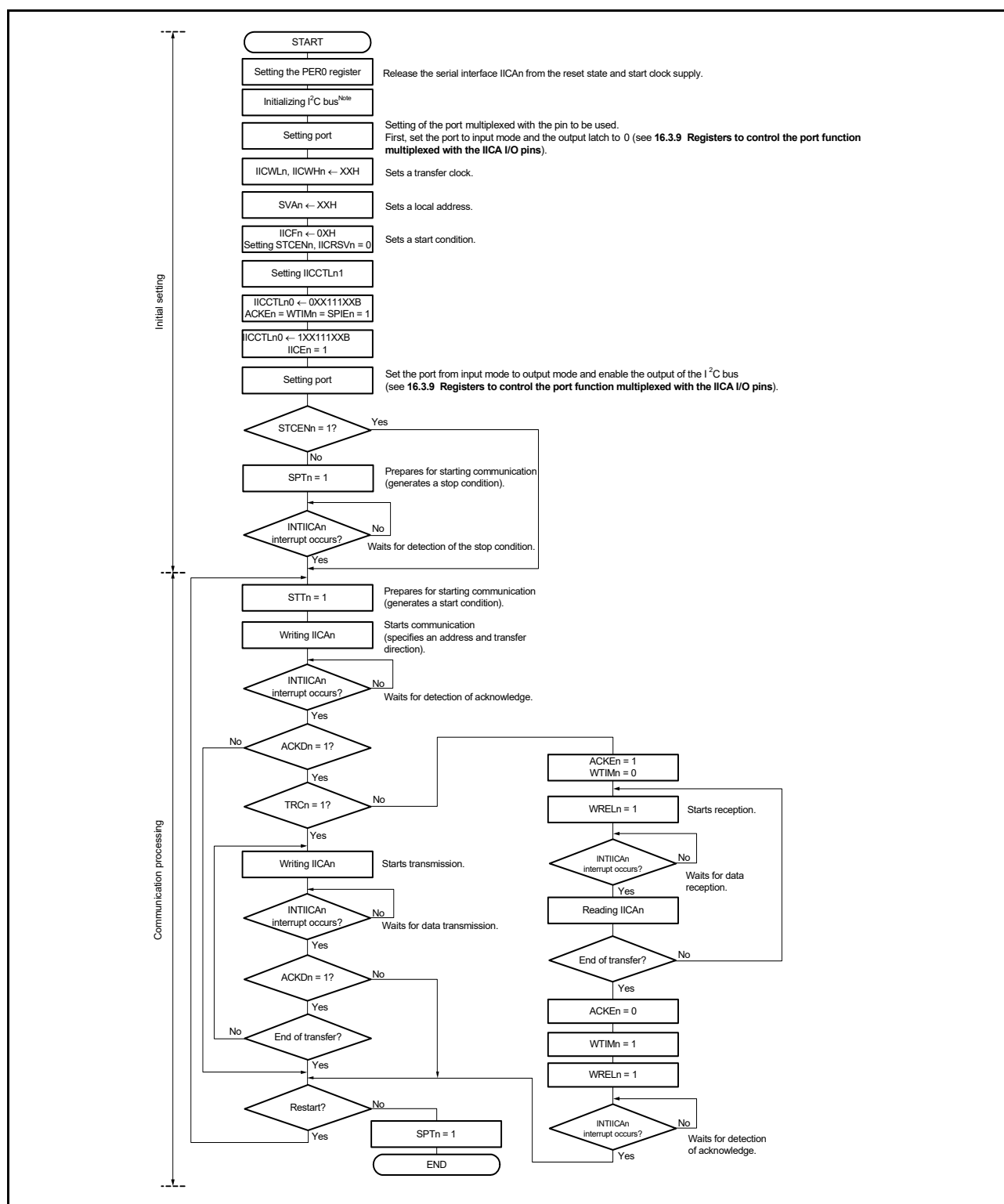
Figure 16 - 28 Master Operation in Single-Master System
