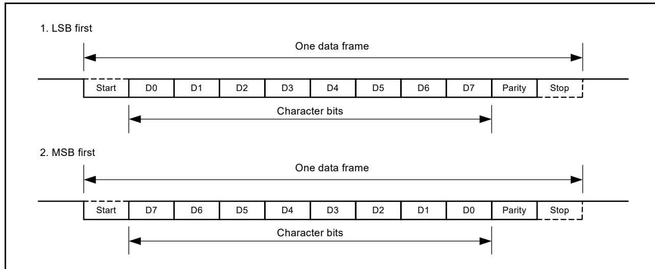
Figure 17 - 14 Transmit/Receive Data Format
