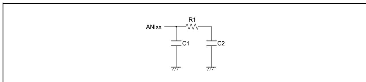
Figure 12 - 54 Internal Equivalent Circuit of ANIxx Pin
