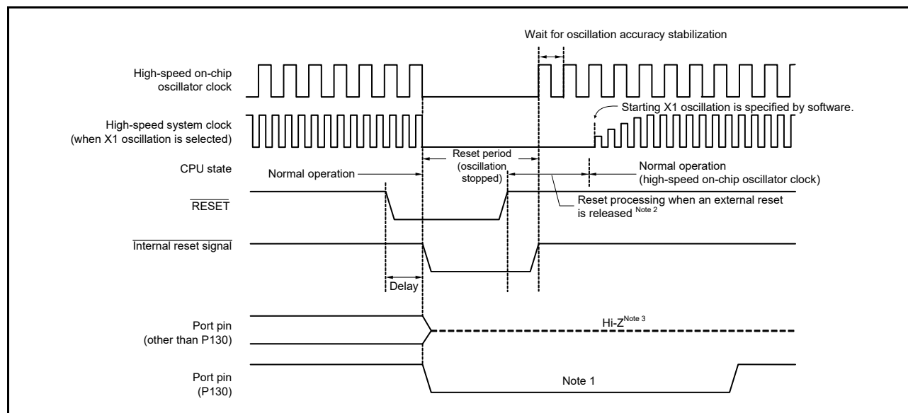
Figure 24 - 2 Timing of Reset by \overline{\text{RESET}} Input
