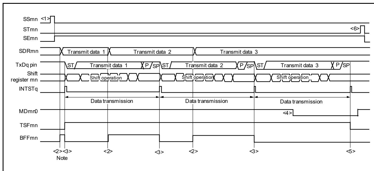
Figure 15 - 84 Timing Chart of UART Transmission (in Continuous Transmission Mode)
