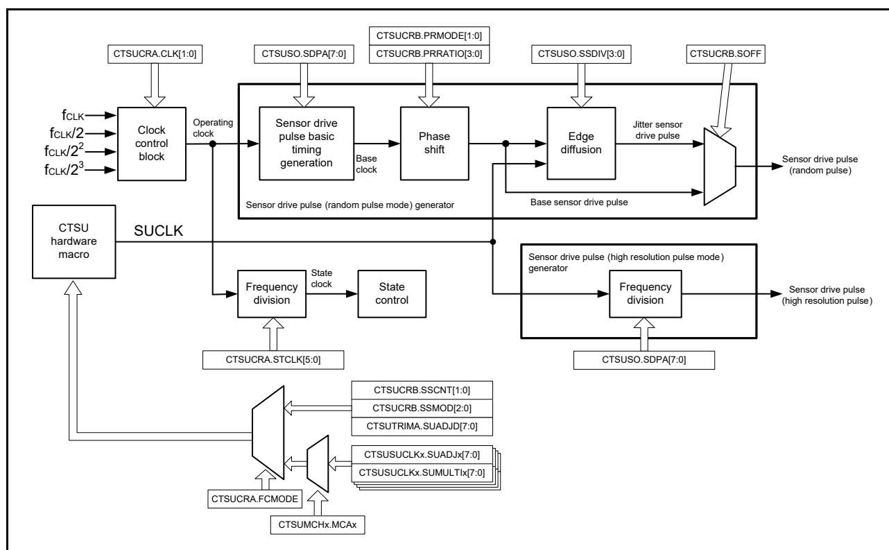
Figure 30 - 4 Sensor Drive Pulse Output Clock Configuration
