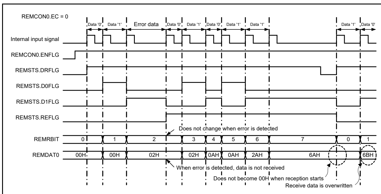
Figure 18 - 39 REMDAT0 and REMRBIT Registers Operation upon Error Detection (REMCN0.EC Bit = 0)
