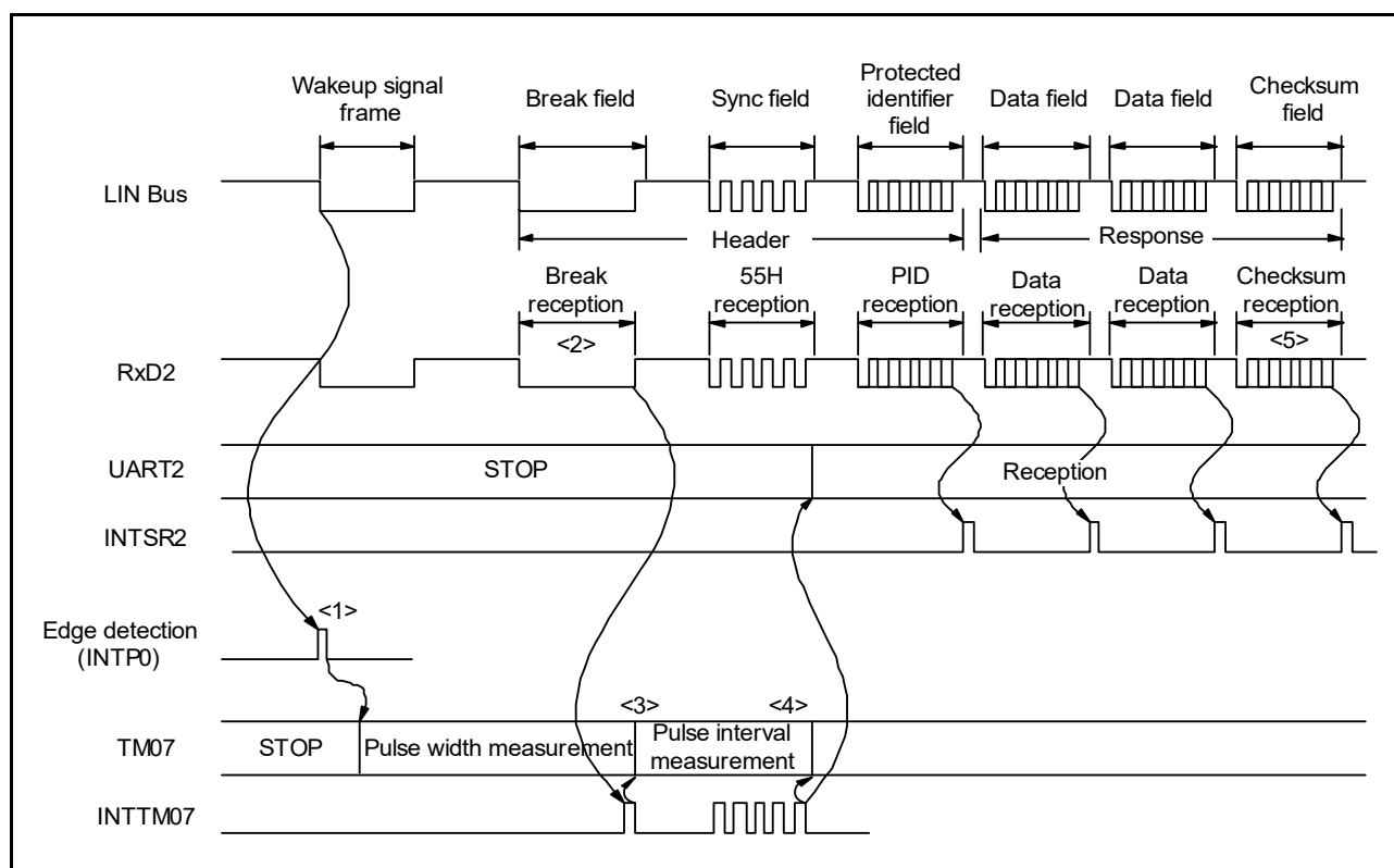
Figure 15 - 102 Reception Operation of LIN
