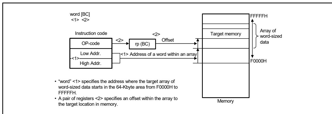
Figure 3 - 32 Example of word [BC]
