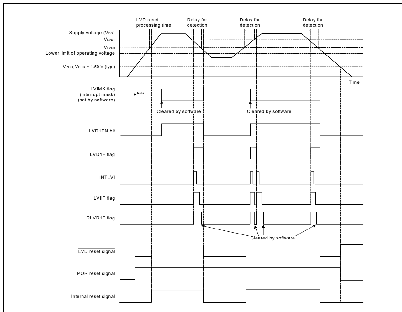
&lt;R&gt; Figure 26 - 9 Timing of LVD1 Interrupt Signal Generation
