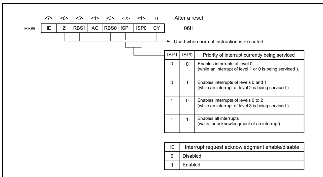
Figure 21 - 6 Configuration of Program Status Word
