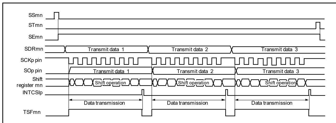
Figure 15 - 31 Timing Chart of Master Transmission (in Single-Transmission Mode) (Type 1: DAPmn = 0, CKPmn = 0)
