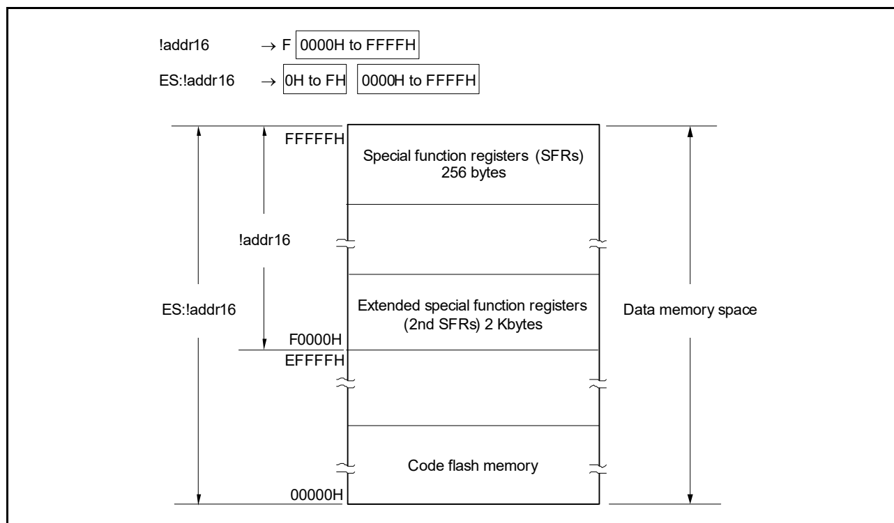
Figure 3 - 15 Extension of Data Area Which Can Be Accessed
