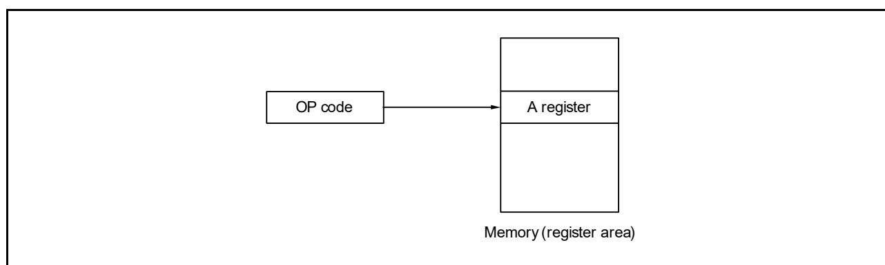
Figure 3 - 21 Outline of Implied Addressing
