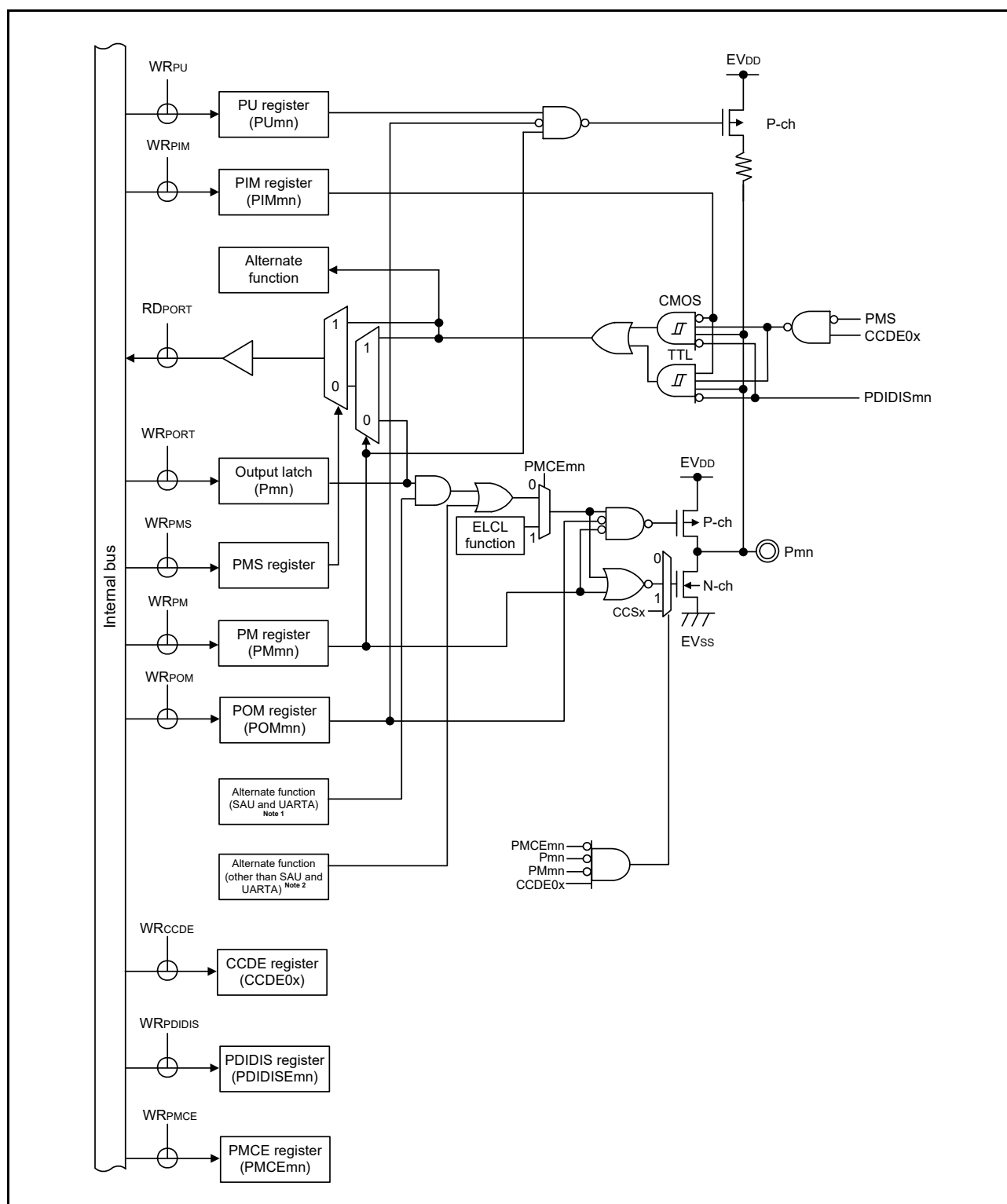
Figure 2 - 30 Pin Block Diagram for Pin Type 8-38-2
