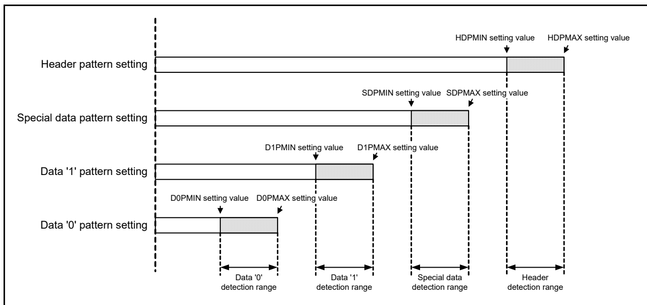
Figure 18 - 31 Examples of Setting Pattern Setting Registers
