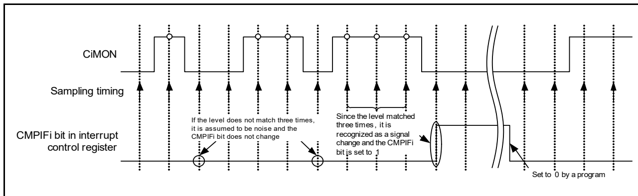
Figure 14 - 8 Comparator i (i = 0, 1) Digital Filter and Interrupt Operation Example
