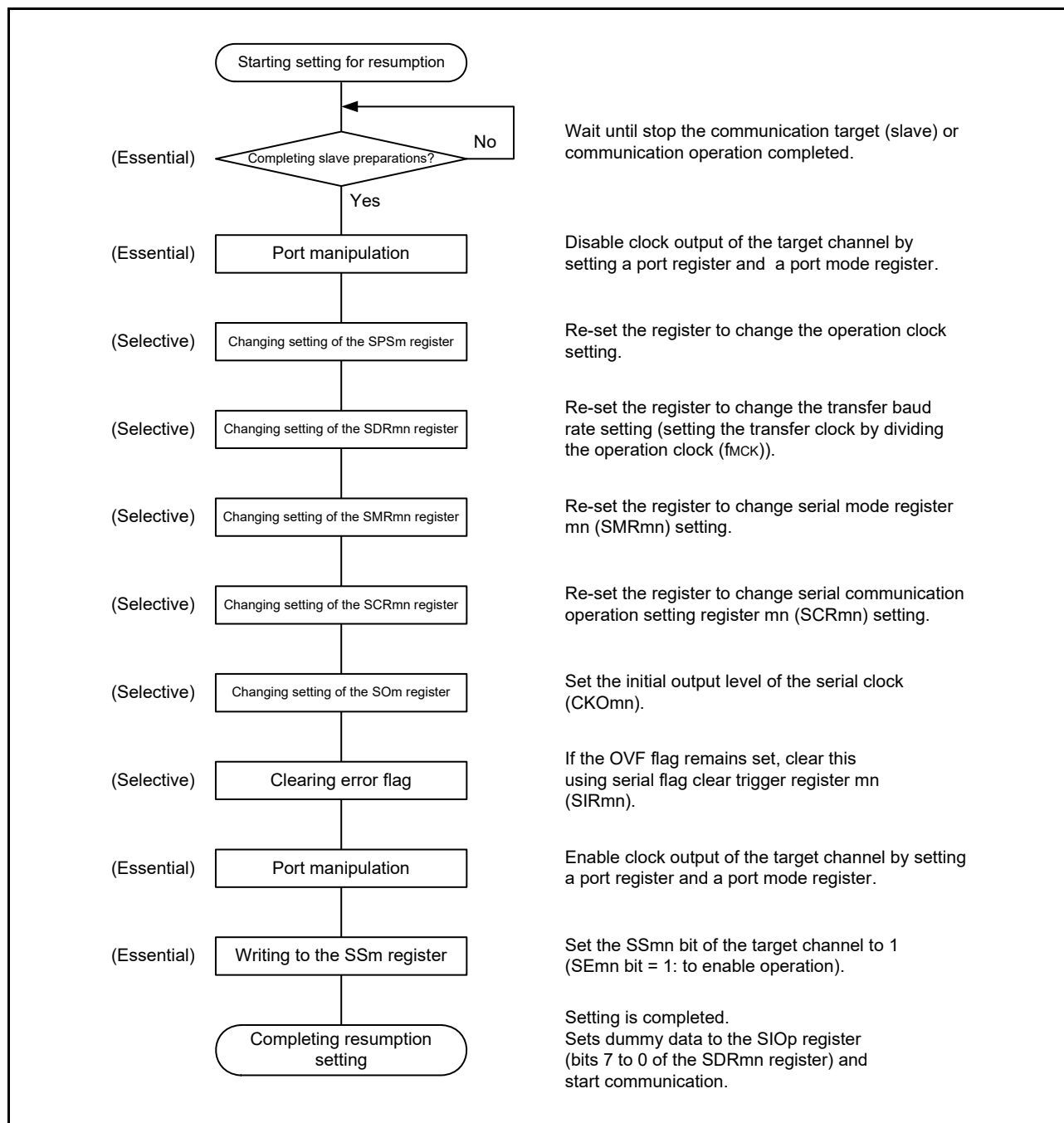
Figure 15 - 38 Procedure for Resuming Master Reception
