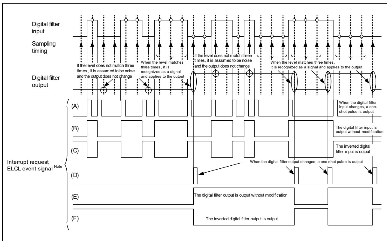
Figure 14 - 9 Digital Filter and Interrupt Request/Event Signal Output for the ELCL
