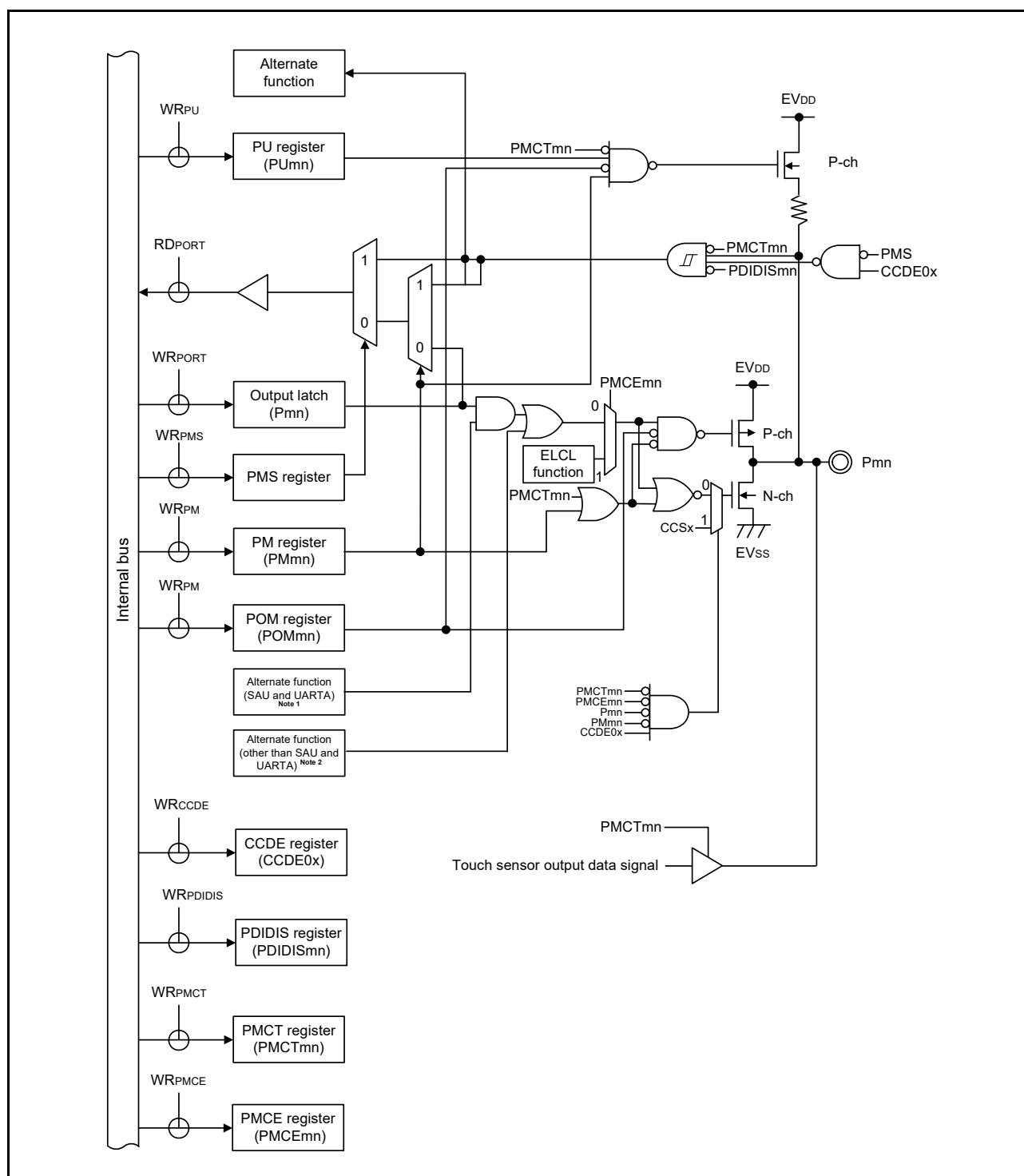
Figure 2 - 20 Pin Block Diagram for Pin Type 7-39-1
