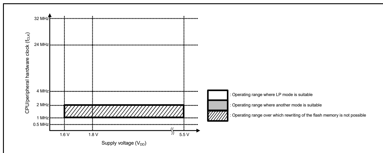
Figure 5 - 7 Operating Range in LP Mode
