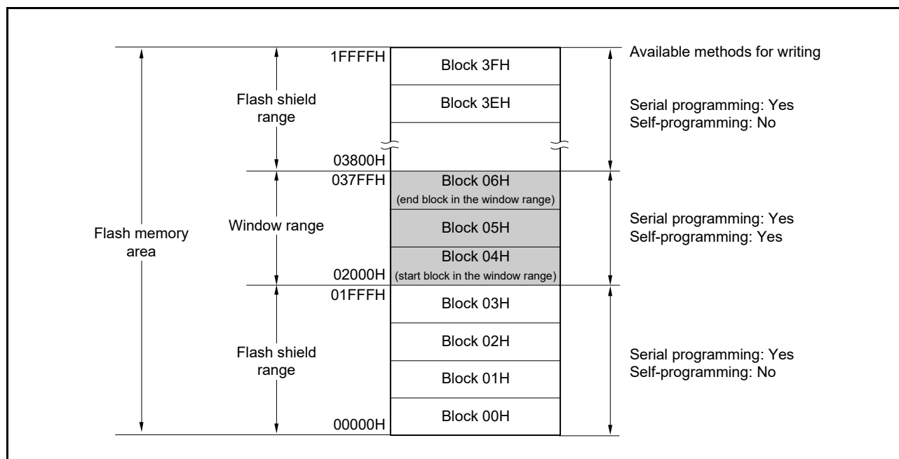
<R> Figure 33 - 29 Flash Shield Window Setting Example (Target Devices: R7F100GLG, Start Block Number in the Window Range: 04H, End Block Number in the Window Range: 06H, FSWC: 1)
