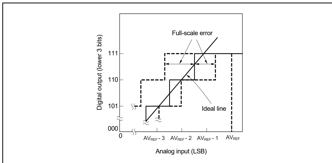
Figure 12 - 49 Full-Scale Error
