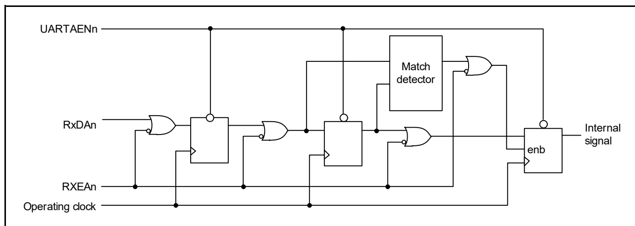
Figure 17 - 23 Noise Filter
