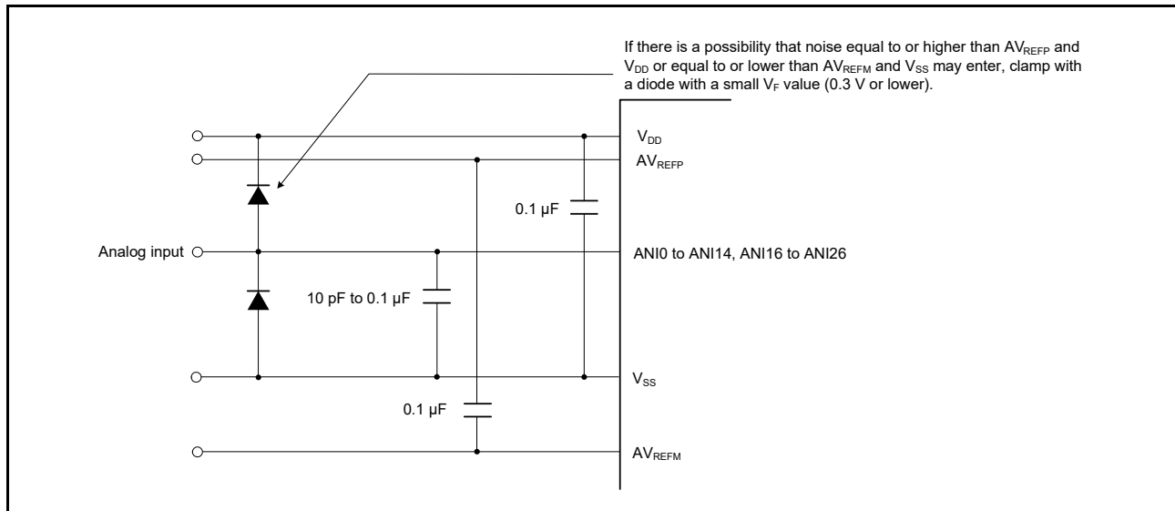
Figure 12 - 52 Connections of VDD, AVREFP, and Analog Input Pins
