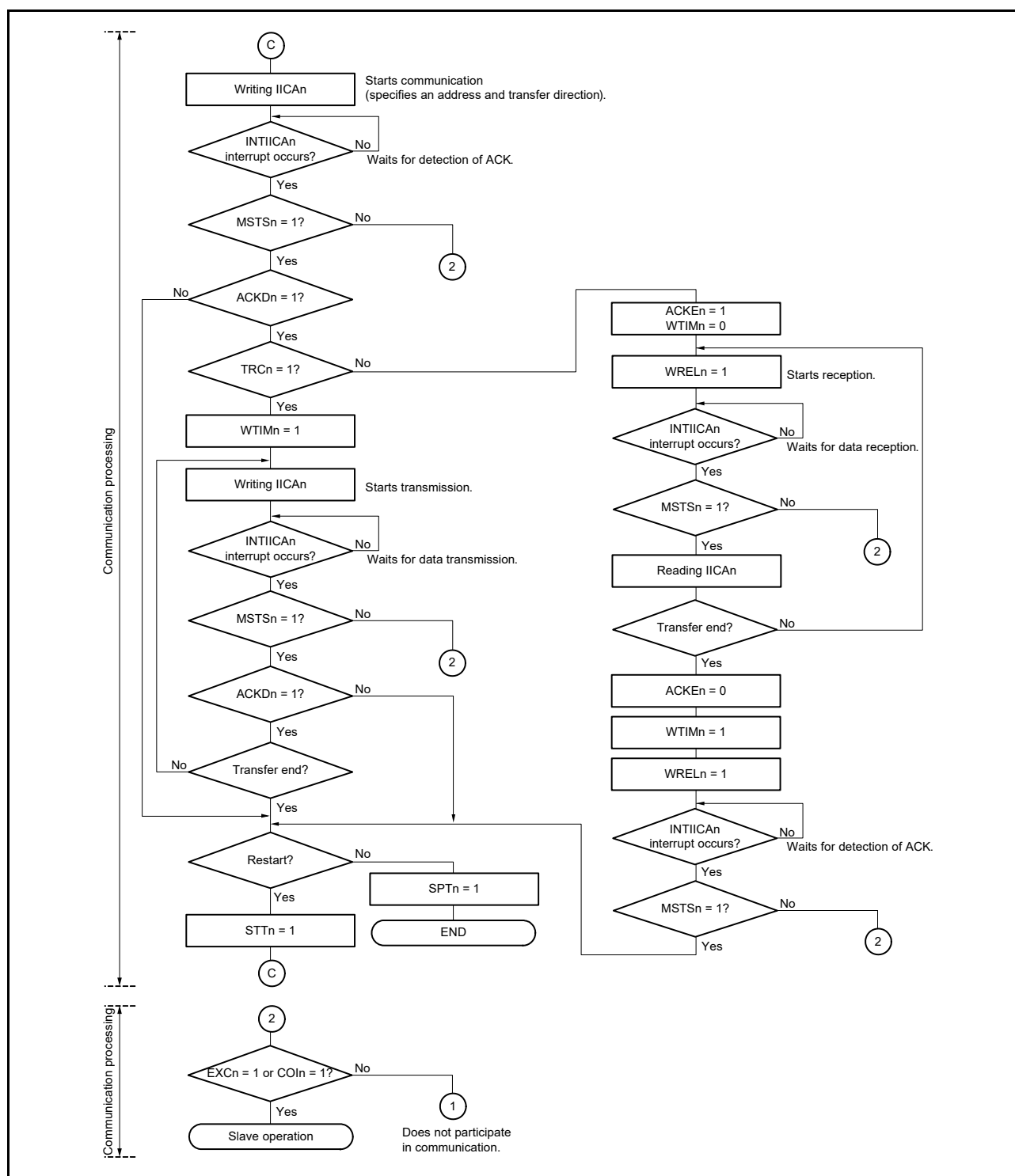
Figure 16 - 29 Master Operation in Multi-Master System (3/3)
