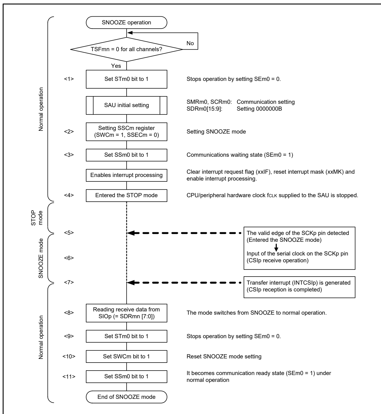
Figure 15 - 74 Flowchart of SNOOZE Mode Operation (once startup)
