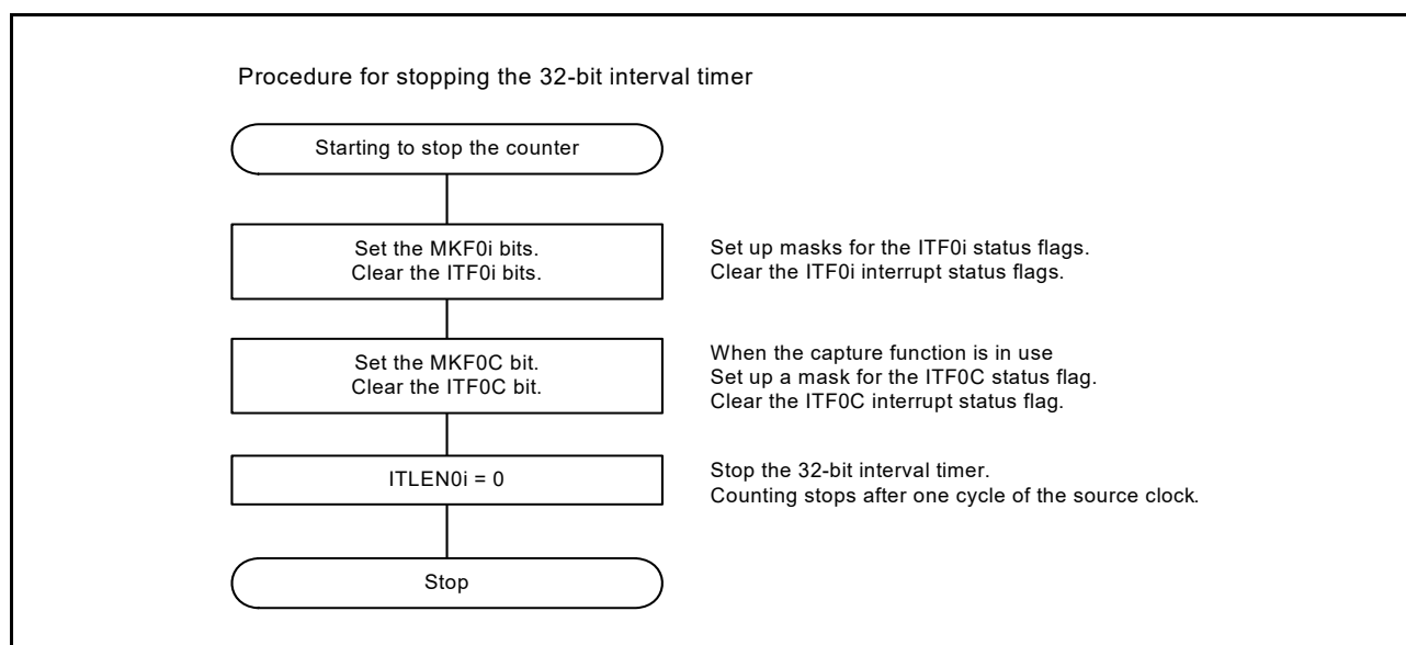
Figure 9 - 17 Procedure for Stopping the 32-Bit Interval Timer
