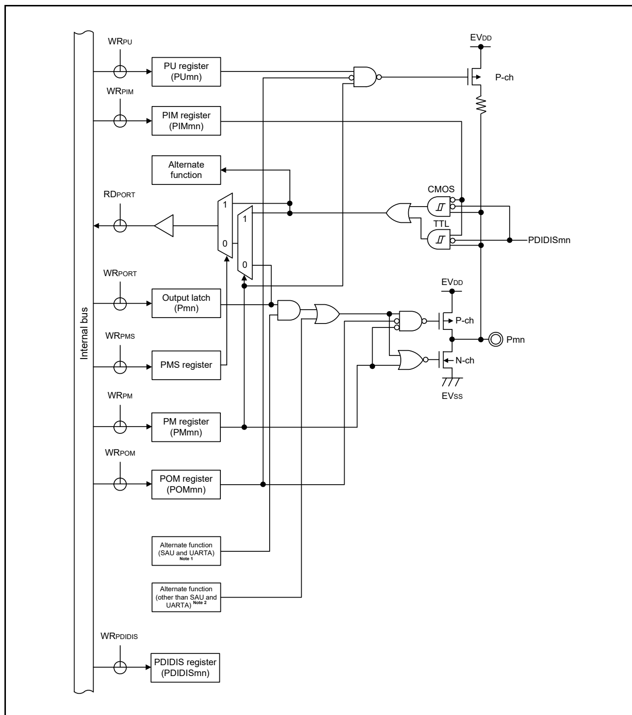
Figure 2 - 22 Pin Block Diagram for Pin Type 8-1-10
