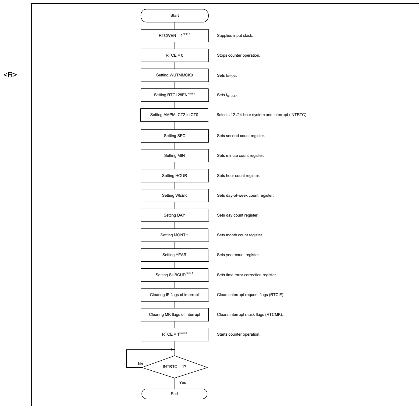
Figure 8 - 19 Procedure for Starting the Realtime Clock Operation
