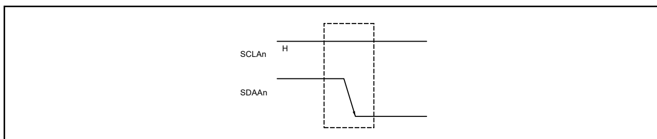
Figure 16 - 15 Start Conditions
