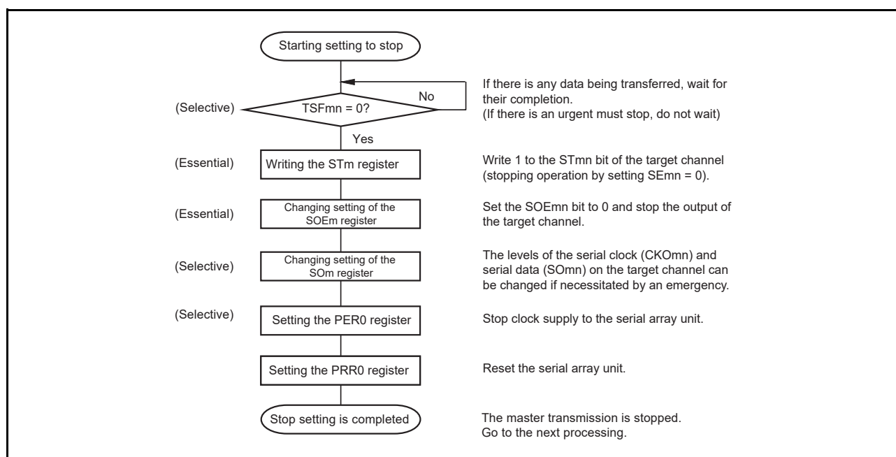
Figure 15 - 29 Procedure for Stopping Master Transmission
