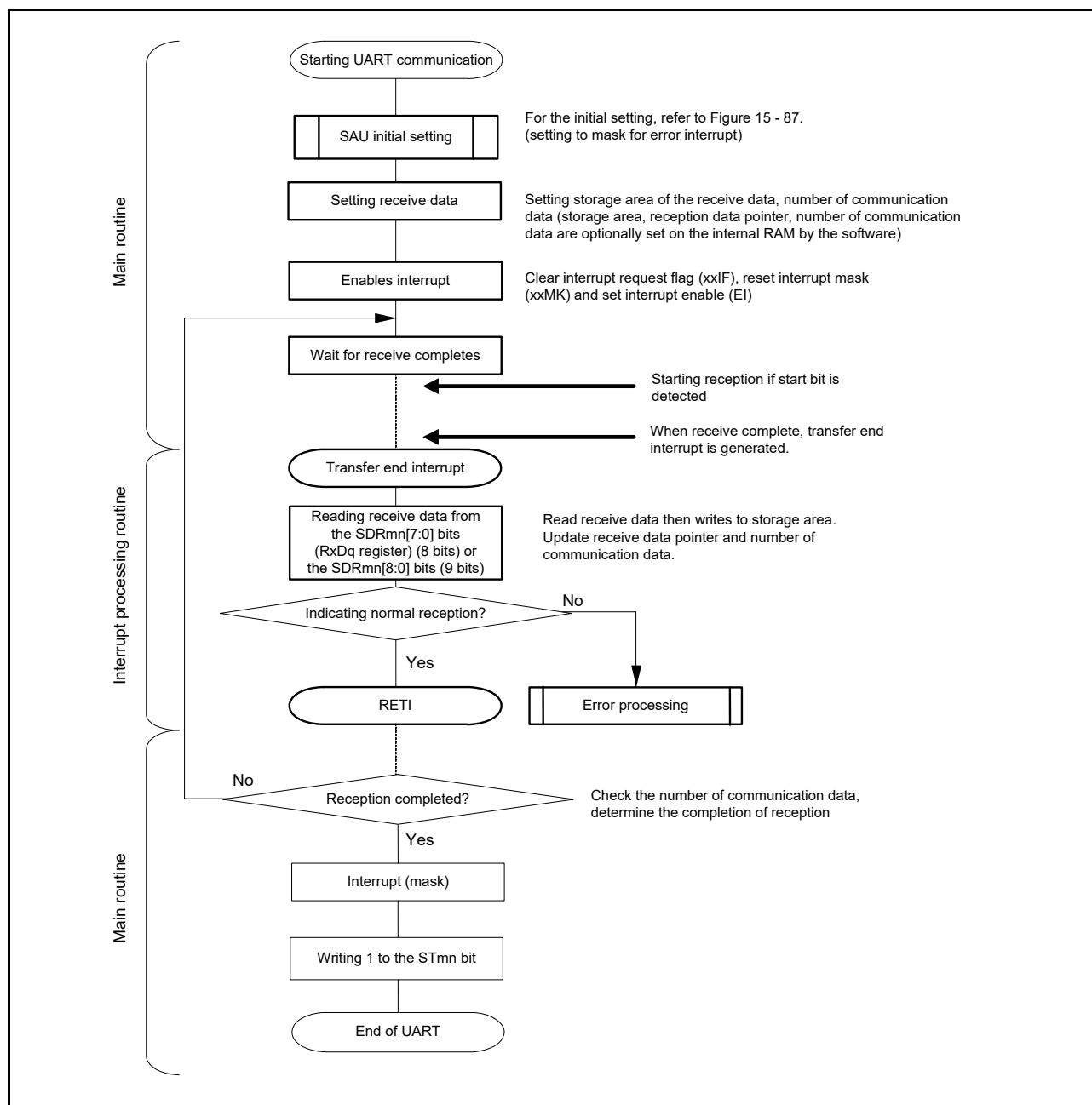
Figure 15 - 91 Flowchart of UART Reception
