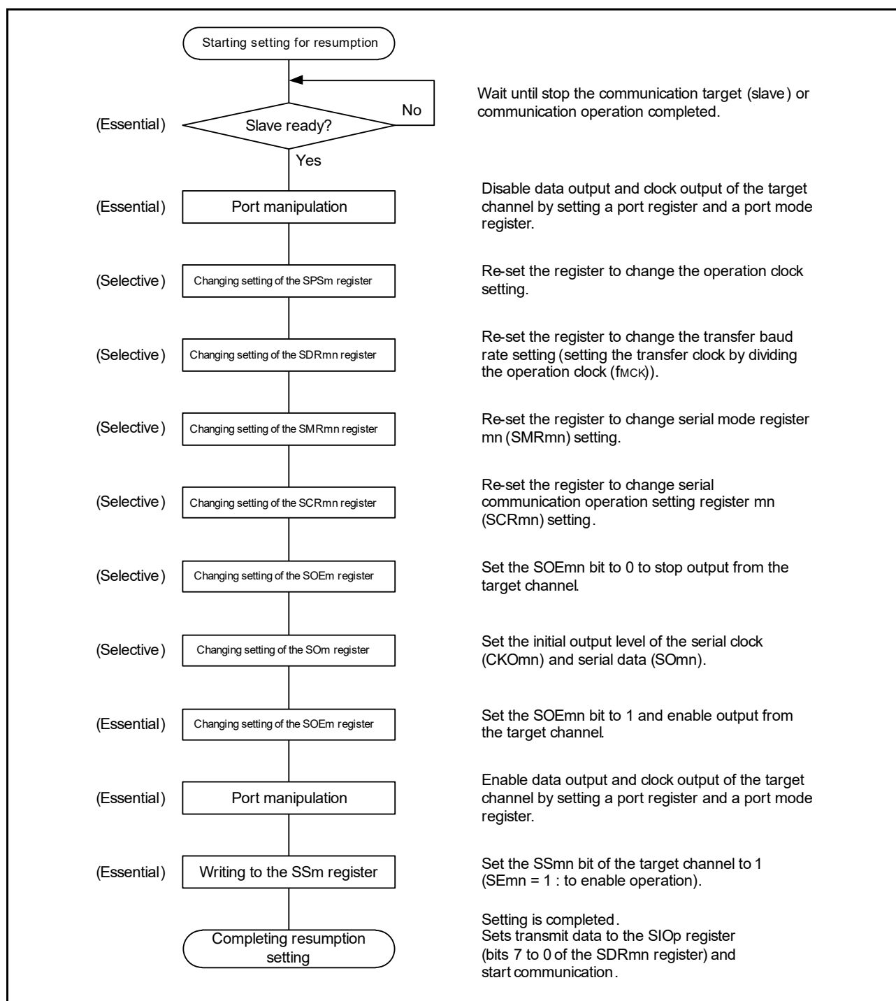
Figure 15 - 30 Procedure for Resuming Master Transmission
