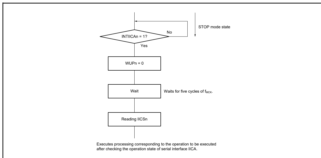
Figure 16 - 23 Flow When Setting WUPn = 0 upon Address Match (or When the All Address Match Function is Enabled) (Including Extension Code Reception)
