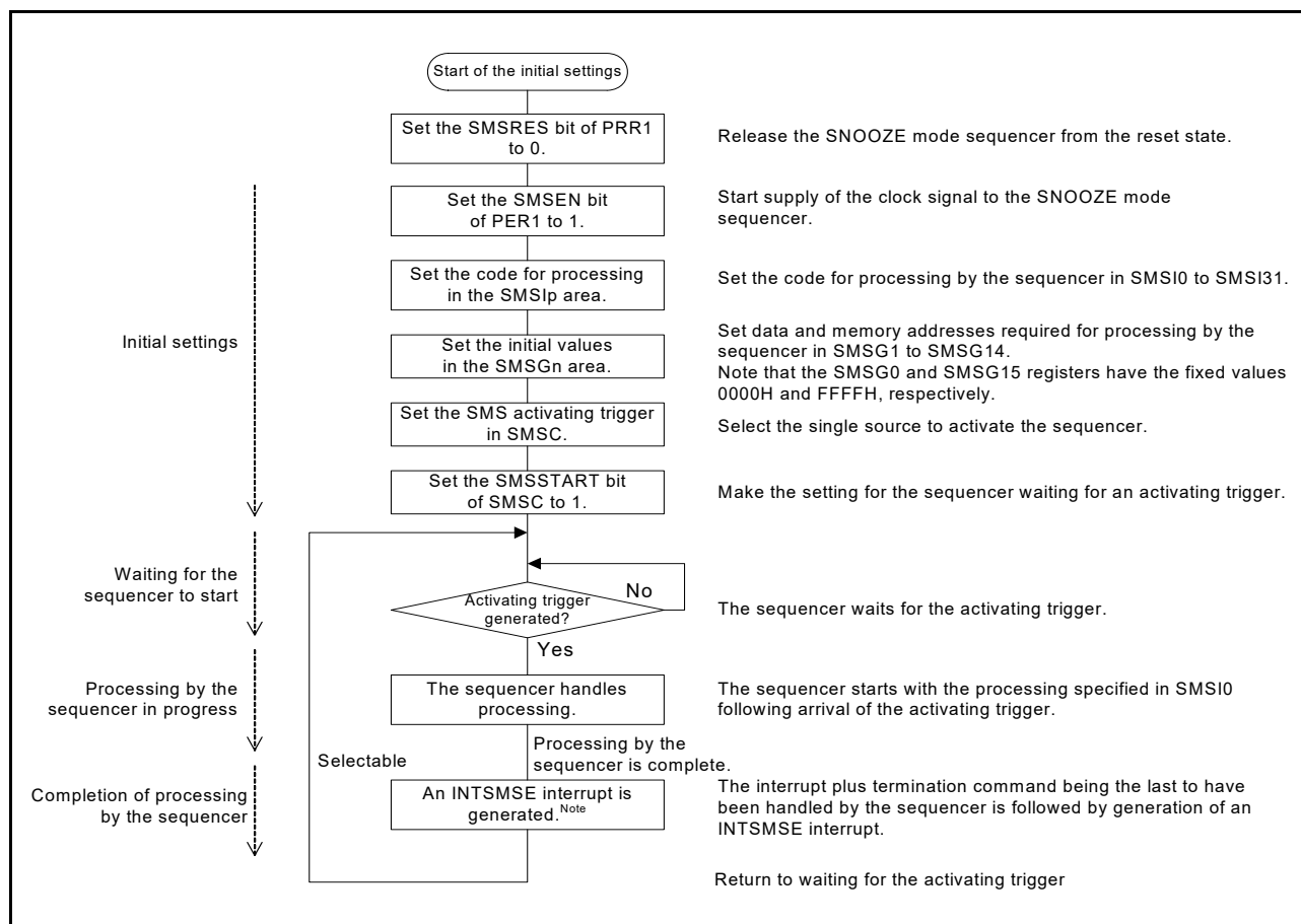
Figure 29 - 11 Flow of Activating and Running the SNOOZE Mode Sequencer
