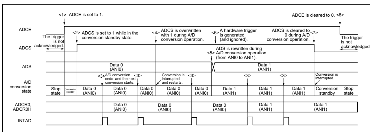
Figure 12 - 18 Example of Software Trigger No-Wait Mode (Select Mode, Sequential Conversion Mode) Operation Timing
