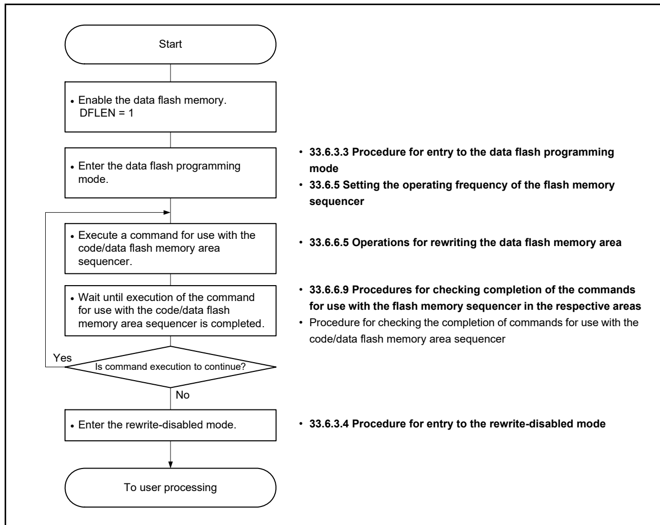
Figure 33 - 31 Flow of Executing the Commands to Rewrite the Data Flash Memory Area
