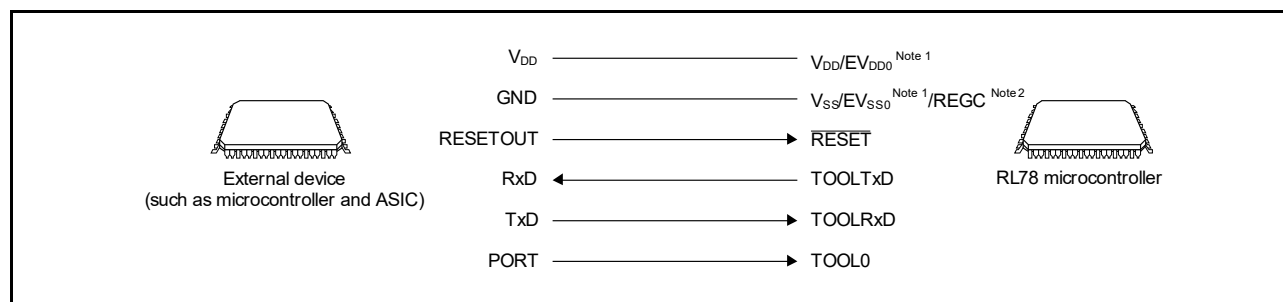
Figure 33 - 4 Communication with External Device
