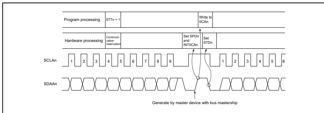
Figure 16 - 25 Communication Reservation Timing
