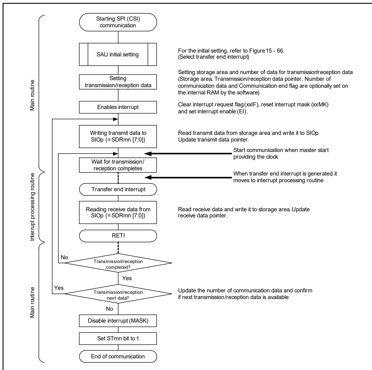
Figure 15 - 70 Flowchart of Slave Transmission/Reception (in Single-Transmission/Reception Mode)
