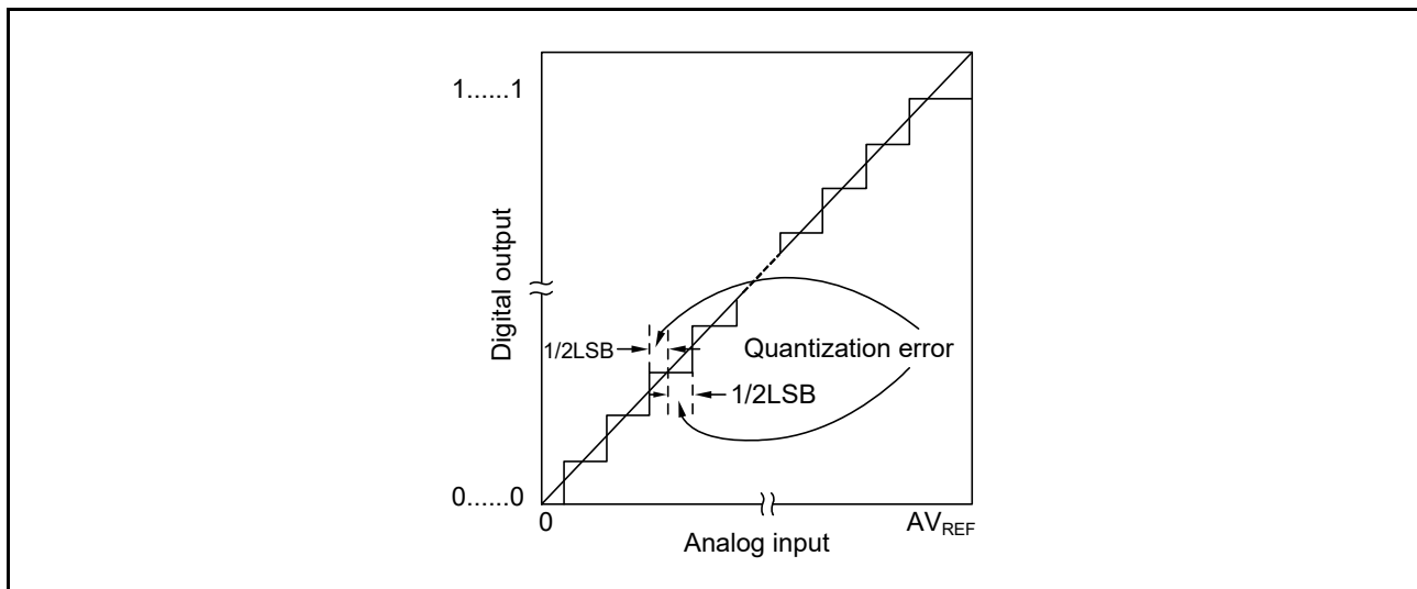
Figure 12 - 47 Quantization Error
