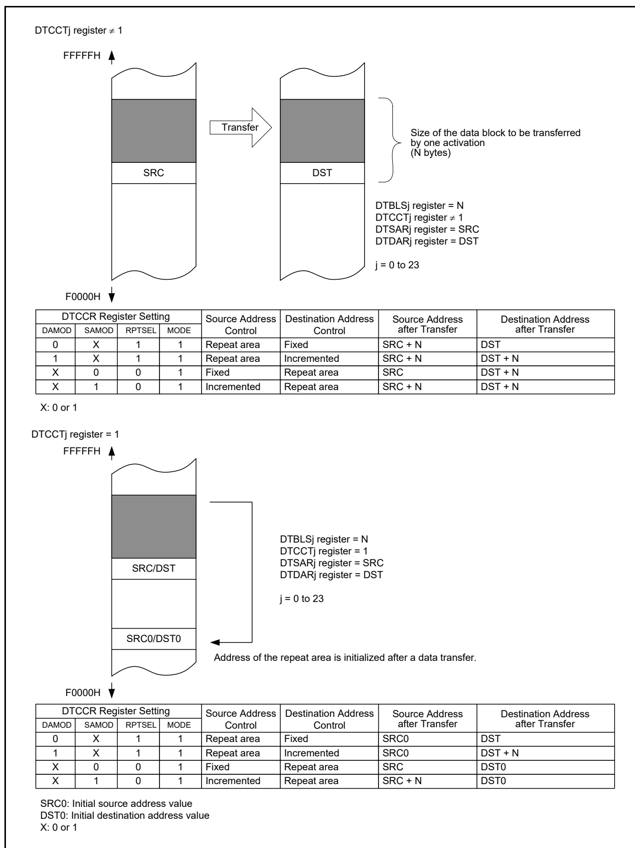
Figure 19 - 18 Data Transfers in Repeat Mode
