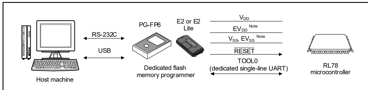
Figure 33 - 1 Environment for Writing Program to Flash Memory
