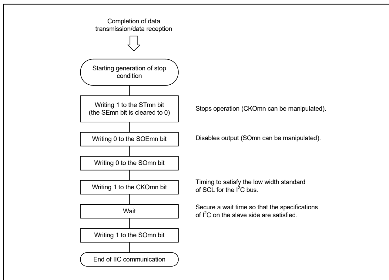
Figure 15 - 117 Flowchart of Stop Condition Generation
