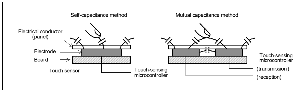
Figure 30 - 2 Self-capacitance Method and Mutual Capacitance Method
