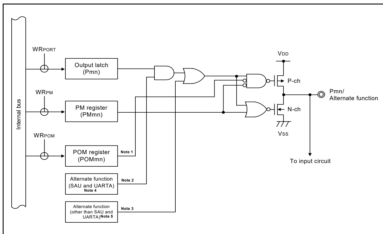
Figure 4 - 17 Basic Configuration of Output Circuit for a Pin
