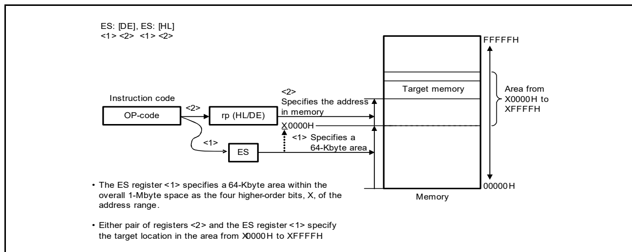
Figure 3 - 28 Example of ES:[DE], ES:[HL]
