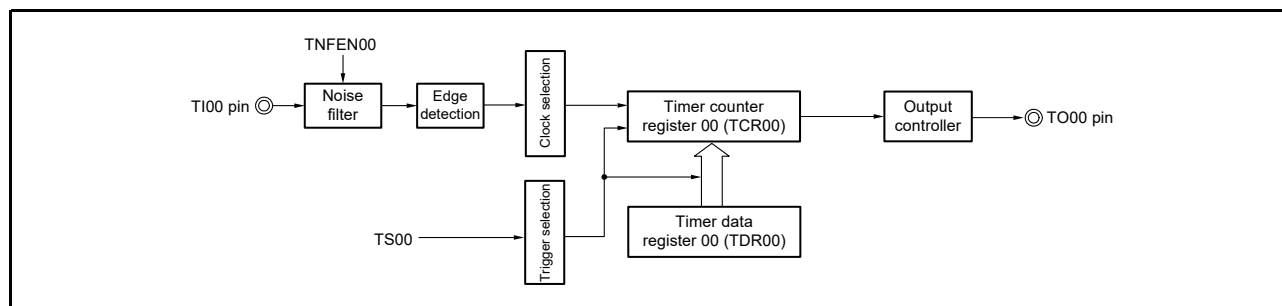
Figure 7 - 53 Block Diagram for Operation as a Frequency Divider
