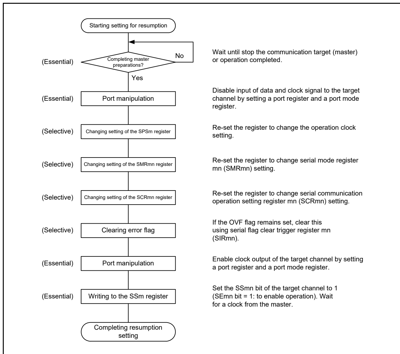
Figure 15 - 62 Procedure for Resuming Slave Reception
