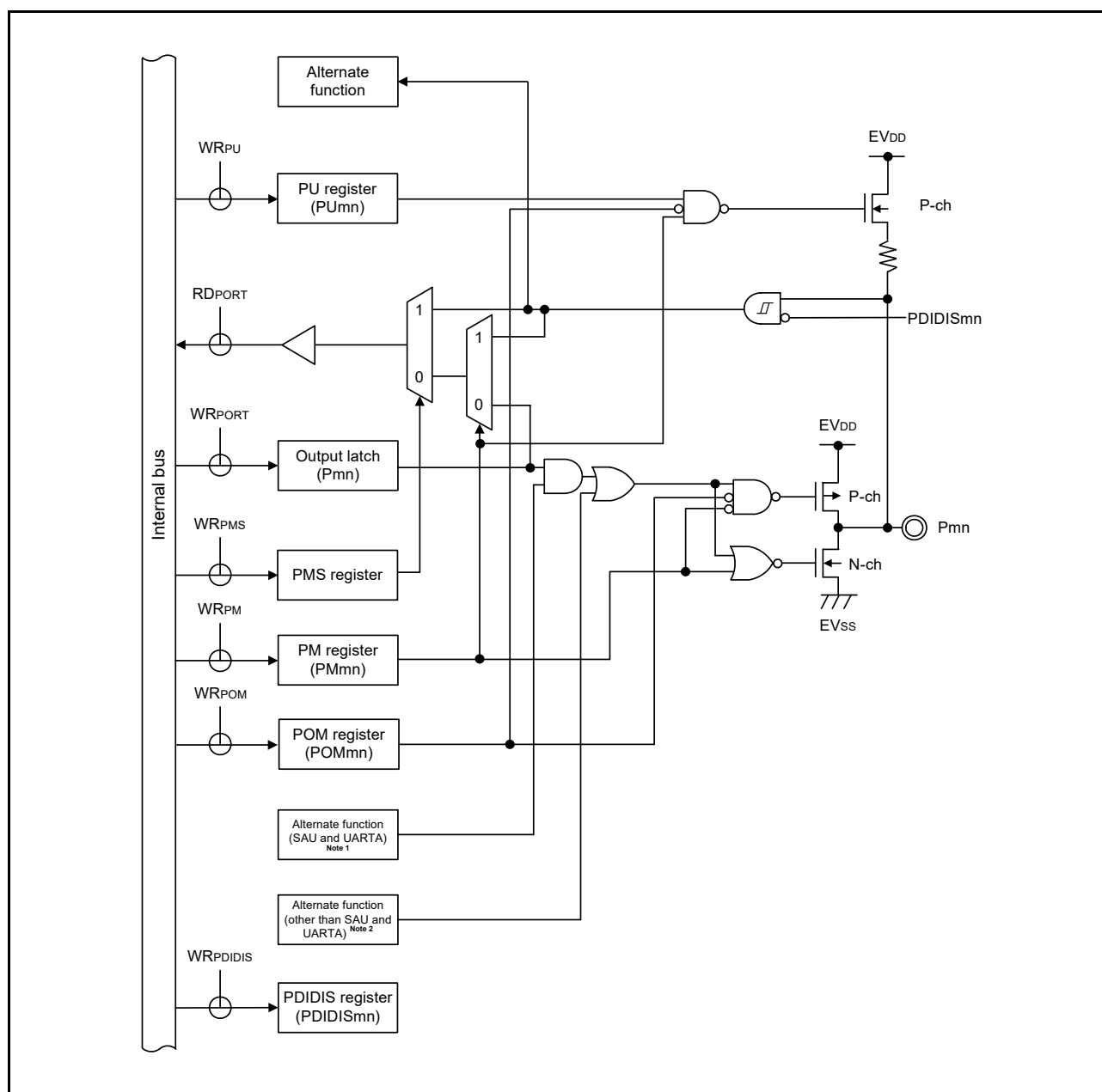
Figure 2 - 10 Pin Block Diagram for Pin Type 7-1-11
