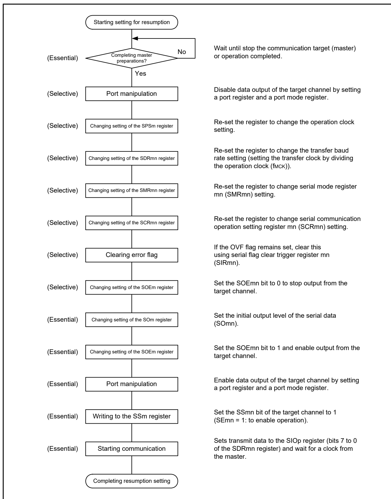
Figure 15 - 54 Procedure for Resuming Slave Transmission
