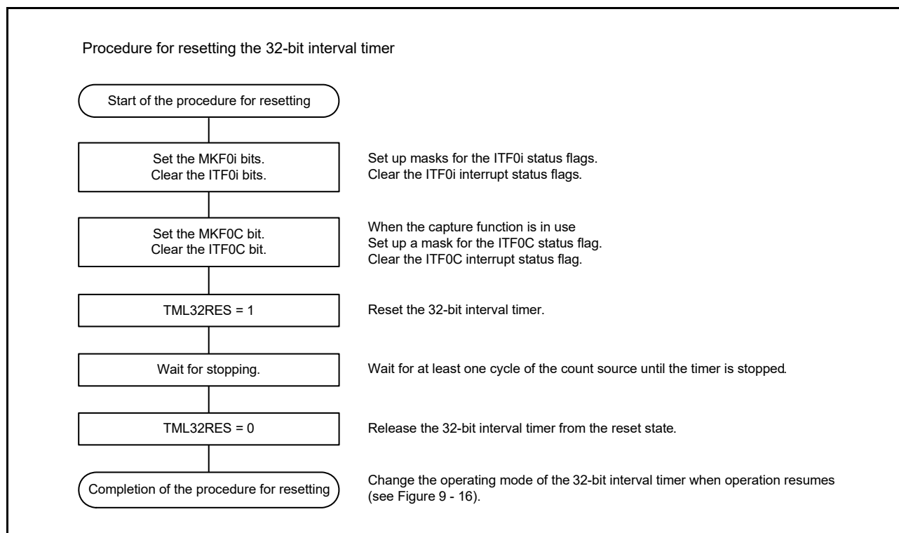
Figure 9 - 19 Procedure for Resetting the 32-Bit Interval Timer
