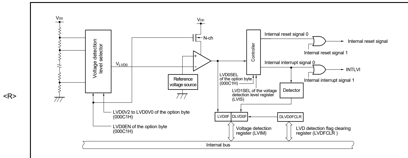
Figure 26 - 1 Block Diagram of LVD0
