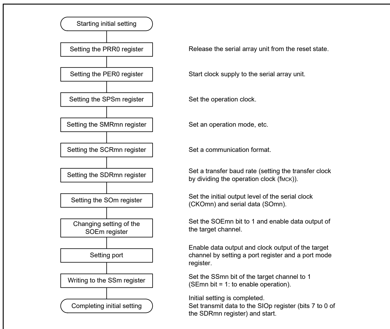
Figure 15 - 44 Initial Setting Procedure for Master Transmission/Reception
