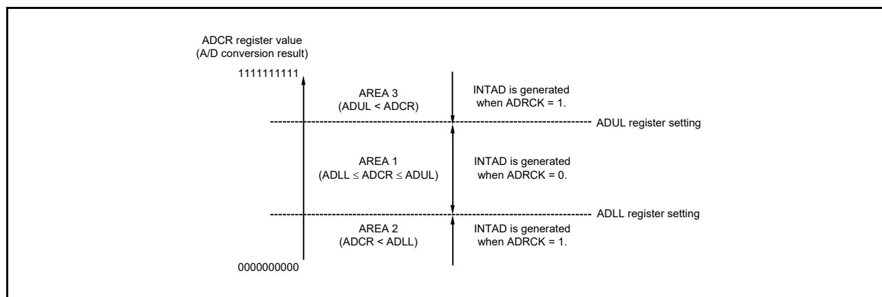
Figure 12 - 9 ADRCK Bit Interrupt Signal Generation Range
