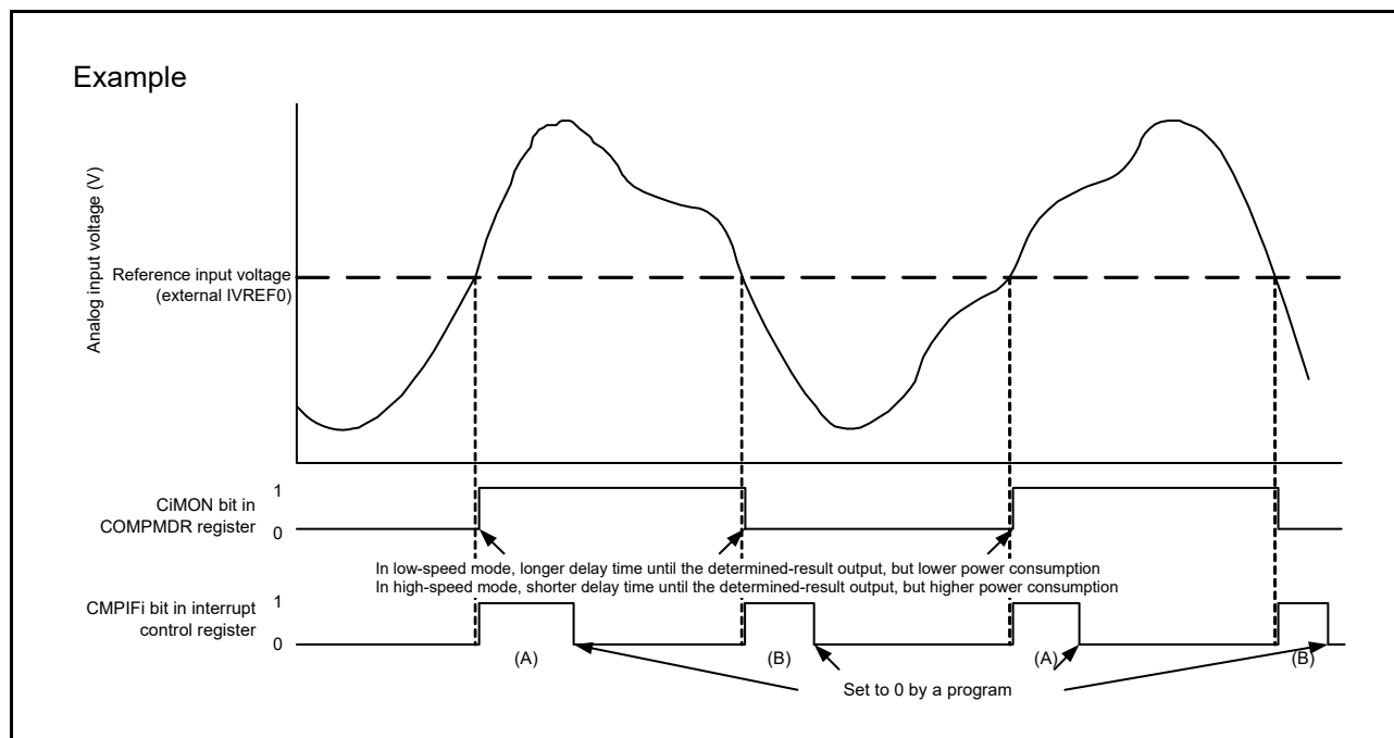
Figure 14 - 7 Comparator i ( i = 0, 1 ) Operation Example
