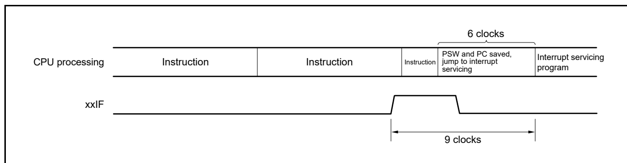
Figure 21 - 8 Interrupt Request Acknowledgment Timing (Minimum Time)
