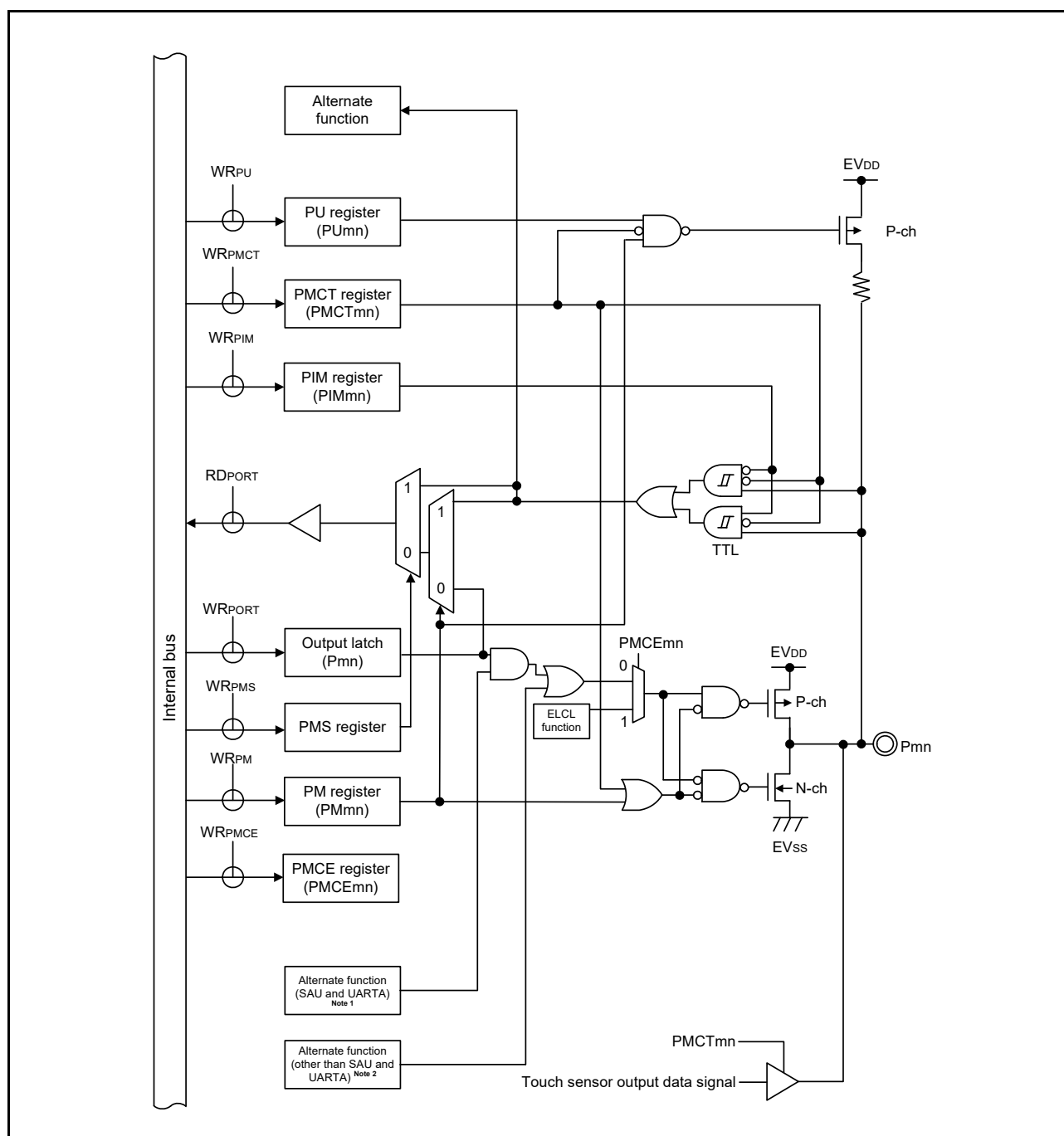
Figure 2 - 25 Pin Block Diagram for Pin Type 8-31-1
