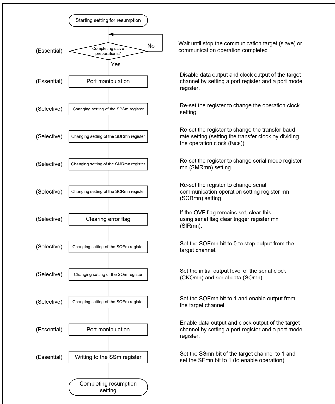
Figure 15 - 46 Procedure for Resuming Master Transmission/Reception
