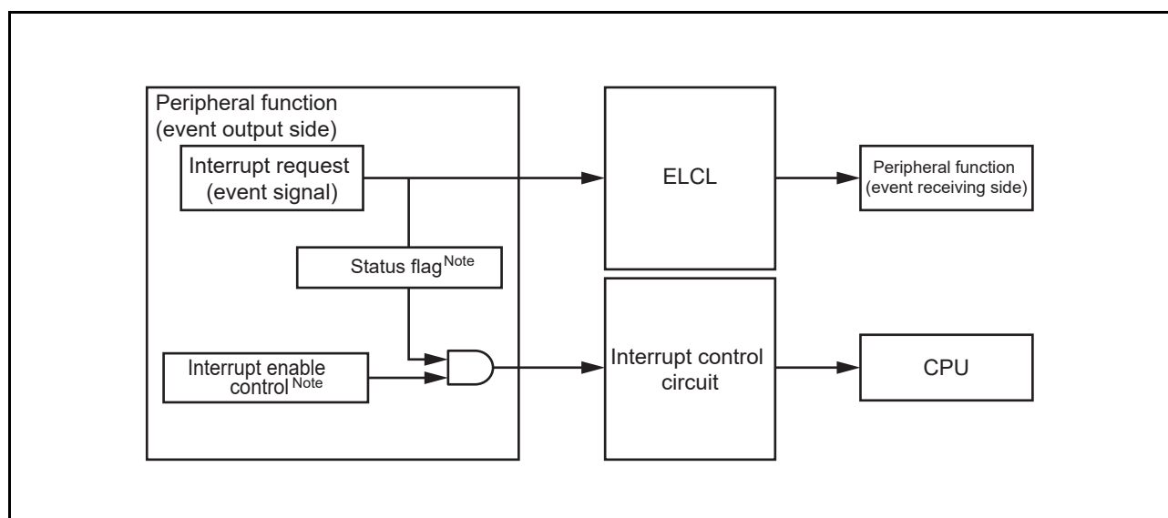
Figure 20 - 30 Relationship between Interrupt Service Routing and ELCL
