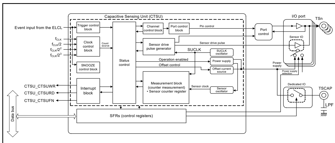
Figure 30 - 3 CTSU Block Diagram
