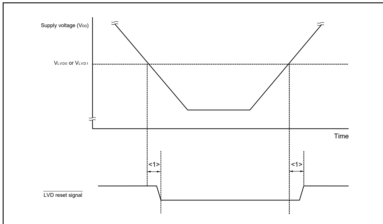
Figure 26 - 11 Delays from the Time an LVD0 or LVD1 Reset Source Condition is Satisfied until an LVD0 or LVD1 Reset has been Generated and Deasserted
