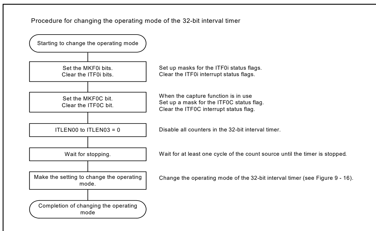
Figure 9 - 18 Procedure for Changing the Operating Mode of the 32-Bit Interval Timer
