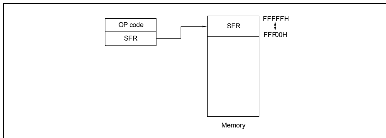
Figure 3 - 26 Outline of SFR Addressing
