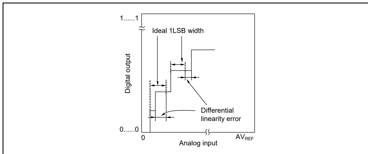
Figure 12 - 51 Differential Linearity Error
