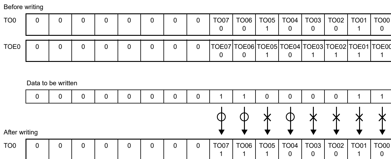
Figure 7 - 40 Example of TO0n Bit Collective Manipulation
