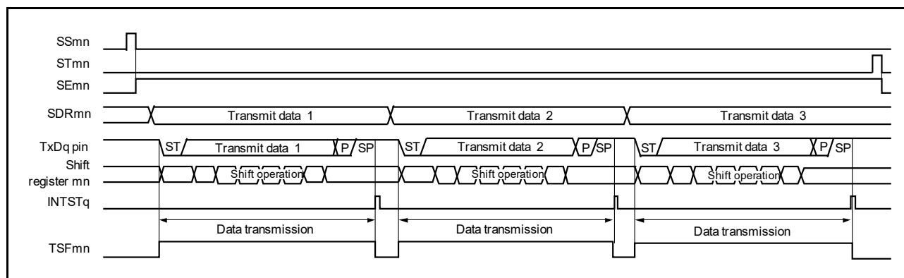
Figure 15 - 82 Timing Chart of UART Transmission (in Single-Transmission Mode)
