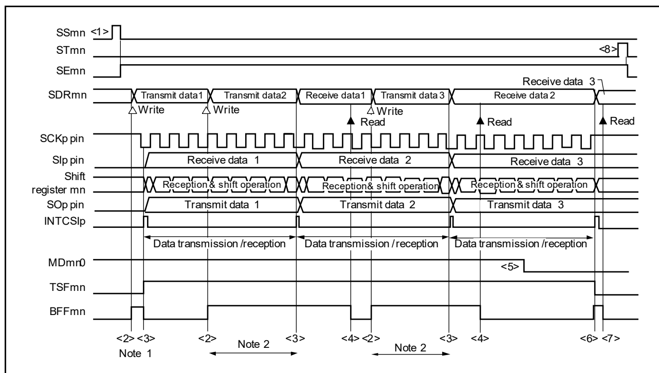
Figure 15 - 71 Timing Chart of Slave Transmission/Reception (in Continuous Transmission/Reception Mode) (Type 1: DAPmn = 0, CKPmn = 0)
