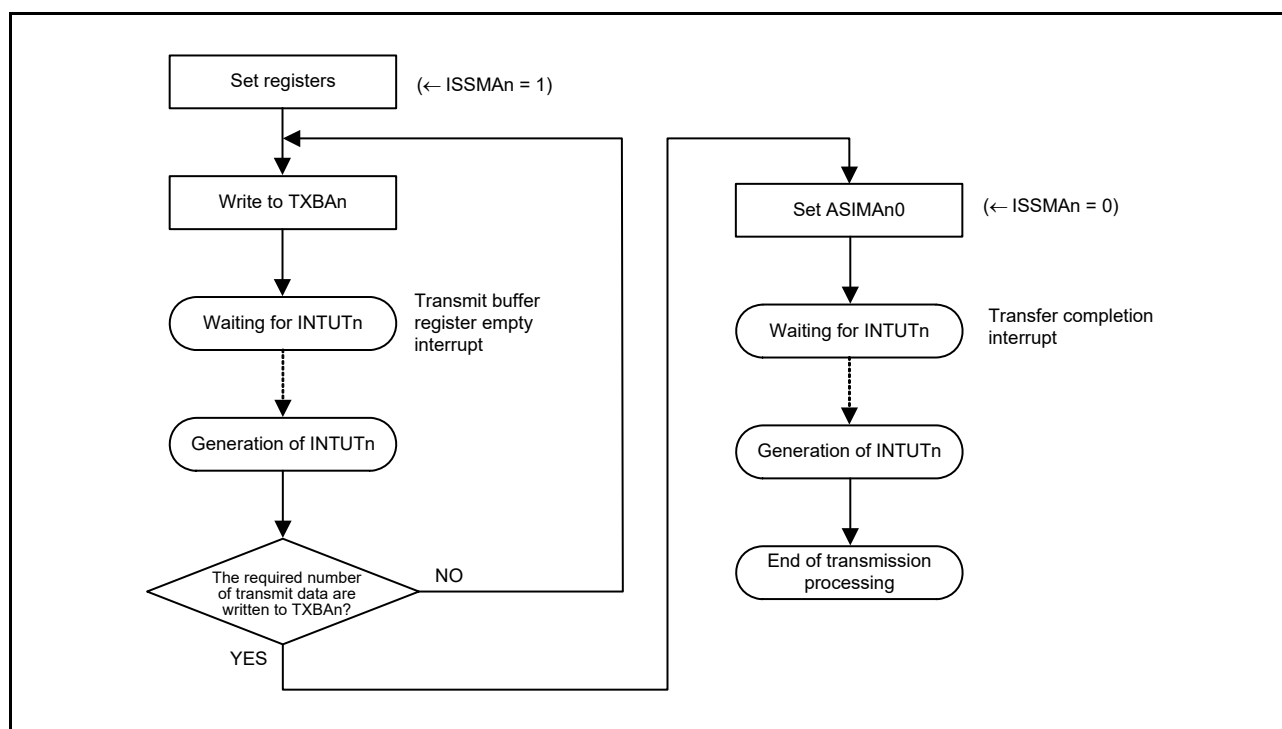
Figure 17 - 18 Flow Example of Continuous Transmission Using Interrupt
