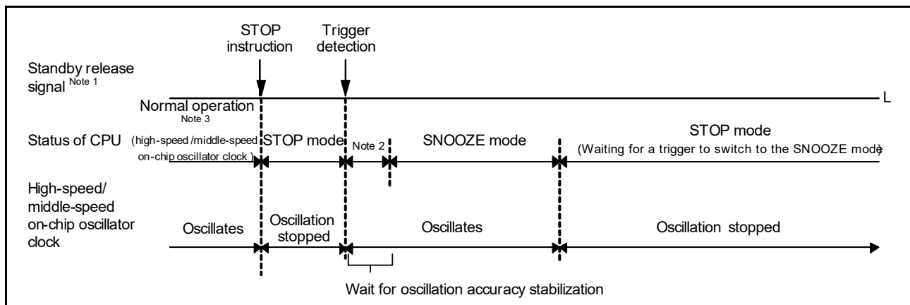
Figure 23 - 10 When the Interrupt Request Signal is not Generated in the SNOOZE Mode
