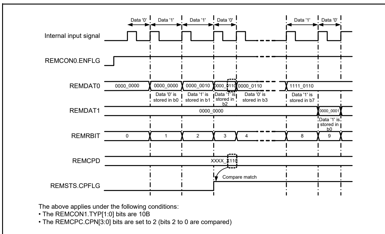
Figure 18 - 38 Receive Buffer and Compare Function
