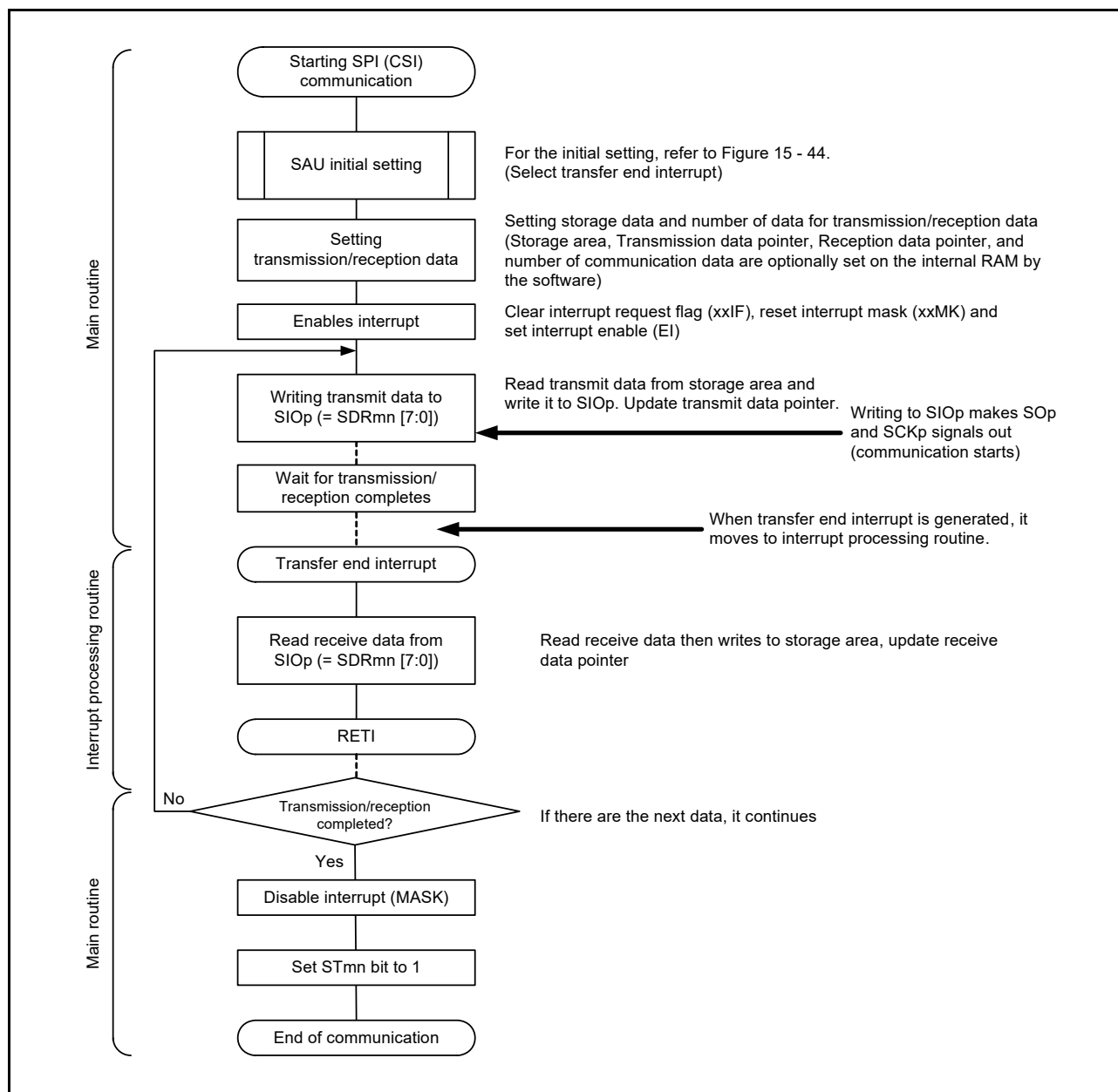
Figure 15 - 48 Flowchart of Master Transmission/Reception (in Single-Transmission/Reception Mode)
