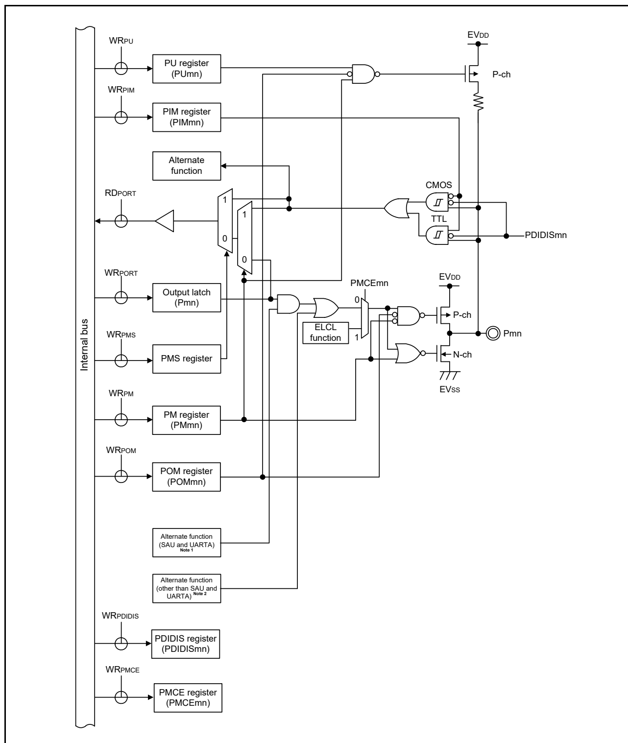
Figure 2 - 23 Pin Block Diagram for Pin Type 8-1-11
