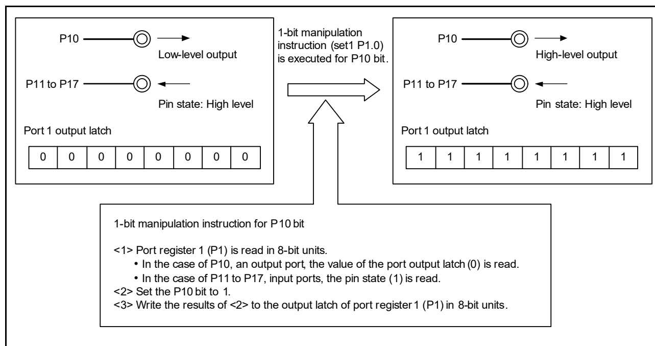
Figure 4 - 18 One-Bit Manipulation Instruction (P10)
