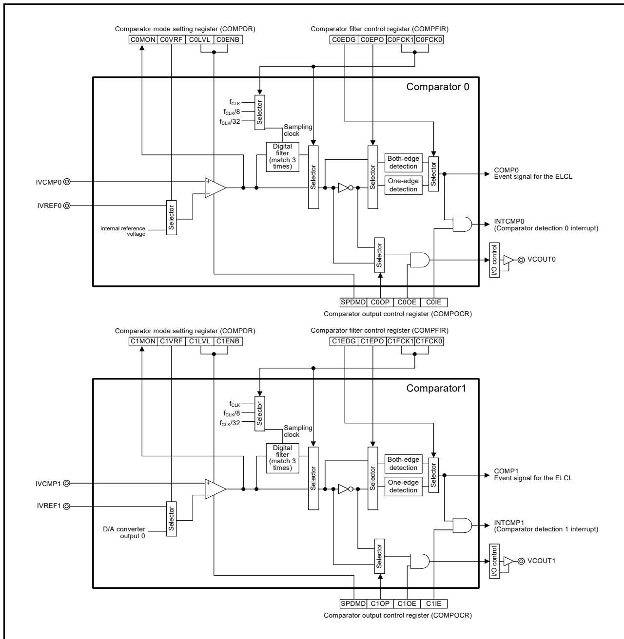
Figure 14 - 1 Comparator Block Diagram
