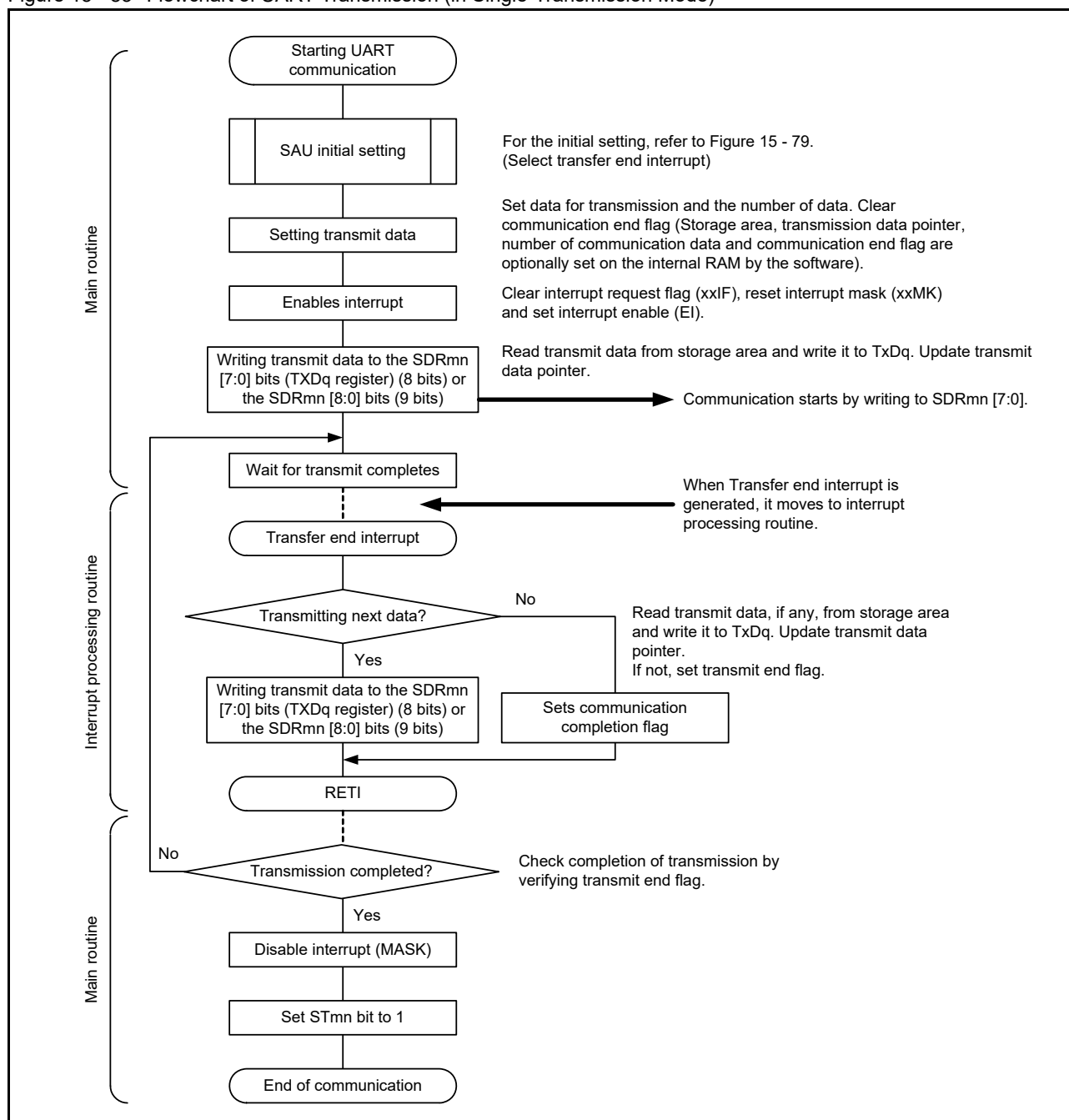
Figure 15 - 83 Flowchart of UART Transmission (in Single-Transmission Mode)
