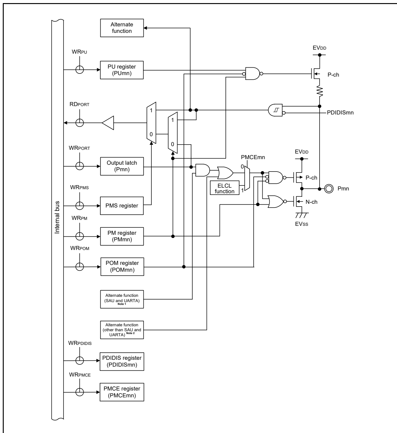
Figure 2 - 11 Pin Block Diagram for Pin Type 7-1-12
