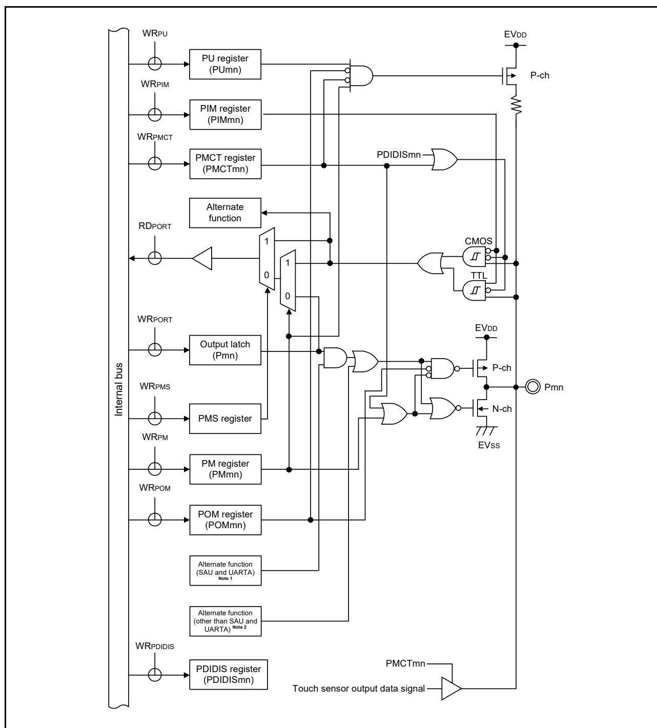
Figure 2 - 26 Pin Block Diagram for Pin Type 8-31-2
