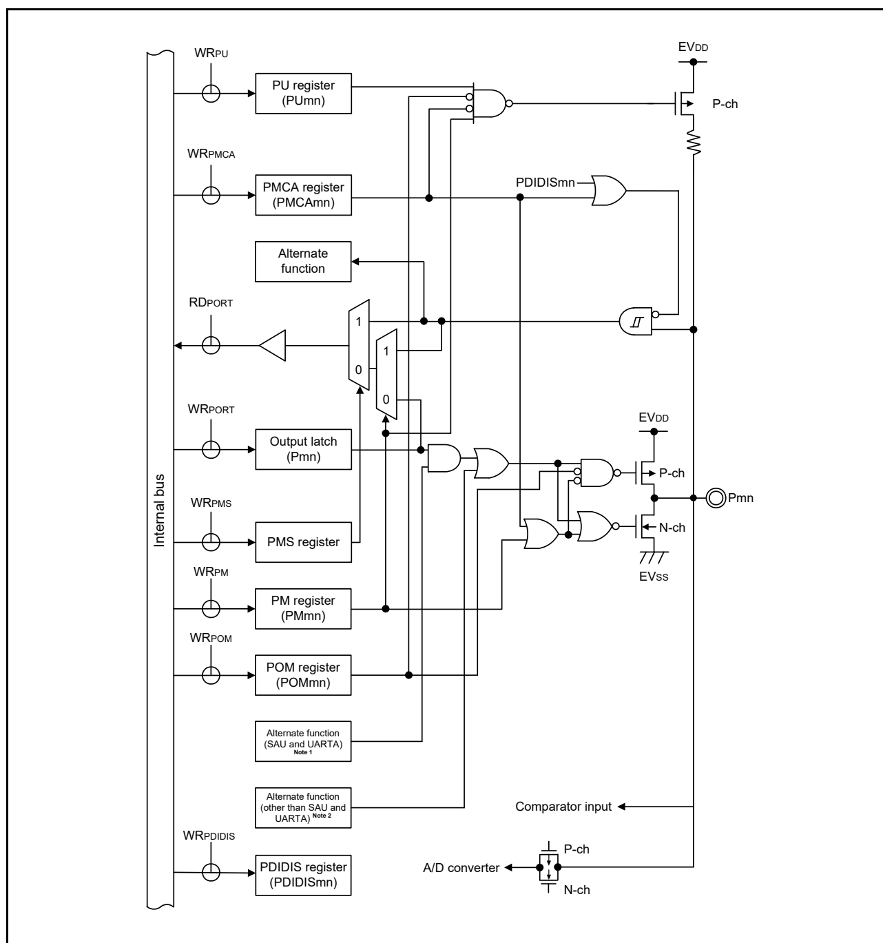
Figure 2 - 15 Pin Block Diagram for Pin Type 7-9-6
