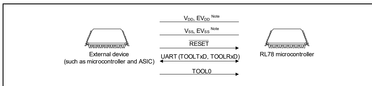
Figure 33 - 3 Environment for Writing Program to Flash Memory
