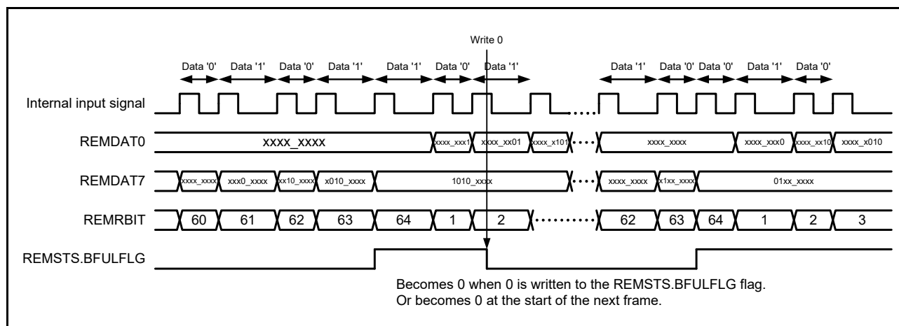
Figure 18 - 37 REMRBIT Register Operation (REMSTS.BFULFLG Flag = 1)
