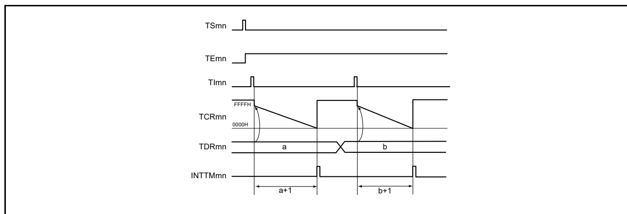
Figure 7 - 66 Example of Basic Timing during Operation as a Delay Counter
