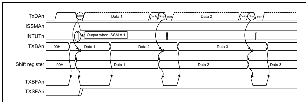
Figure 17 - 19 Timing Chart When Continuous Transmission Is Started
