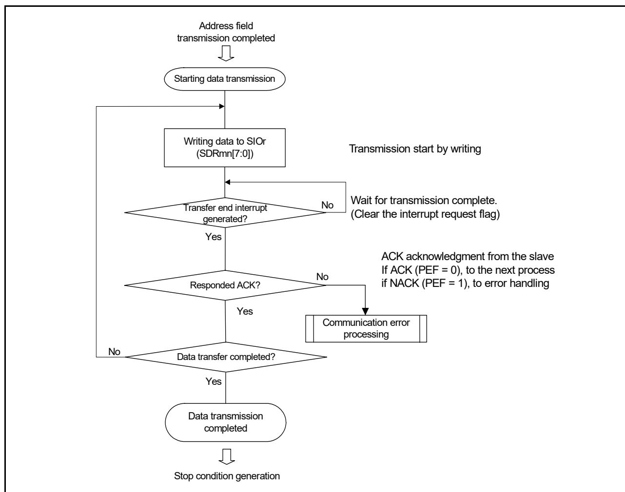
Figure 15 - 112 Flowchart of Simplified I 2 C Data Transmission
