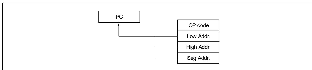
Figure 3 - 18 Example of CALL !addr16/BR !addr16
