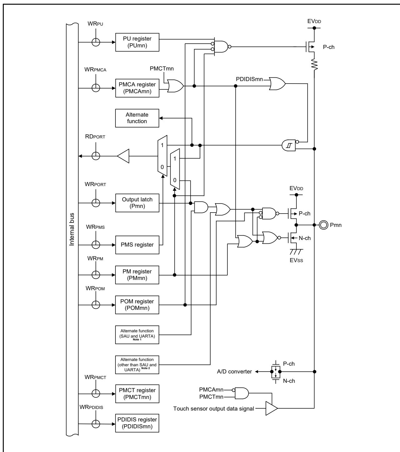
Figure 2 - 18 Pin Block Diagram for Pin Type 7-33-4
