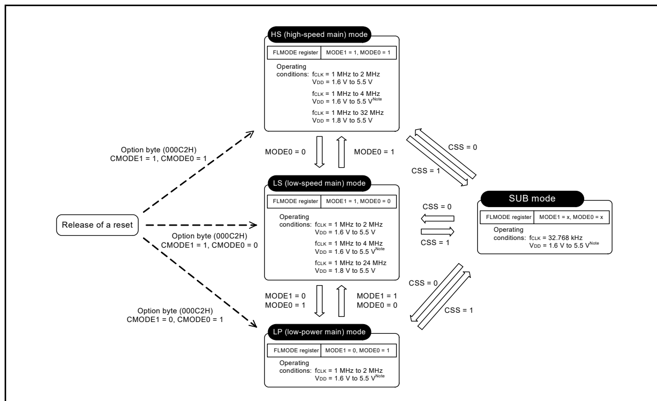
Figure 5 - 4 State Transitions between Flash Operation Modes
