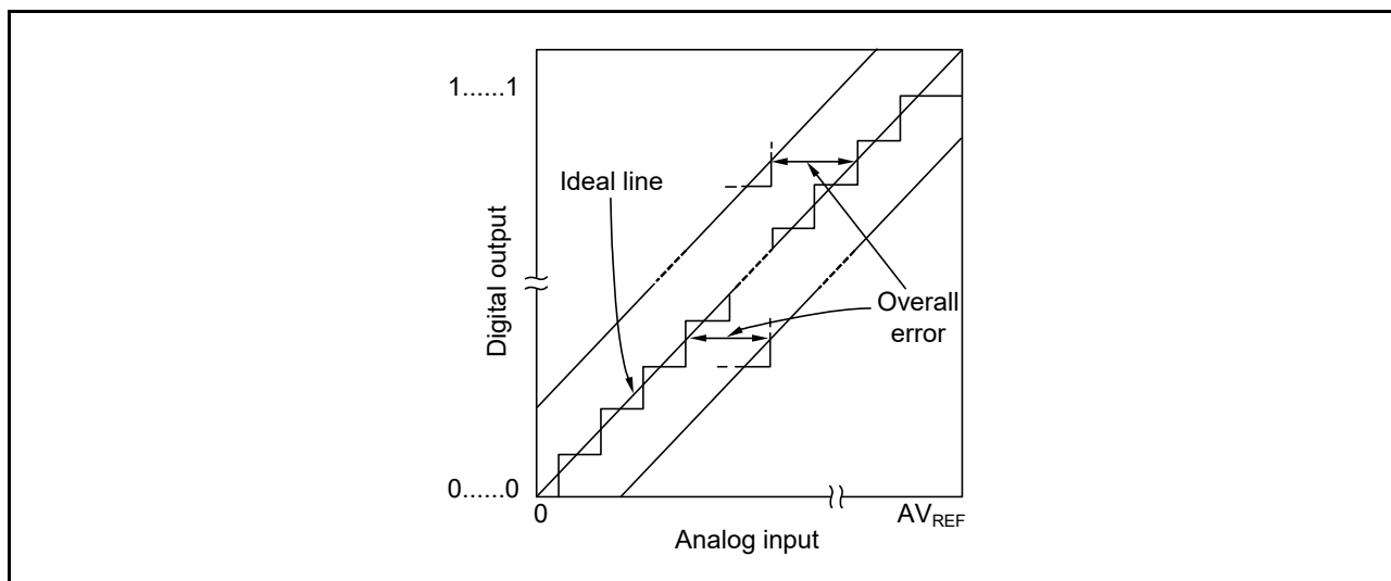
Figure 12 - 46 Overall Error
