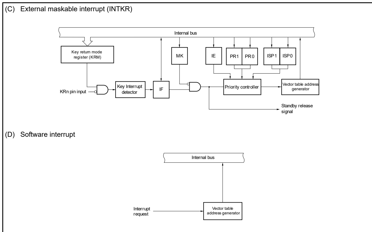
Figure 21 - 1 Basic Configuration of Interrupt Function (2/2)
