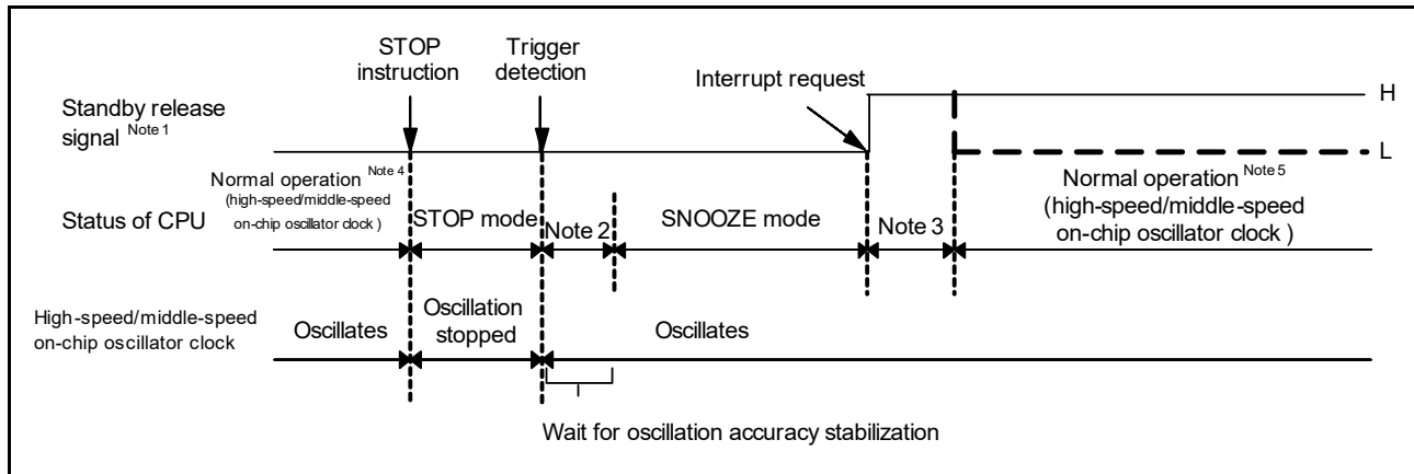
Figure 23 - 9 When the Interrupt Request Signal is Generated in the SNOOZE Mode
