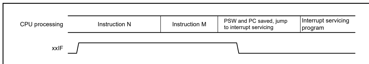
Figure 21 - 11 Holding Interrupt Requests Pending
