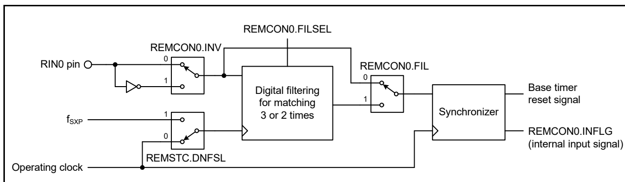
Figure 18 - 28 RIN0 Internal Input Signal Generation Configuration
