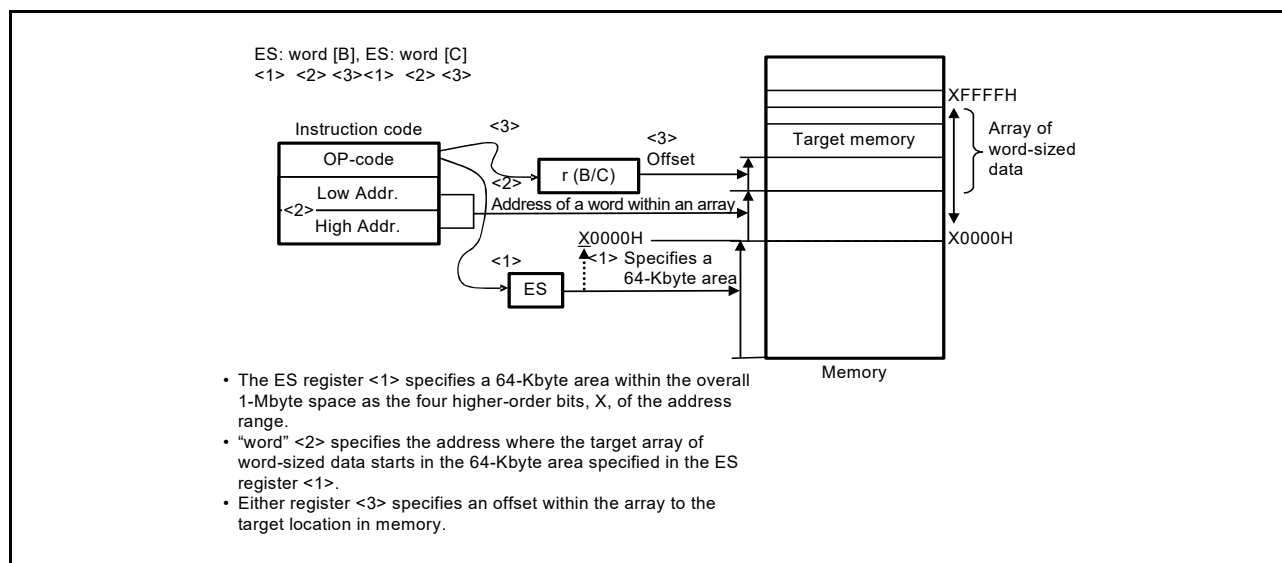
Figure 3 - 34 Example of ES:word [B], ES:word [C]
