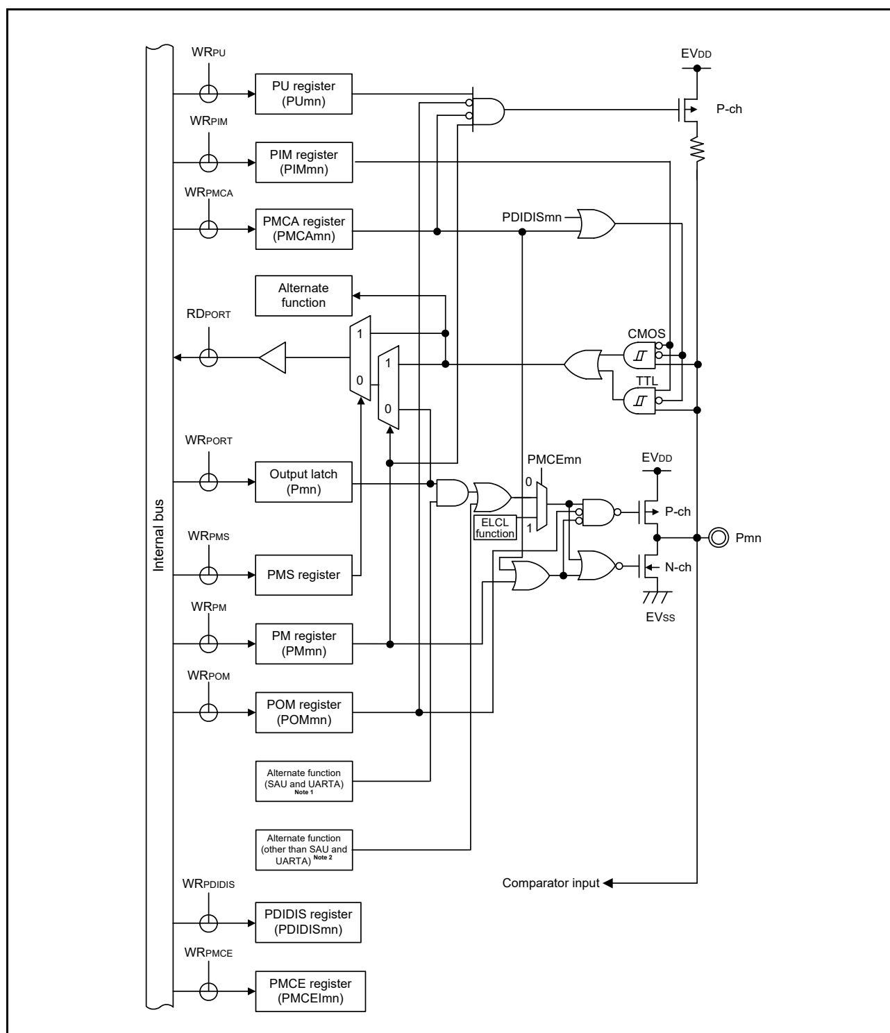
Figure 2 - 24 Pin Block Diagram for Pin Type 8-6-9
