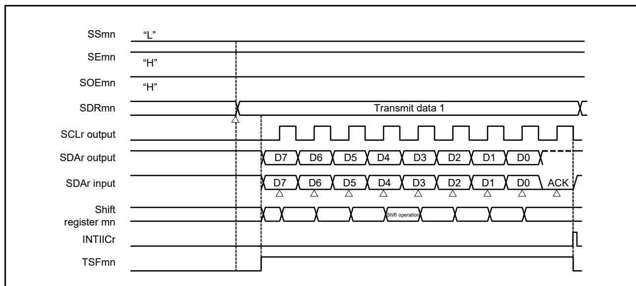
Figure 15 - 111 Timing Chart of Data Transmission
