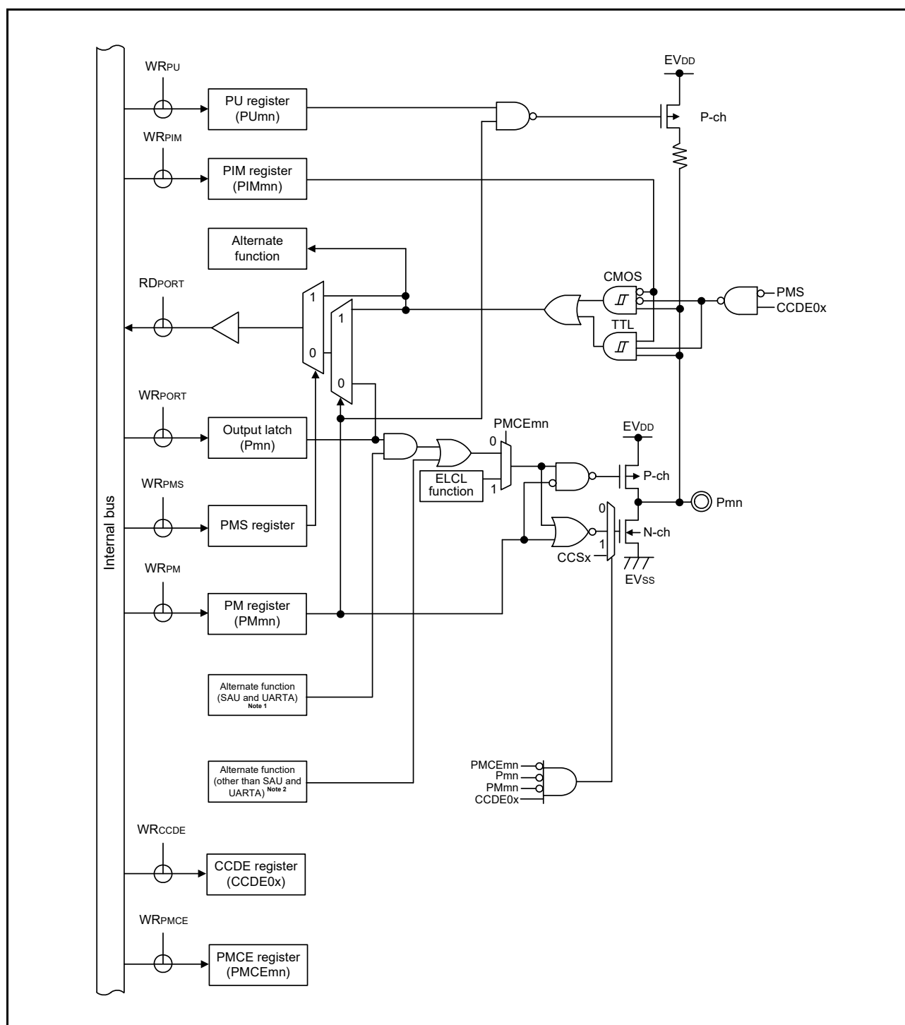
Figure 2 - 29 Pin Block Diagram for Pin Type 8-38-1
