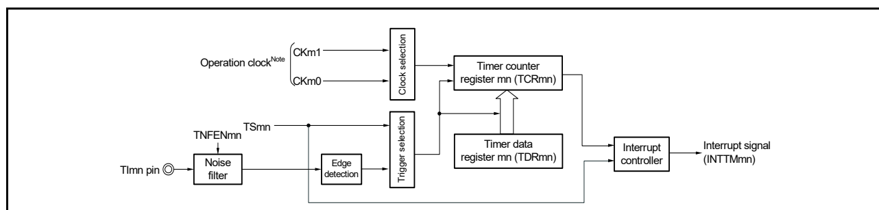
Figure 7 - 65 Block Diagram for Operation as a Delay Counter
