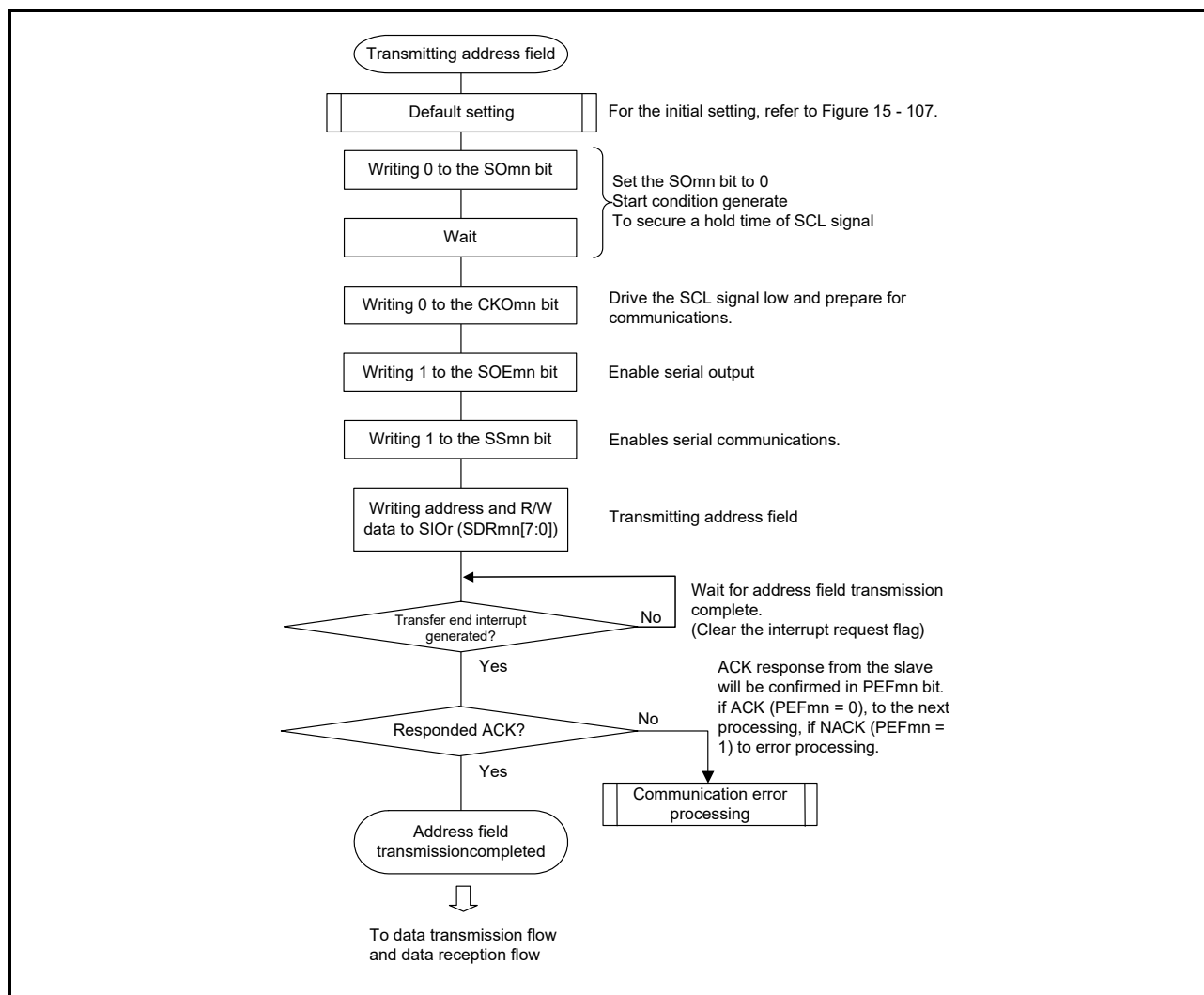
Figure 15 - 109 Flowchart of Simplified I 2 C Address Field Transmission
