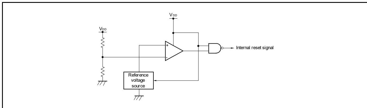
Figure 25 - 1 Block Diagram of Power-on-reset Circuit
