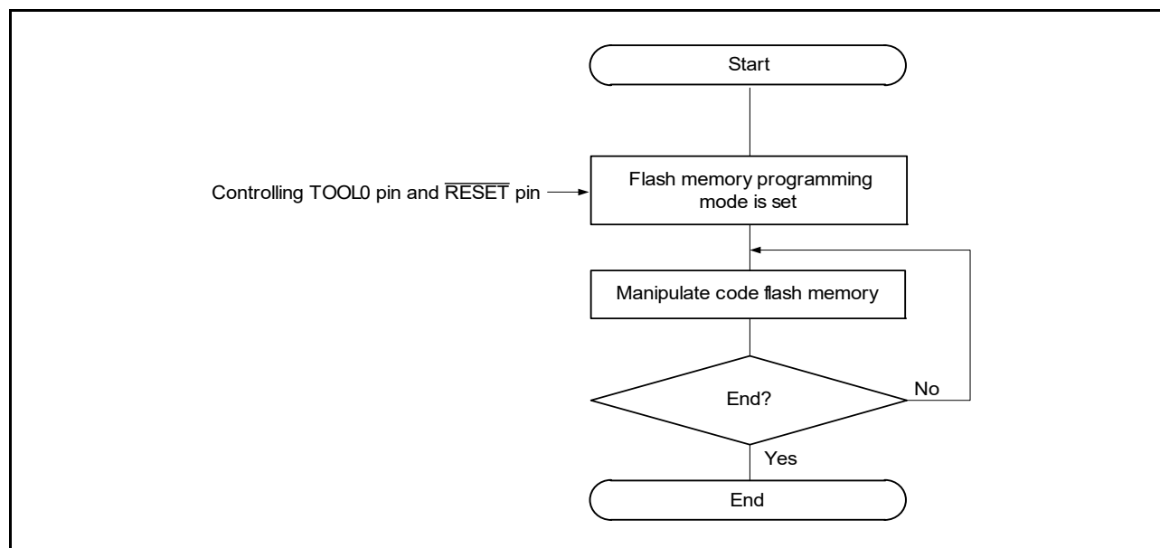
Figure 33 - 6 Code Flash Memory Manipulation Procedure
