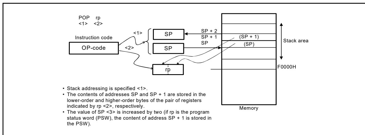
Figure 3 - 39 Example of POP
