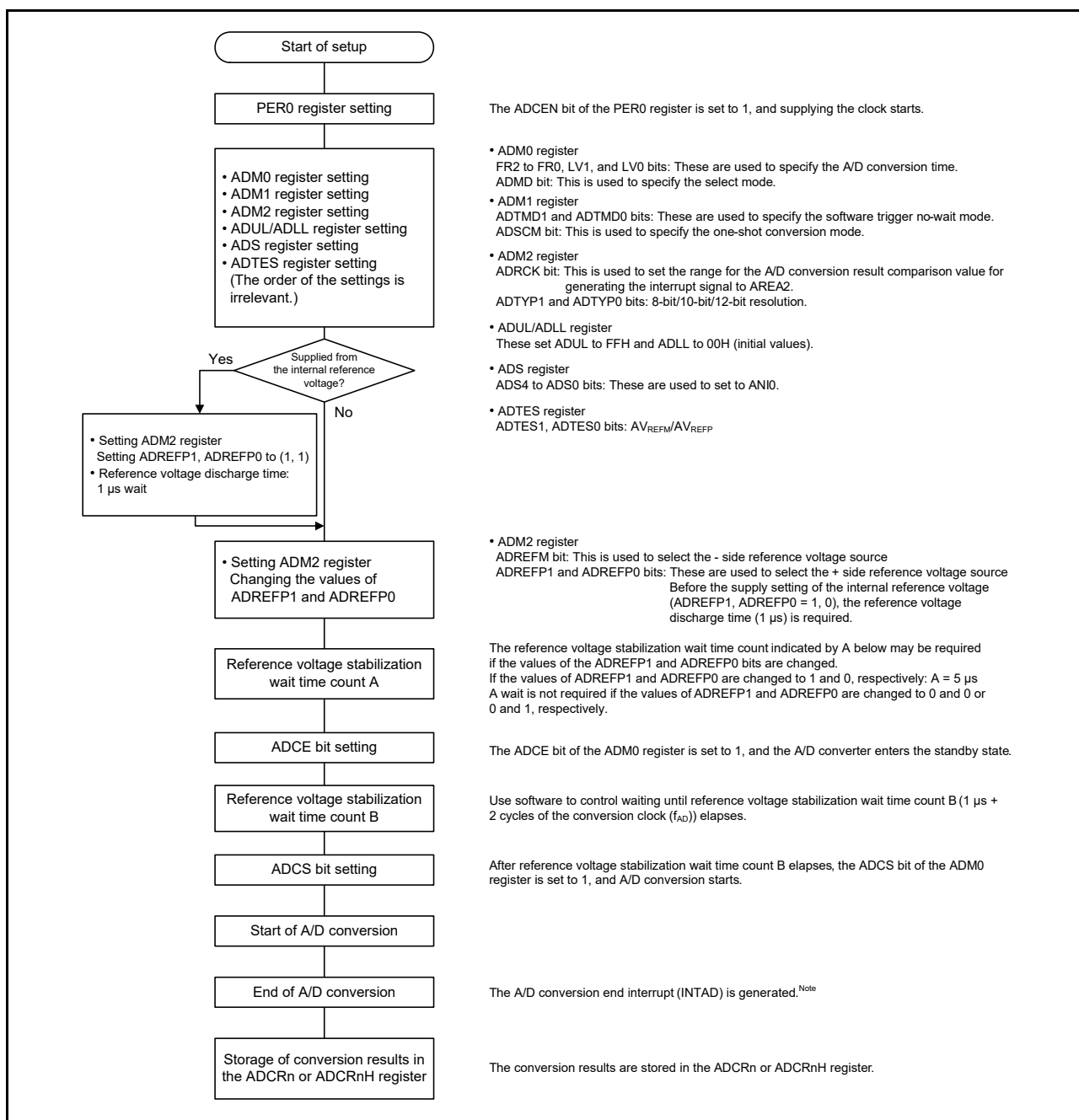
Figure 12 - 39 Setting up Test Mode
