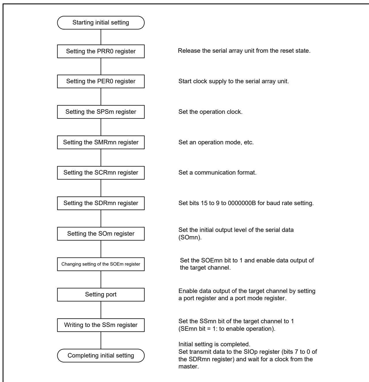
Figure 15 - 52 Initial Setting Procedure for Slave Transmission
