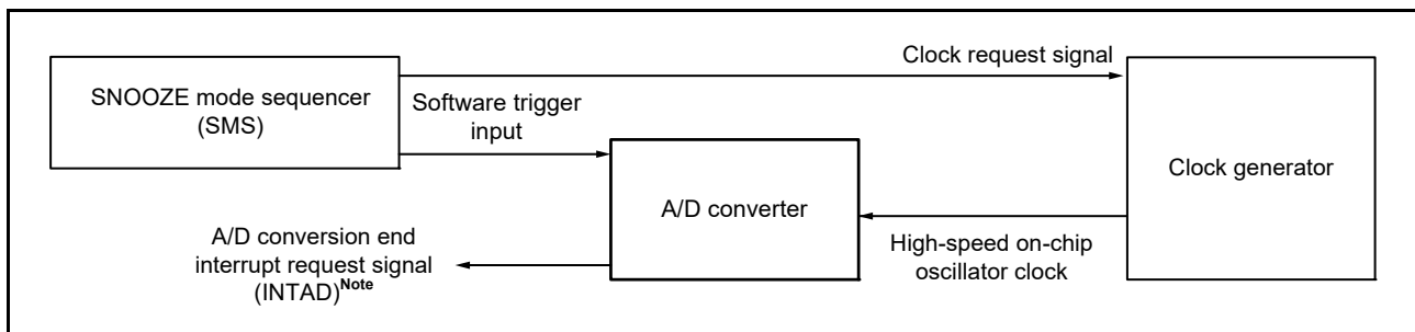
Figure 12 - 40 Block Diagram When Using SNOOZE Mode Function (in Software Trigger Wait Mode)
