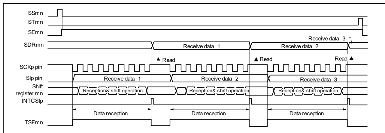
Figure 15 - 63 Timing Chart of Slave Reception (in Single-Reception Mode) (Type 1: DAPmn = 0, CKPmn = 0)
