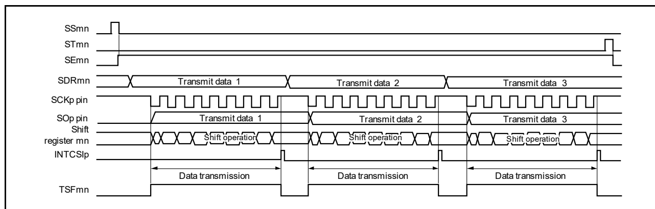
Figure 15 - 55 Timing Chart of Slave Transmission (in Single-Transmission Mode) (Type 1: DAPmn = 0, CKPmn = 0)
