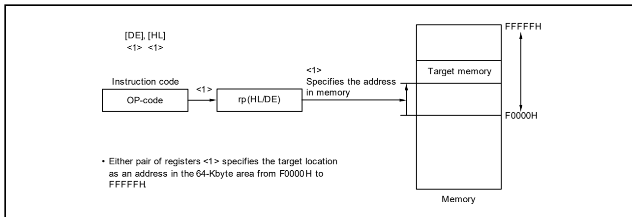
Figure 3 - 27 Example of [DE], [HL]
