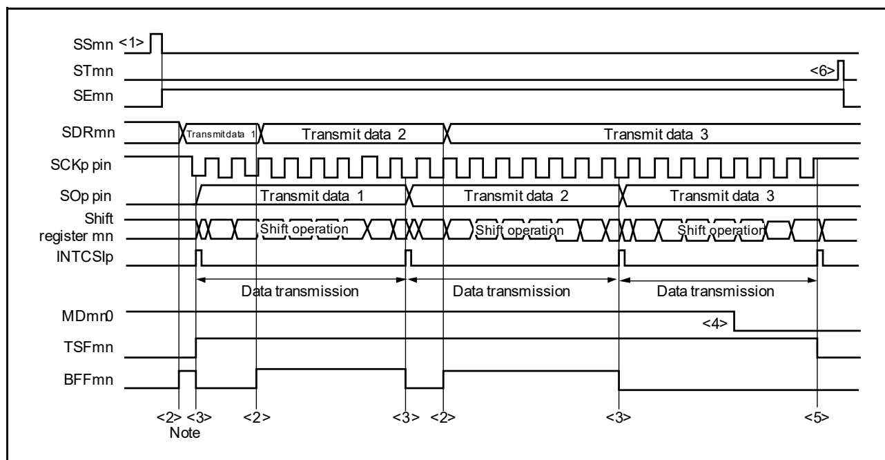
Figure 15 - 57 Timing Chart of Slave Transmission (in Continuous Transmission Mode) (Type 1: DAPmn = 0, CKPmn = 0)
