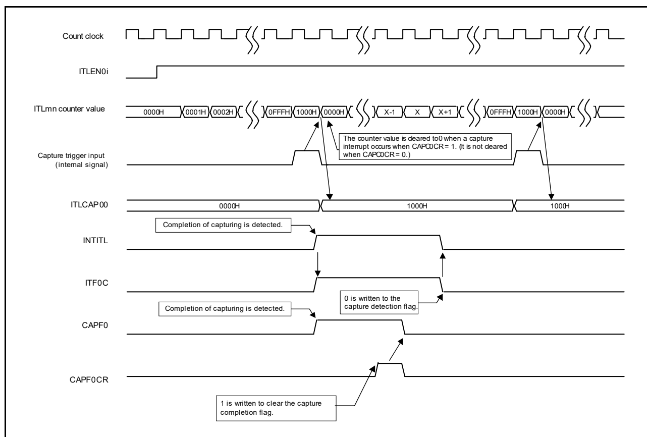
Figure 9 - 15 Example of Capture Operation
