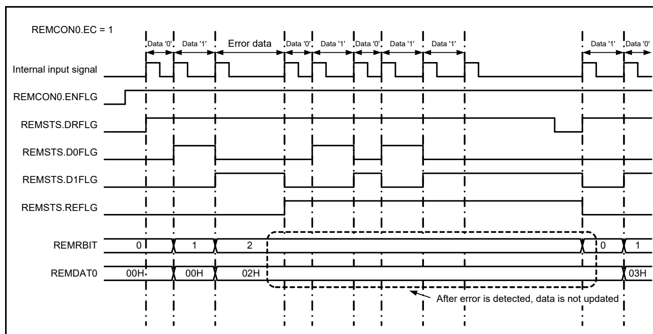
Figure 18 - 40 REMDAT0 and REMRBIT Registers Operation upon Error Detection (REMCON0.EC Bit = 1)
