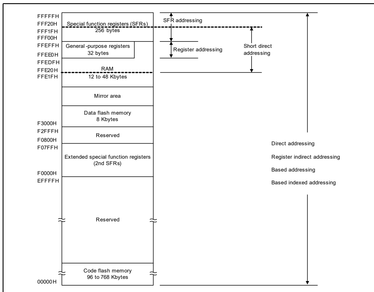
Figure 3 - 9 Correspondence Between Data Memory and Addressing
