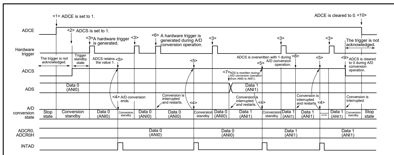
Figure 12 - 27 Example of Hardware Trigger No-Wait Mode (Select Mode, One-Shot Conversion Mode) Operation Timing
