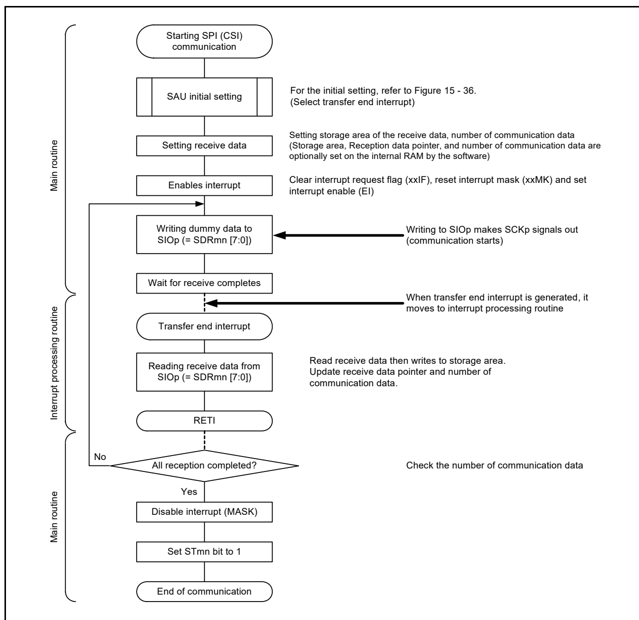
Figure 15 - 40 Flowchart of Master Reception (in Single-Reception Mode)
