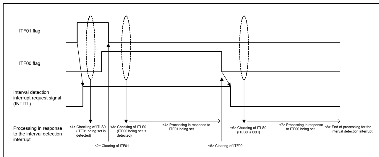
Figure 9 - 22 Example of Clearing the Detection Flags
