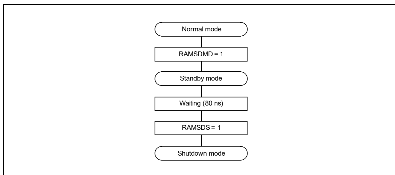
Figure 23 - 3 Procedure for Settings to Switch from Normal Mode to Shutdown Mode
