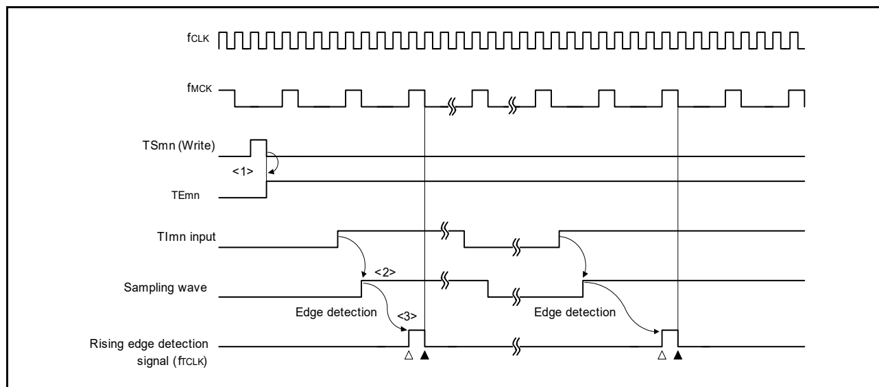
Figure 7 - 28 Timing of fCLK and Count Clock (fTCLK) (When CCSmn = 1, Noise Filter Unused)
