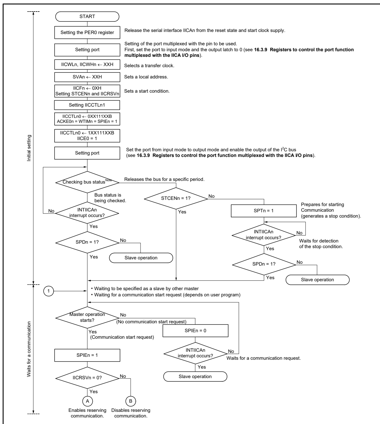
Figure 16 - 29 Master Operation in Multi-Master System (1/3)
