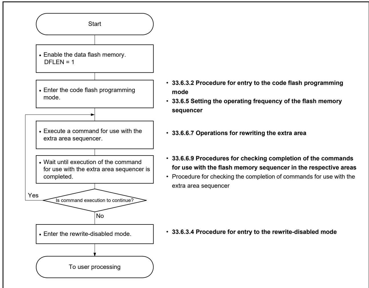
Figure 33 - 32 Flow of Executing the Commands to Rewrite the Extra Area
