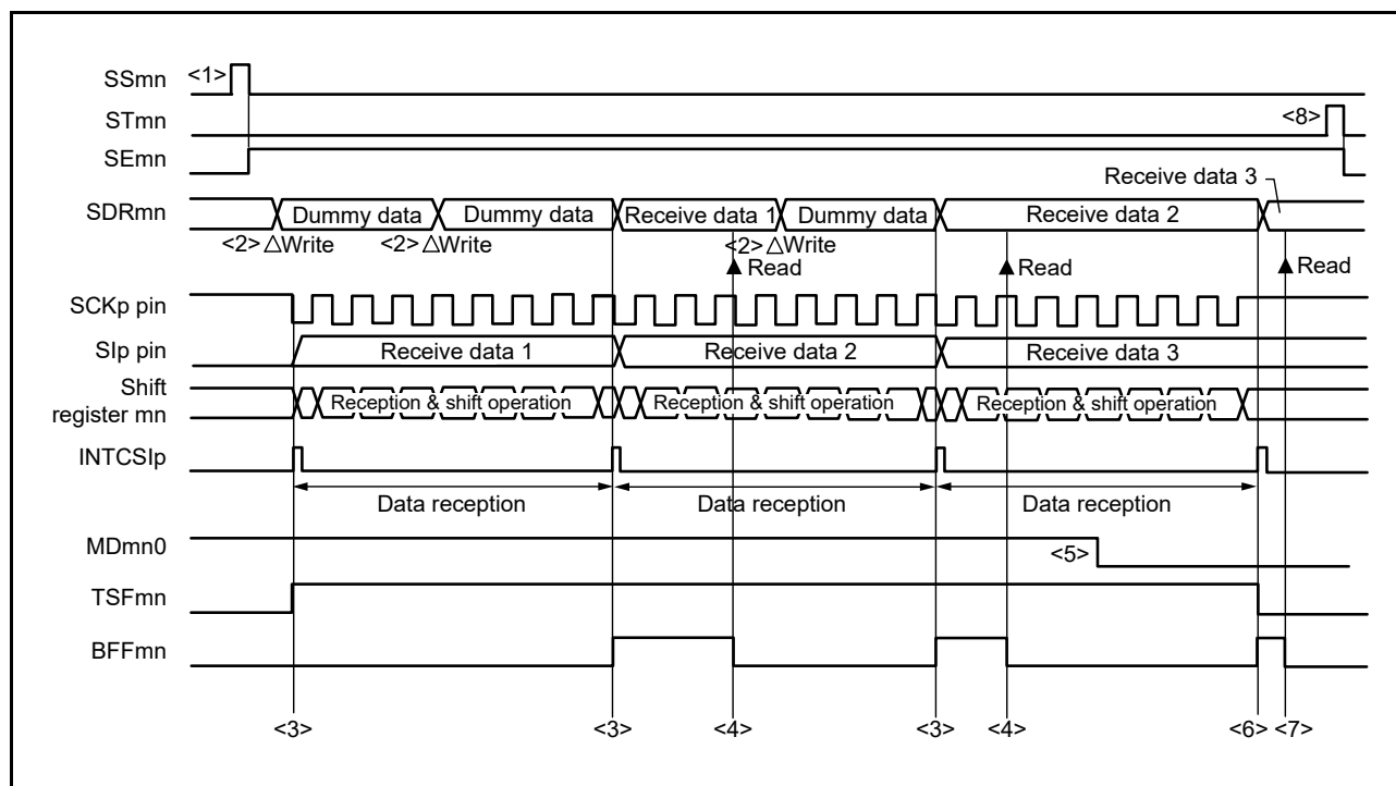
Figure 15 - 41 Timing Chart of Master Reception (in Continuous Reception Mode) (Type 1: DAPmn = 0, CKPmn = 0)
