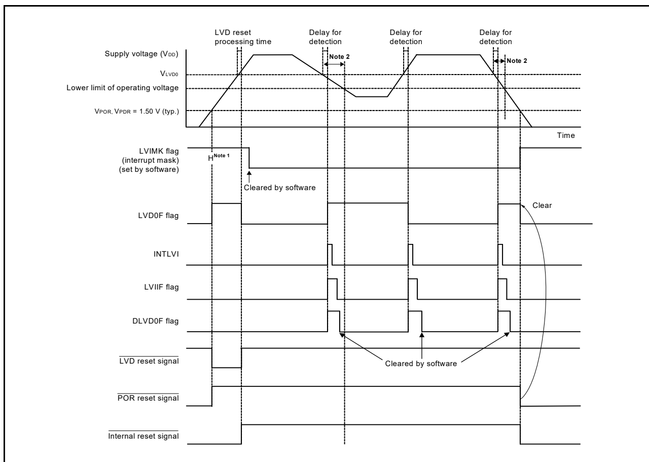
&lt;R&gt; Figure 26 - 8 Timing of LVD0 Interrupt Signal Generation
