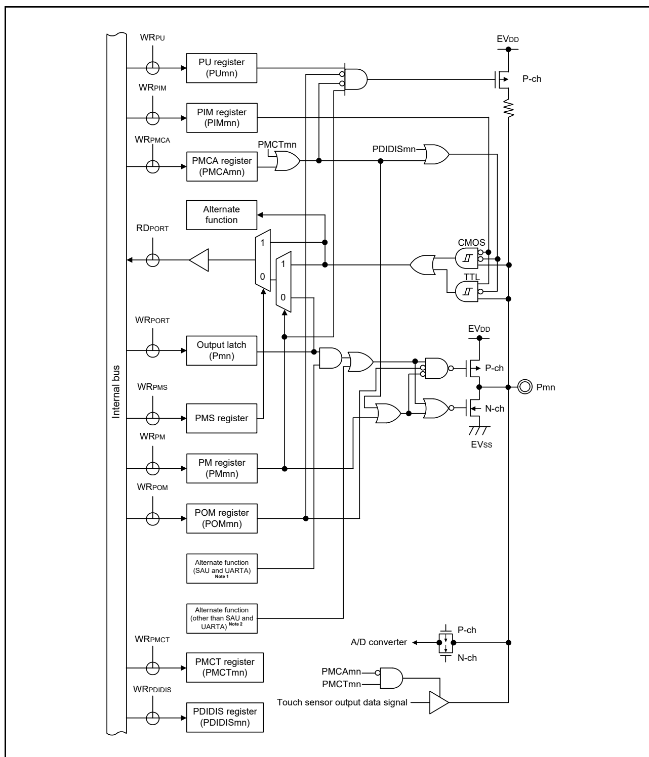
Figure 2 - 28 Pin Block Diagram for Pin Type 8-33-3
