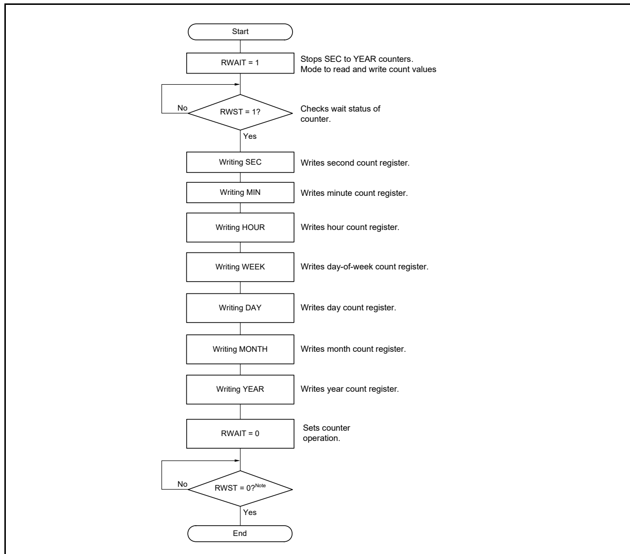
Figure 8 - 22 Procedure for Writing Realtime Clock
