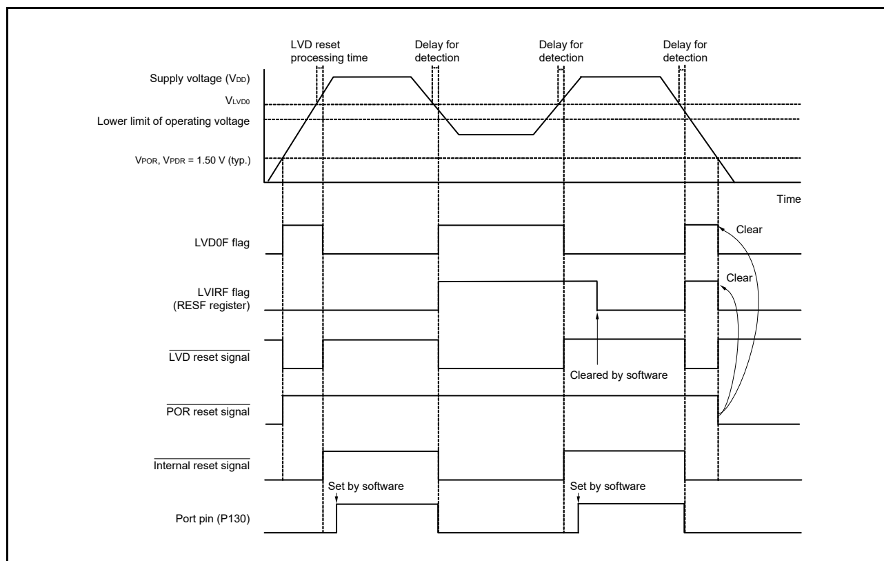
&lt;R&gt; Figure 26 - 6 Timing of LVD0 Internal Reset Signal Generation
