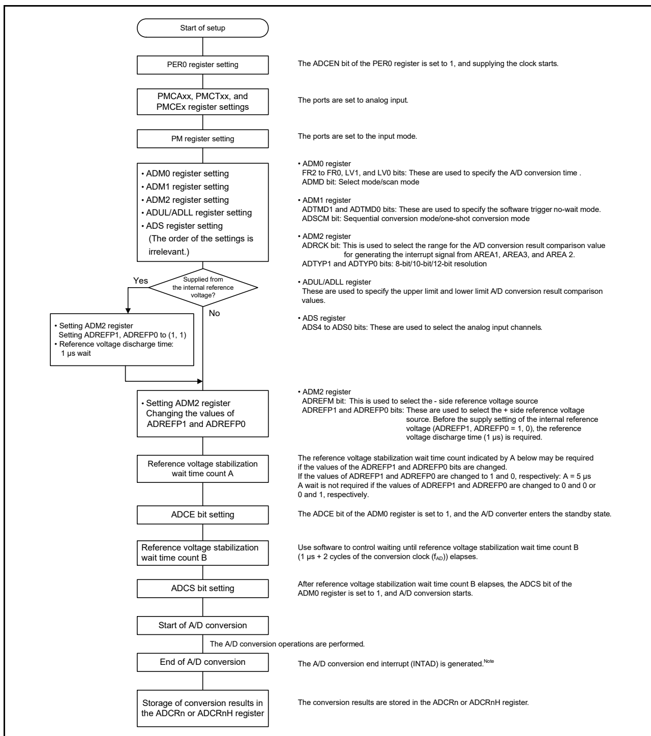
Figure 12 - 34 Setting up Software Trigger No-Wait Mode
