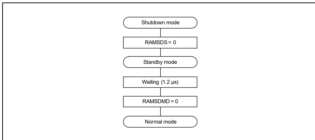
Figure 23 - 4 Procedure for Settings to Switch from Shutdown Mode to Normal Mode
