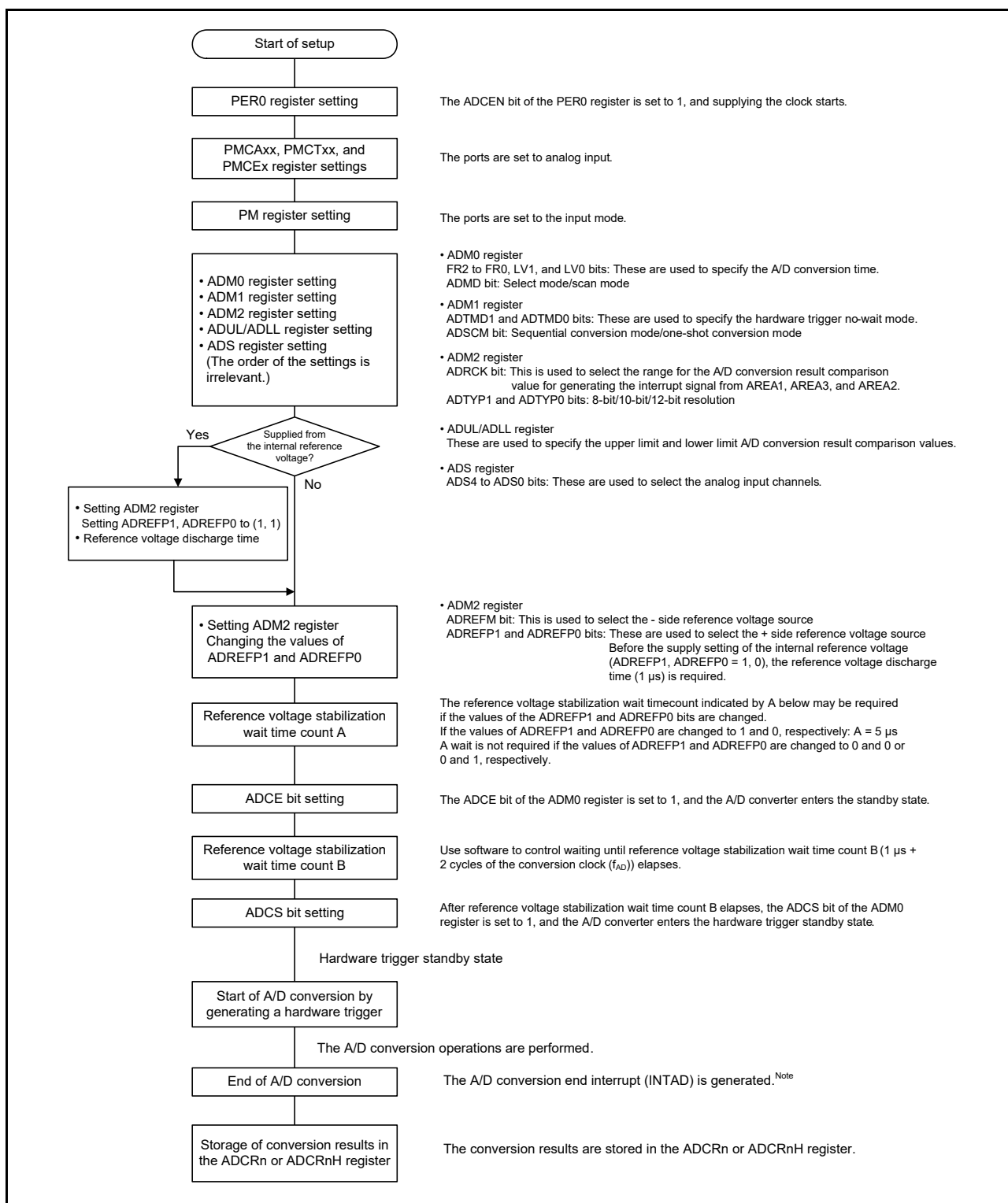
Figure 12 - 36 Setting up Hardware Trigger No-Wait Mode
