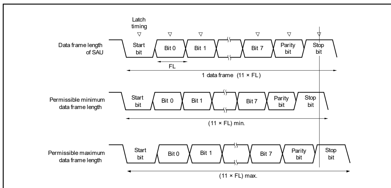
Figure 15 - 97 Permissible Baud Rate Range for Reception (1 Data Frame Length = 11 Bits)
