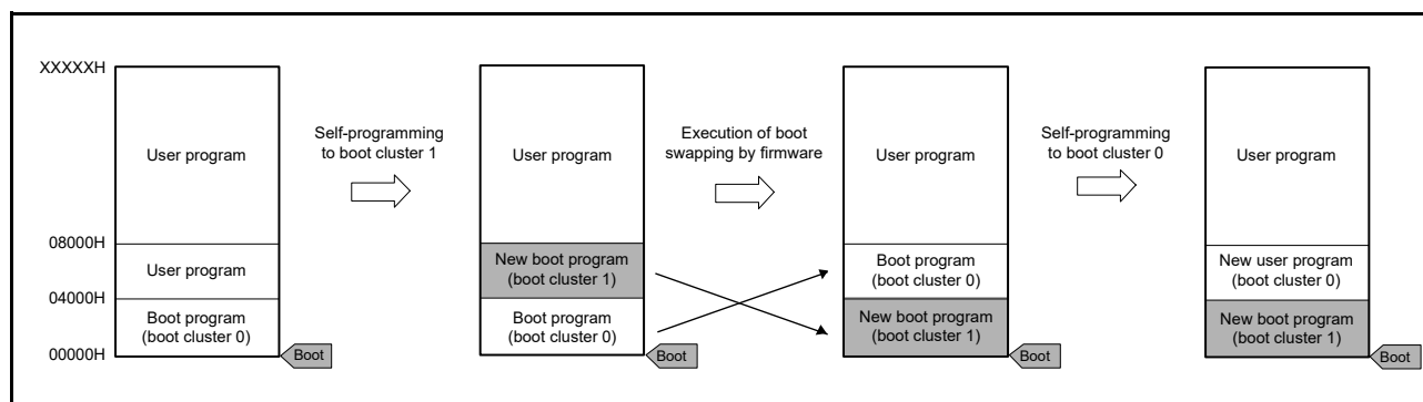
Figure 33 - 27 Boot Swap Function
