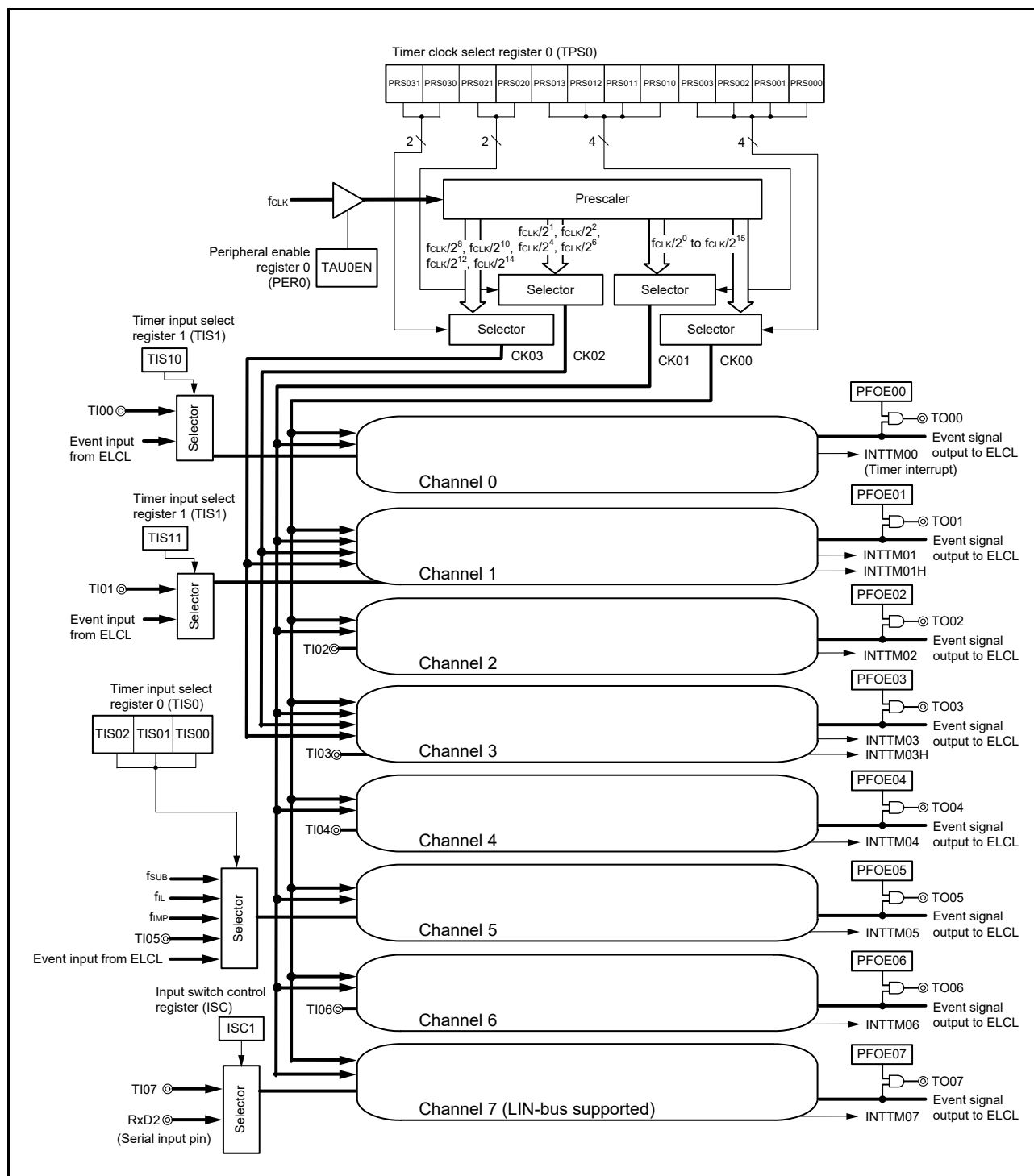
Figure 7 - 1 Entire Configuration of Timer Array Unit 0 (Example: 64-Pin Products)
