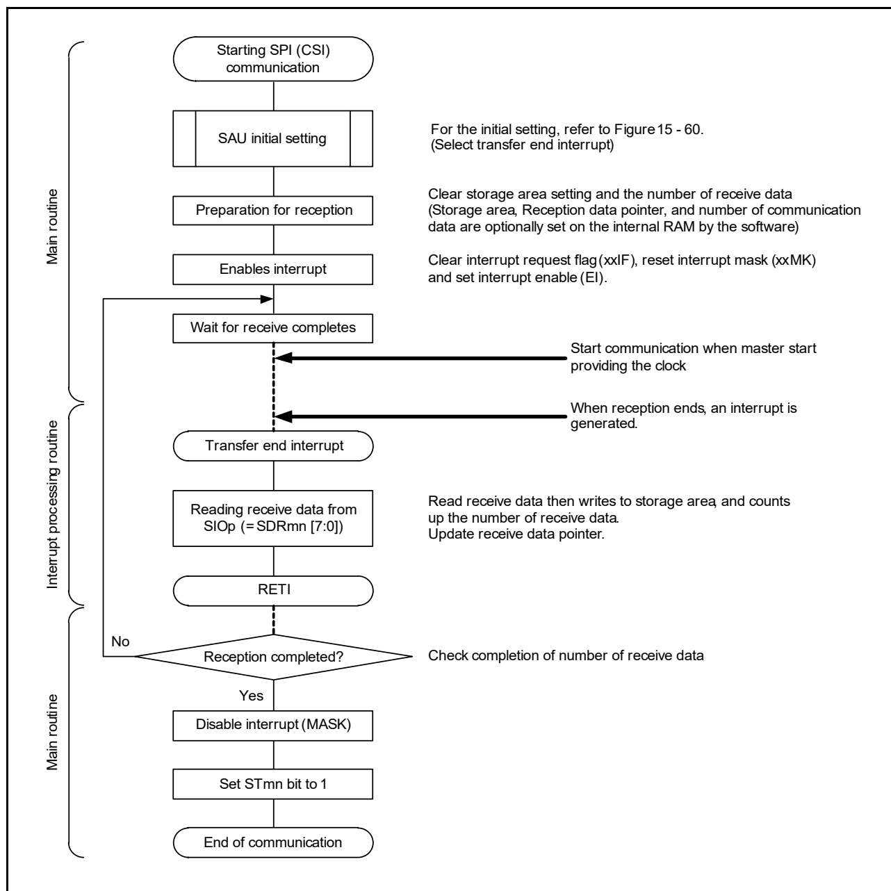
Figure 15 - 64 Flowchart of Slave Reception (in Single-Reception Mode)
