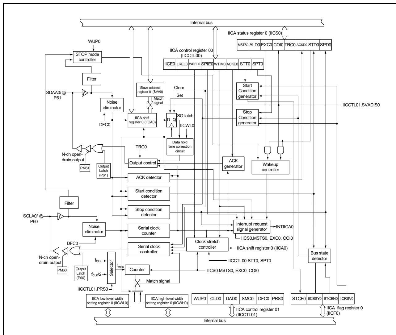
Figure 16 - 1 Block Diagram of Serial Interface IICA0
