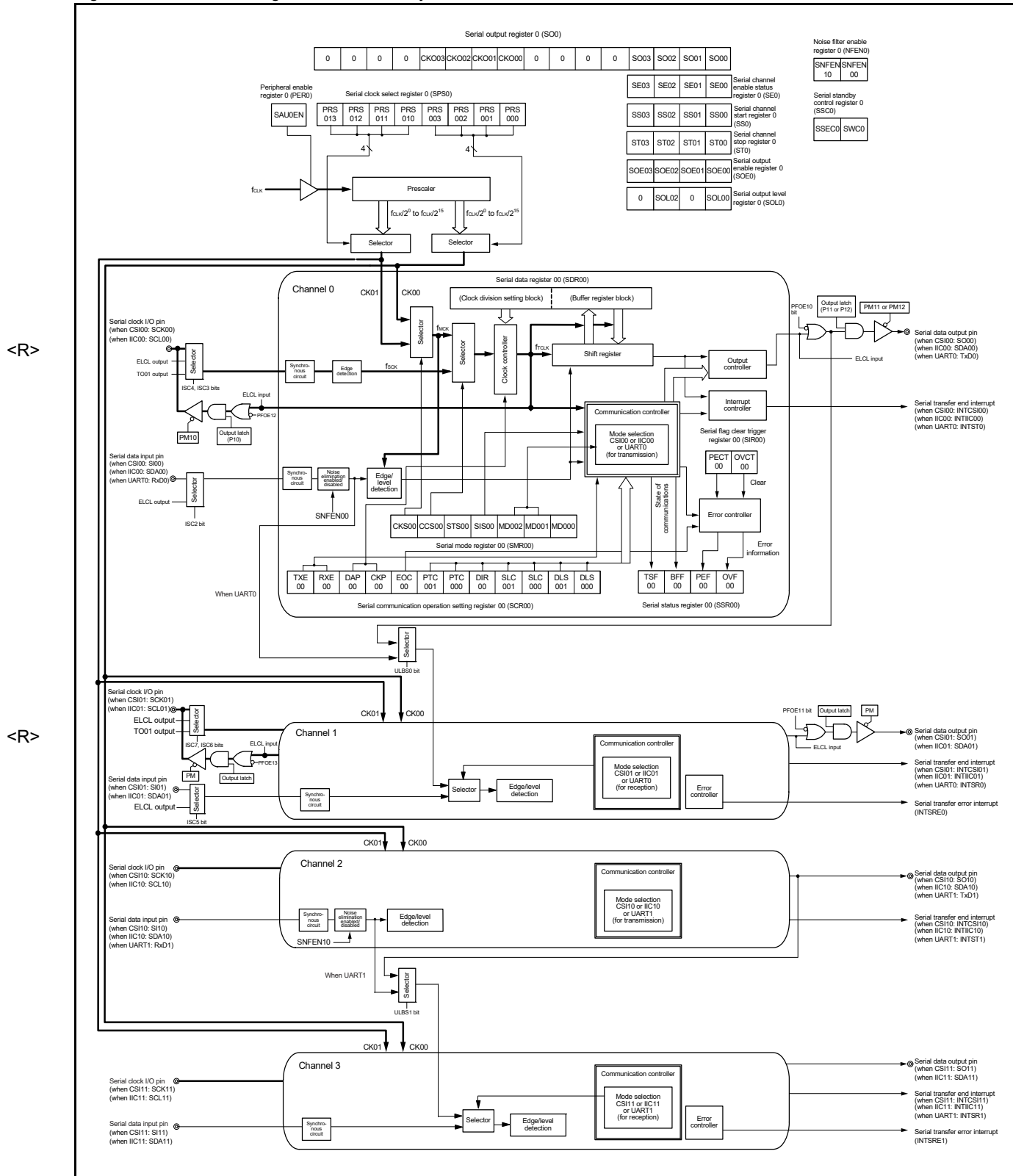
Figure 15 - 1 Block Diagram of Serial Array Unit 0
