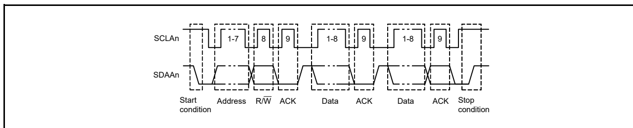
Figure 16 - 14 I 2 C Bus Serial Data Transfer Timing
