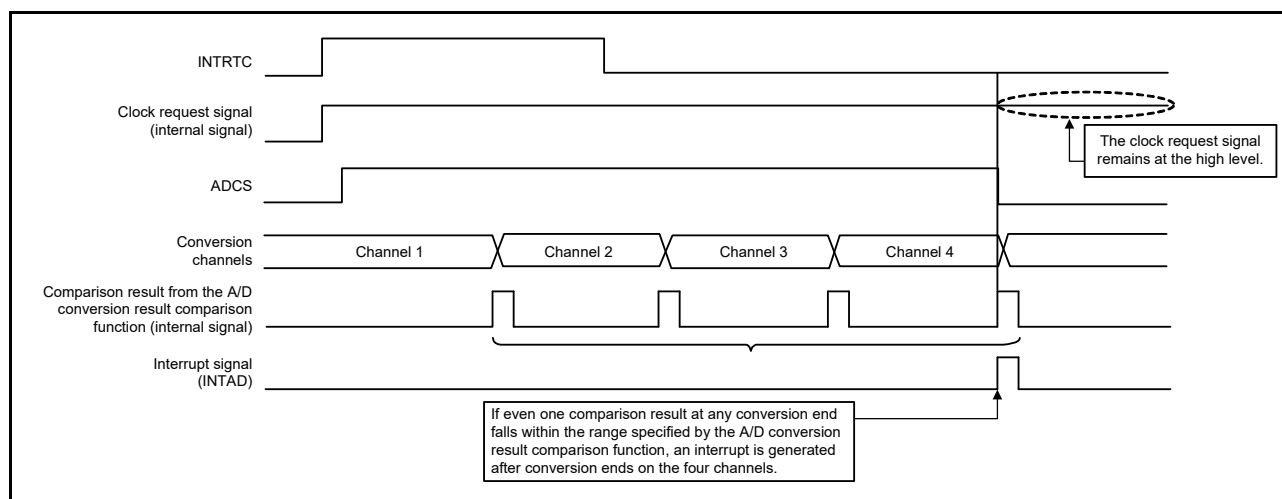
Figure 12 - 43 Operation Example When Interrupt Is Generated After A/D Conversion Ends (While in Scan Mode)
