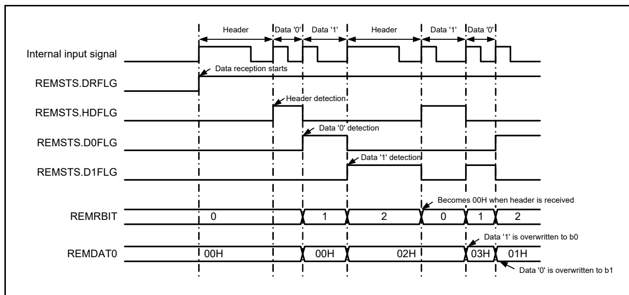
Figure 18 - 36 Operation of Header Pattern Detection during Data Reception
