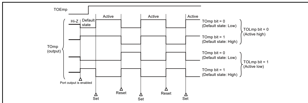
Figure 7 - 37 TOmp Pin Output States with PWM Output (TOMmp = 1)
