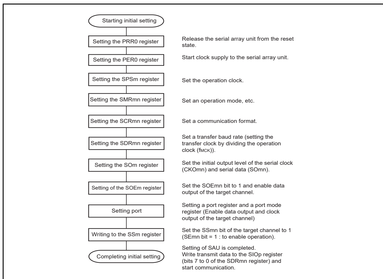
Figure 15 - 28 Initial Setting Procedure for Master Transmission
