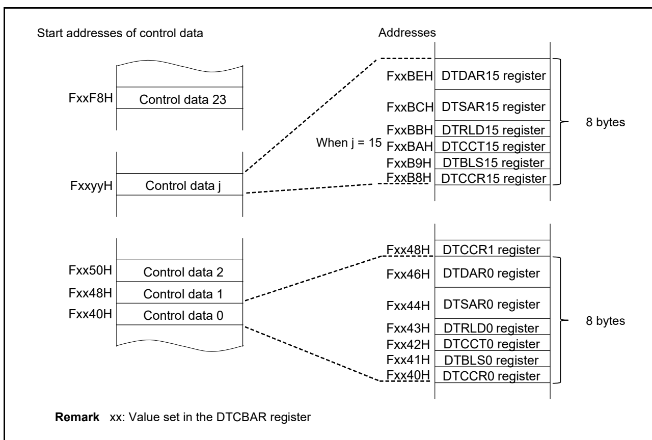
Figure 19 - 3 Control Data Allocation
