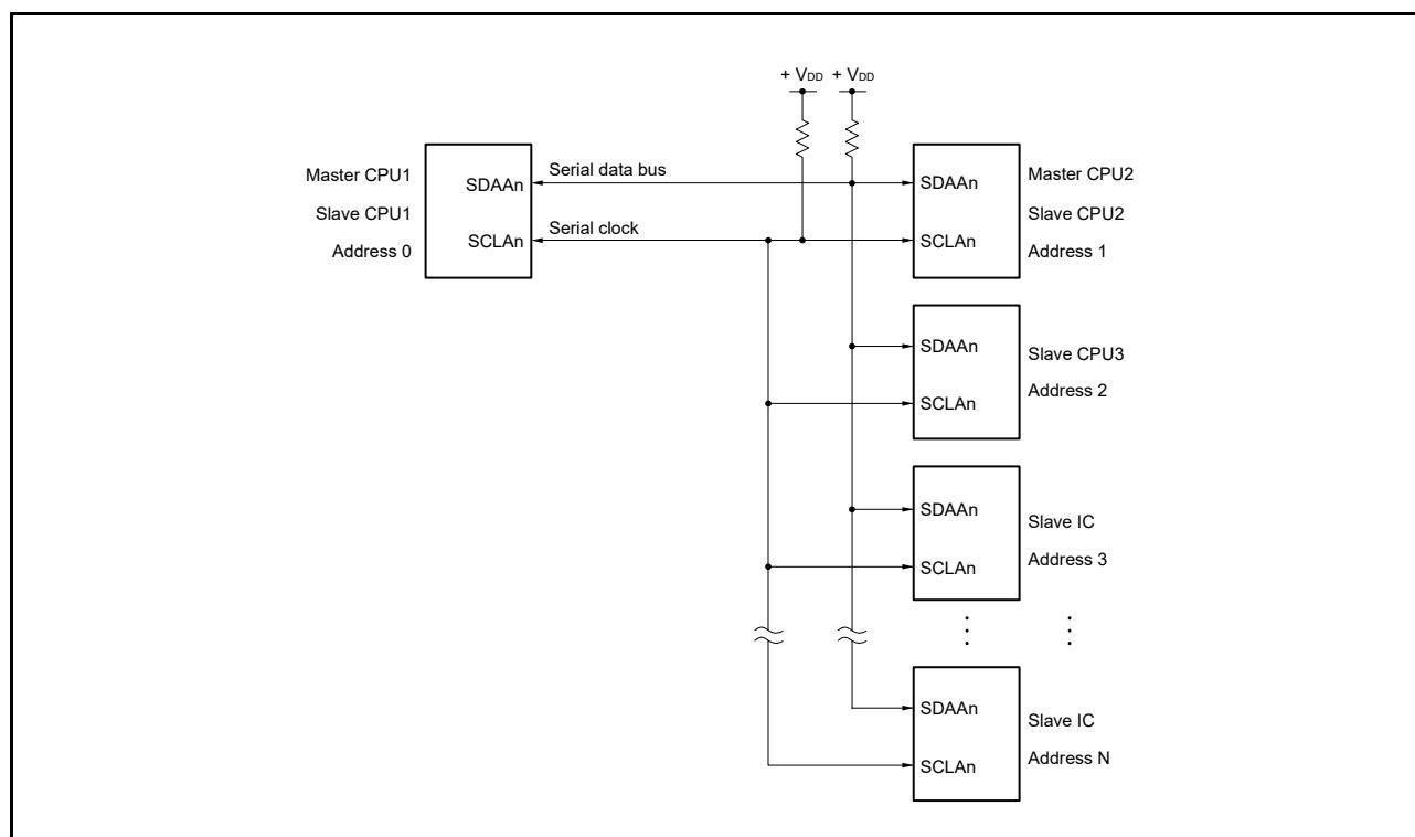
Figure 16 - 2 Example of the Serial Bus Configuration Using the I 2 C Bus
