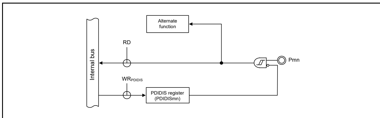
Figure 2 - 3 Pin Block Diagram for Pin Type 2-1-3
