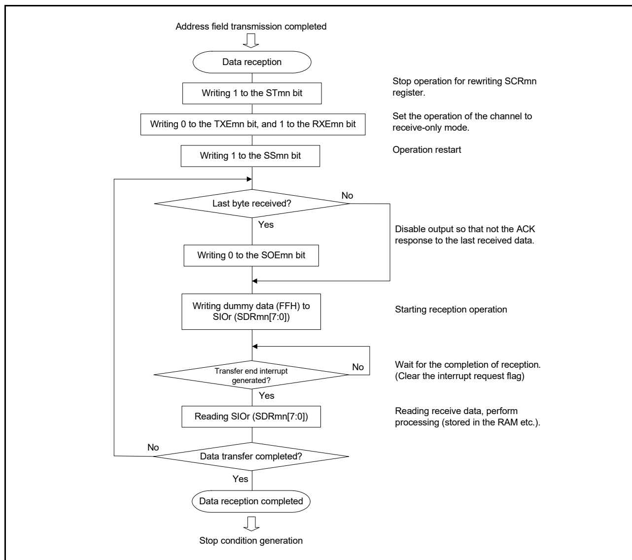
Figure 15 - 115 Flowchart of Data Reception
