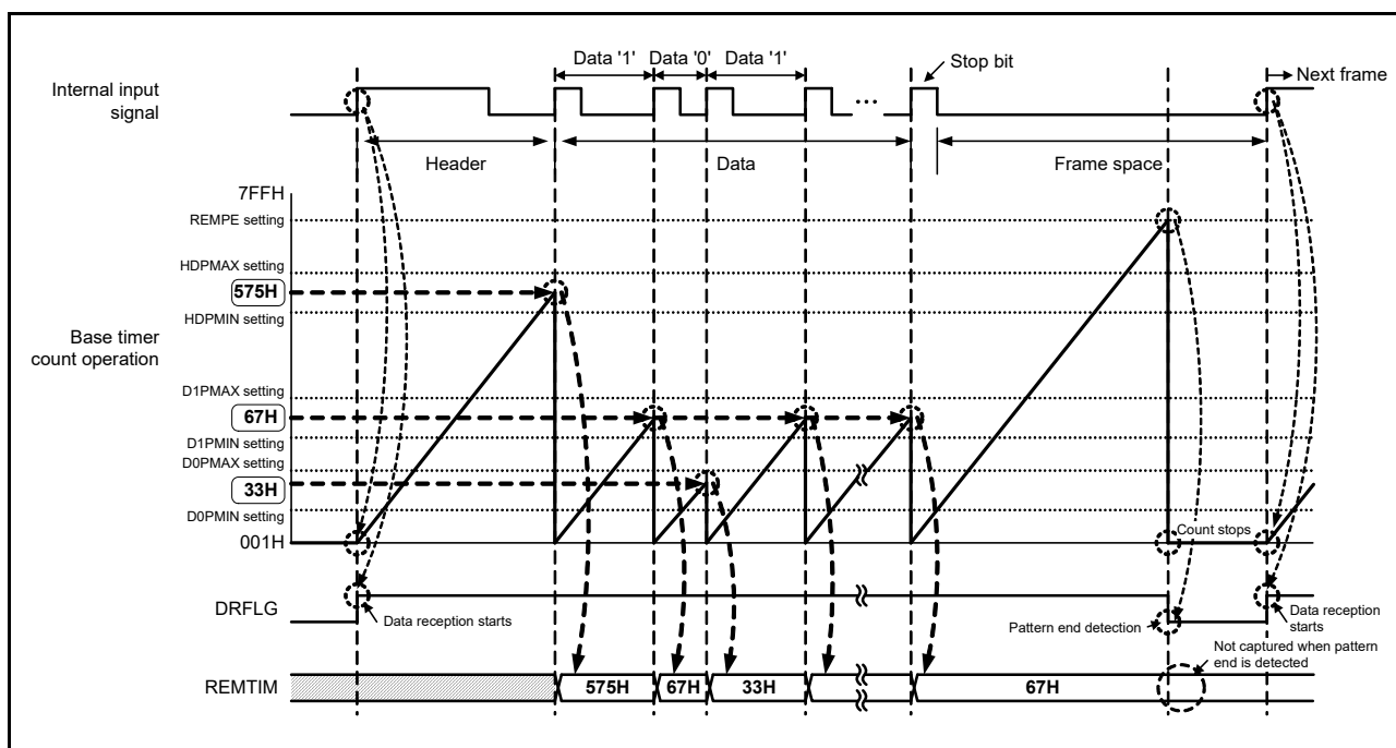
Figure 18 - 41 Operation Example of Measurement Function
