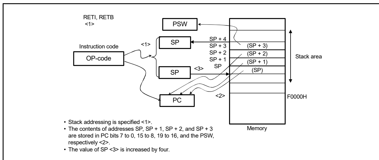
Figure 3 - 43 Example of RETI, RETB
