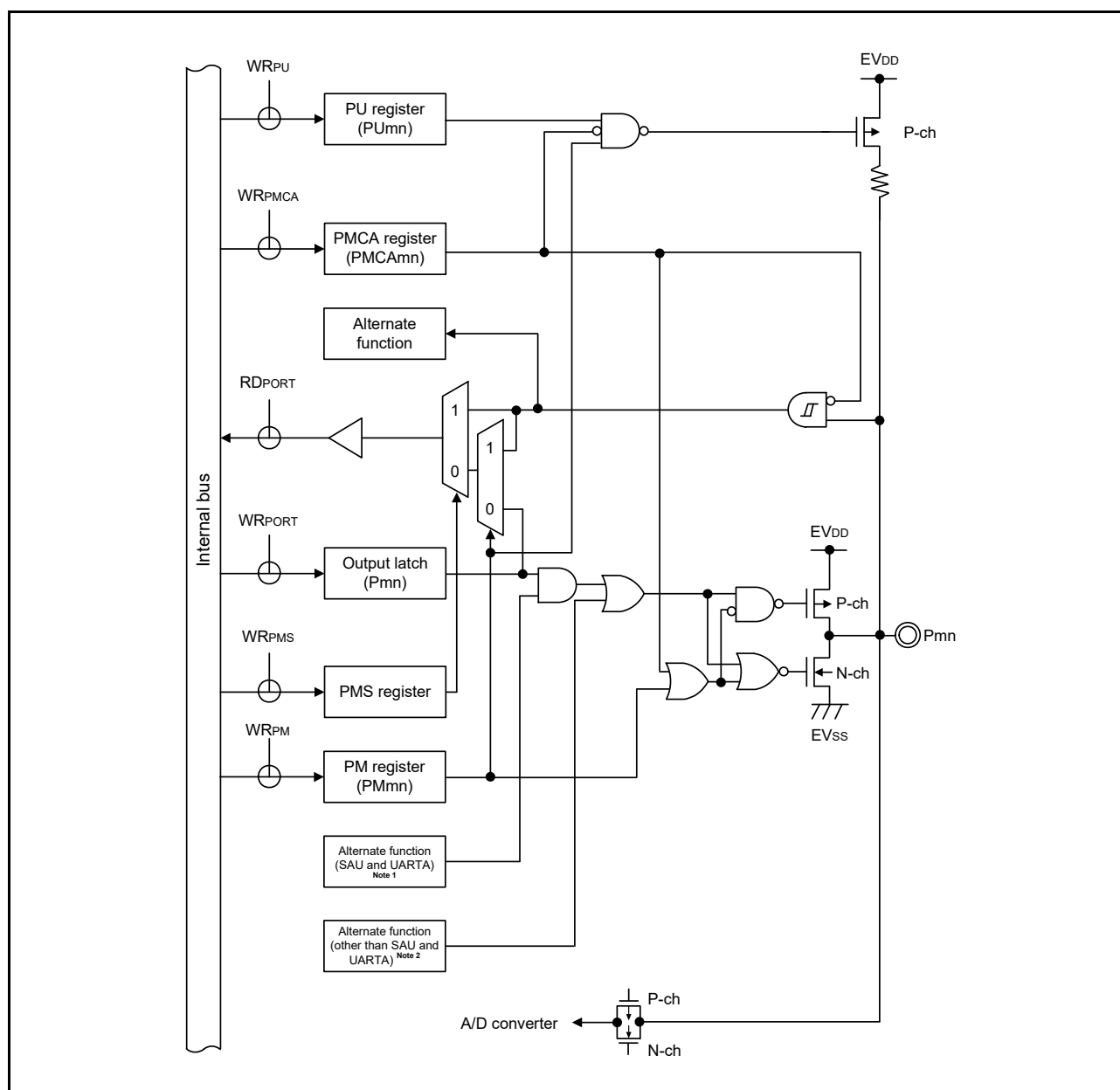
Figure 2 - 13 Pin Block Diagram for Pin Type 7-3-3
