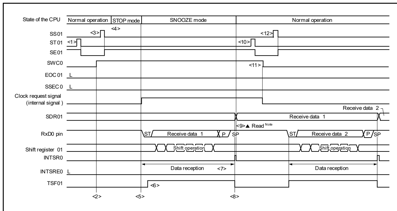
Figure 15 - 92 Timing Chart of SNOOZE Mode Operation (EOCm1 = 0, SSECm = 0/1)
