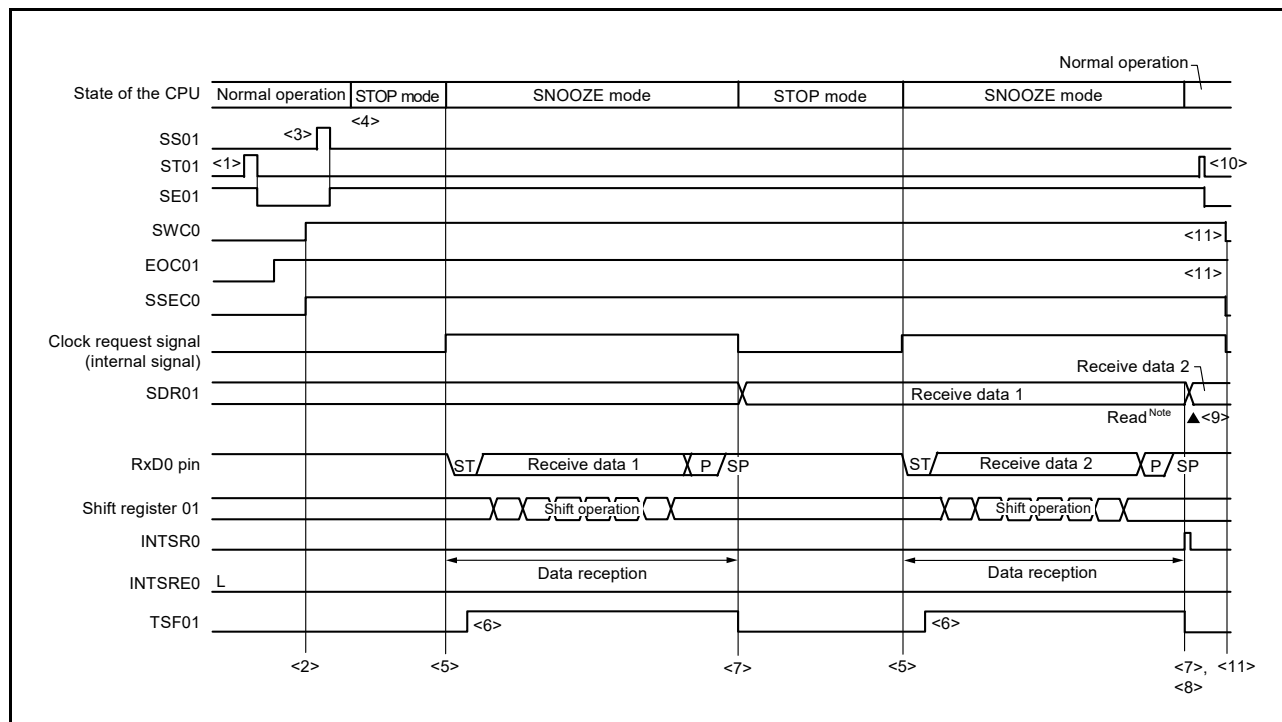
Figure 15 - 95 Timing Chart of SNOOZE Mode Operation (EOCm1 = 1, SSECm = 1)
