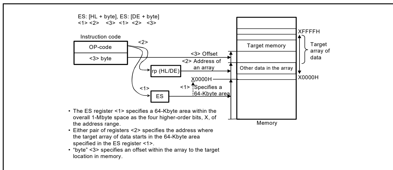
Figure 3 - 33 Example of ES:[HL + byte], ES:[DE + byte]
