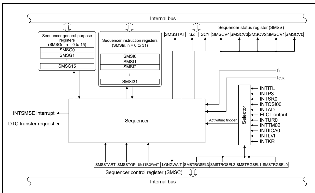
Figure 29 - 1 Block Diagram of the SNOOZE Mode Sequencer
