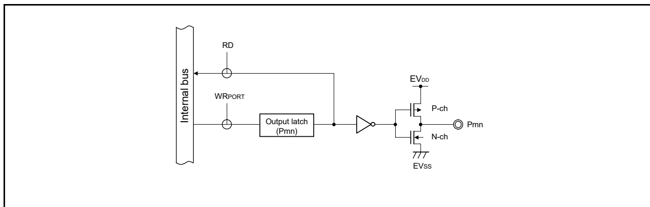
Figure 2 - 2 Pin Block Diagram for Pin Type 2-1-1
