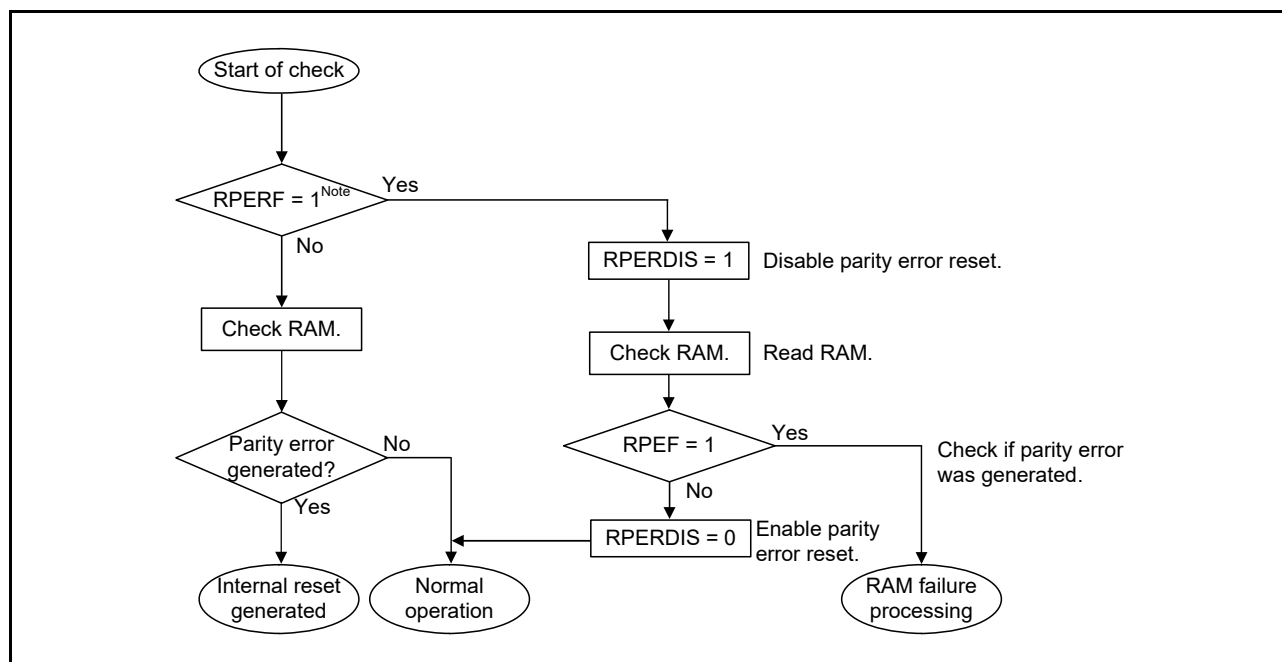
Figure 27 - 11 Flowchart of RAM Parity Check
