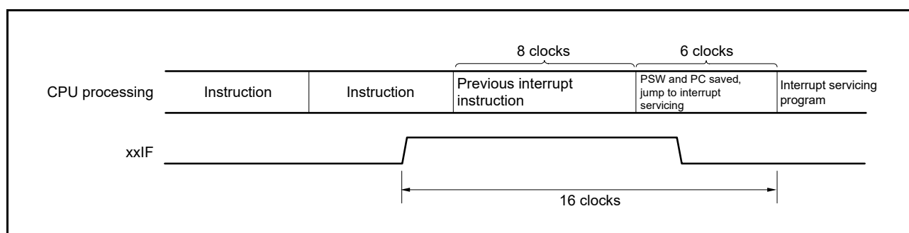
Figure 21 - 9 Interrupt Request Acknowledgment Timing (Maximum Time)
