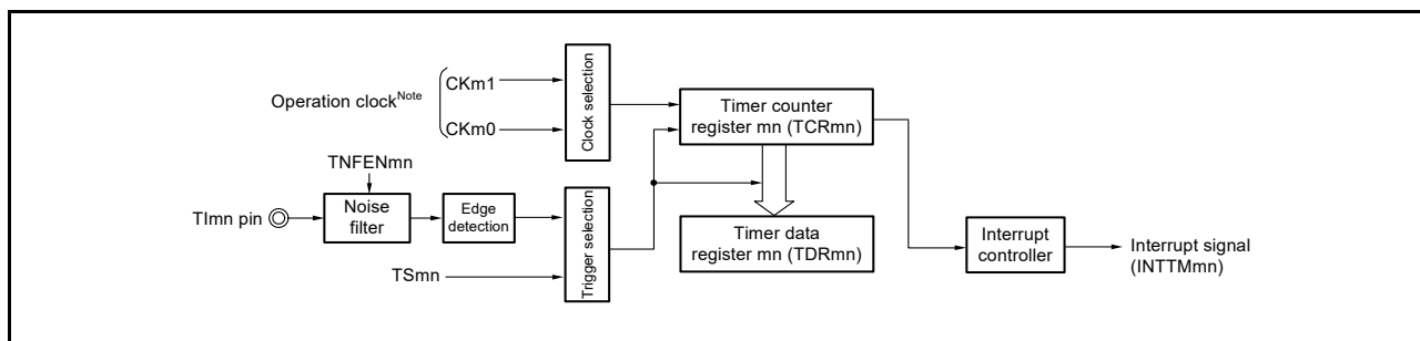
Figure 7 - 57 Block Diagram for Operation for Input Pulse Interval Measurement
