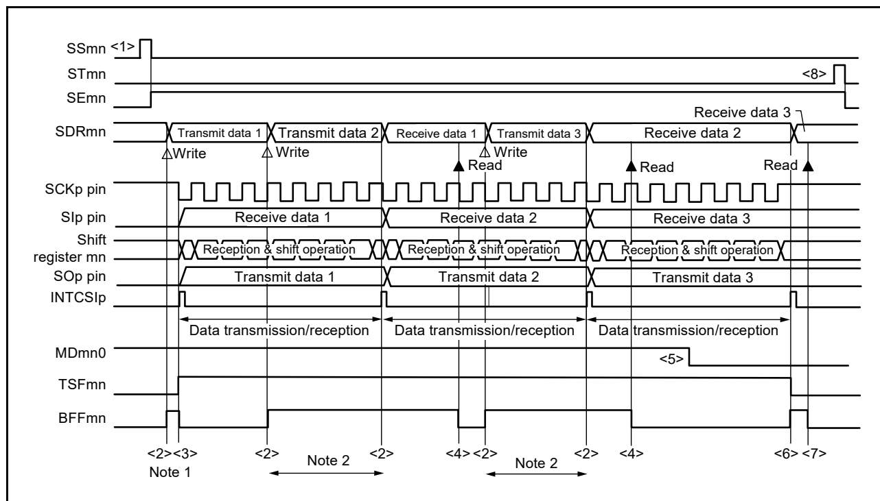
Figure 15 - 49 Timing Chart of Master Transmission/Reception (in Continuous Transmission/Reception Mode) (Type 1: DAPmn = 0, CKPmn = 0)
