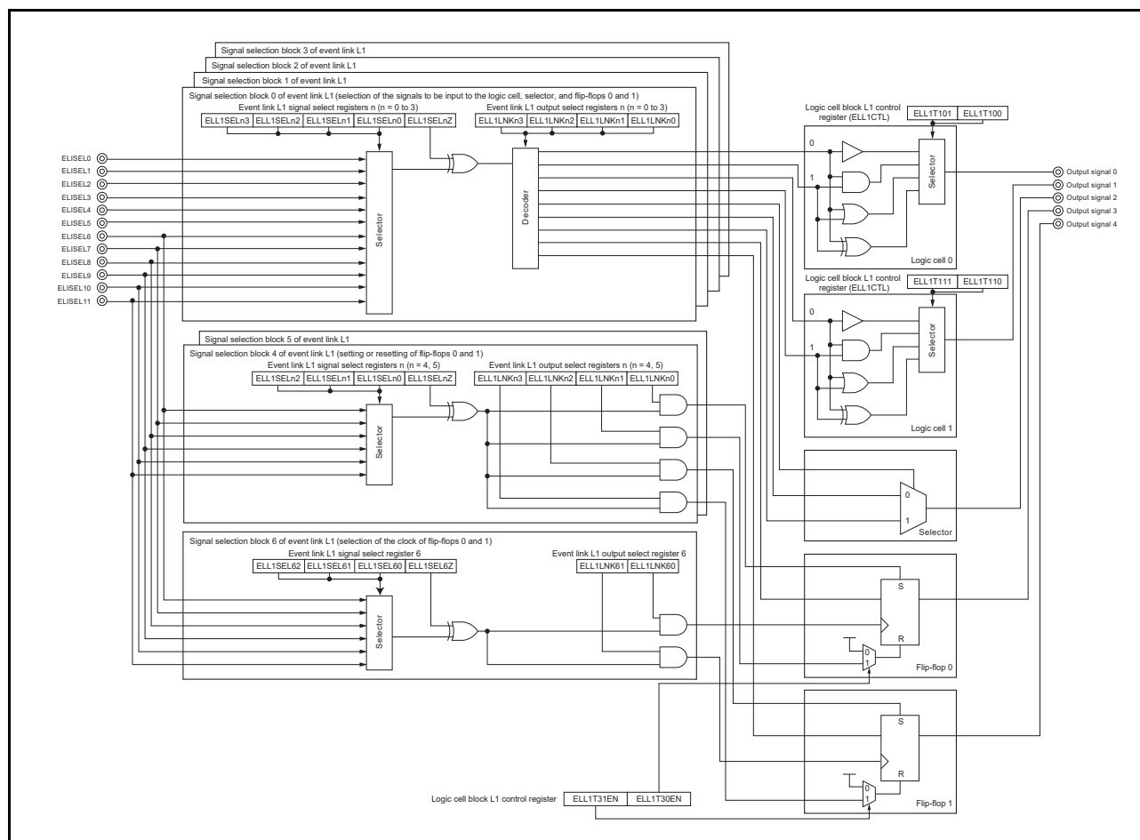
Figure 20 - 2 Block Diagram of Logic Cell Block L1
