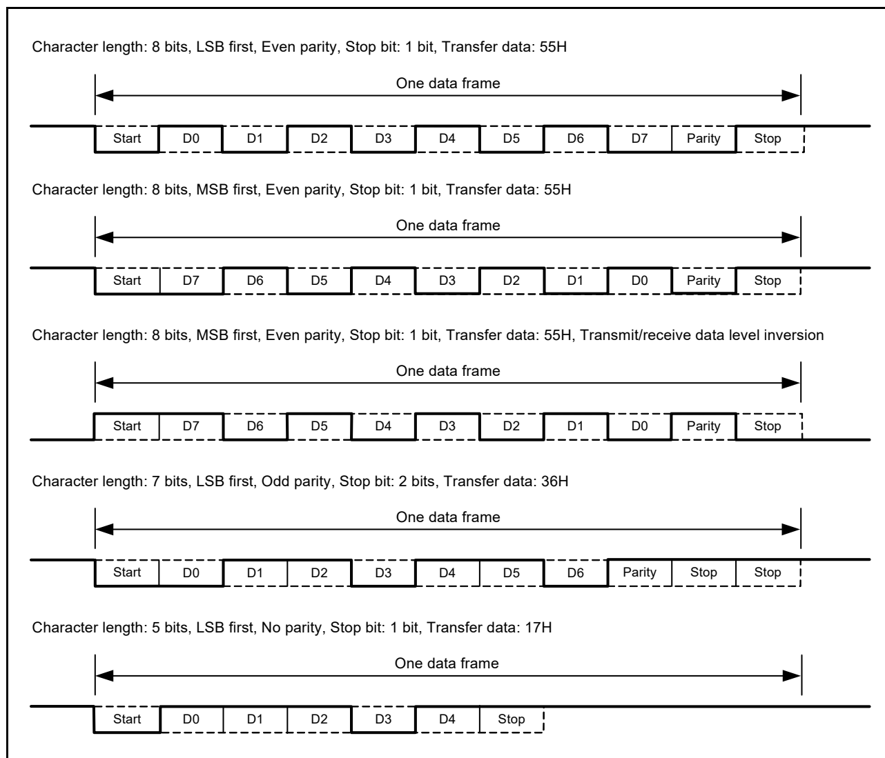
Figure 17 - 15 Example of Transmit/Receive Data Waveform
