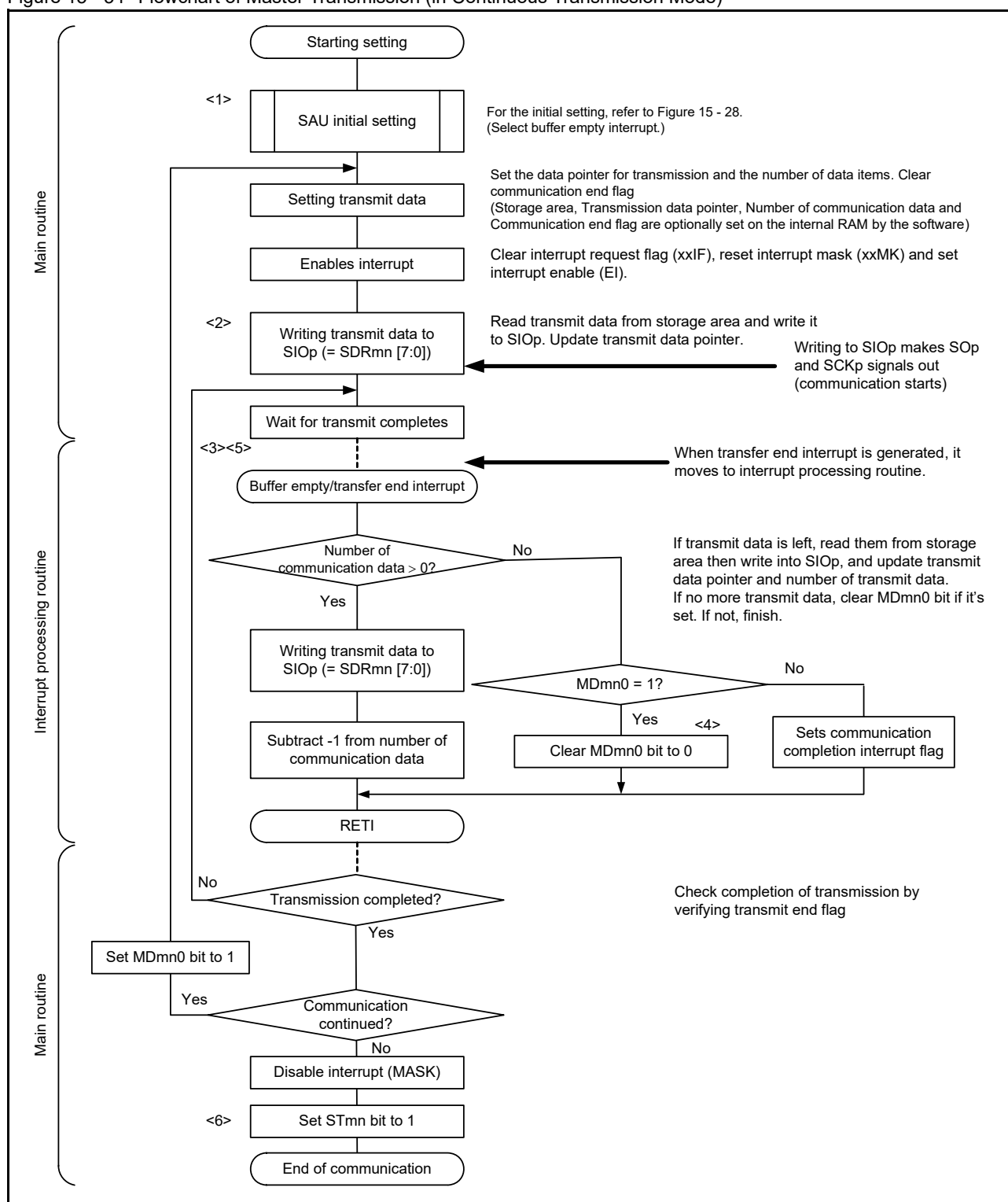
Figure 15 - 34 Flowchart of Master Transmission (in Continuous Transmission Mode)
