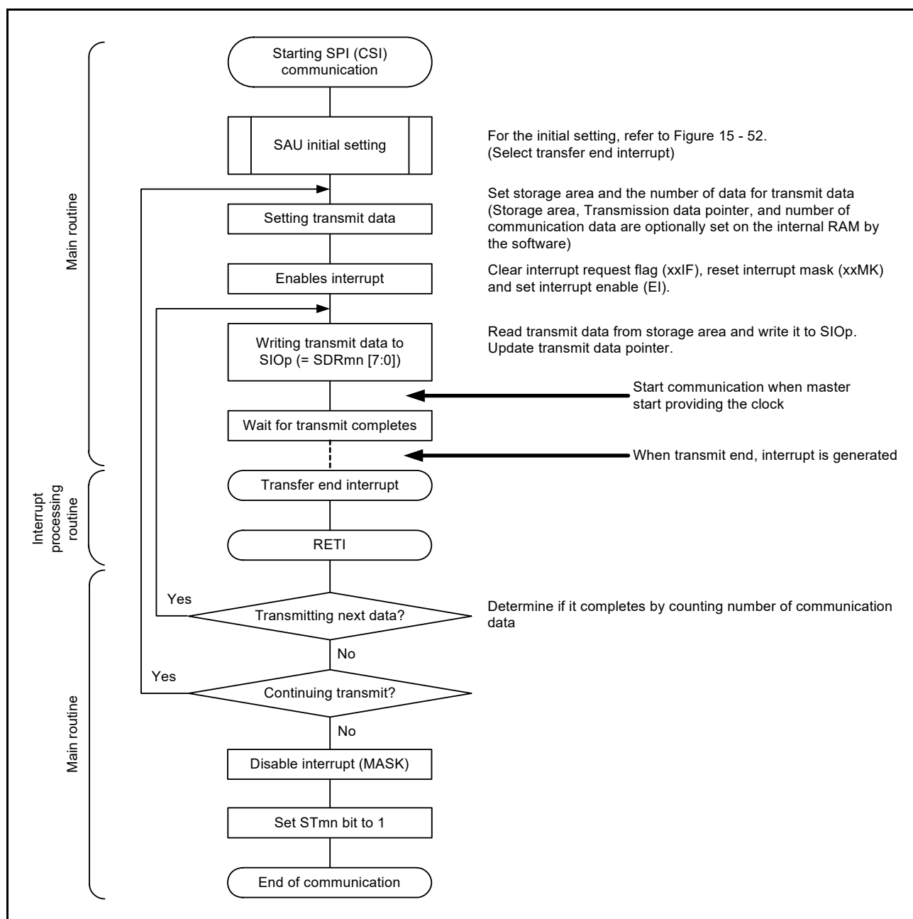
Figure 15 - 56 Flowchart of Slave Transmission (in Single-Transmission Mode)
