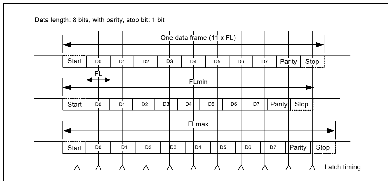
Figure 17 - 25 Permissible Baud Rate Range during Reception
