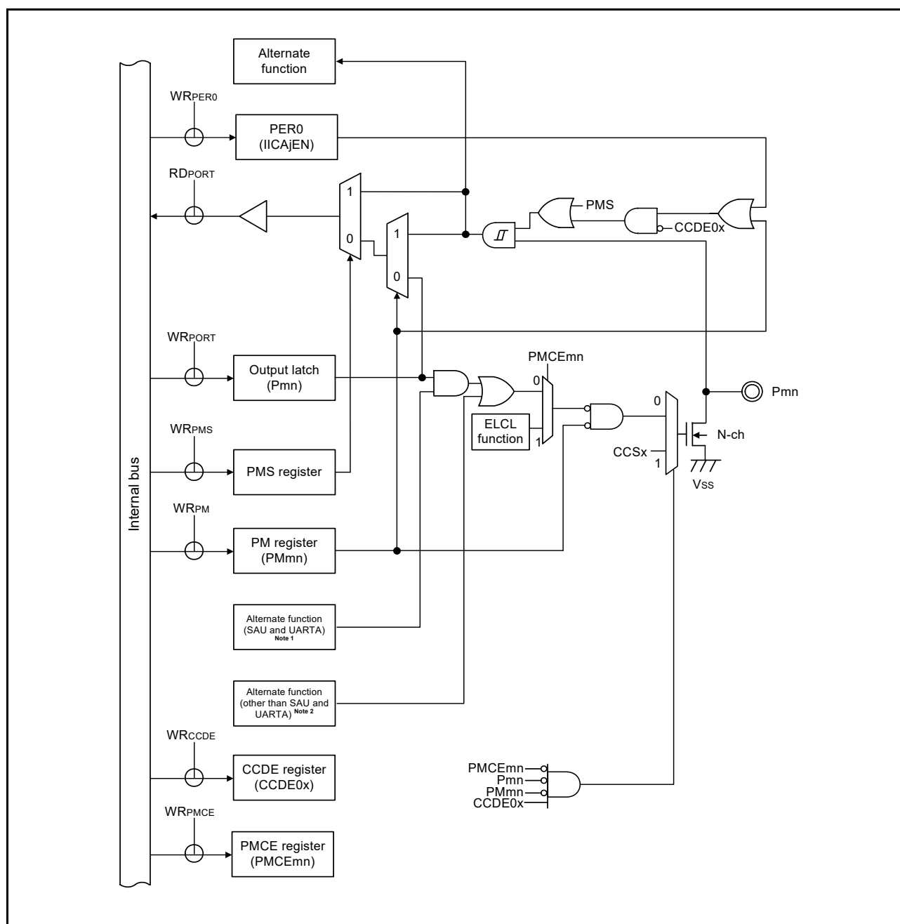
Figure 2 - 33 Pin Block Diagram for Pin Type 12-38-3
