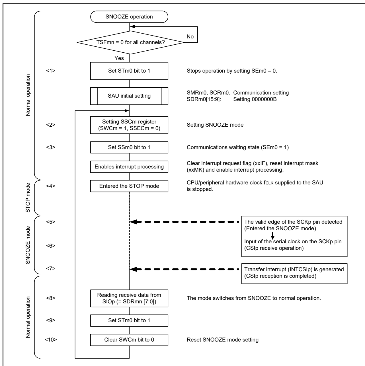
Figure 15 - 76 Flowchart of SNOOZE Mode Operation (continuous startup)
