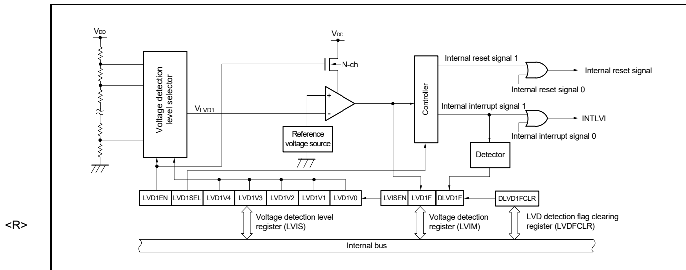
Figure 26 - 2 Block Diagram of LVD1
