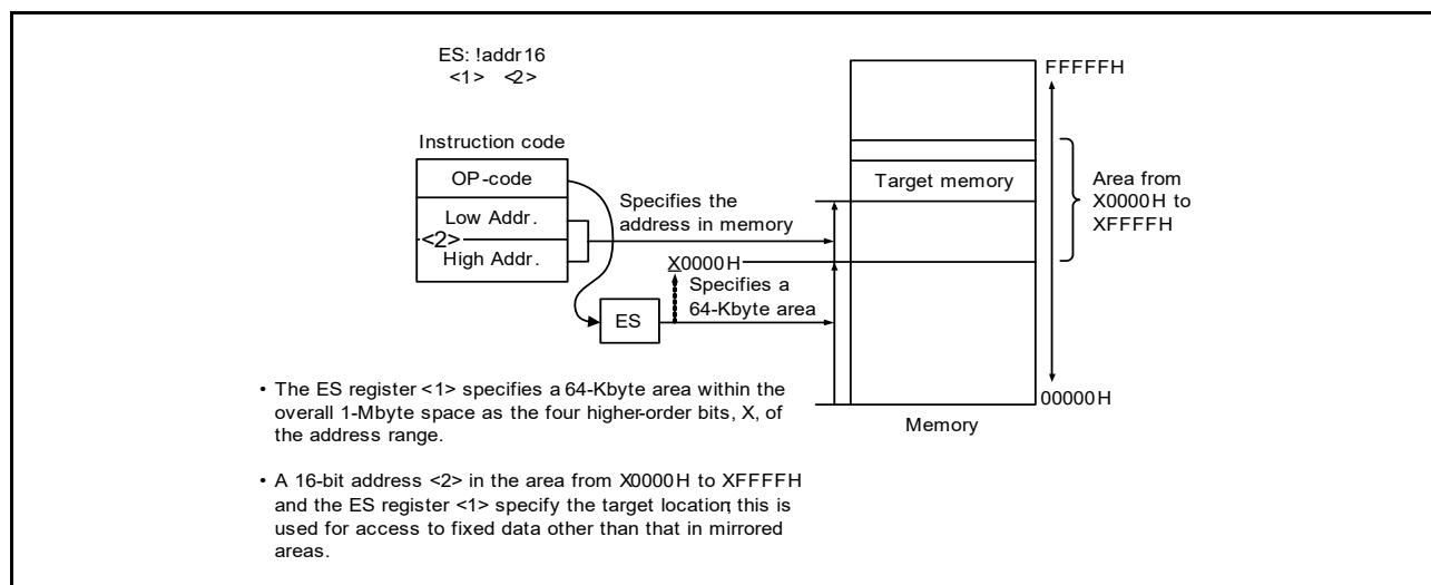
Figure 3 - 24 Example of ES:!addr16
