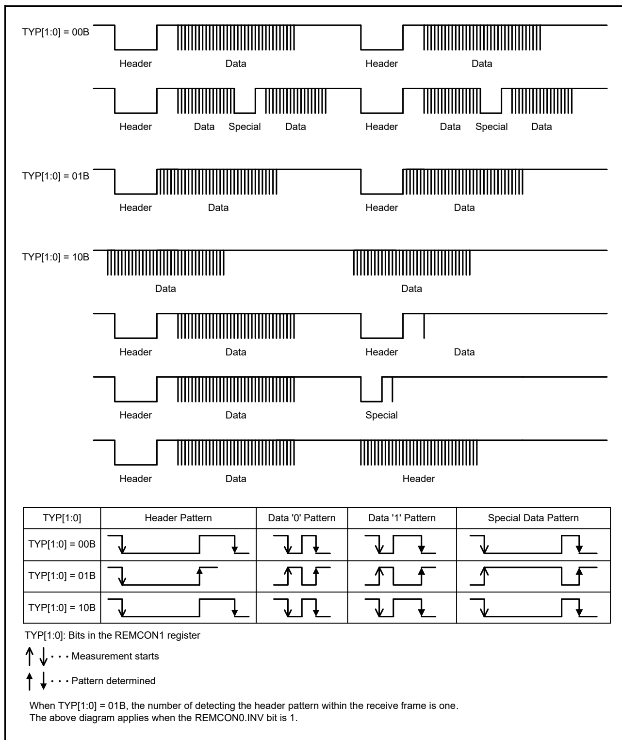
Figure 18 - 27 Example of Remote Control Signal Reception Waveform Captured by Setting REMCON1.TYP[1:0] Bits (REMCN0.INV = 1)
