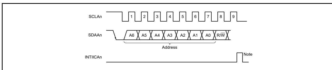
Figure 16 - 16 Addresses
