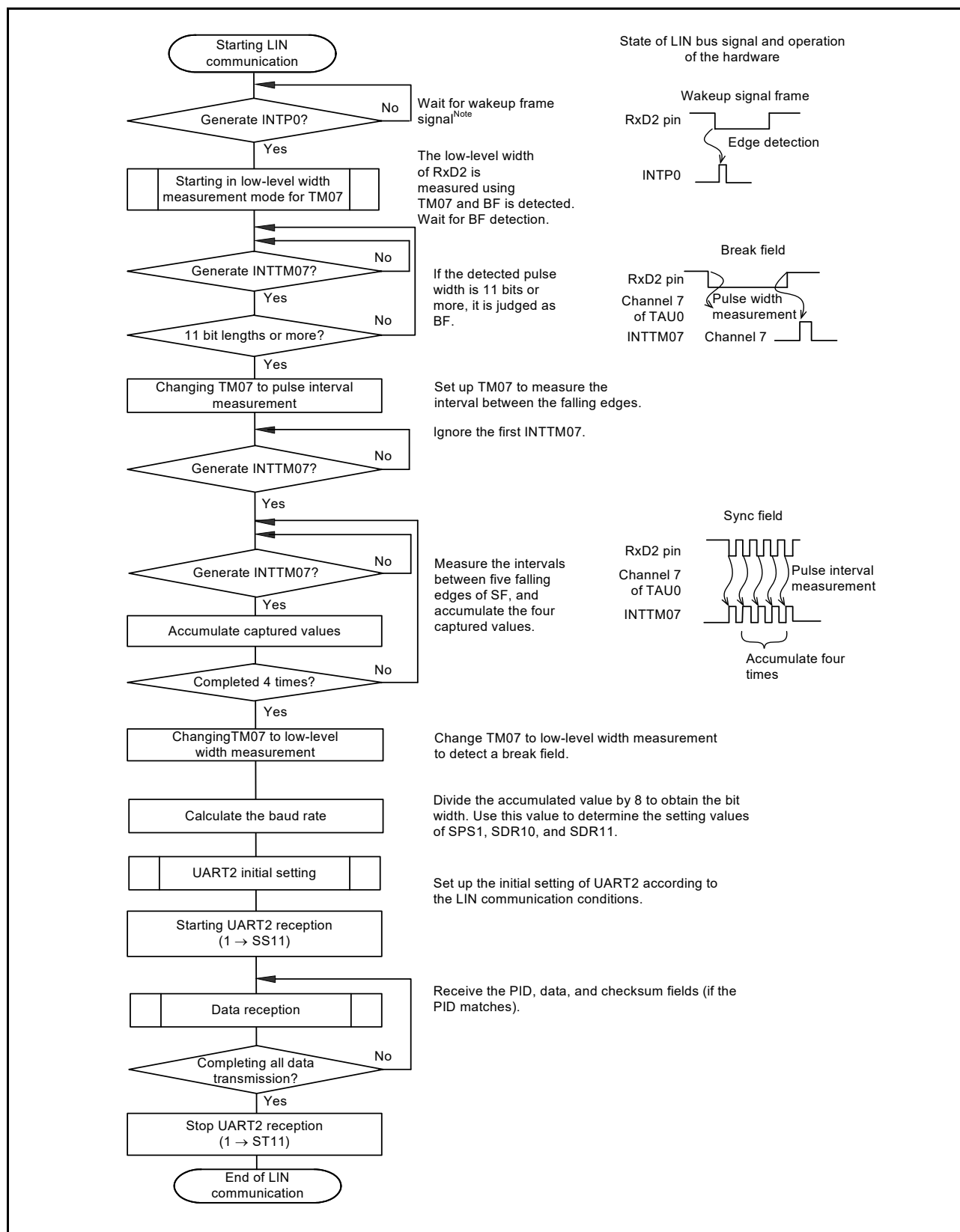
Figure 15 - 103 Flowchart of LIN Reception
