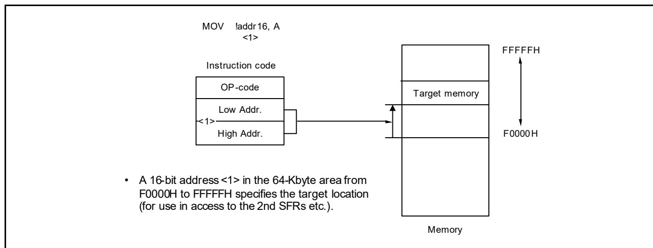
Figure 3 - 23 Example of !addr16
