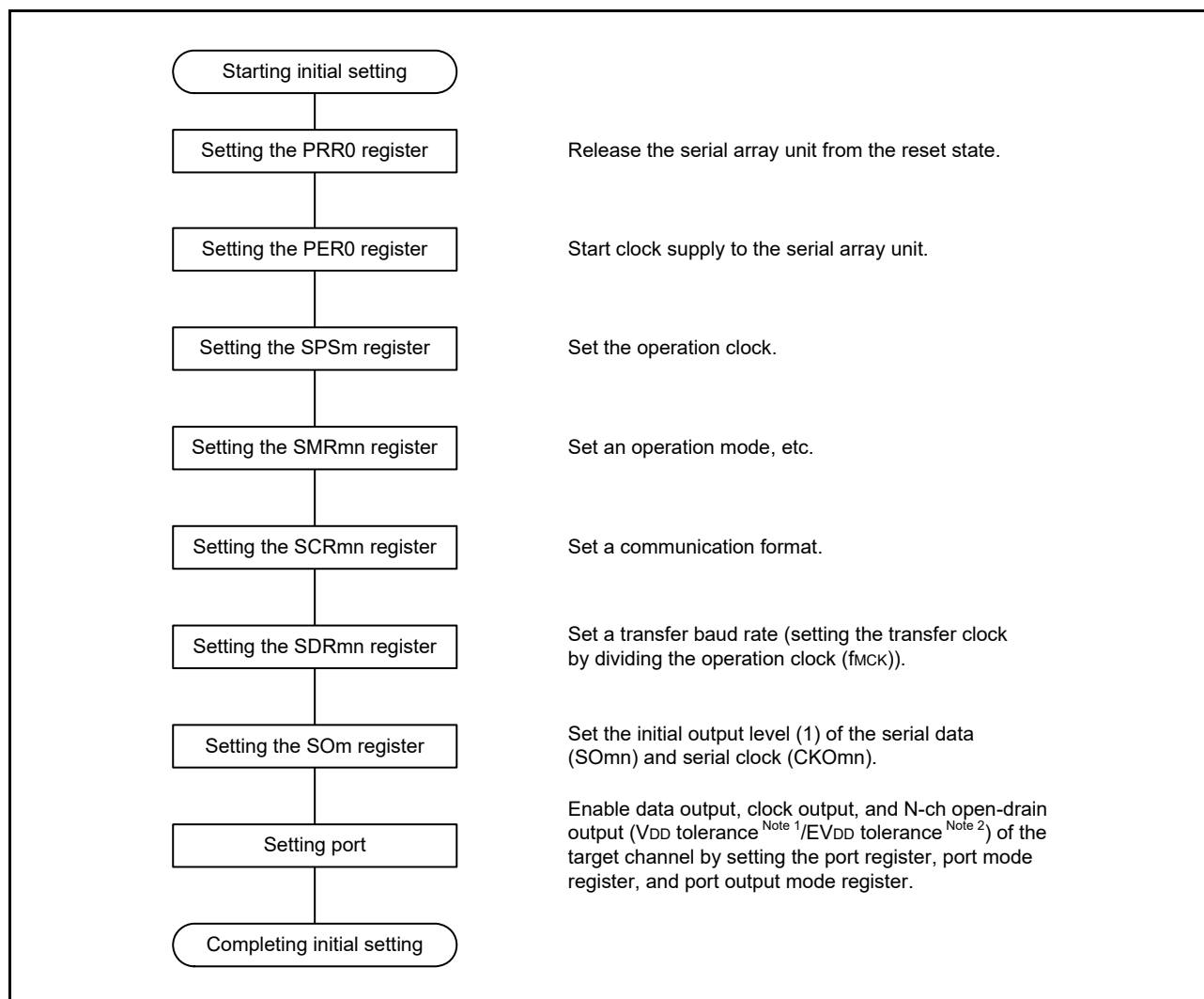
Figure 15 - 107 Initial Setting Procedure for Simplified I 2 C Address Field Transmission
