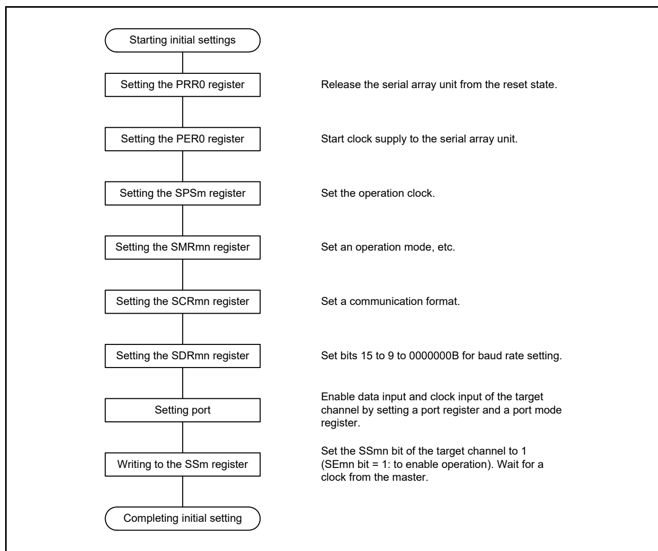
Figure 15 - 60 Initial Setting Procedure for Slave Reception
