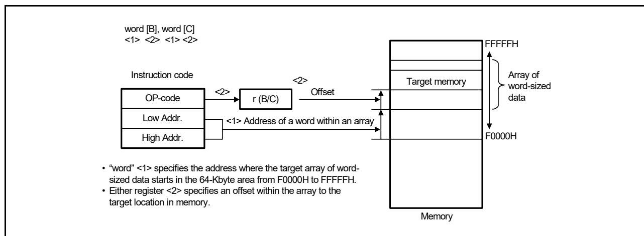
Figure 3 - 31 Example of word [B], word [C]
