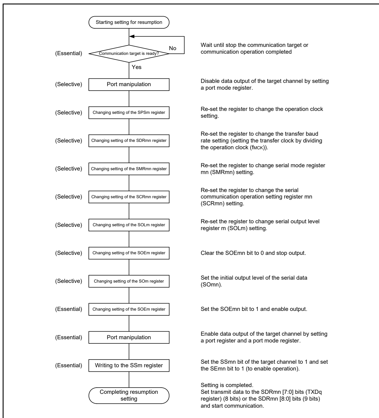
Figure 15 - 81 Procedure for Resuming UART Transmission
