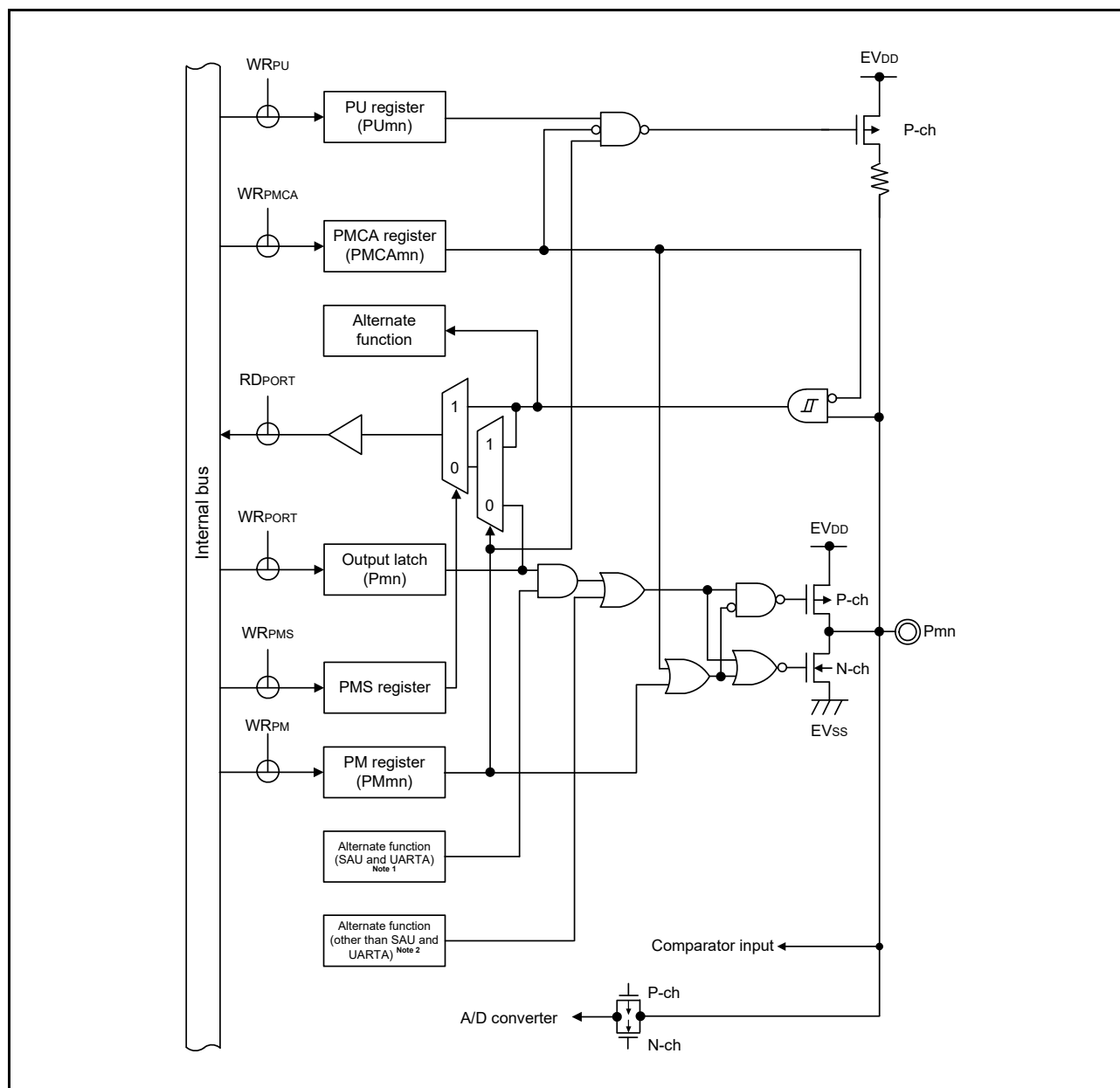
Figure 2 - 14 Pin Block Diagram for Pin Type 7-9-5
