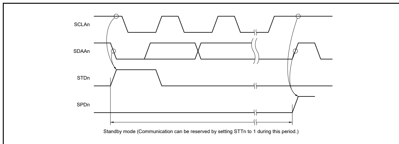
Figure 16 - 26 Timing for Accepting Communication Reservations
