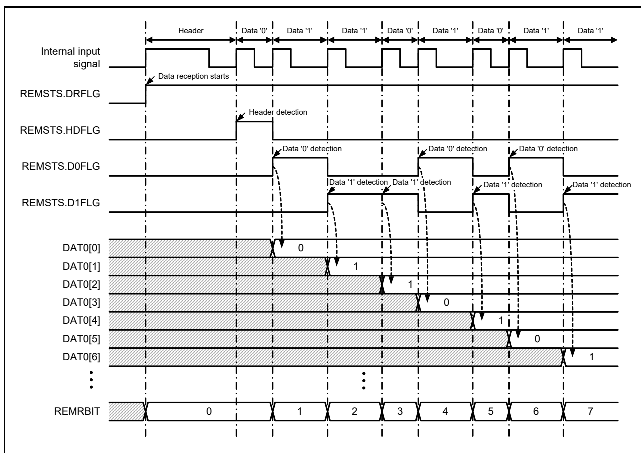
Figure 18 - 34 Operation of Receive Data Buffer
