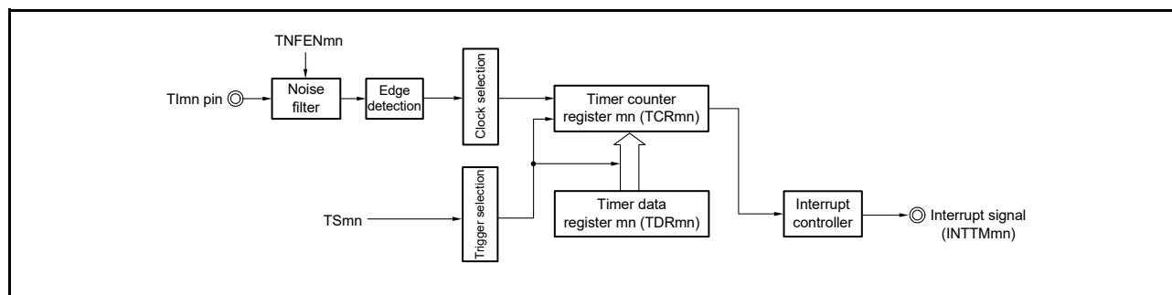
Figure 7 - 49 Block Diagram for Operation as an External Event Counter
