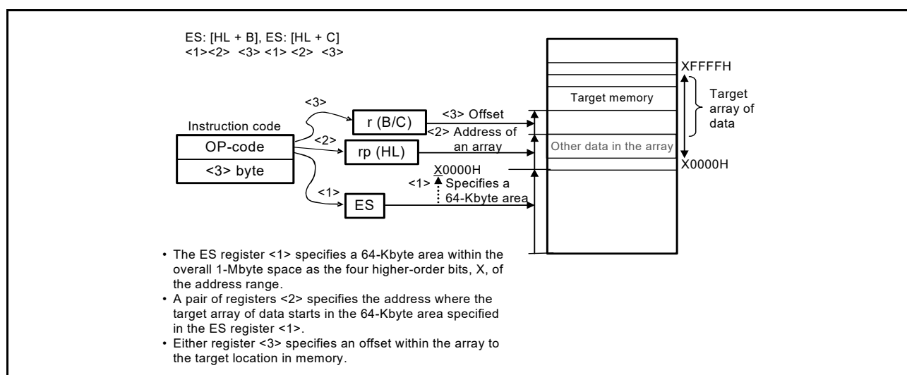
Figure 3 - 37 Example of ES:[HL + B], ES:[HL + C]
