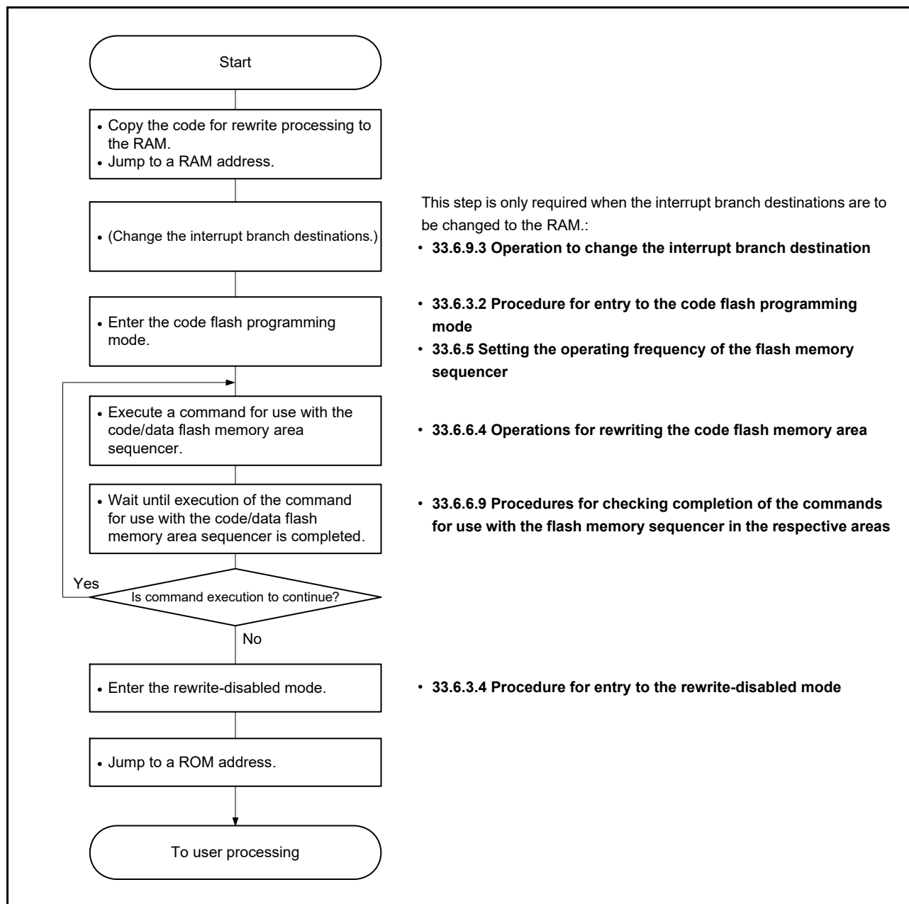
Figure 33 - 30 Flow of Executing the Commands to Rewrite the Code Flash Memory Area
