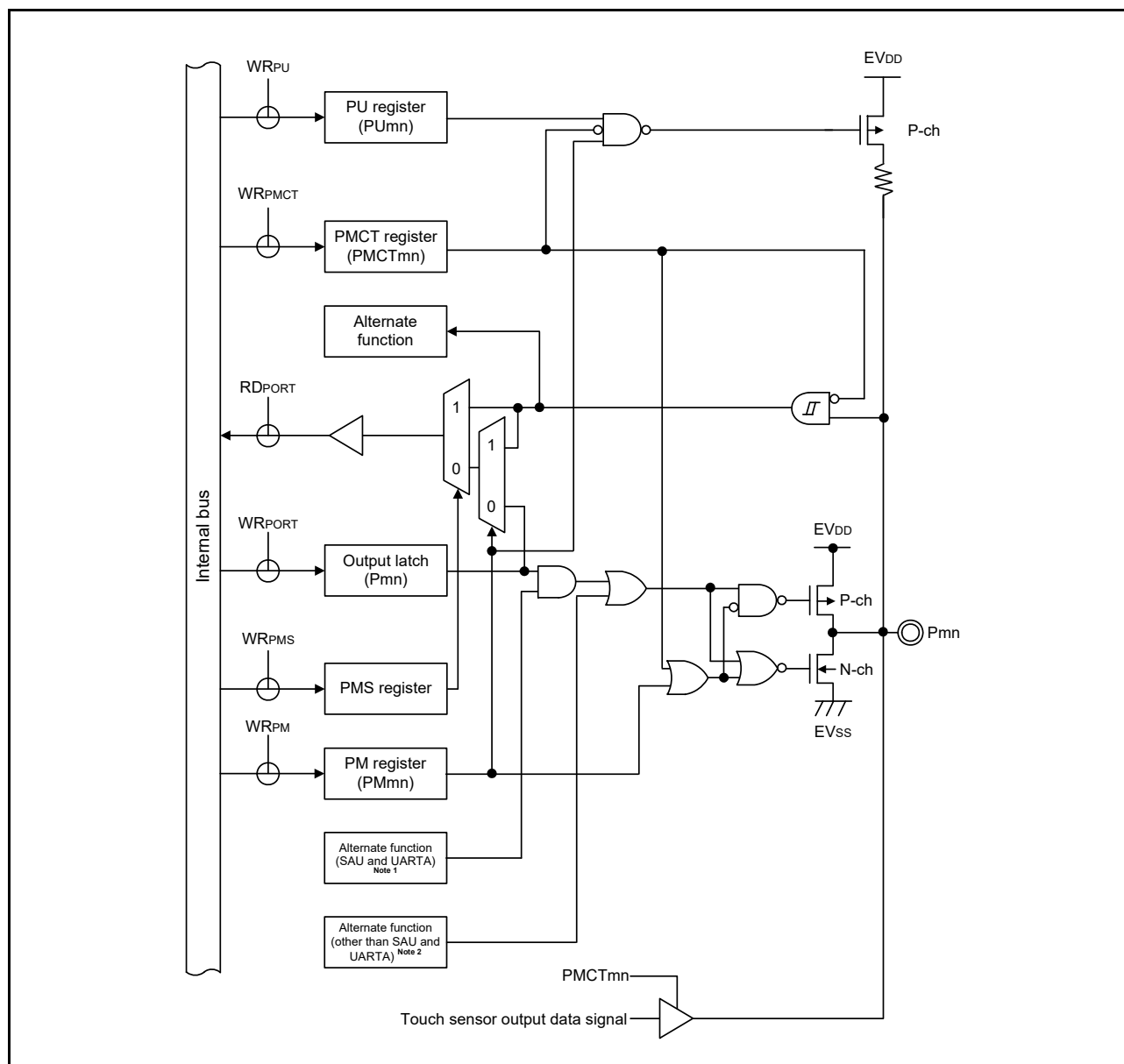
Figure 2 - 16 Pin Block Diagram for Pin Type 7-31-2
