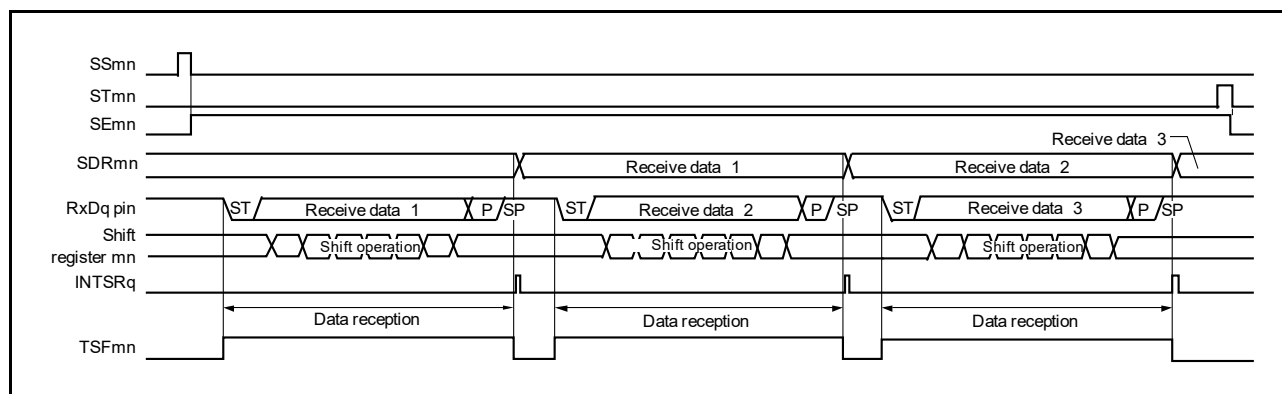
Figure 15 - 90 Timing Chart of UART Reception
