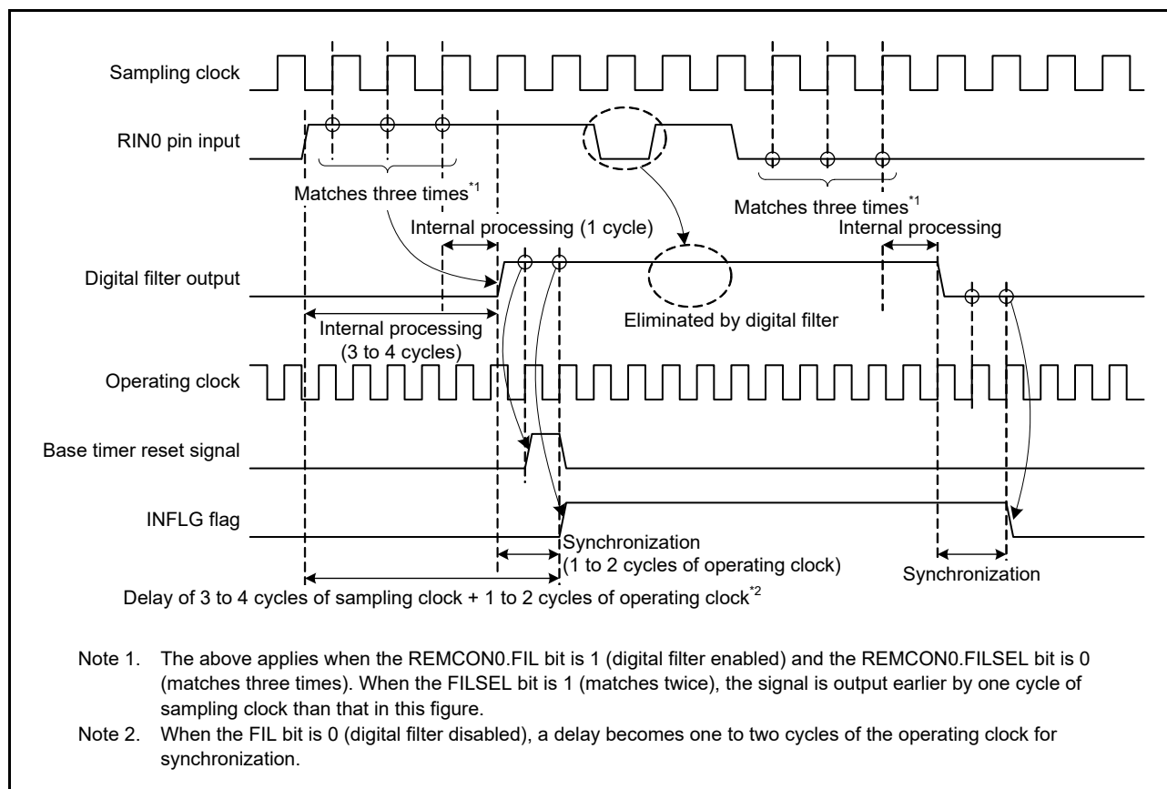
Figure 18 - 29 Digital Filtering for RIN0 Input
