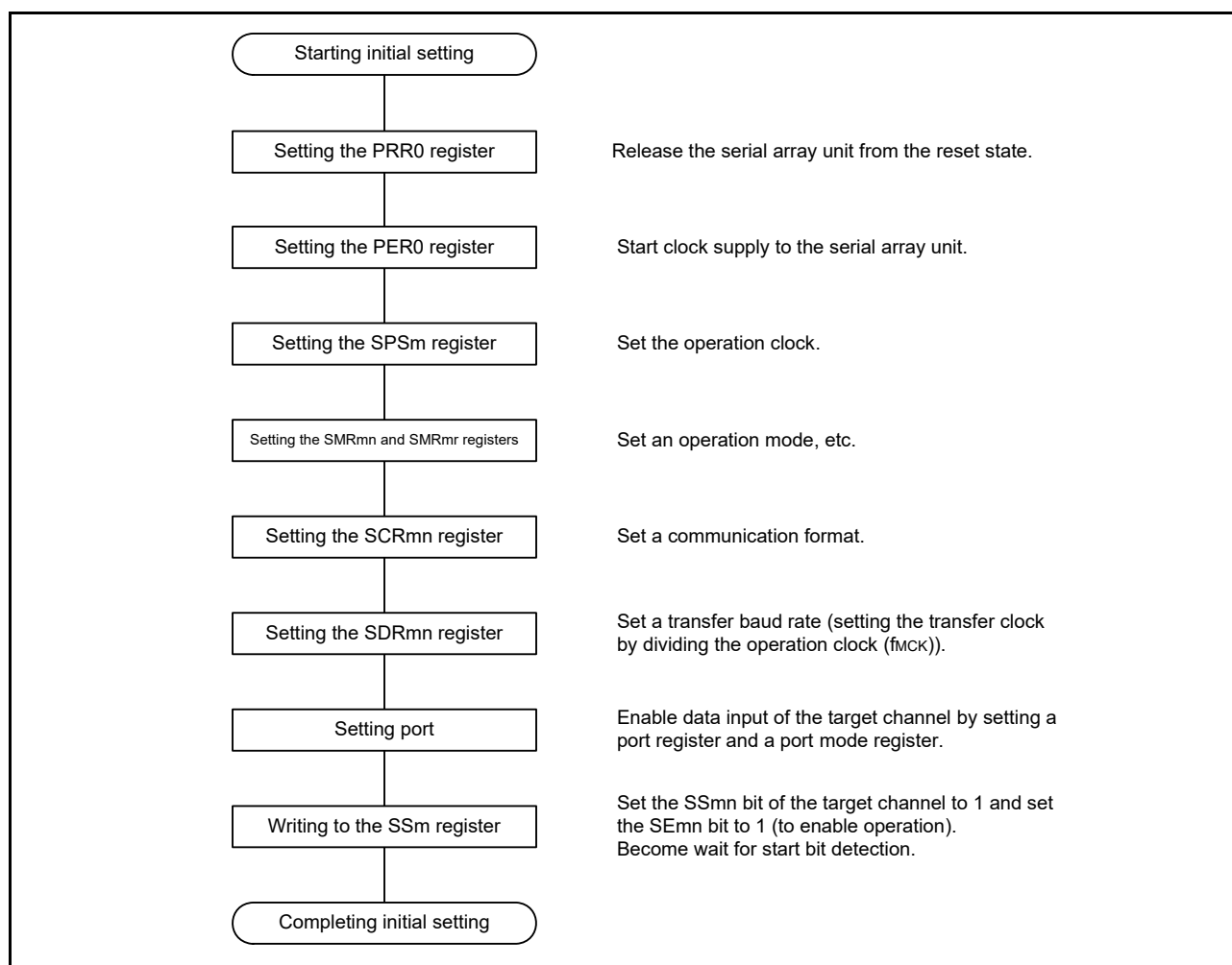
Figure 15 - 87 Initial Setting Procedure for UART Reception
