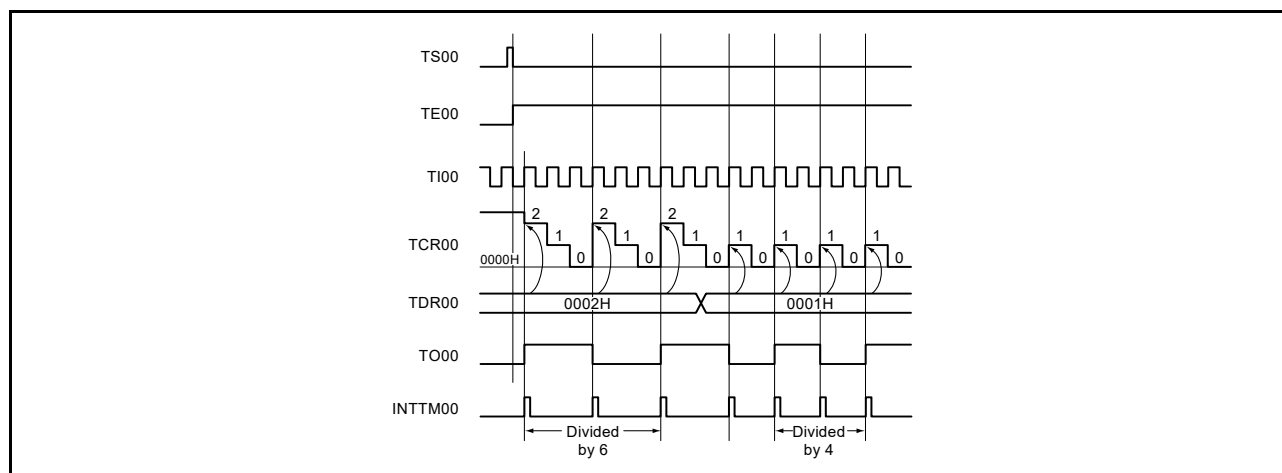
Figure 7 - 54 Example of Basic Timing during Operation as a Frequency Divider (MD000 = 1)
