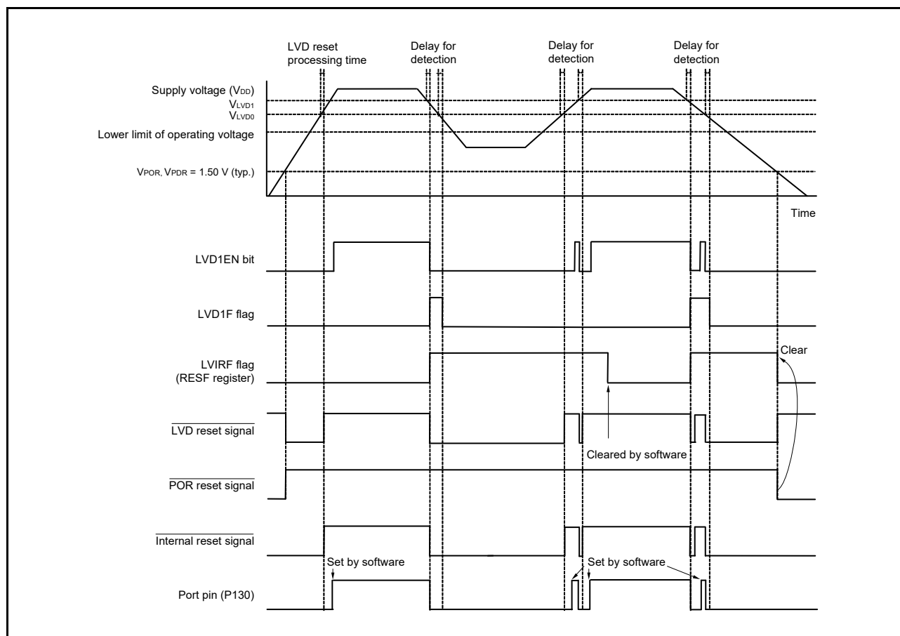
&lt;R&gt; Figure 26 - 7 Timing of LVD1 Internal Reset Signal Generation
