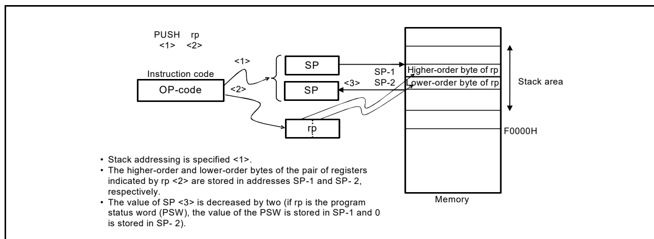
Figure 3 - 38 Example of PUSH rp
