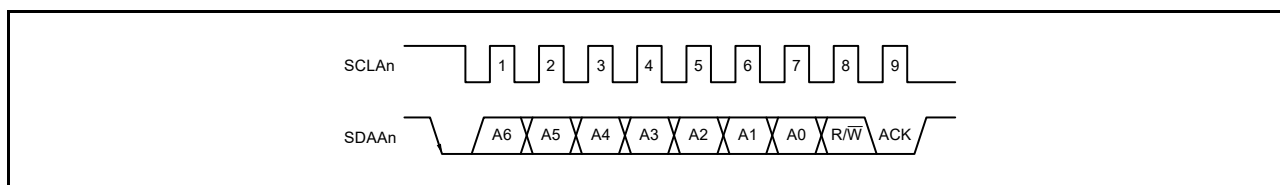
Figure 16 - 18 ACK
