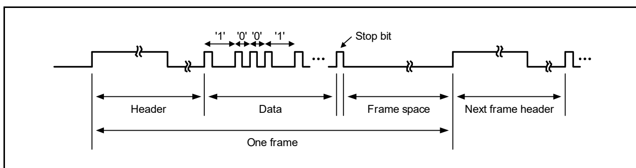
Figure 18 - 24 Example of Remote Control Signal
