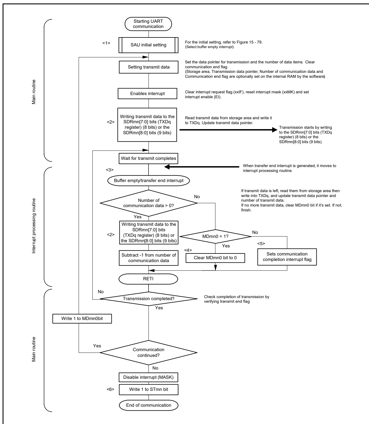
Figure 15 - 85 Flowchart of UART Transmission (in Continuous Transmission Mode)
