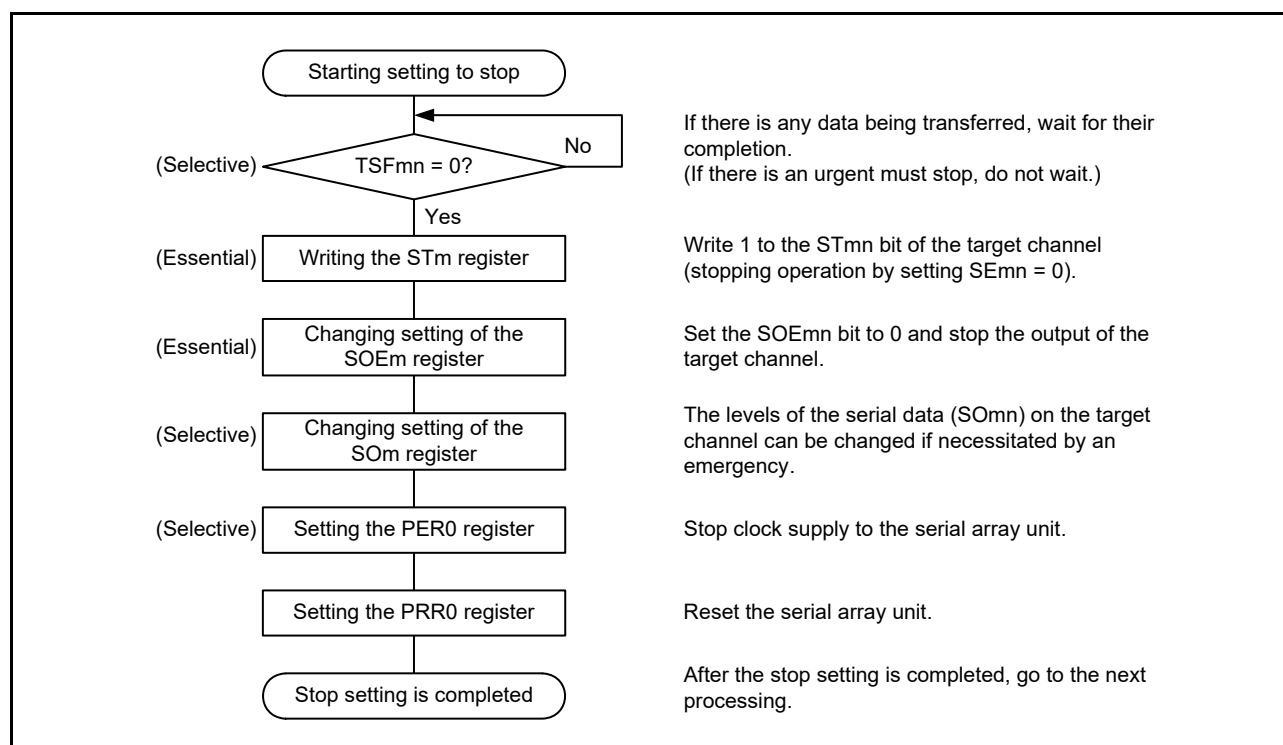
Figure 15 - 53 Procedure for Stopping Slave Transmission
