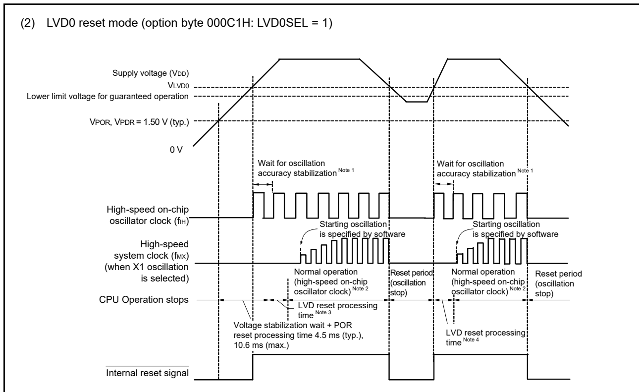
Figure 25 - 2 Timing of Generation of Internal Reset Signal by Power-on-reset Circuit and Voltage Detector (2/2)
