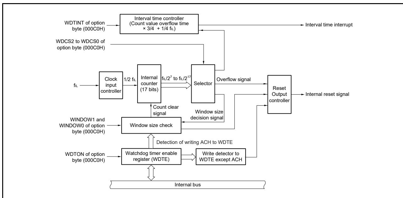
Figure 11 - 1 Block Diagram of Watchdog Timer
