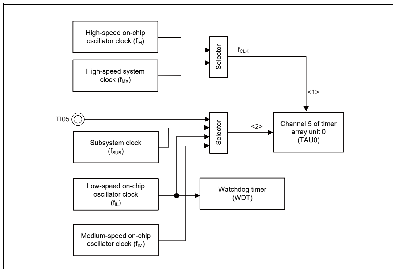
Figure 27 - 17 Configuration of Frequency Detection Function
