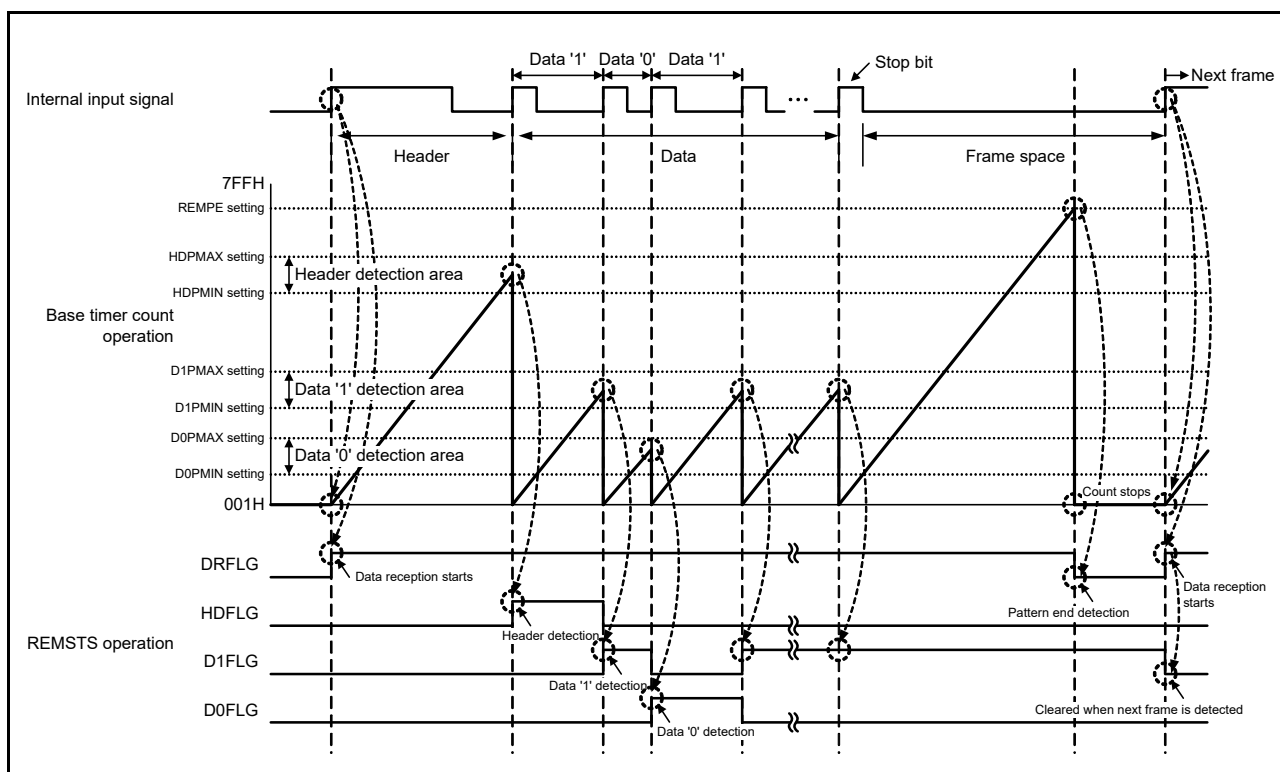
Figure 18 - 30 Waveform of REMC Operation
