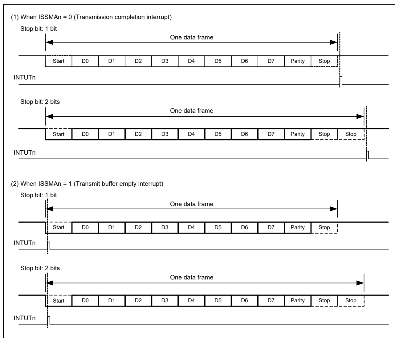
Figure 17 - 16 Interrupt Output Timing
