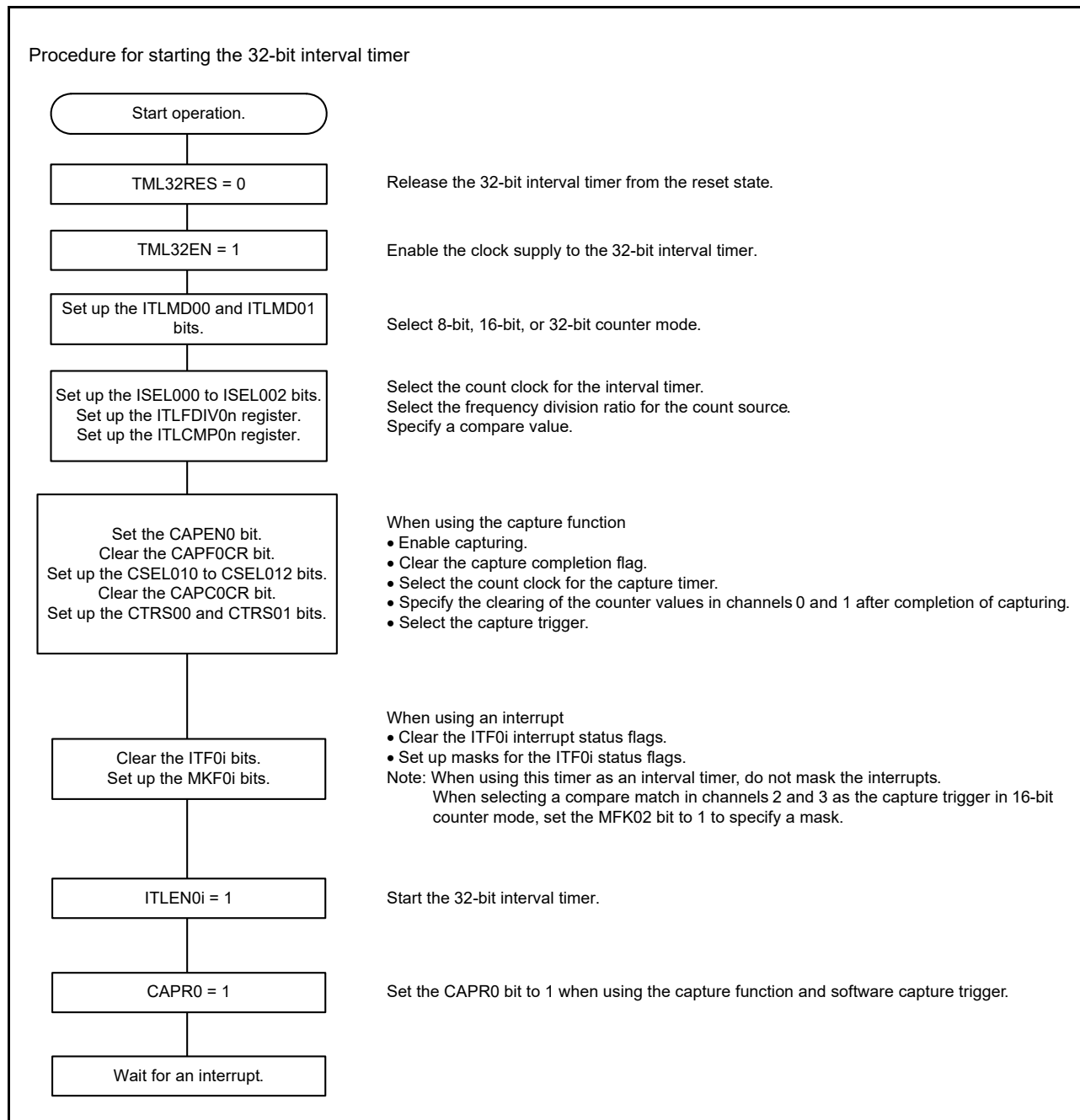
Figure 9 - 16 Procedure for Starting the 32-Bit Interval Timer
