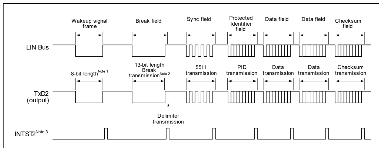
Figure 15 - 100 Transmission Operation of LIN
