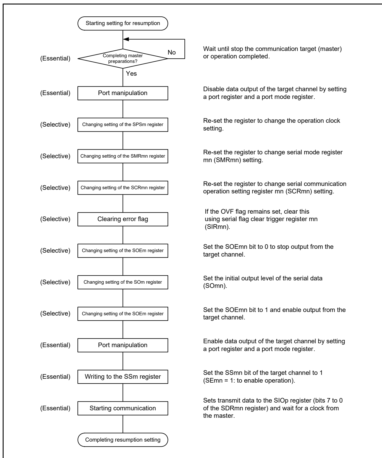
Figure 15 - 68 Procedure for Resuming Slave Transmission/Reception
