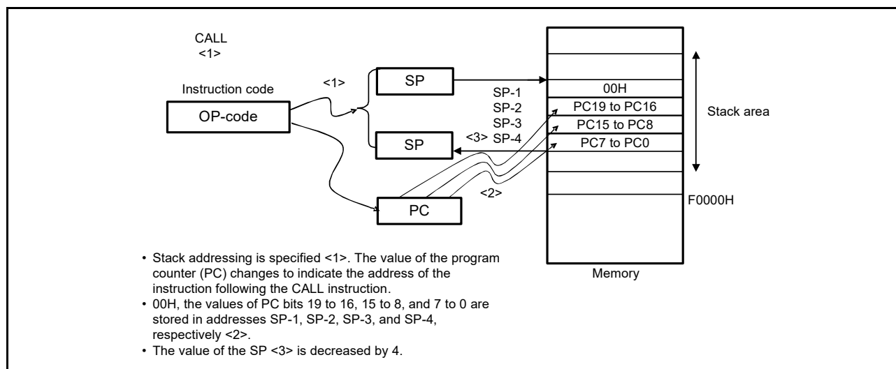
Figure 3 - 40 Example of CALL, CALLT
