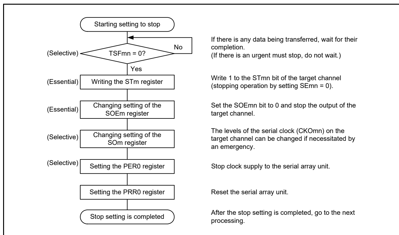
Figure 15 - 37 Procedure for Stopping Master Reception
