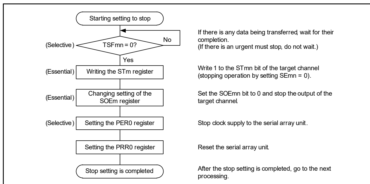
Figure 15 - 61 Procedure for Stopping Slave Reception
