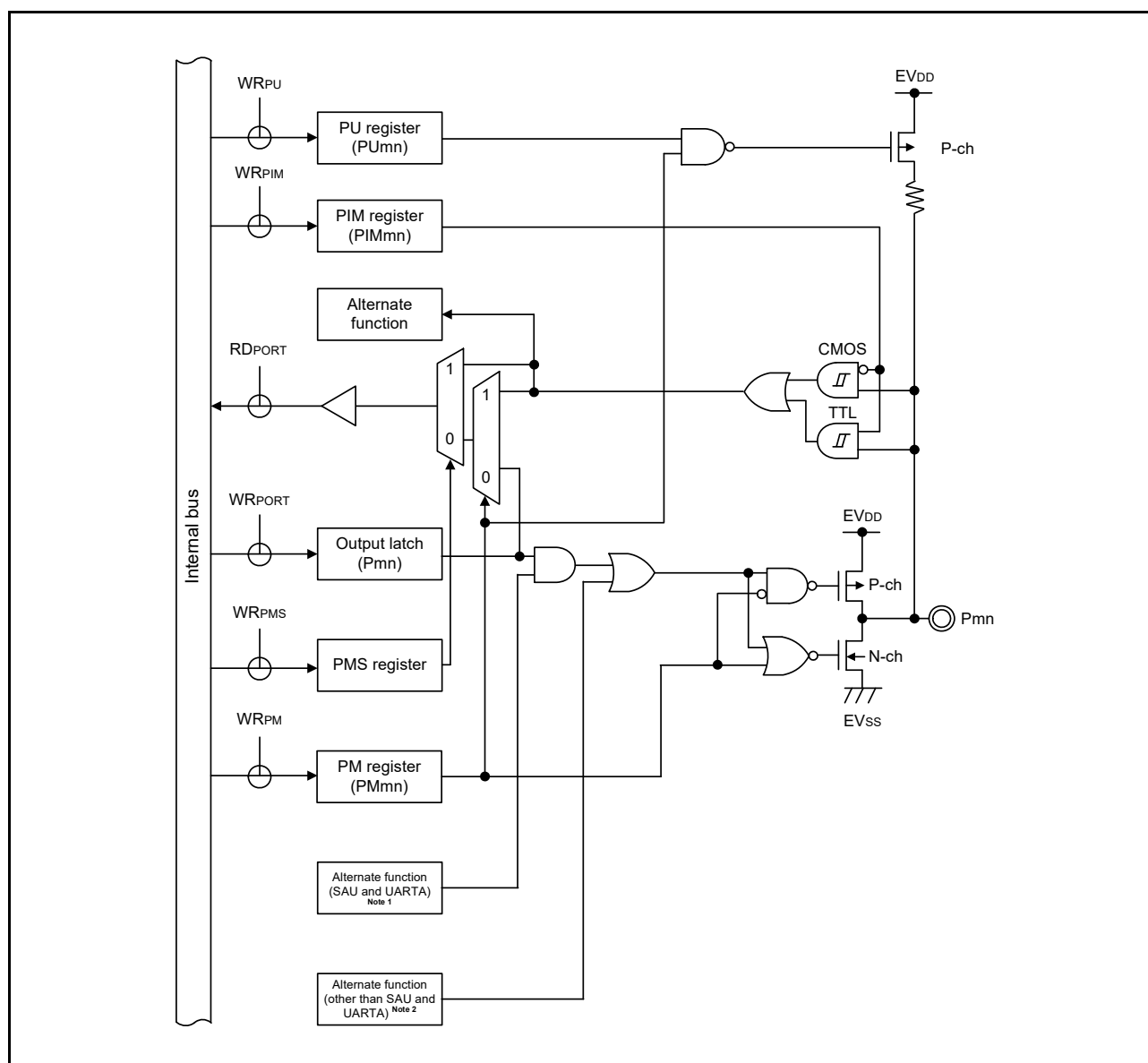
Figure 2 - 21 Pin Block Diagram for Pin Type 8-1-3
