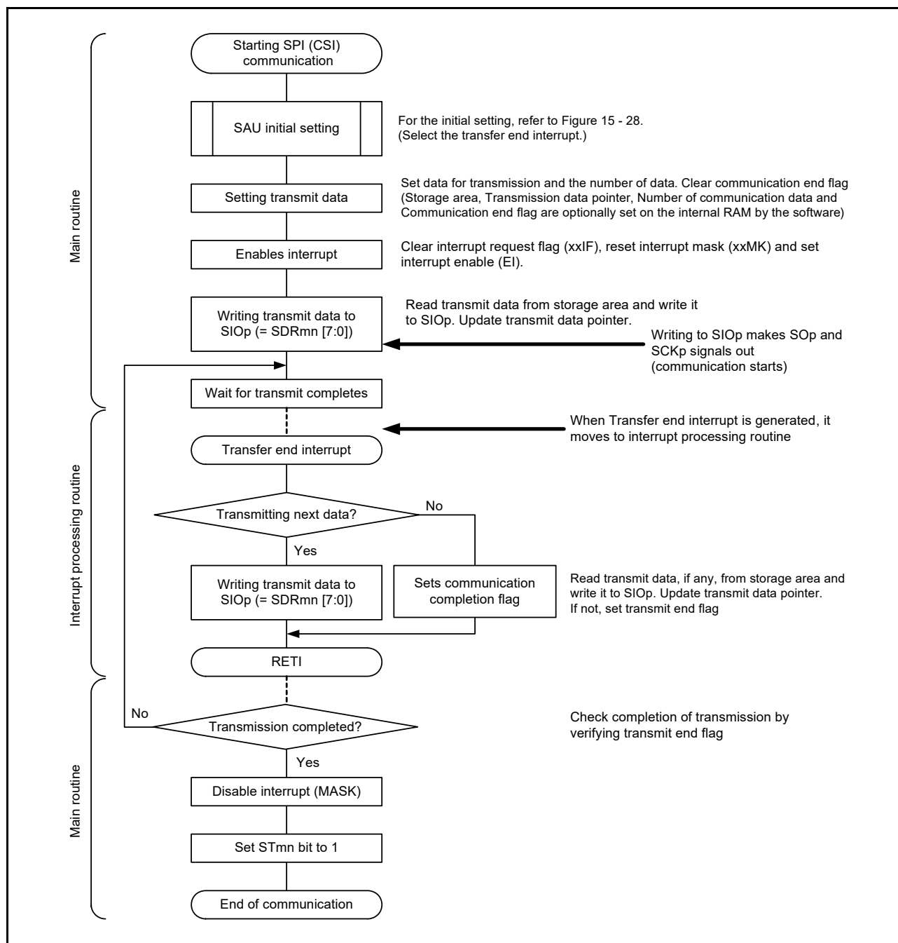
Figure 15 - 32 Flowchart of Master Transmission (in Single-Transmission Mode)
