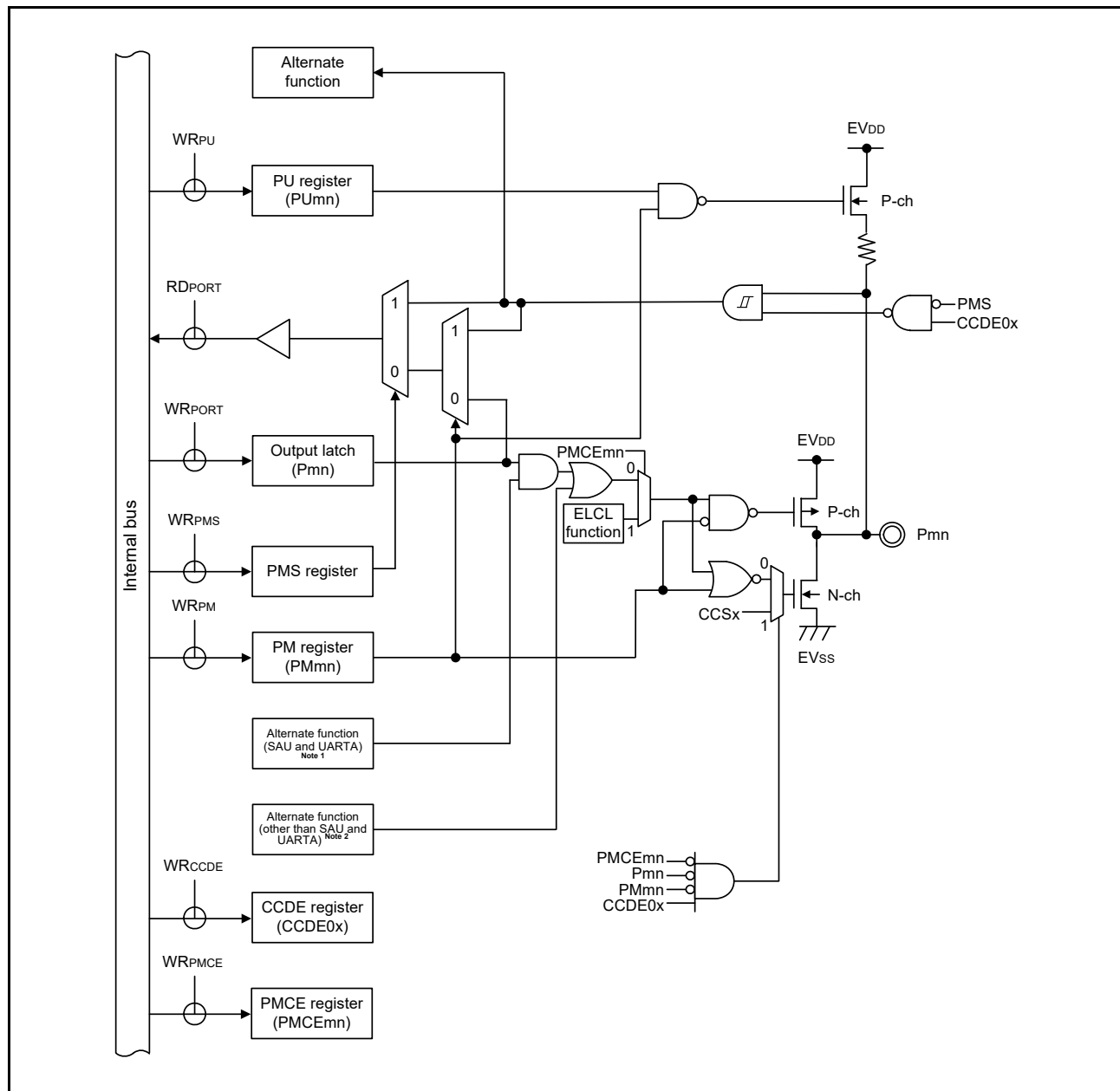
Figure 2 - 19 Pin Block Diagram for Pin Type 7-38-1
