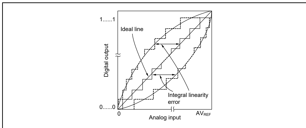
Figure 12 - 50 Integral Linearity Error
