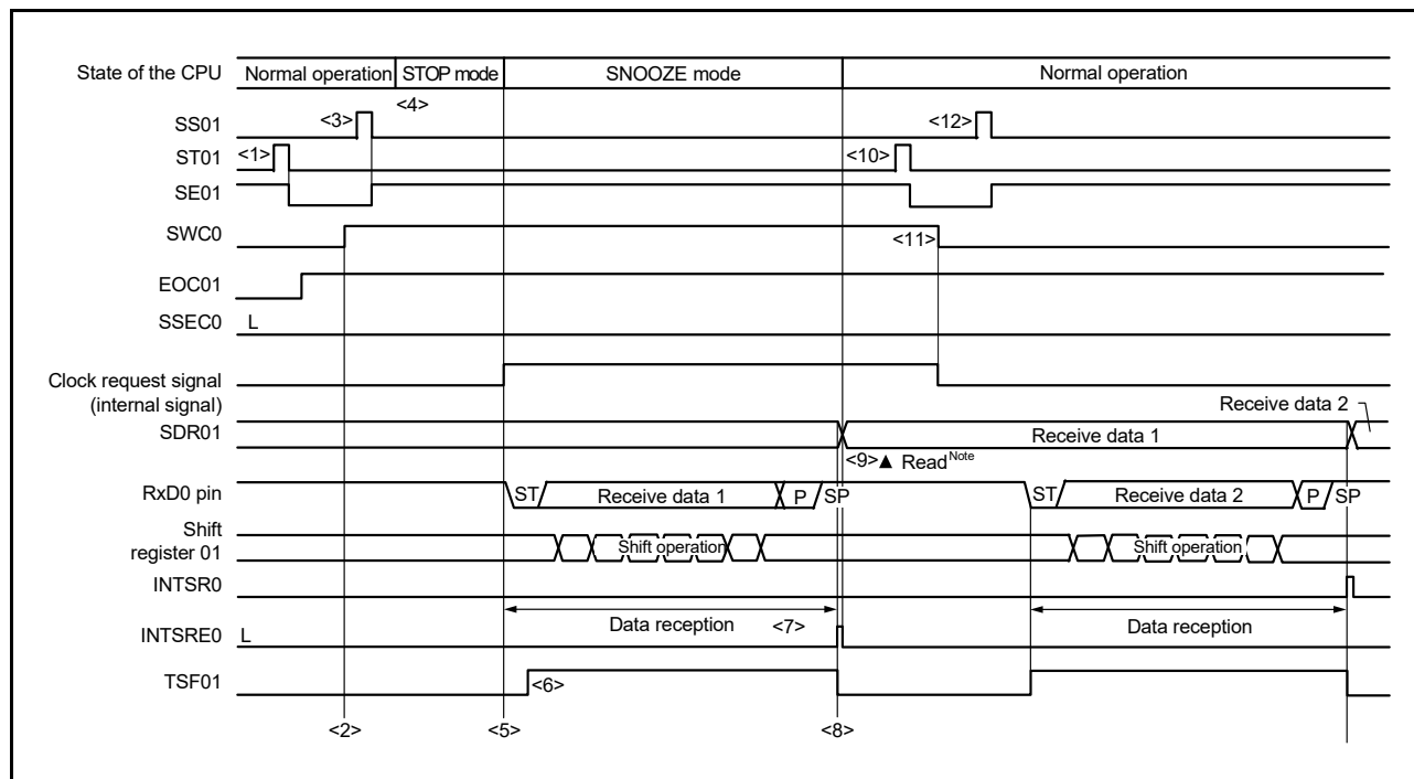
Figure 15 - 93 Timing Chart of SNOOZE Mode Operation (EOCm1 = 1, SSECm = 0)
