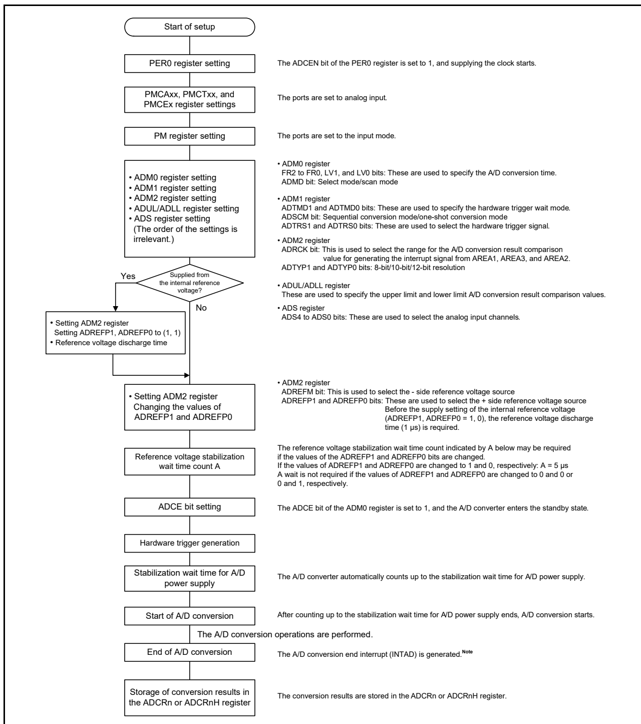
Figure 12 - 37 Setting up Hardware Trigger Wait Mode
