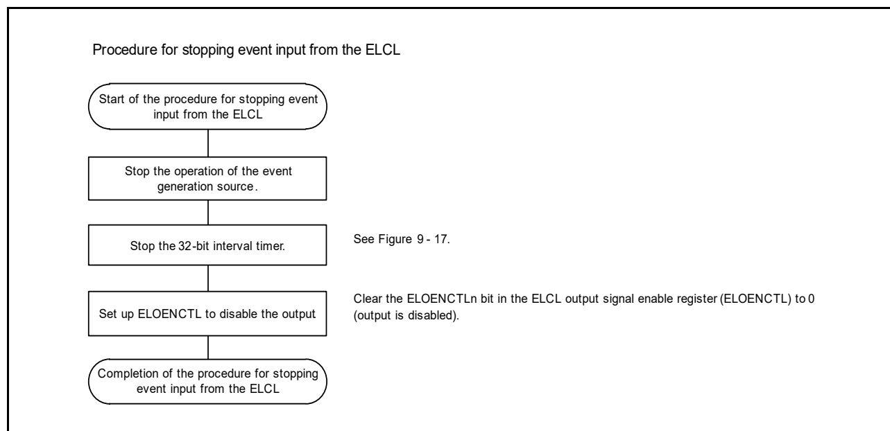
Figure 9 - 21 Procedure for Stopping Event Input from the ELCL
