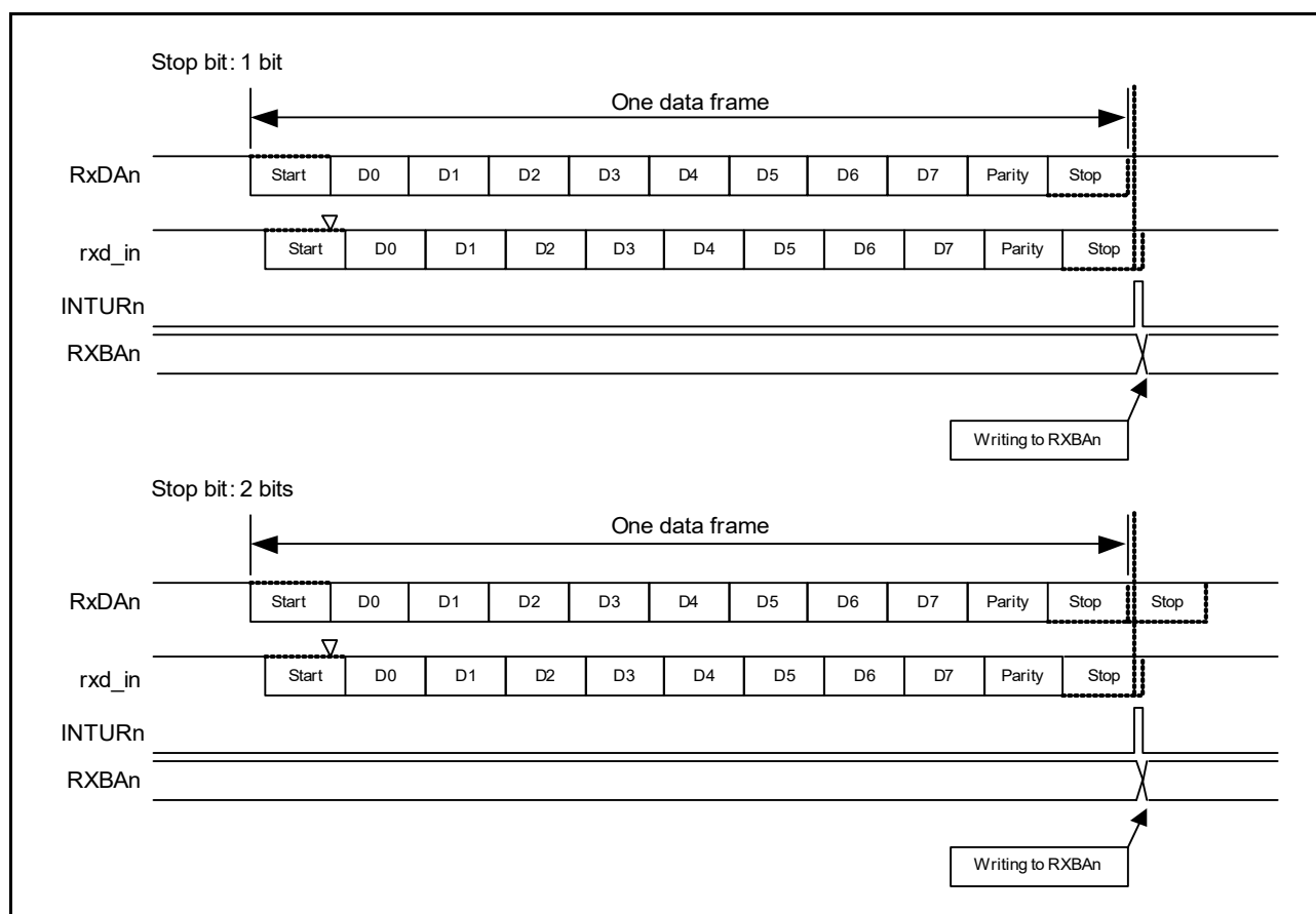
Figure 17 - 21 Timing of UART Receive Operation
