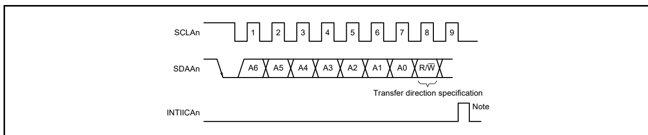
Figure 16 - 17 Transfer Direction Specification
