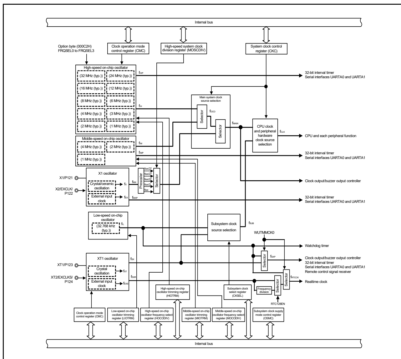
Figure 6 - 1 Block Diagram of Clock Generator
