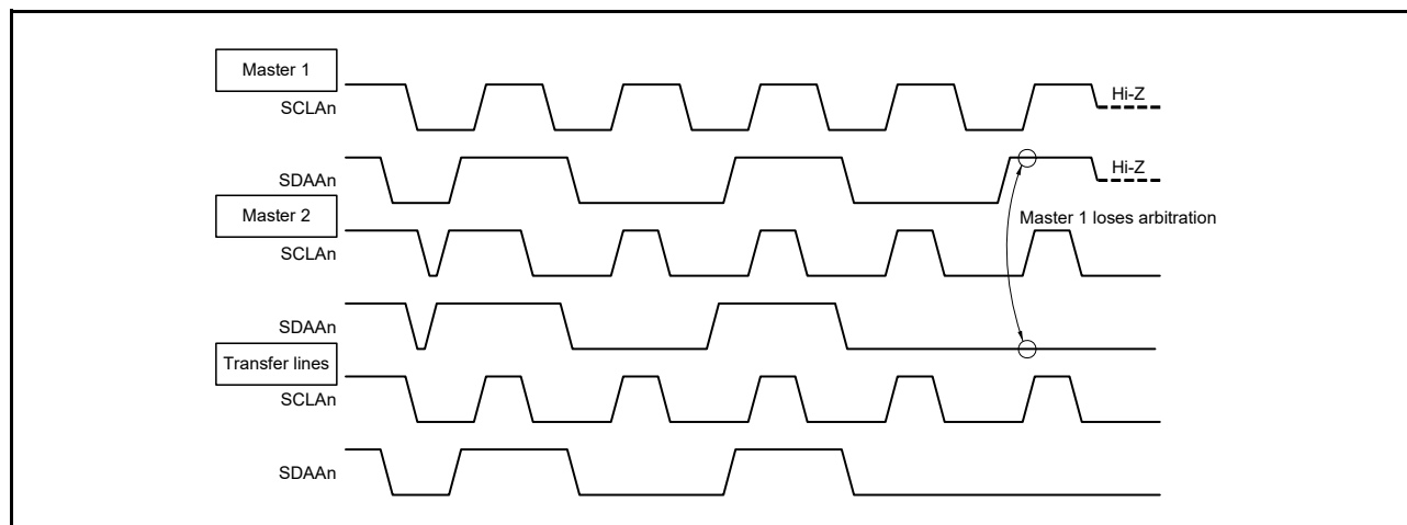
Figure 16 - 21 Arbitration Timing Example
