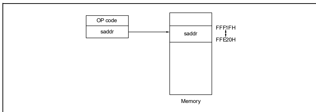
Figure 3 - 25 Outline of Short Direct Addressing
