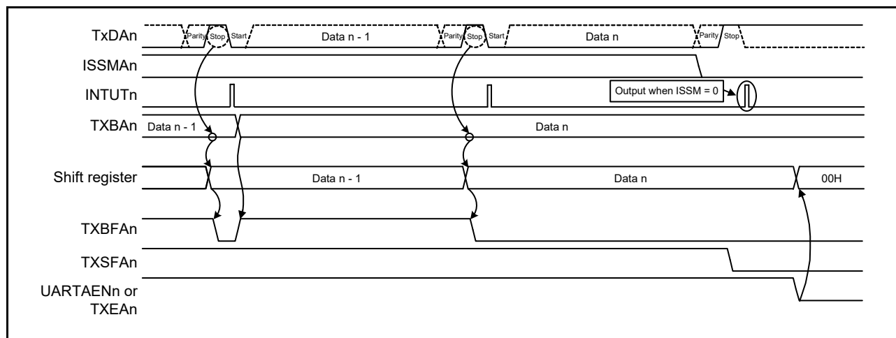
Figure 17 - 20 Timing Chart When Continuous Transmission Is Completed
