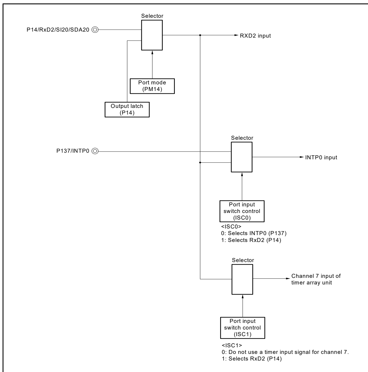
Figure 15 - 104 Port Configuration for Reception of LIN (30-, 32-, 36-, and 40-pin)
