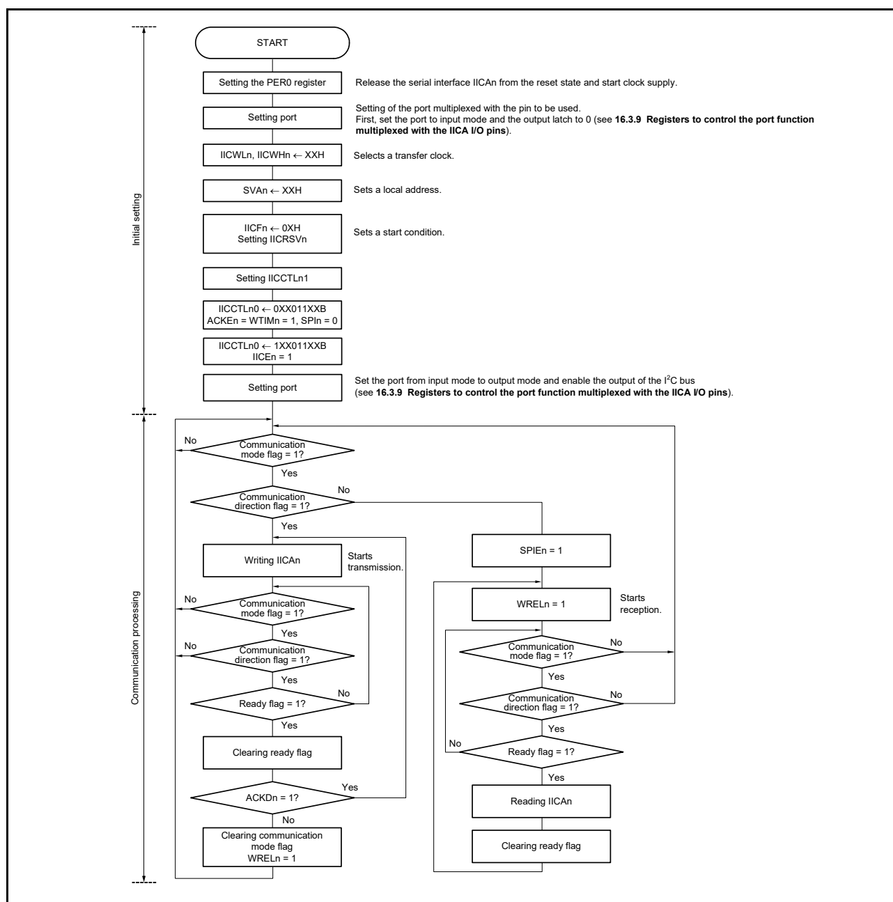
Figure 16 - 30 Slave Operation Flowchart (1)
