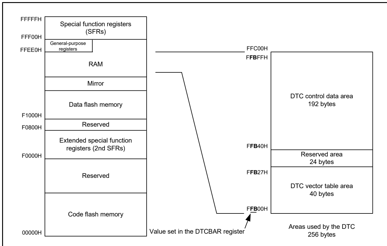
Figure 19 - 2 Memory Map Example when the DTCBAR Register is Set to FBH
