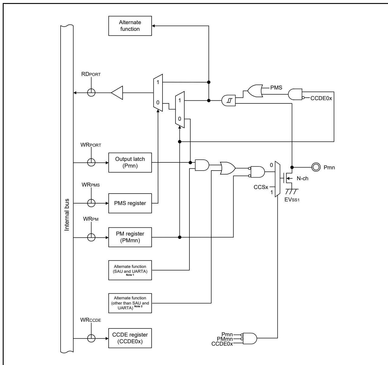
Figure 2 - 31 Pin Block Diagram for Pin Type 12-38-1
