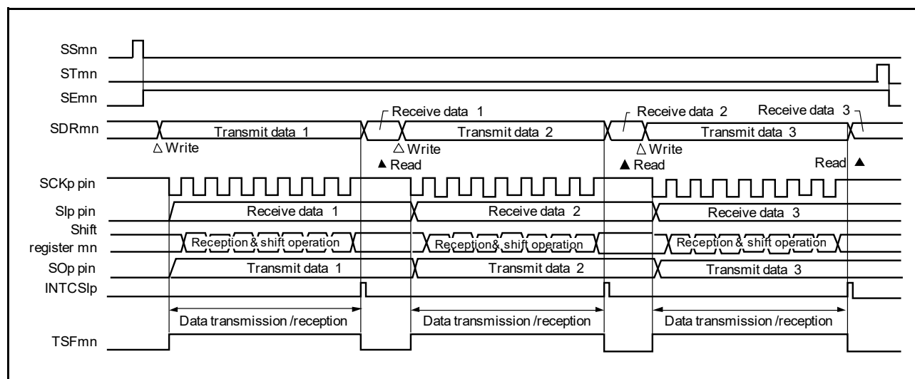
Figure 15 - 47 Timing Chart of Master Transmission/Reception (in Single-Transmission/Reception Mode) (Type 1: DAPmn = 0, CKPmn = 0)
