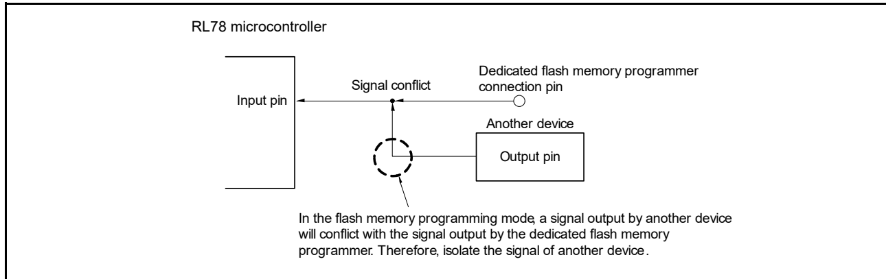
Figure 33 - 5 Signal Conflict ( \overline{\text{RESET}} Pin)
