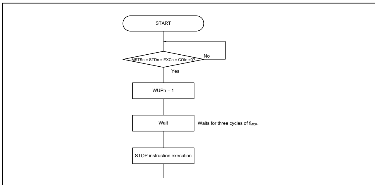
Figure 16 - 22 Flow When Setting WUPn = 1
