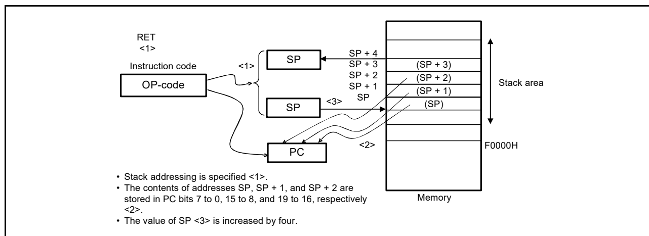
Figure 3 - 41 Example of RET
