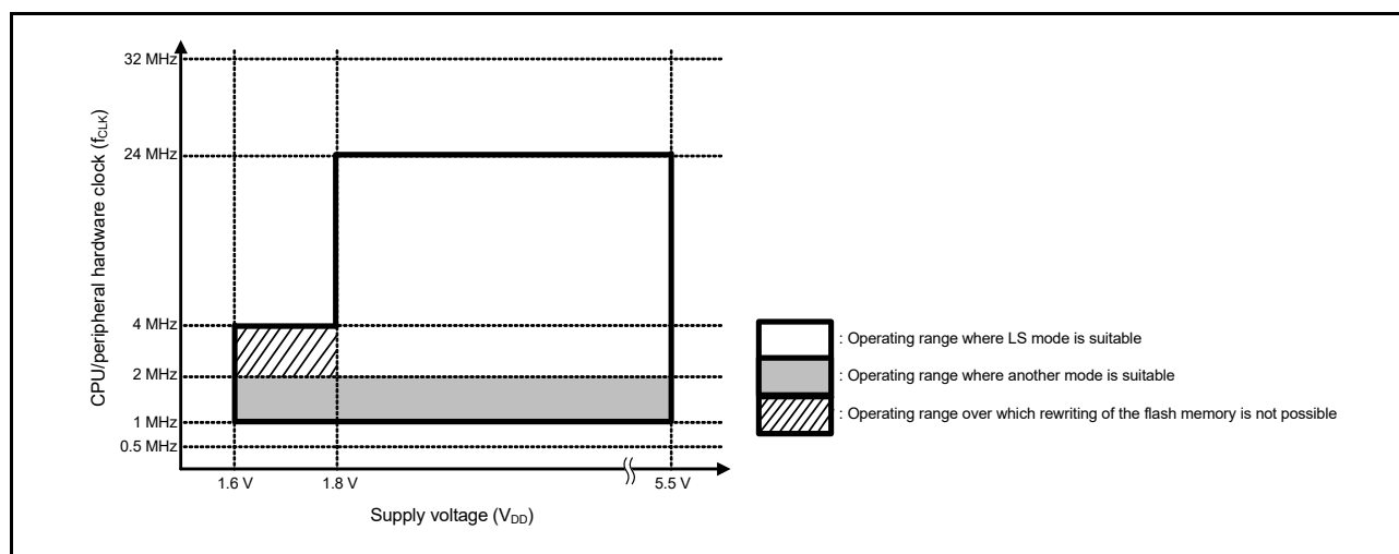
Figure 5 - 6 Operating Range in LS Mode
