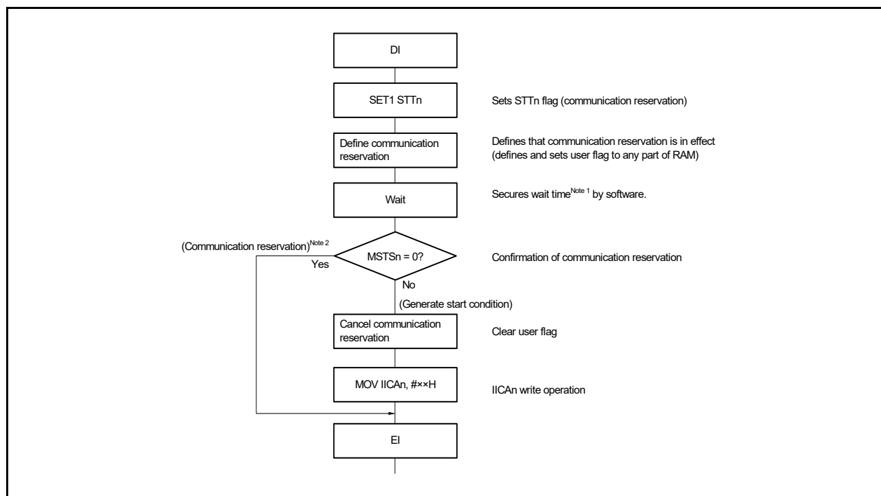
Figure 16 - 27 Communication Reservation Protocol
