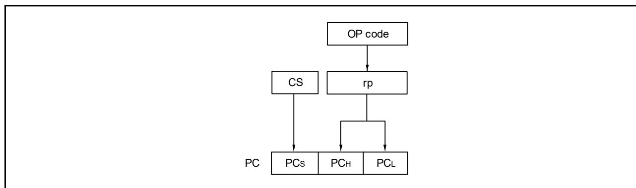
Figure 3 - 20 Outline of Register Indirect Addressing
