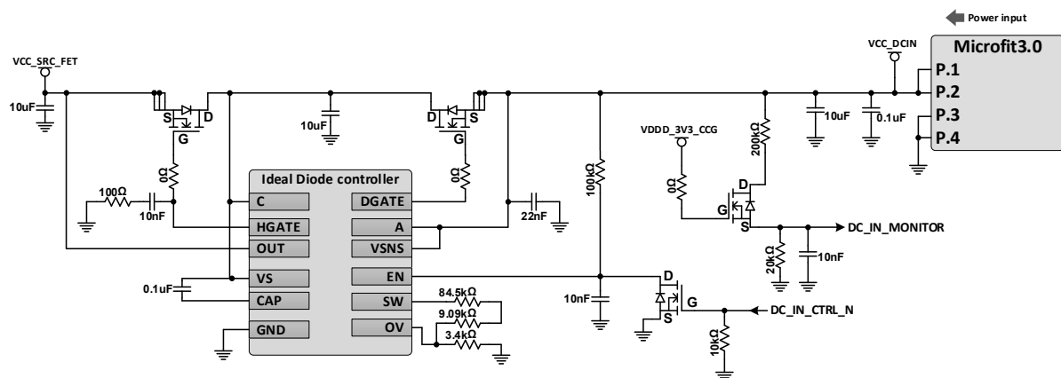
Figure 5-6. Simplified Microfit Connector Connections
