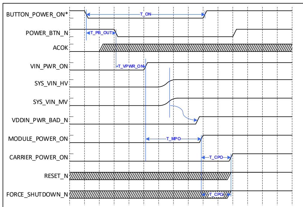
Figure 5-8. Power-OFF to On Sequence Power Button Case
