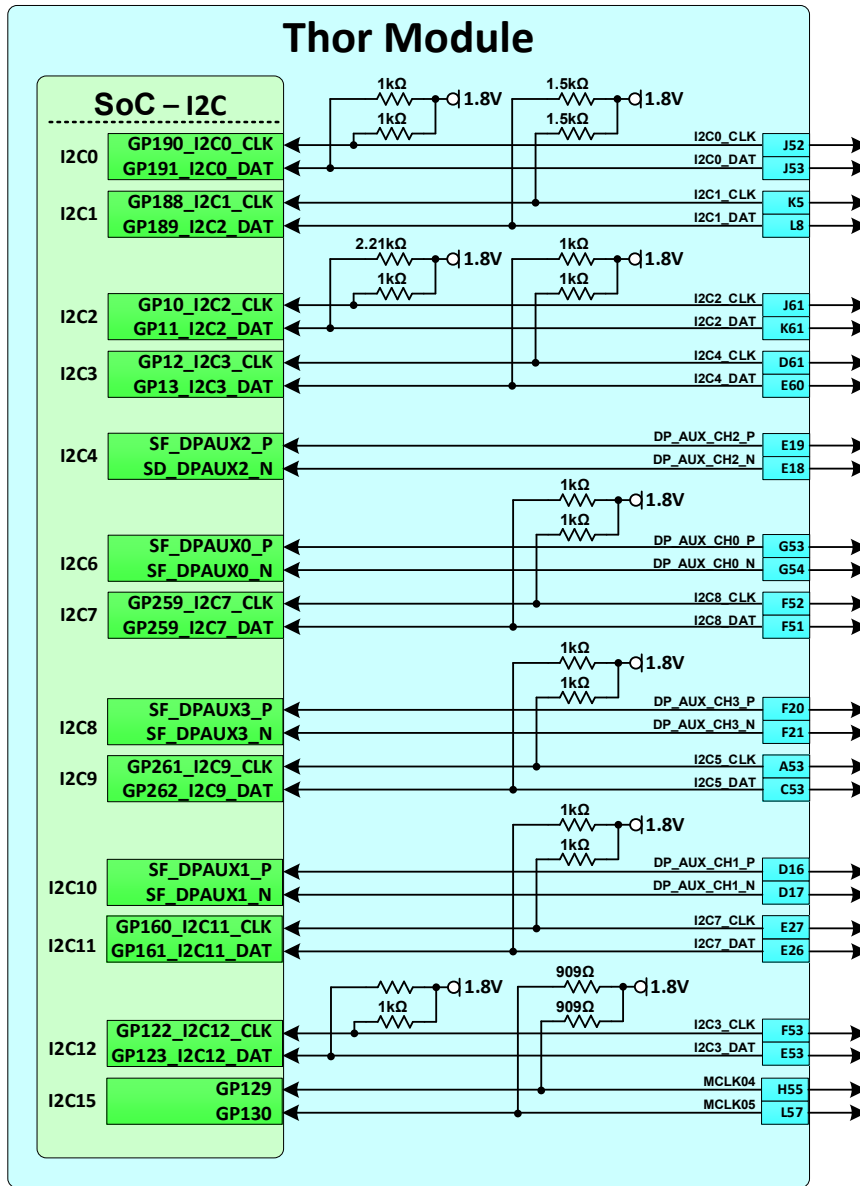
Figure 12-1. I2C Connections
