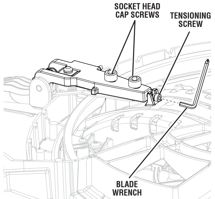
BOTTOM VIEW OF SAW
