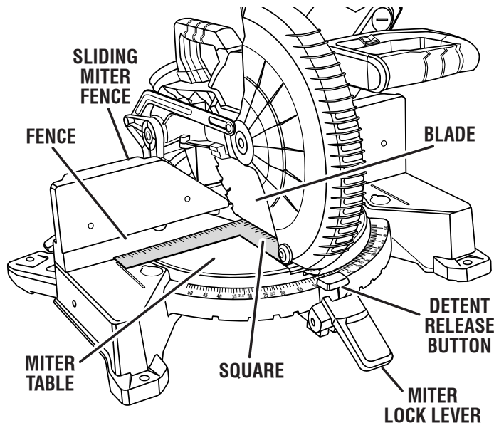
VIEW OF BLADE SQUARE WITH FENCE
