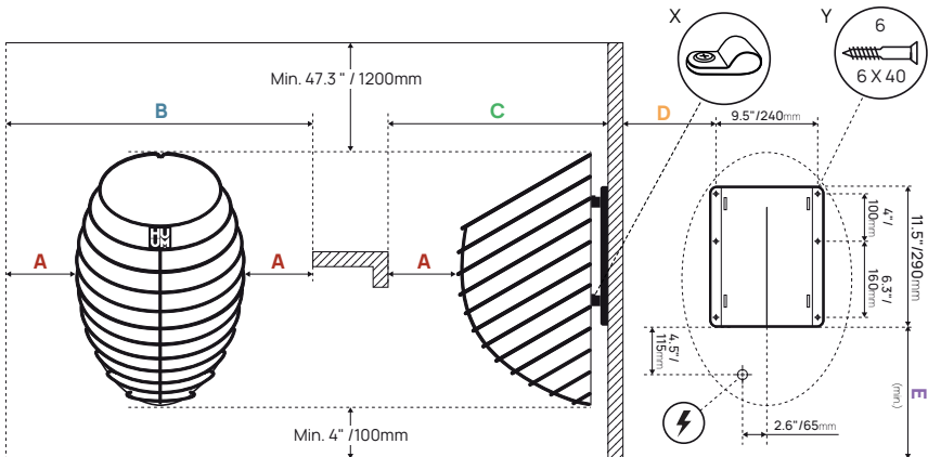
Figure 1. Positioning the heater
