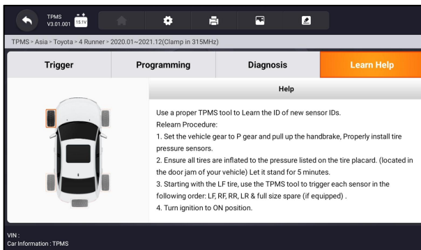
Figure 11-13 Sample OBD Learn Help Screen
