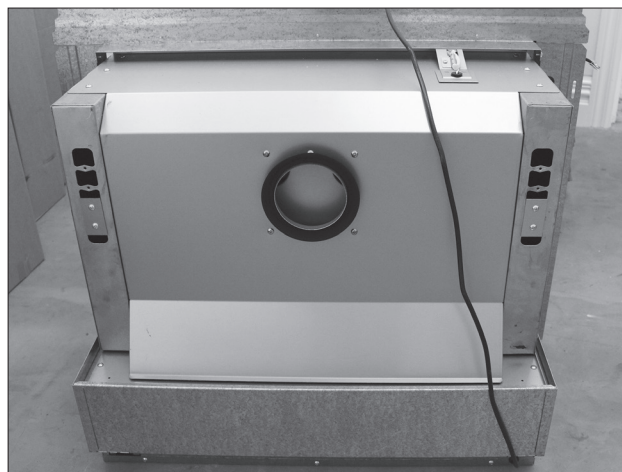
SS850 with Zero Clearance Box and adapter removed
