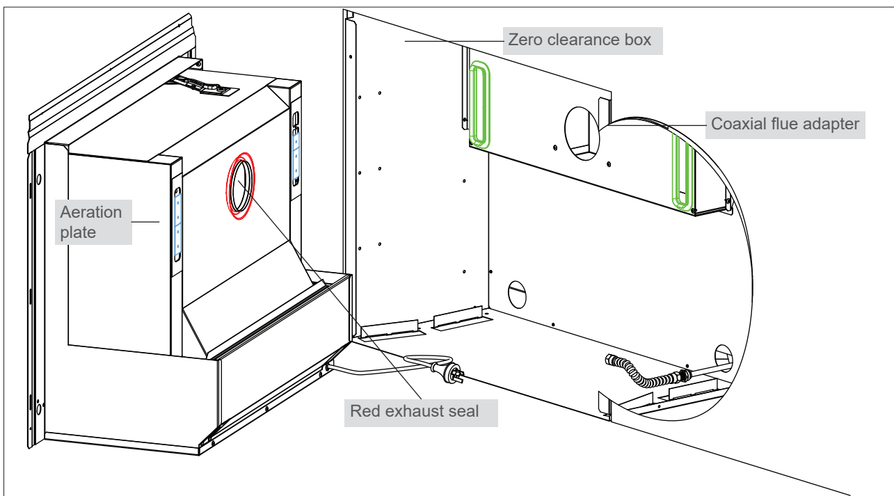
Zero Clearance Box and coaxial flue adapter
