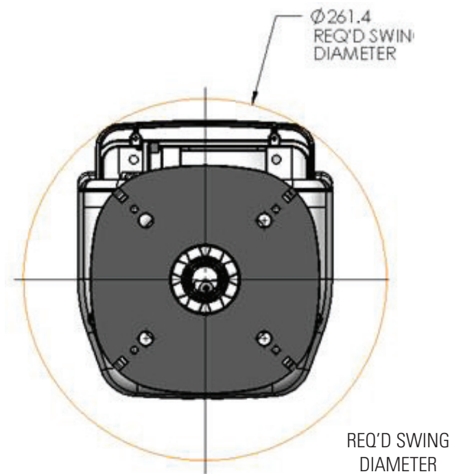
Figure 2 – Permanent Mount Golight® GT Spotlight – Bottom View Looking Up -Dimension in mm
