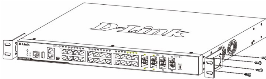
Figure 2 — Attaching rack-mount brackets to the Switch
