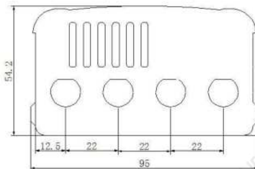
Right View
