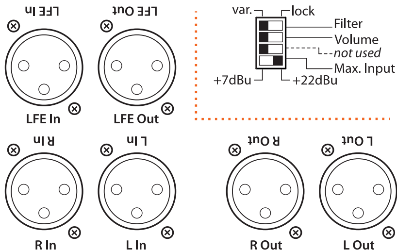
Rear Connections & DIP Switches
