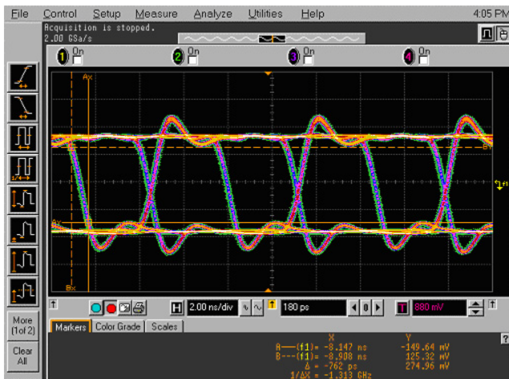
Figure 5-2 • LVDS Signal across RX Termination at 300 Mbps
