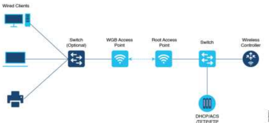
Figure 47: Example of a WGB
