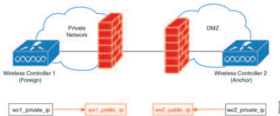
Figure 40: Mobility NAT
