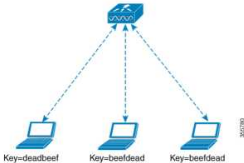
Figure 26: Multi-PSK
