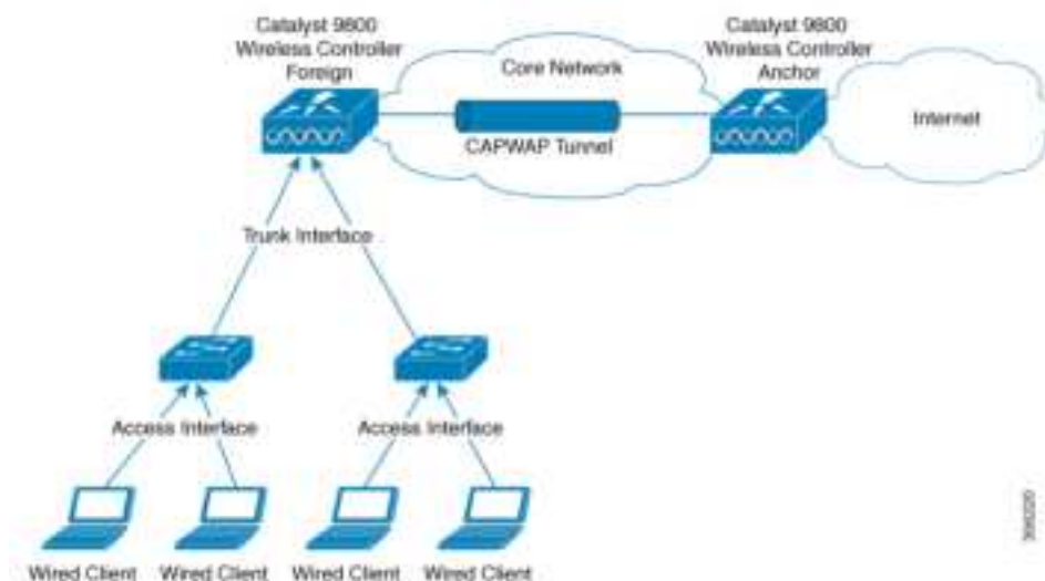
Figure 48: Guest Access Architecture
