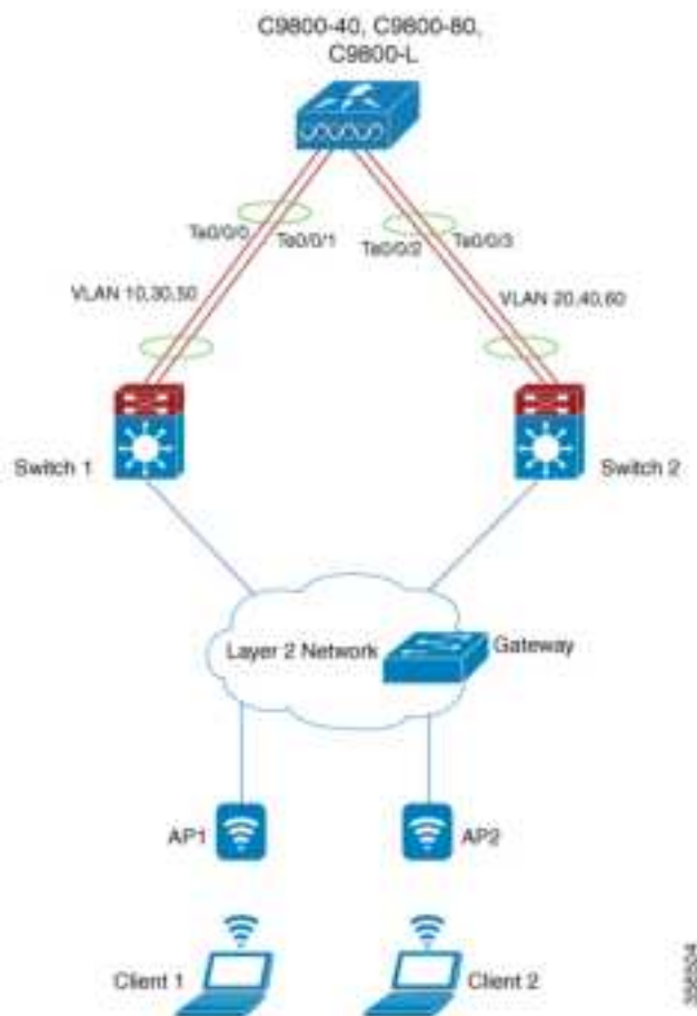
Figure 13: Single Controller with Multi-LAG
