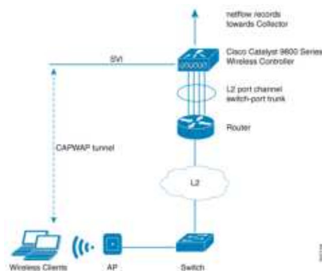
Figure 34: Encrypted Traffic Analytics Deployed on Cisco Catalyst 9800 Series Wireless Controller in Local Mode
