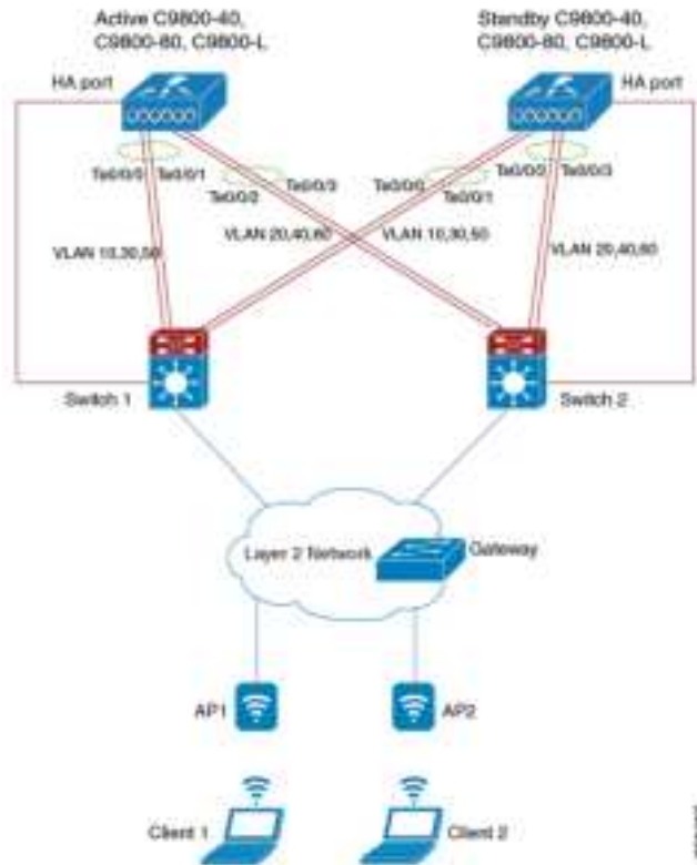
Figure 14: SSO Pair with Multi-LAG
