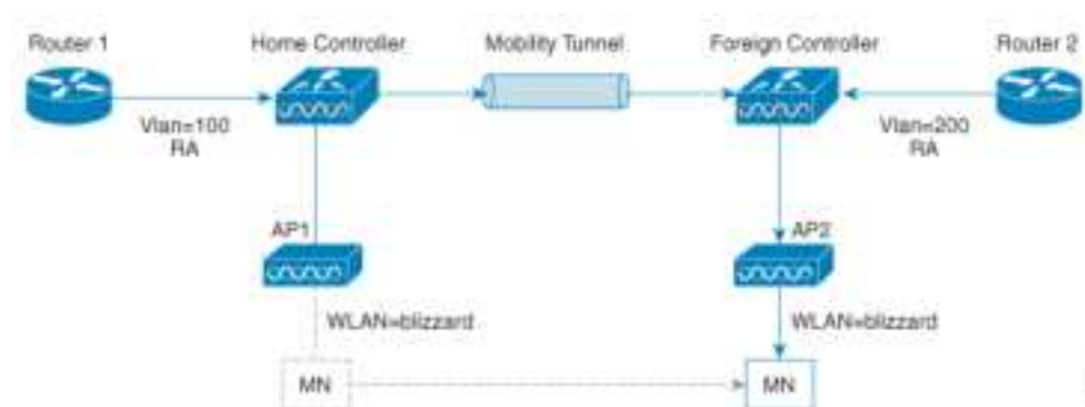
Figure 43: Roaming Client Receives Valid RA from Router 1
